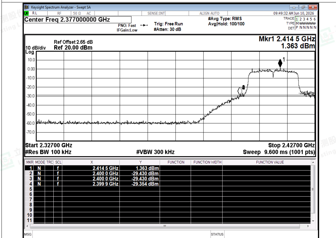
Band Edge NVNT n20 2412MHz Ant1 Emission
