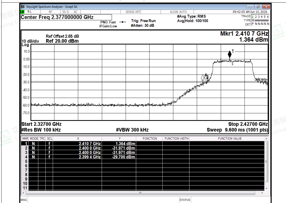
Band Edge NVNT g 2412MHz Ant1 Emission
