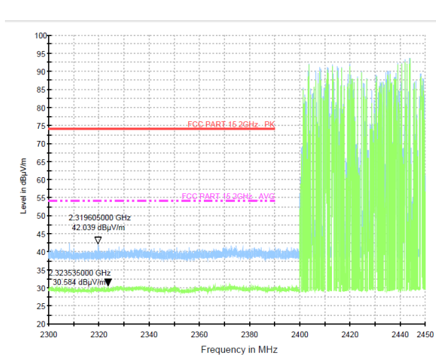
Test Mode: GFSK-Low Hopping-on
