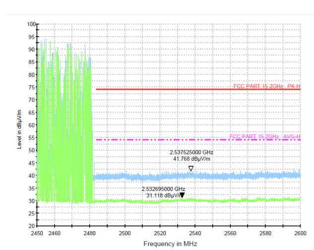
Test Mode: GFSK-High Hopping-on
