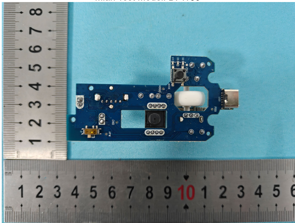
Photo 3 Internal photos of EUT Mian Test Model: DI-W30
