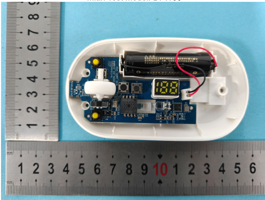
Photo 2 Internal photos of EUT Mian Test Model: DI-W30
