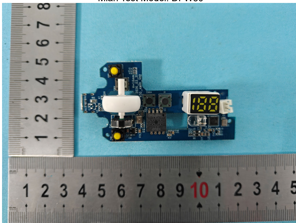
Photo 4 Internal photos of EUT Mian Test Model: DI-W30
