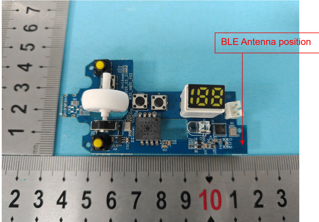
Photo 5 Internal photos of EUT Mian Test Model: DI-W30
