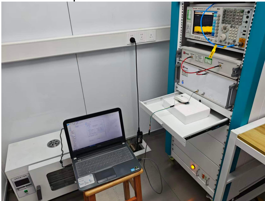
Photo 3 Test Setup Photos of Connect EUT Antenna Terminal Test
