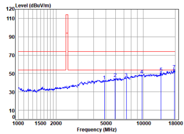
2.4G SRD_TX_CH_M_Vertical
