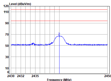
2.4G SRD_TX_CH_M_Vertical
