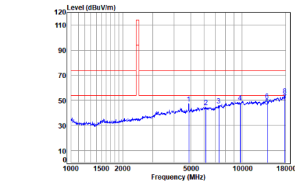
2.4G SRD_TX_CH_M_Horizontal
