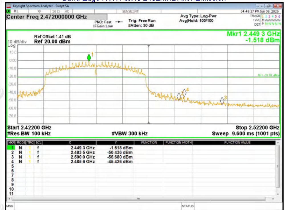
Band Edge NVNT ax40 2452MHz Ant1 Emission
