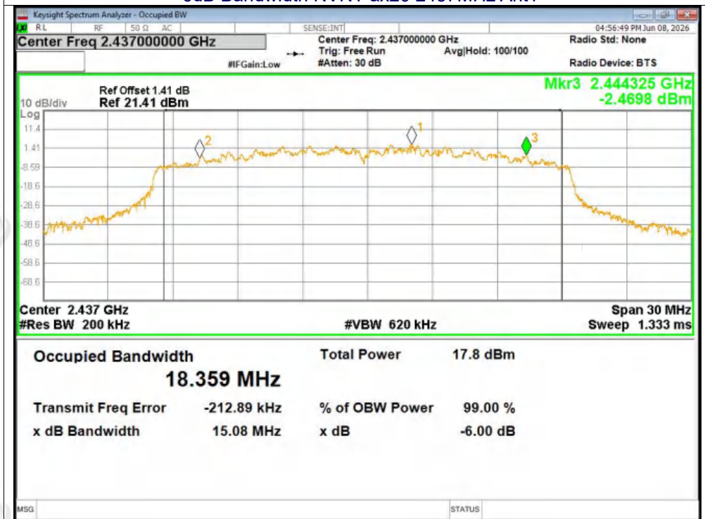
-6dB Bandwidth NVNT ax20 2437MHz Ant1
