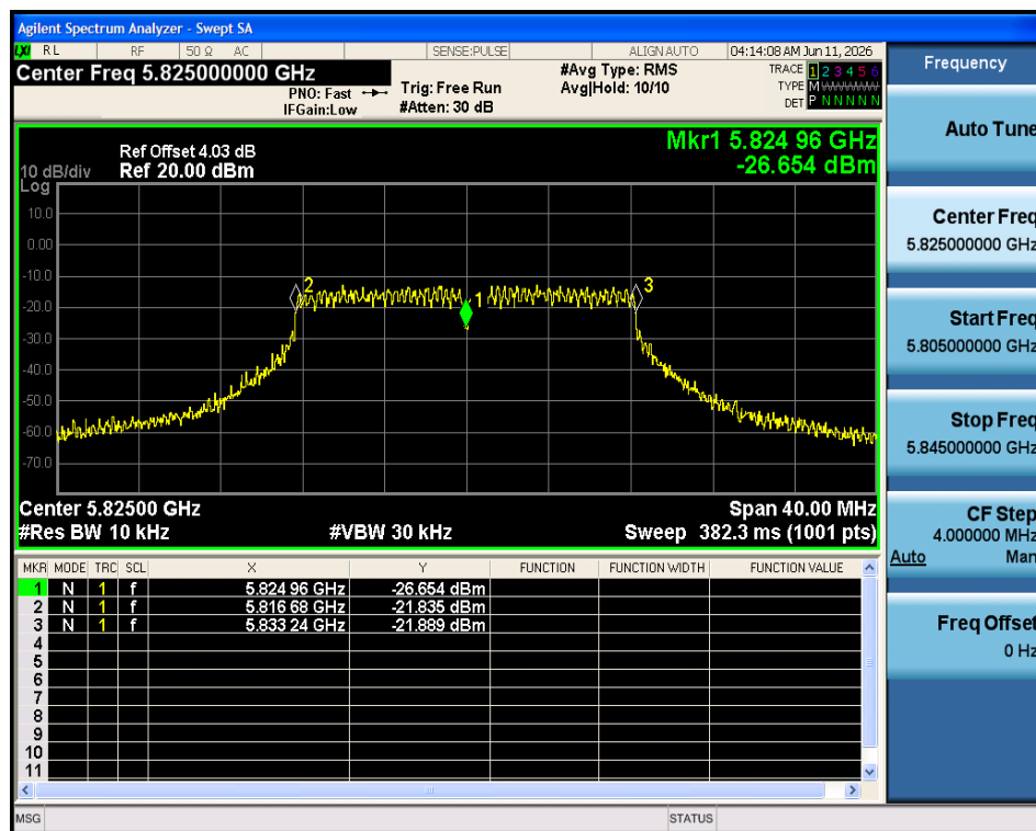
Freq. Stability -20C 5V a 5825MHz Ant1
