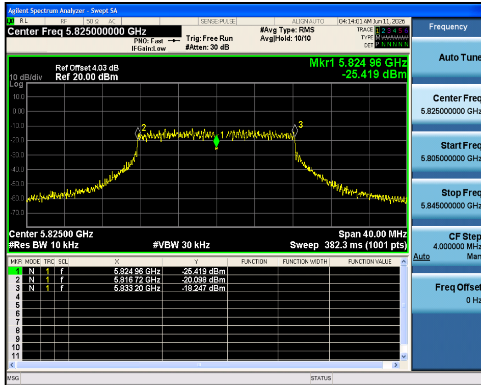
Freq. Stability 20C 5.75V a 5825MHz Ant1
