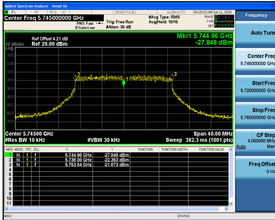
Freq. Stability -10C 5V n20 5745MHz Ant1
