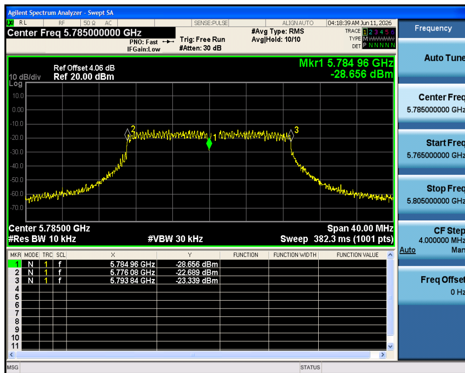
Freq. Stability 20C 5V n20 5785MHz Ant1
