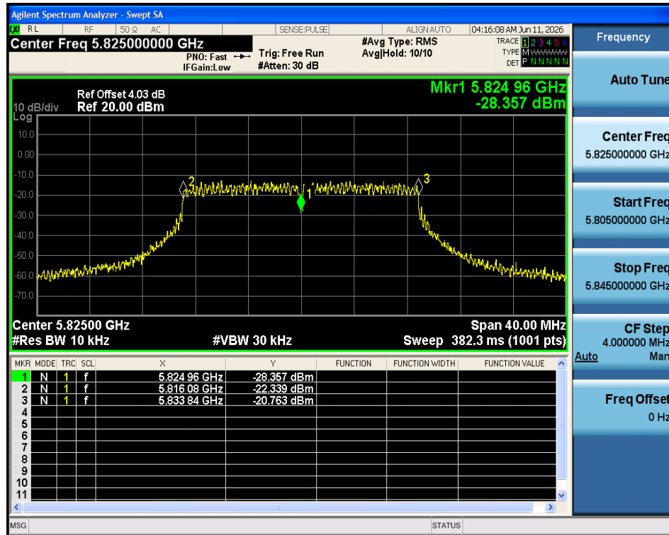
Freq. Stability 20C 5.75V n20 5825MHz Ant1
