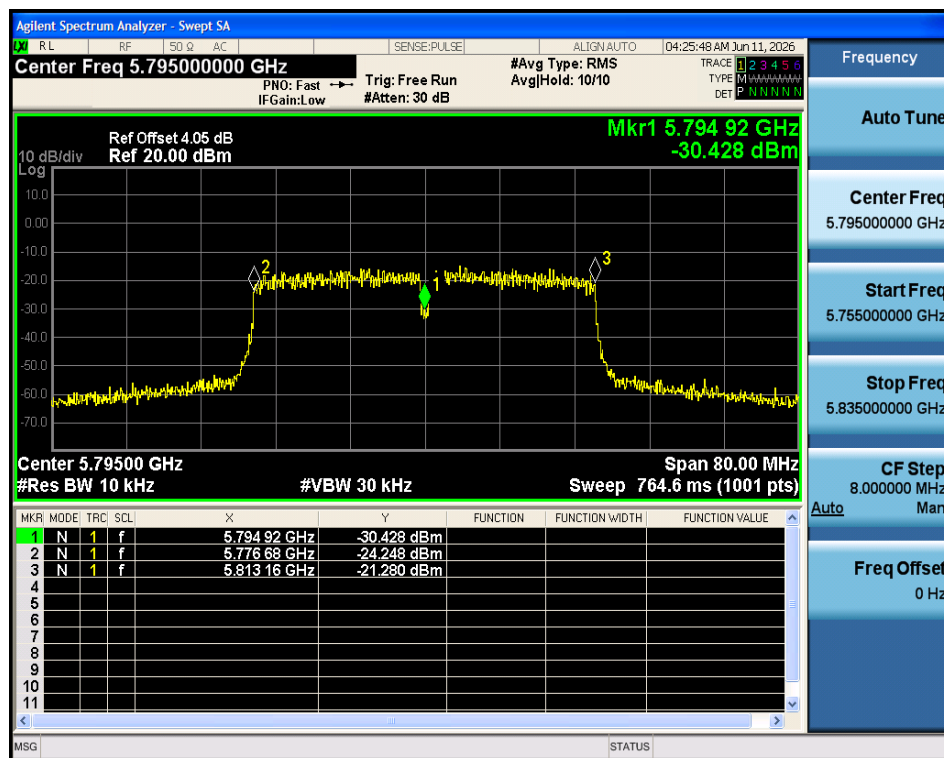
Freq. Stability 0C 5V n40 5795MHz Ant1
