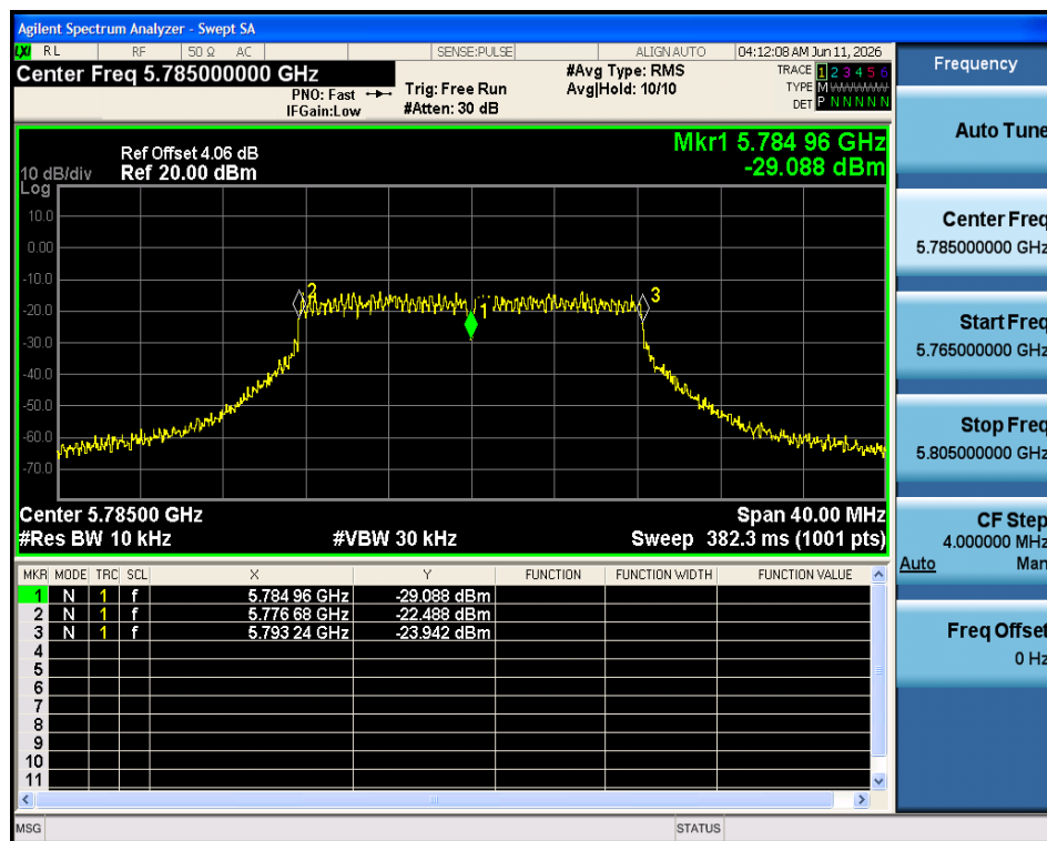
Freq. Stability 50C 5V a 5785MHz Ant1
