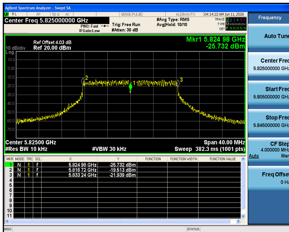
Freq. Stability 0C 5V a 5825MHz Ant1
