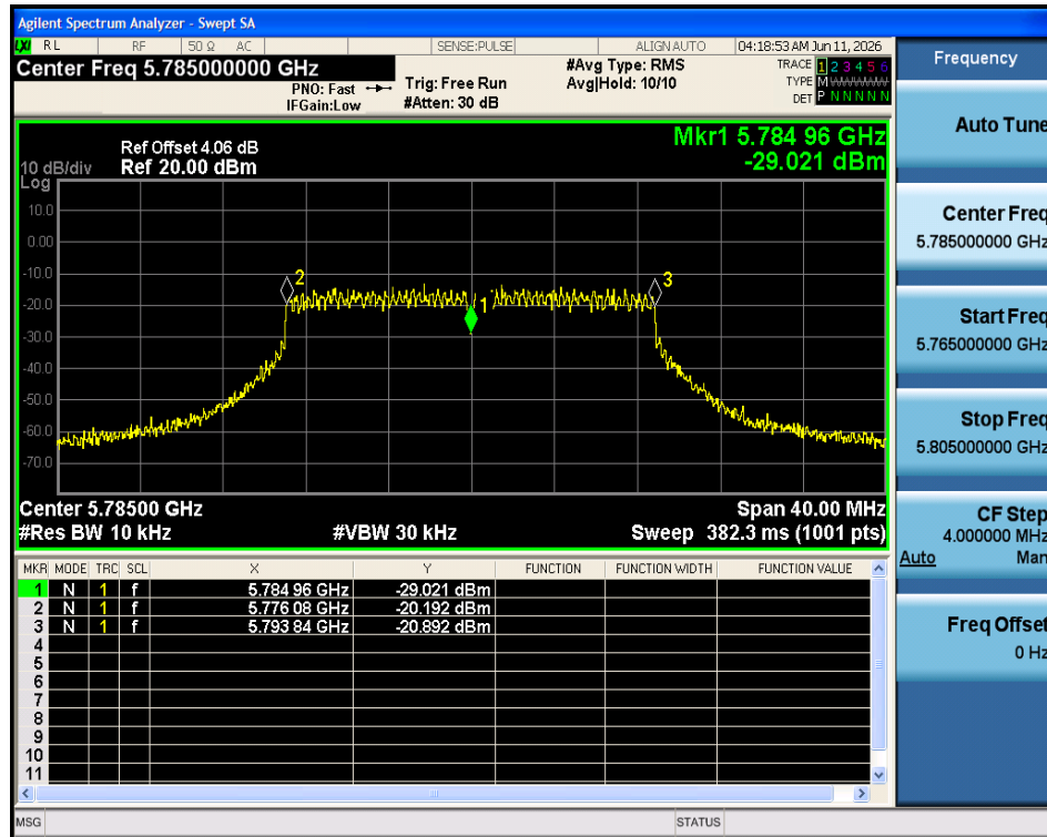
Freq. Stability 40C 5V n20 5785MHz Ant1
