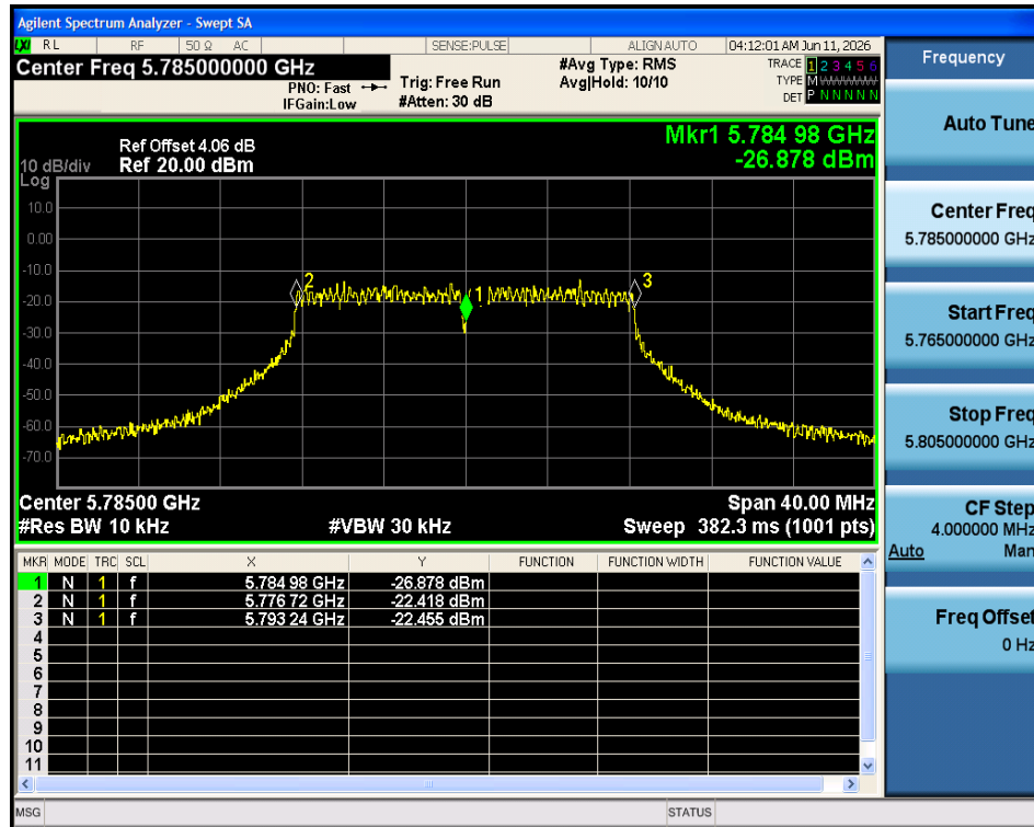
Freq. Stability 40C 5V a 5785MHz Ant1
