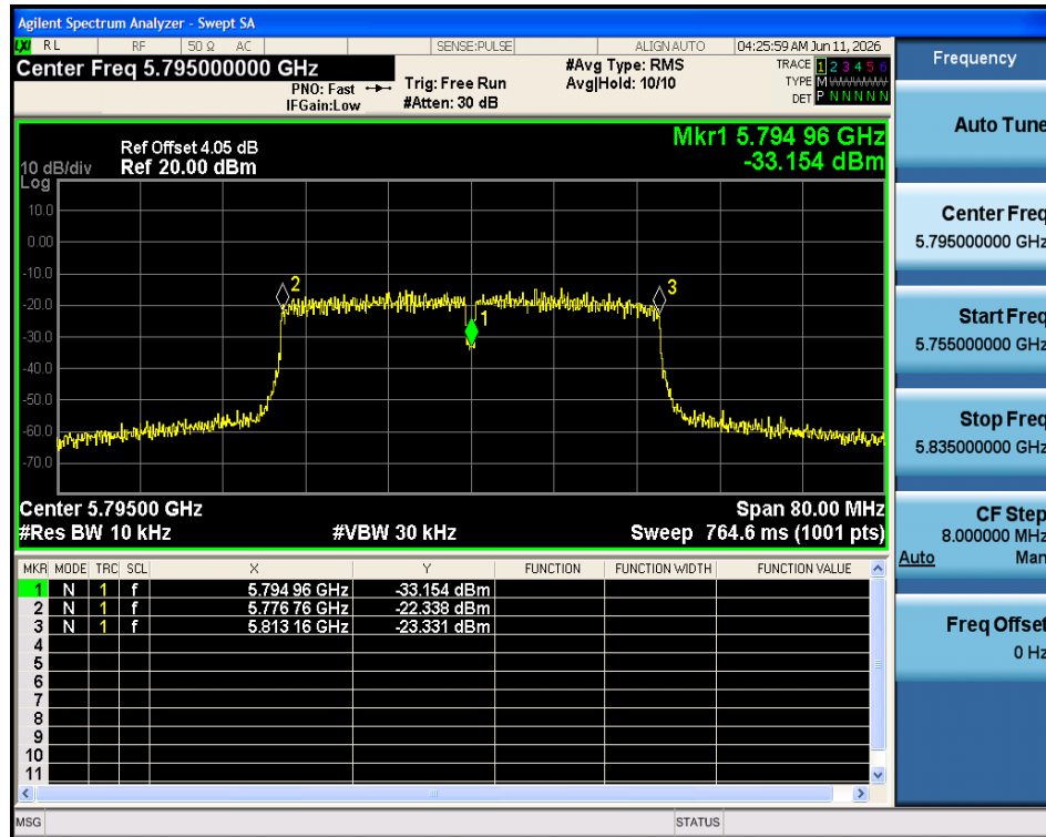
Freq. Stability 10C 5V n40 5795MHz Ant1
