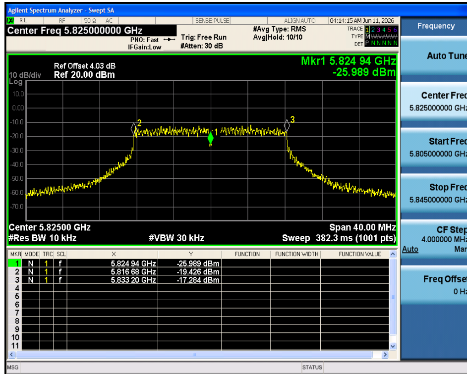
Freq. Stability -10C 5V a 5825MHz Ant1
