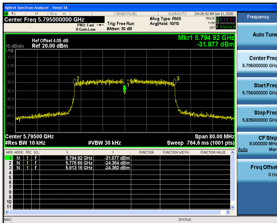
Freq. Stability 50C 5V n40 5795MHz Ant1
