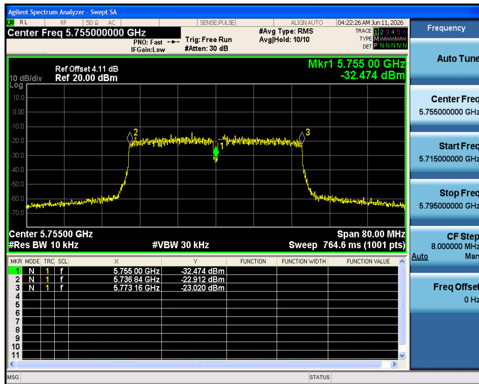
Freq. Stability -10C 5V n40 5755MHz Ant1
