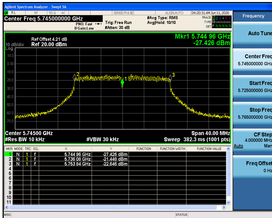
Freq. Stability 30C 5V n20 5745MHz Ant1
