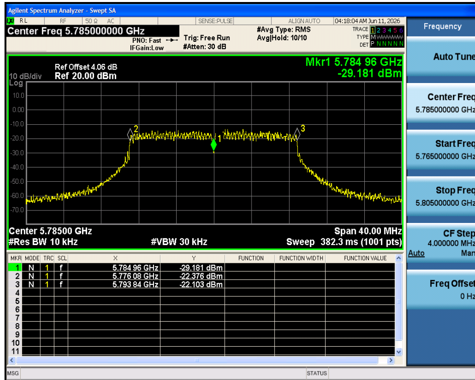
Freq. Stability 20C 5.75V n20 5785MHz Ant1
