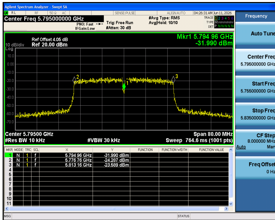
Freq. Stability 40C 5V n40 5795MHz Ant1
