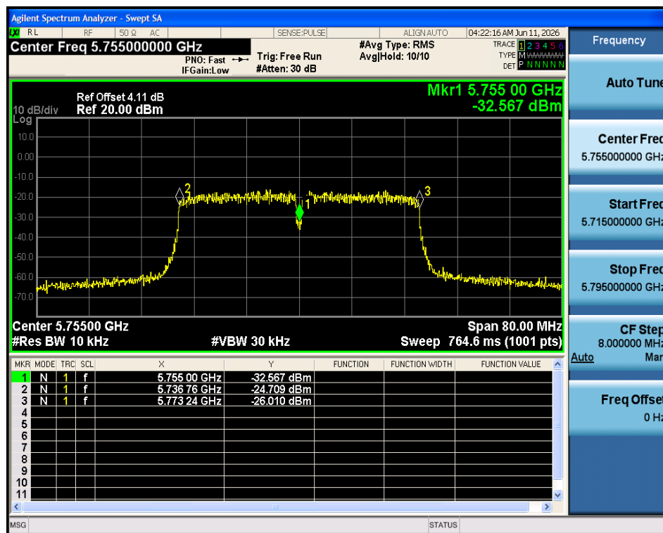
Freq. Stability -20C 5V n40 5755MHz Ant1
