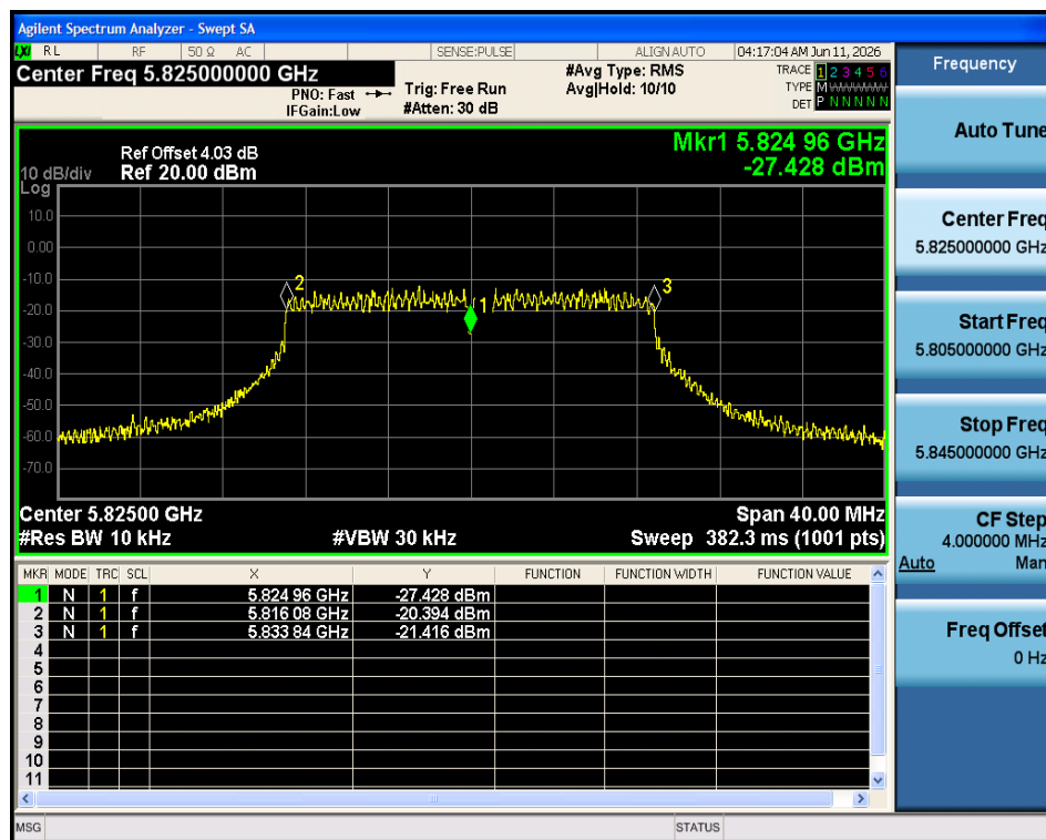
Freq. Stability 50C 5V n20 5825MHz Ant1
