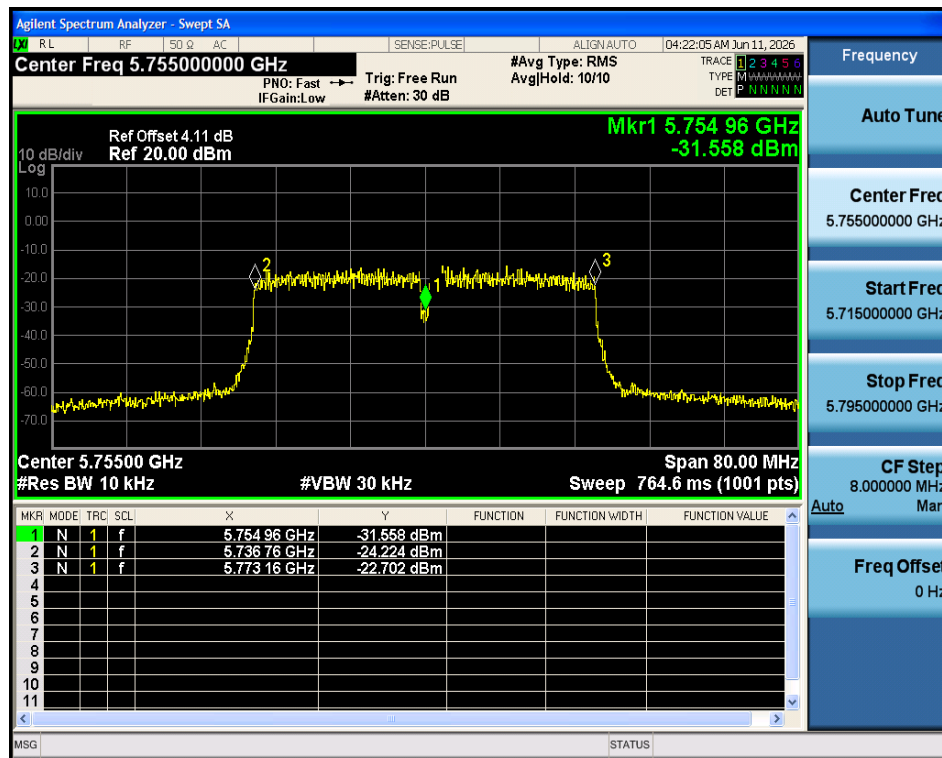
Freq. Stability 20C 5.75V n40 5755MHz Ant1
