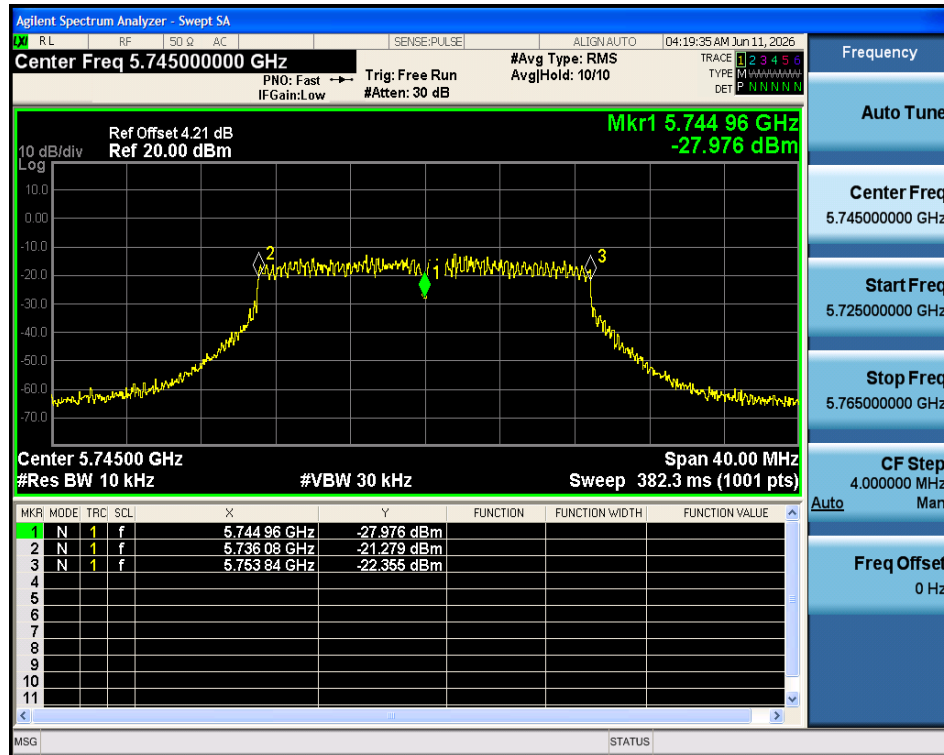
Freq. Stability 20C 4.25V n20 5745MHz Ant1
