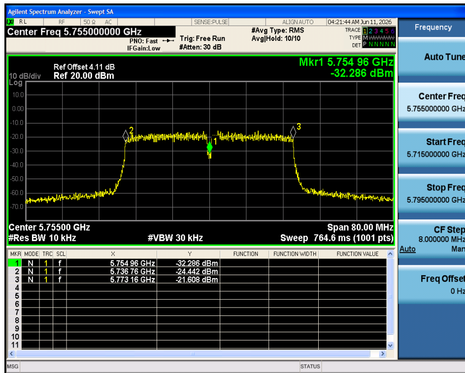
Freq. Stability 20C 4.25V n40 5755MHz Ant1
