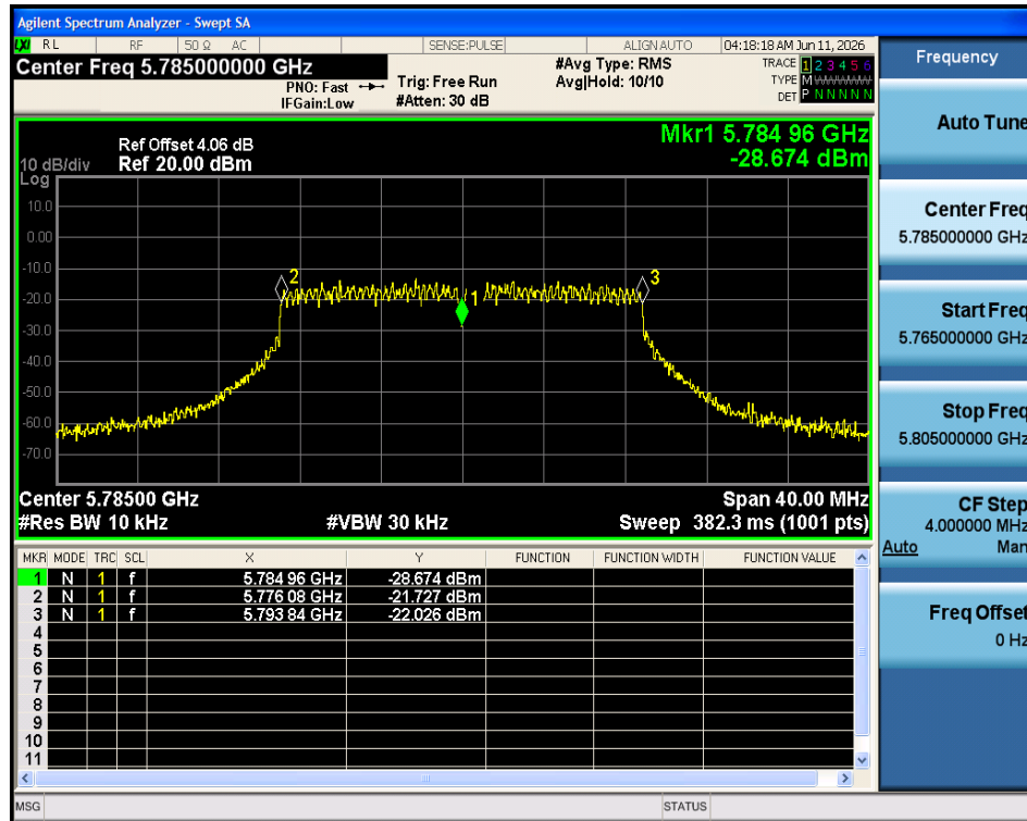
Freq. Stability -10C 5V n20 5785MHz Ant1
