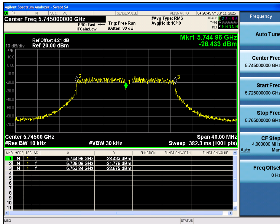
Freq. Stability 50C 5V n20 5745MHz Ant1
