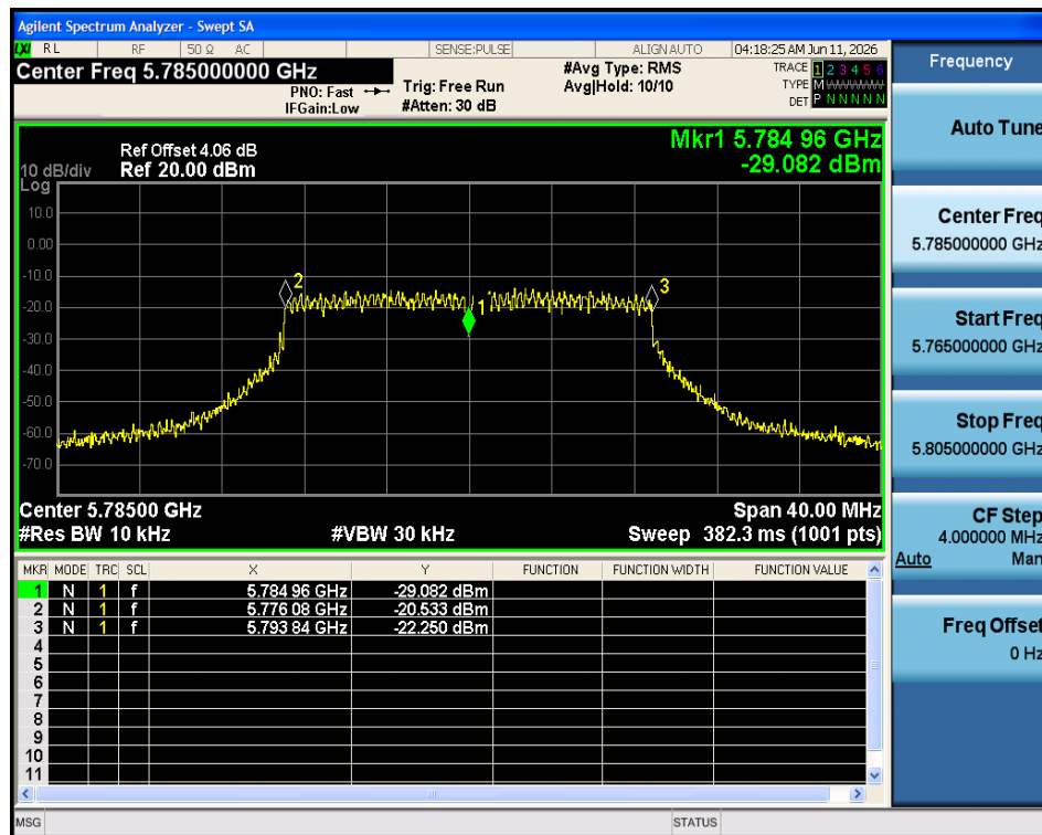
Freq. Stability 0C 5V n20 5785MHz Ant1
