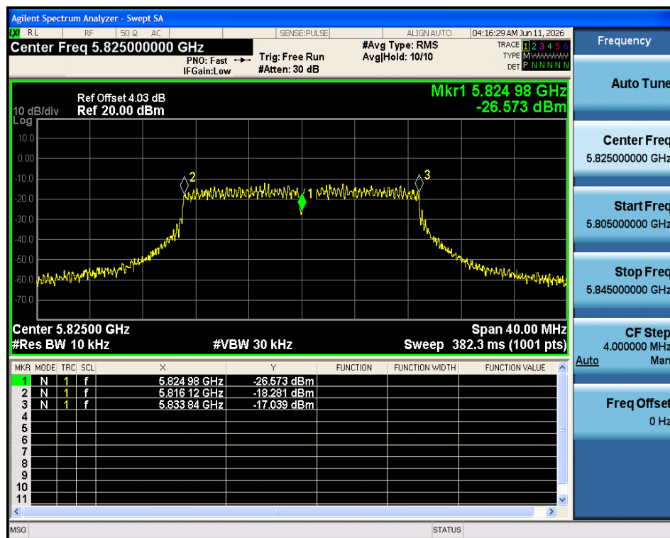
Freq. Stability 0C 5V n20 5825MHz Ant1
