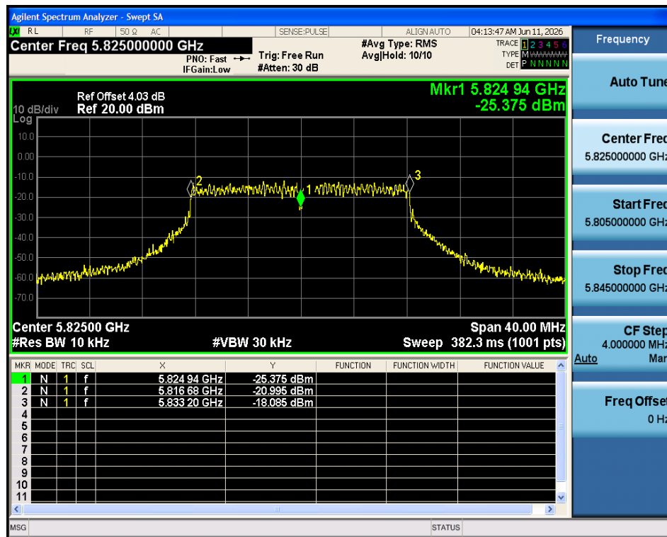
Freq. Stability 20C 4.25V a 5825MHz Ant1
