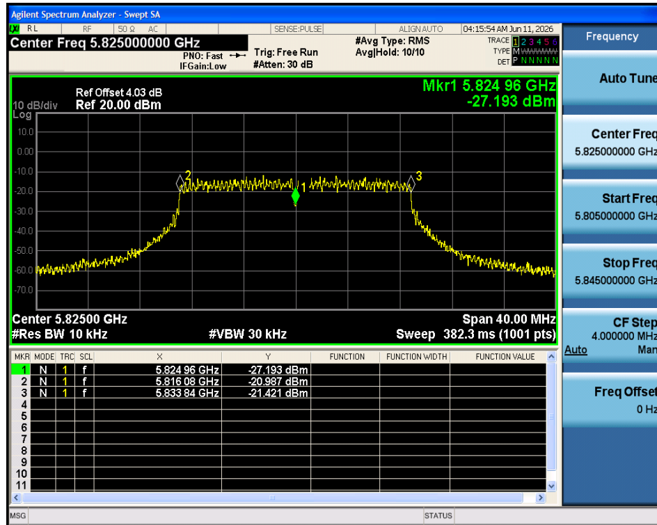
Freq. Stability 20C 4.25V n20 5825MHz Ant1
