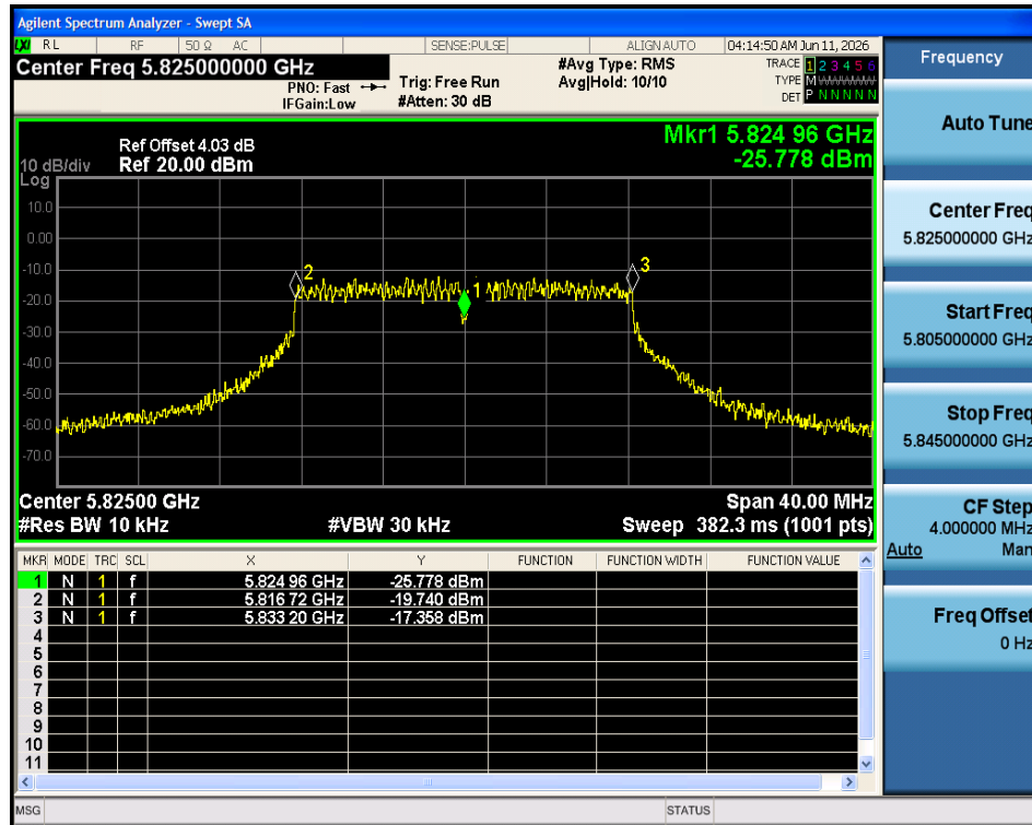
Freq. Stability 40C 5V a 5825MHz Ant1
