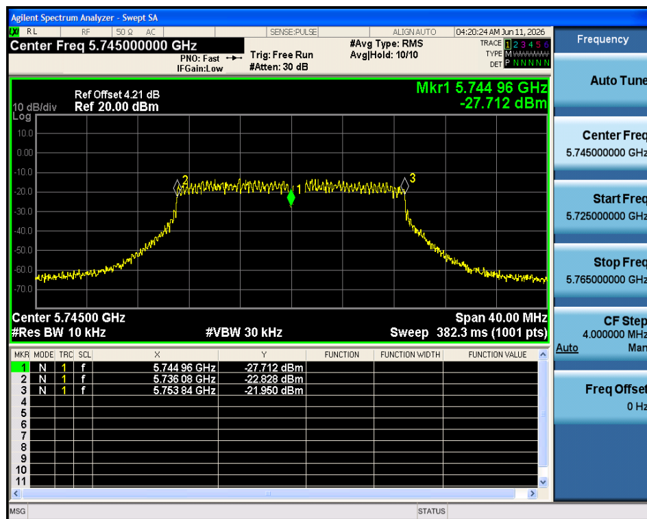
Freq. Stability 20C 5V n20 5745MHz Ant1
