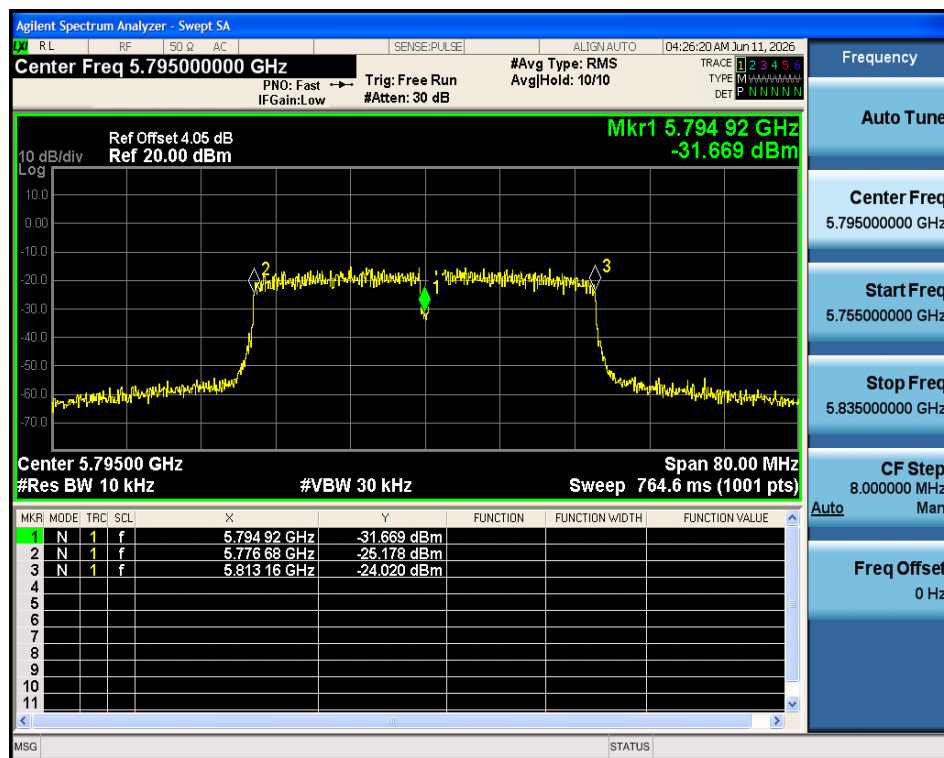
Freq. Stability 30C 5V n40 5795MHz Ant1
