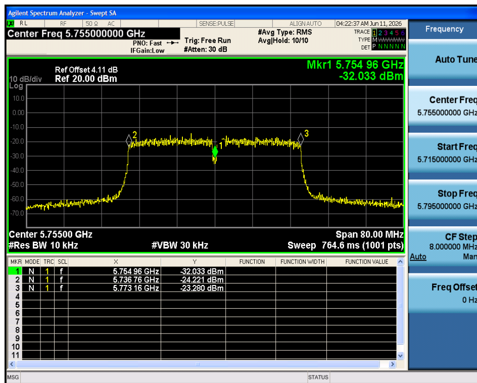
Freq. Stability 0C 5V n40 5755MHz Ant1
