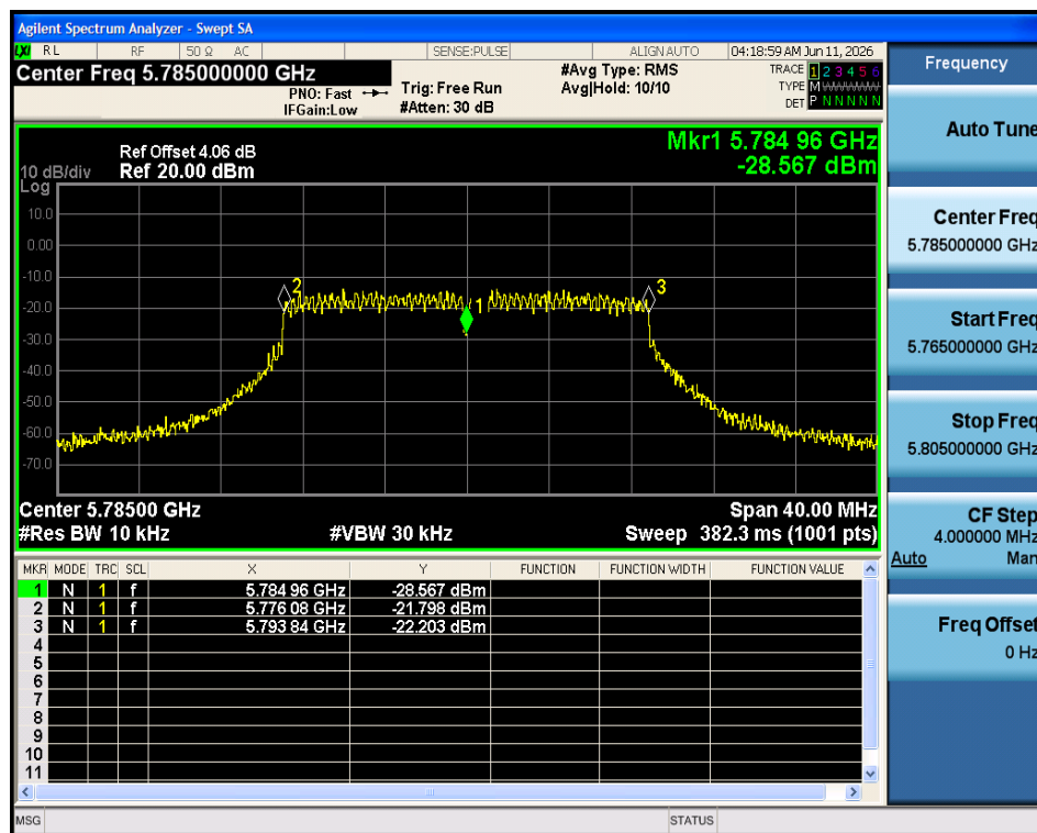
Freq. Stability 50C 5V n20 5785MHz Ant1
