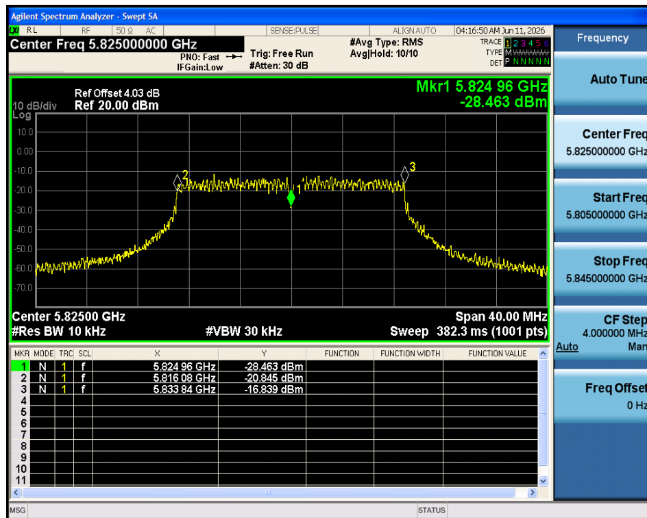
Freq. Stability 30C 5V n20 5825MHz Ant1
