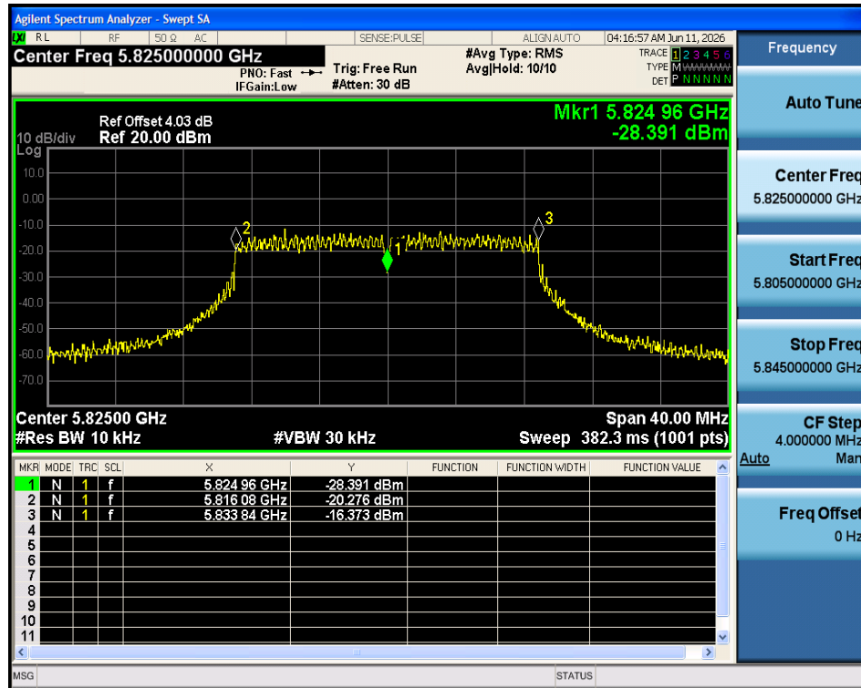
Freq. Stability 40C 5V n20 5825MHz Ant1
