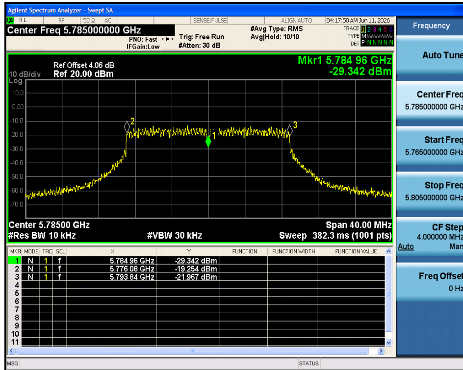
Freq. Stability 20C 4.25V n20 5785MHz Ant1
