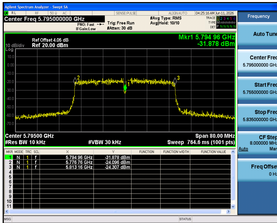
Freq. Stability 20C 5.75V n40 5795MHz Ant1
