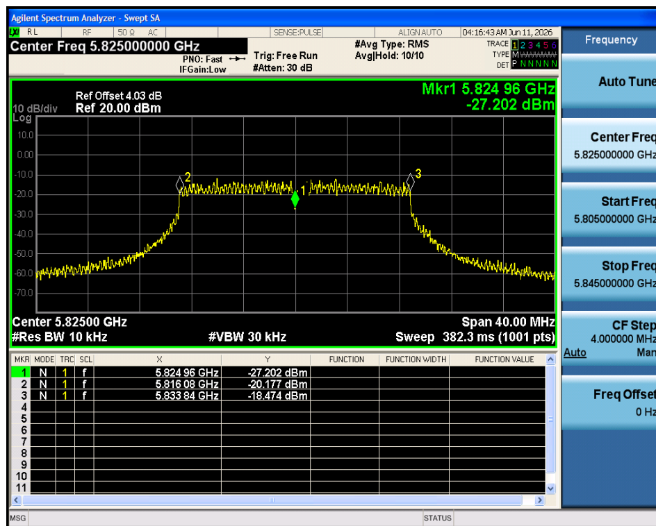
Freq. Stability 20C 5V n20 5825MHz Ant1
