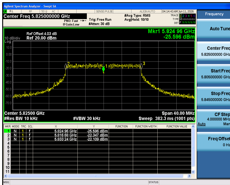
Freq. Stability 30C 5V a 5825MHz Ant1
