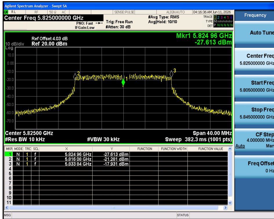
Freq. Stability 10C 5V n20 5825MHz Ant1
