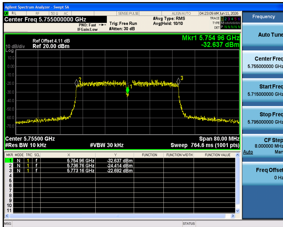
Freq. Stability 30C 5V n40 5755MHz Ant1
