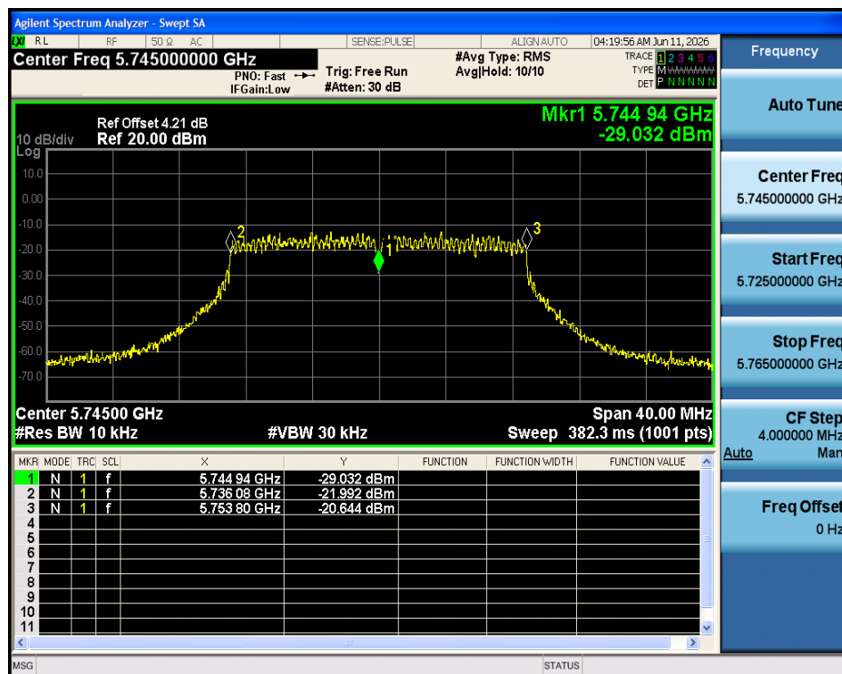
Freq. Stability -20C 5V n20 5745MHz Ant1
