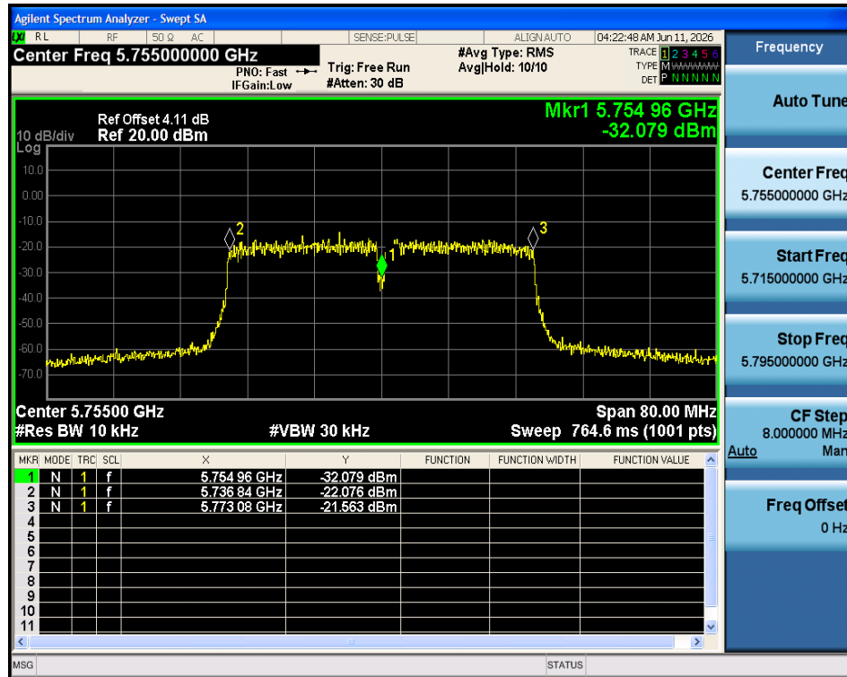
Freq. Stability 10C 5V n40 5755MHz Ant1
