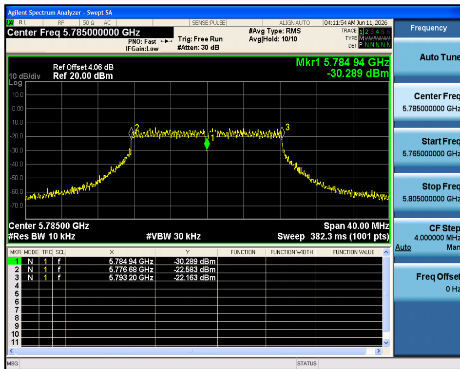
Freq. Stability 30C 5V a 5785MHz Ant1
