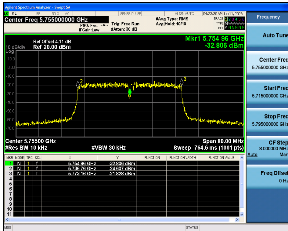
Freq. Stability 50C 5V n40 5755MHz Ant1
