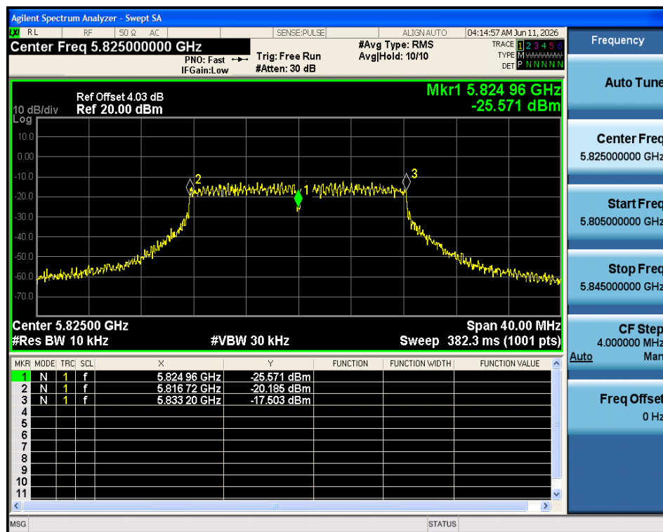
Freq. Stability 50C 5V a 5825MHz Ant1
