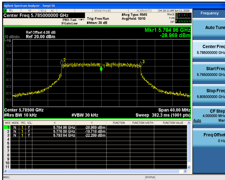
Freq. Stability -20C 5V n20 5785MHz Ant1
