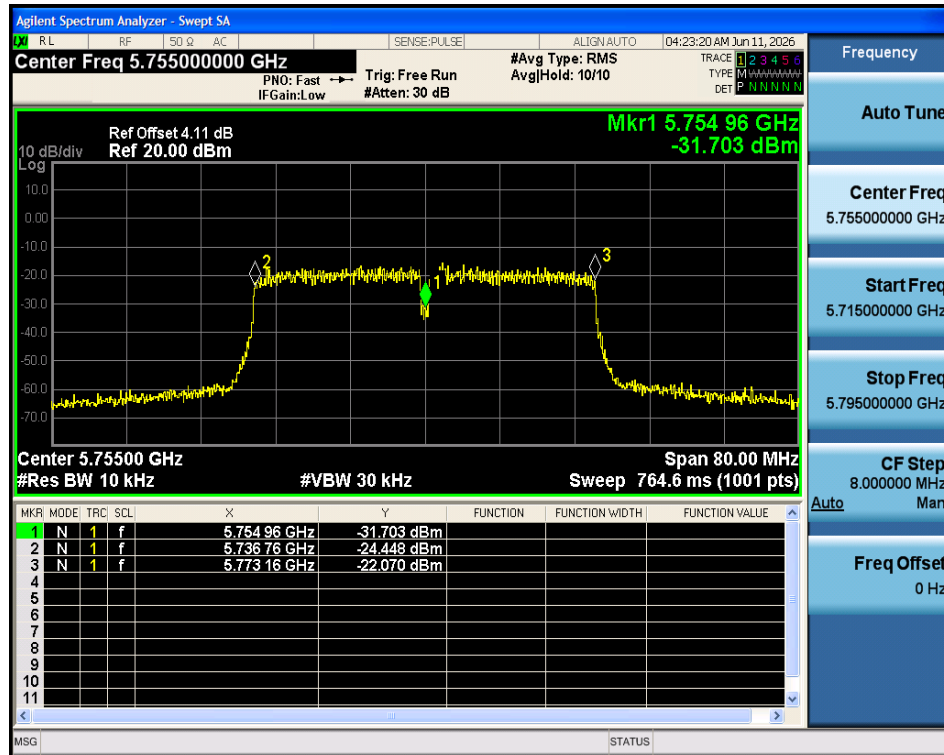
Freq. Stability 40C 5V n40 5755MHz Ant1
