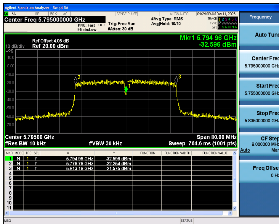
Freq. Stability 20C 5V n40 5795MHz Ant1
