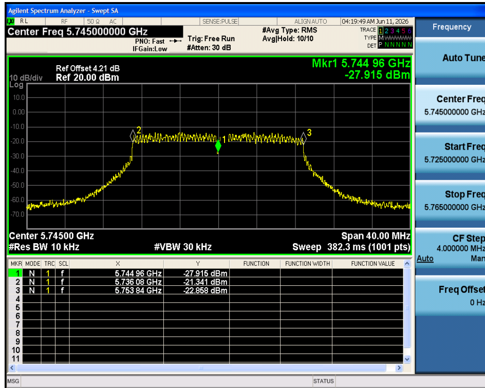
Freq. Stability 20C 5.75V n20 5745MHz Ant1
