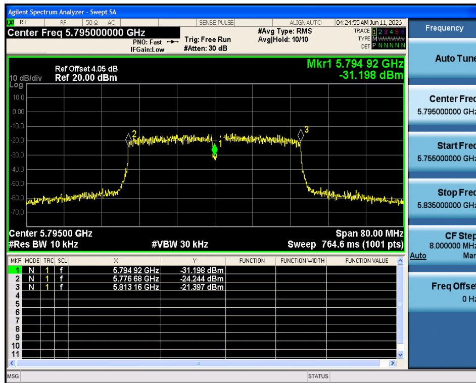
Freq. Stability 20C 4.25V n40 5795MHz Ant1
