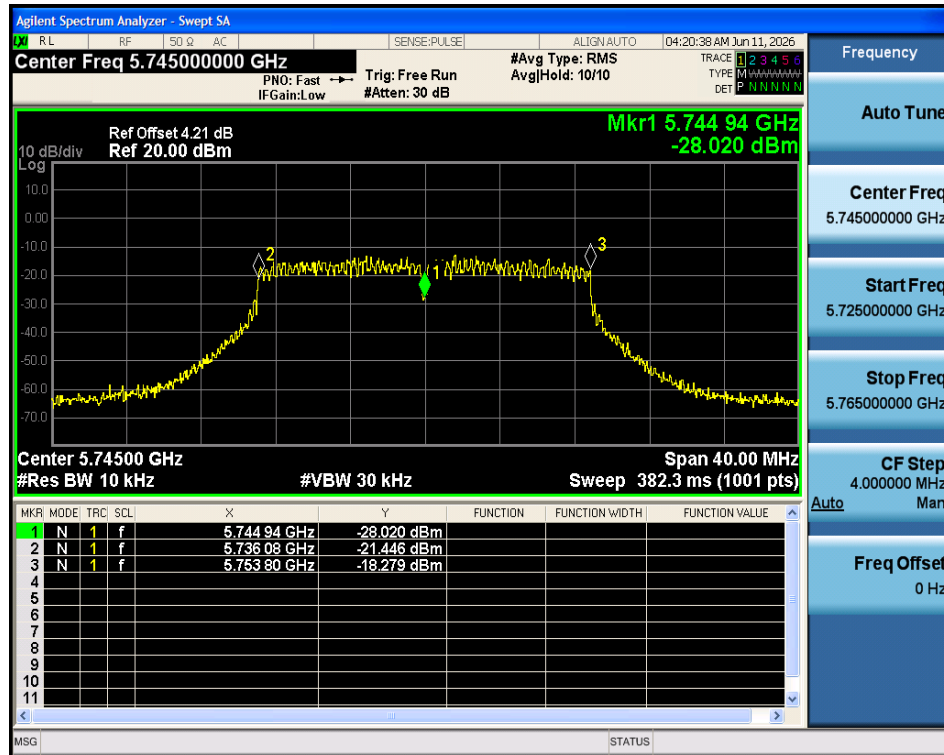
Freq. Stability 40C 5V n20 5745MHz Ant1
