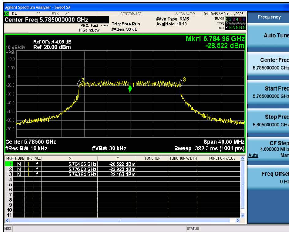
Freq. Stability 30C 5V n20 5785MHz Ant1
