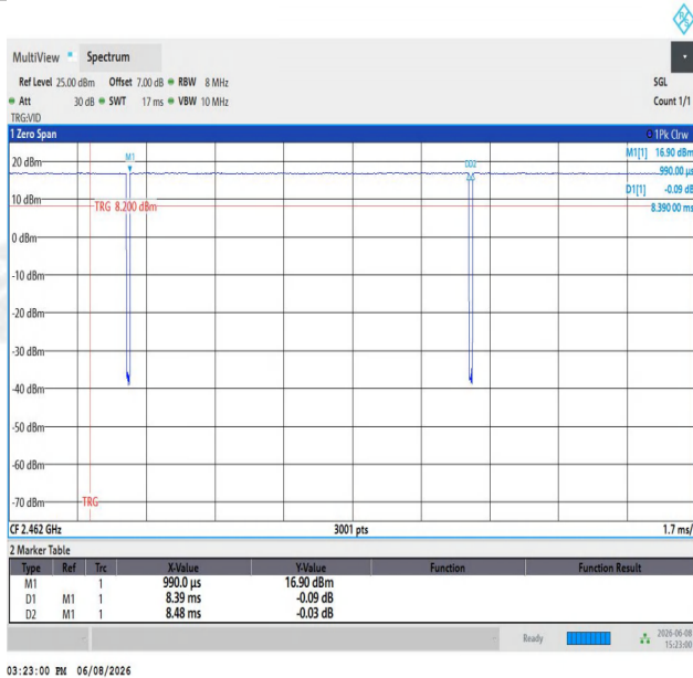
NTNV-11B-Ant1-2462
