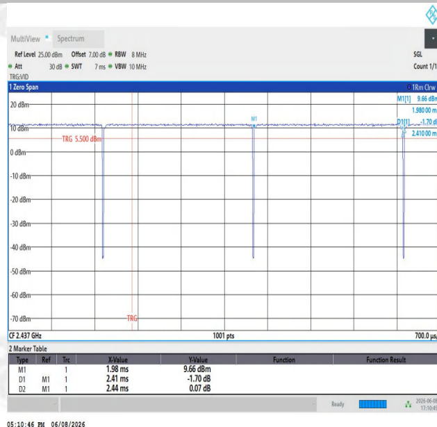
NTNV-11N20SISO-Ant1-2437
