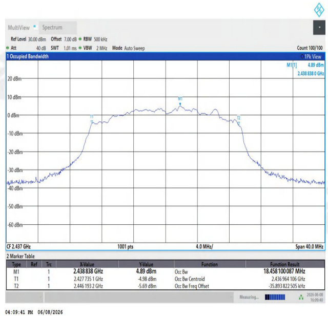
11AX20SISO-Ant1-2437
