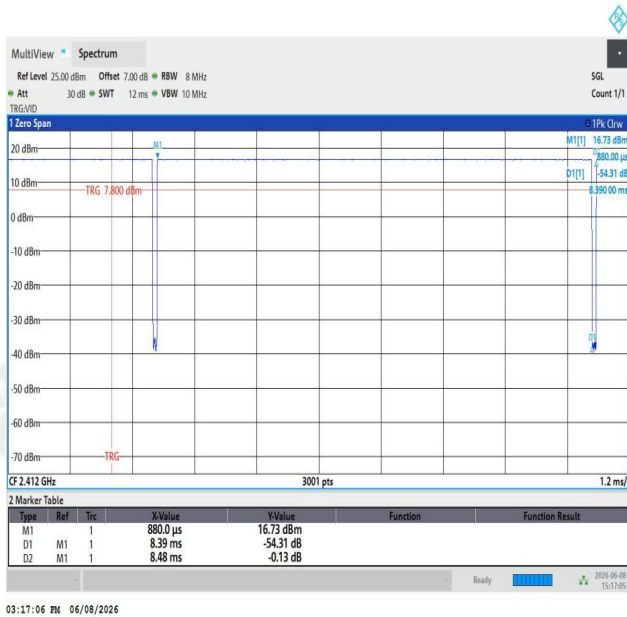
NTNV-11B-Ant1-2412
