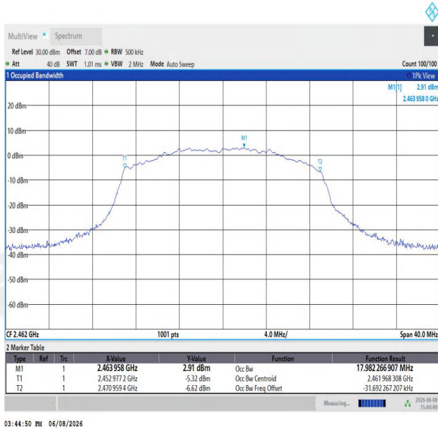
11N20SISO-Ant1-2462
