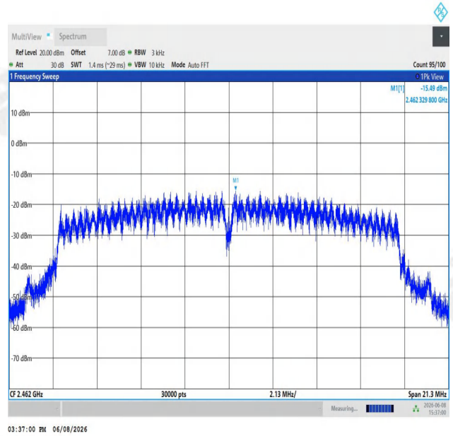
11G-Ant1-2462-PASS
