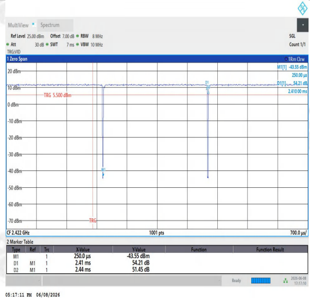
NTNV-11AX40SISO-Ant1-2422
