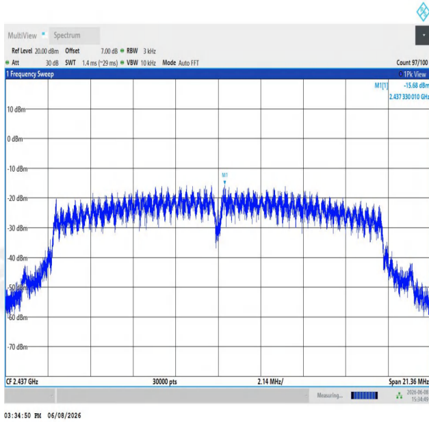
11G-Ant1-2437-PASS
