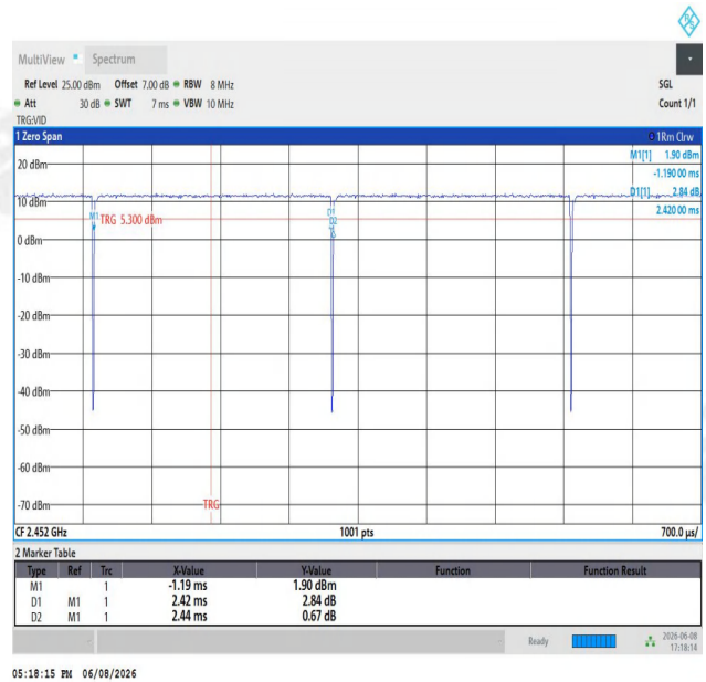
NTNV-11AX40SISO-Ant1-2452
