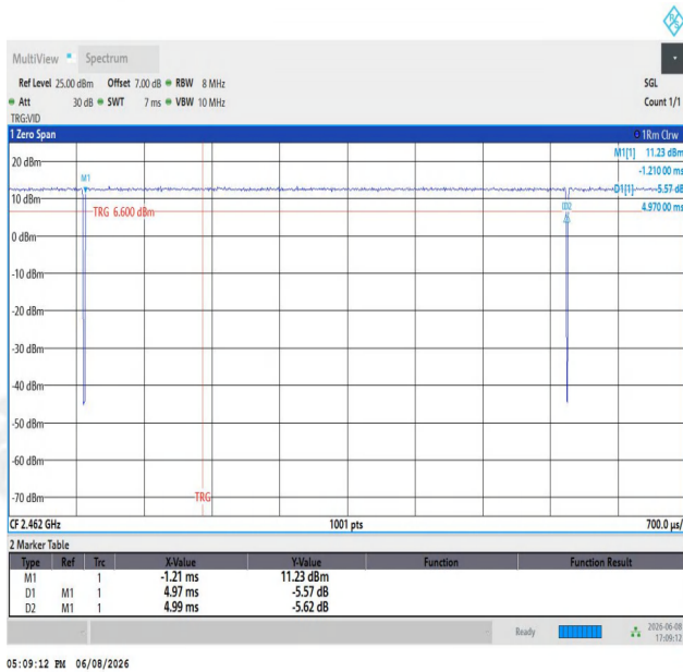
NTNV-11N20SISO-Ant1-2462
