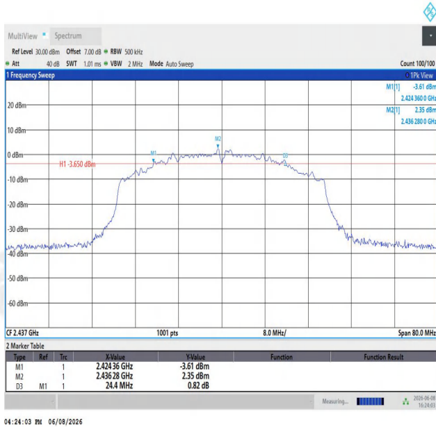
11AX40SISO-Ant1-2437-PASS
