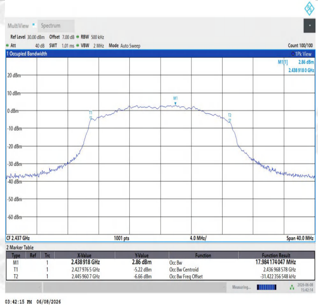
11N20SISO-Ant1-2437
