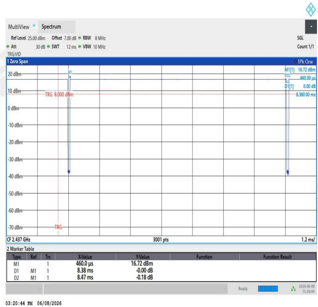
NTNV-11B-Ant1-2437
