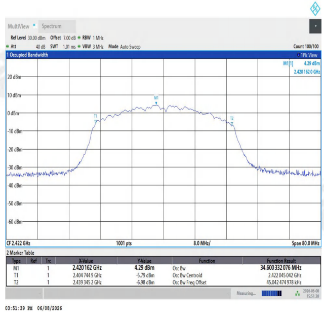
11N40SISO-Ant1-2422
