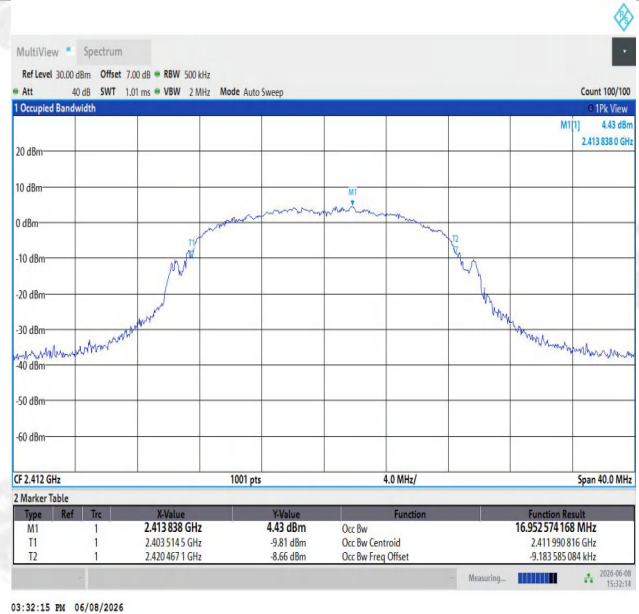
11G-Ant1-2412
