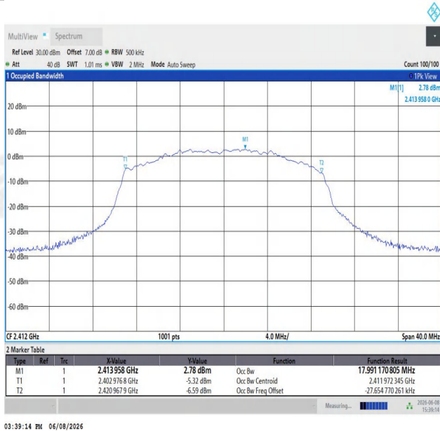
11N20SISO-Ant1-2412
