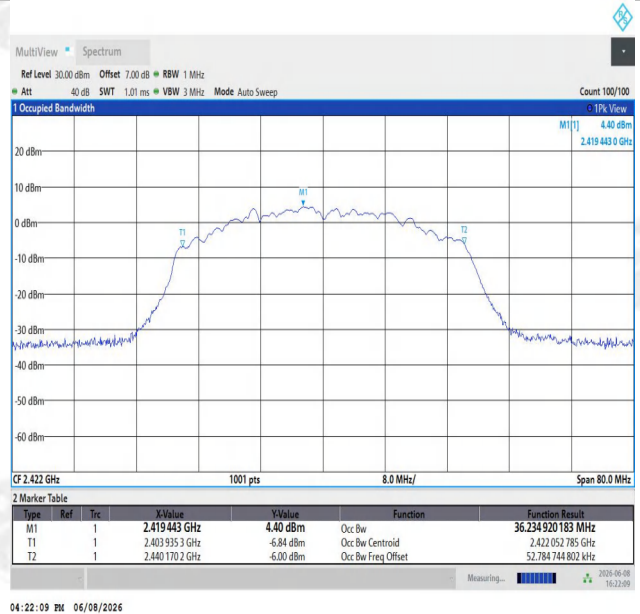
11AX40SISO-Ant1-2422
