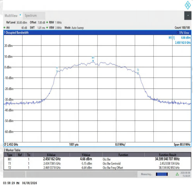
11N40SISO-Ant1-2452
