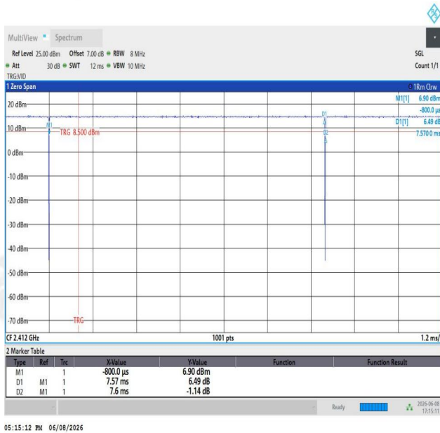
NTNV-11AX20SISO-Ant1-2412
