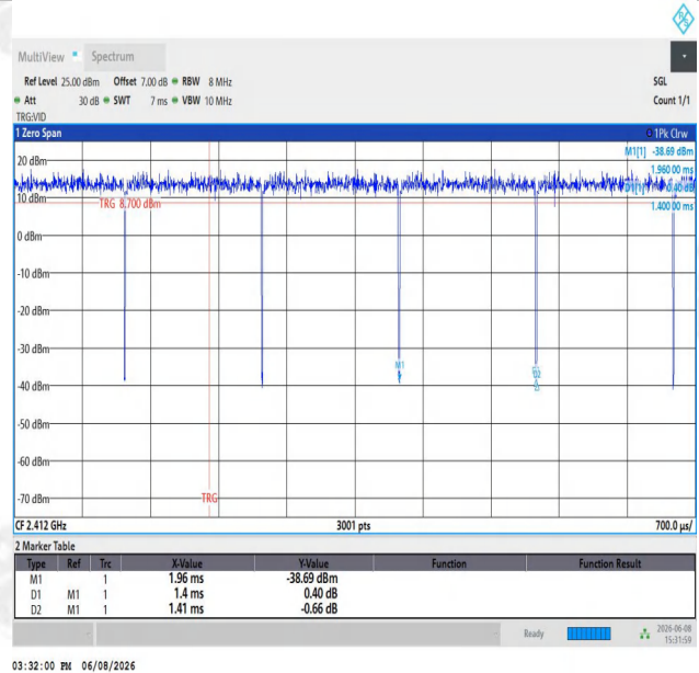
NTNV-11G-Ant1-2412
