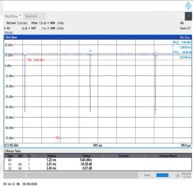
NTNV-11N40SISO-Ant1-2452
