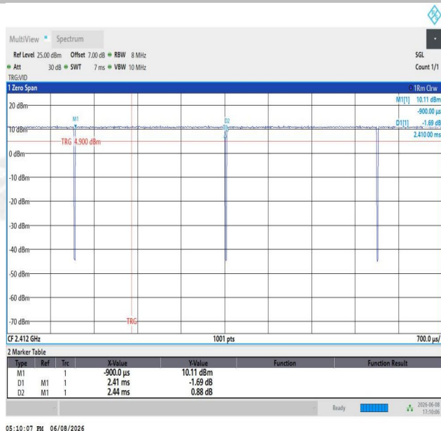
NTNV-11N20SISO-Ant1-2412
