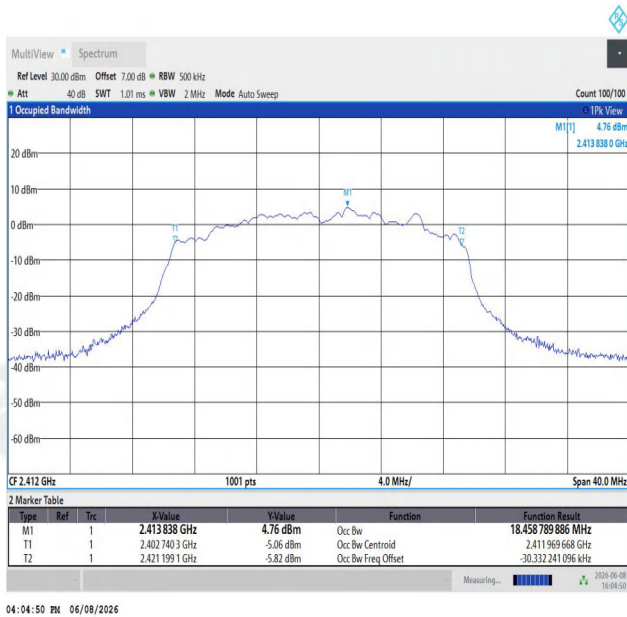
11AX20SISO-Ant1-2412
