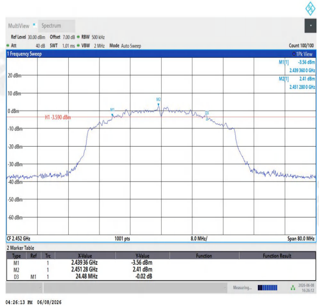
11AX40SISO-Ant1-2452-PASS
