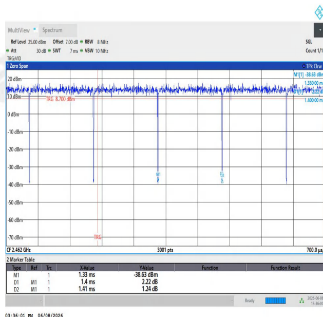
NTNV-11G-Ant1-2462
