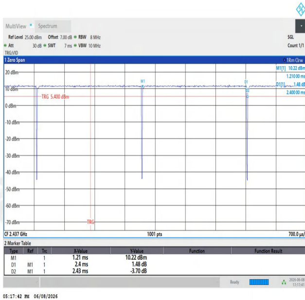
NTNV-11AX40SISO-Ant1-2437
