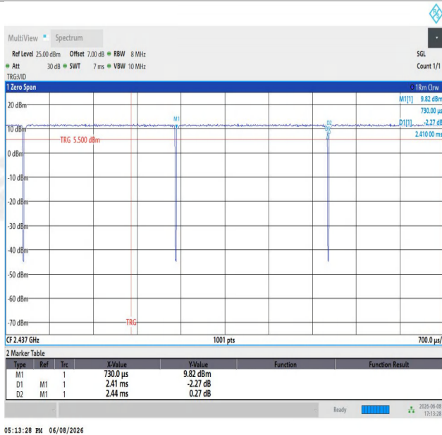
NTNV-11N40SISO-Ant1-2437
