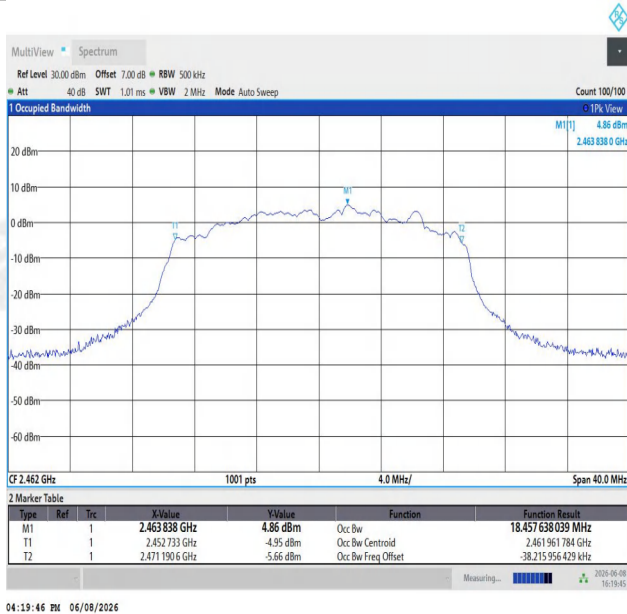
11AX20SISO-Ant1-2462
