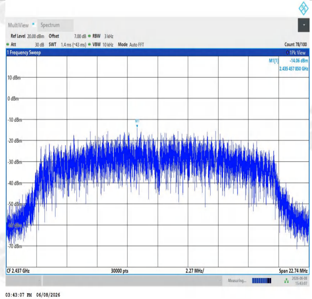
11N20SISO-Ant1-2437-PASS
