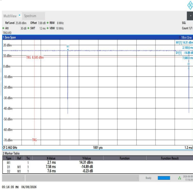
NTNV-11AX20SISO-Ant1-2462
