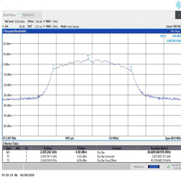
11N40SISO-Ant1-2437
