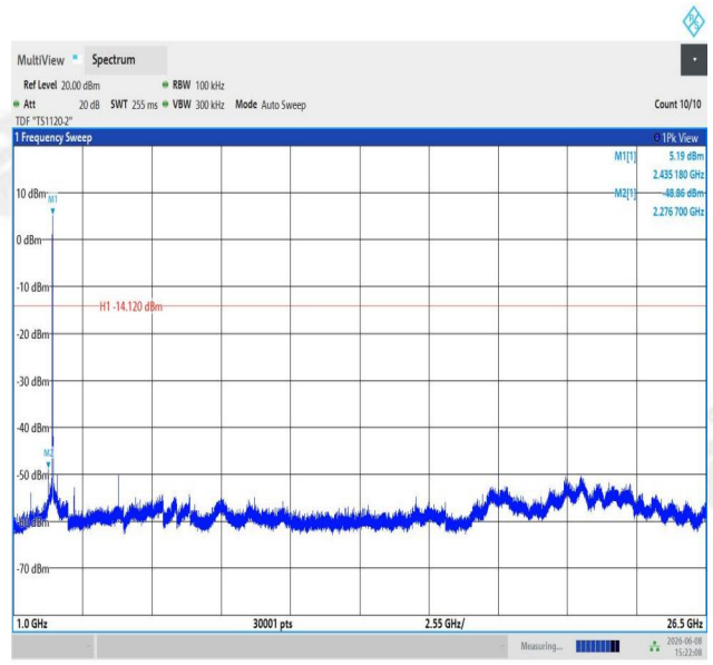
11B-Ant1-2437-1000~26500-PASS
