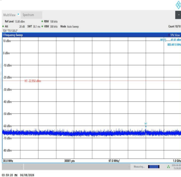
11N40SISO-Ant1-2452-30~1000-PASS
