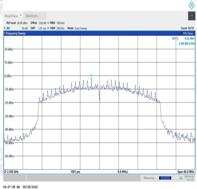
11AX40ISO-Ant1-2452-0~Reference-PASS
