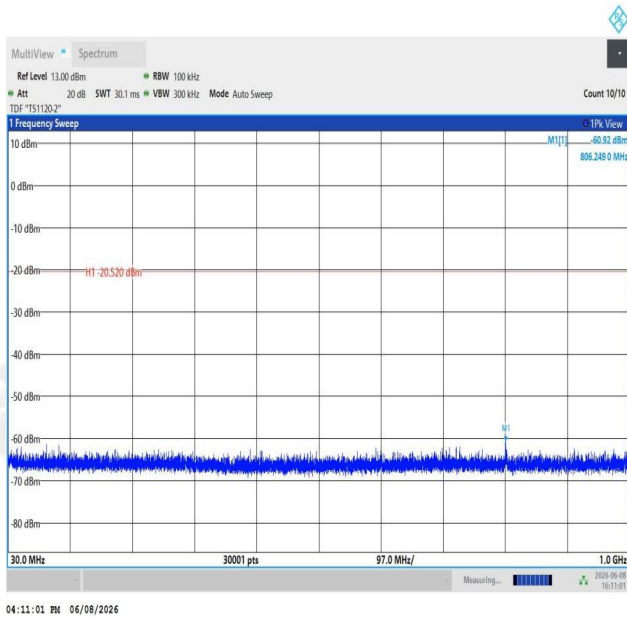
11AX20SISO-Ant1-2437-30~1000-PASS
