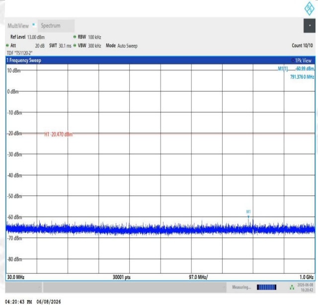
11AX20SISO-Ant1-2462-30~1000-PASS
