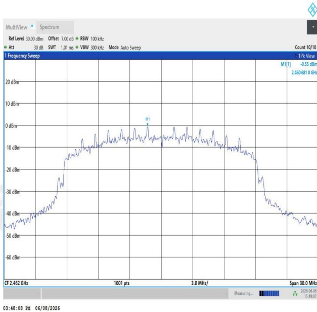
11N20SISO-Ant1-2462-0~Reference-PASS
