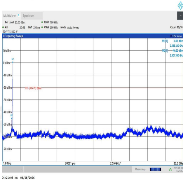
11AX20SISO-Ant1-2462-1000~26500-PASS
