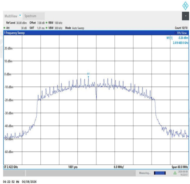
11AX40SISO-Ant1-2422-0~Reference-PASS
