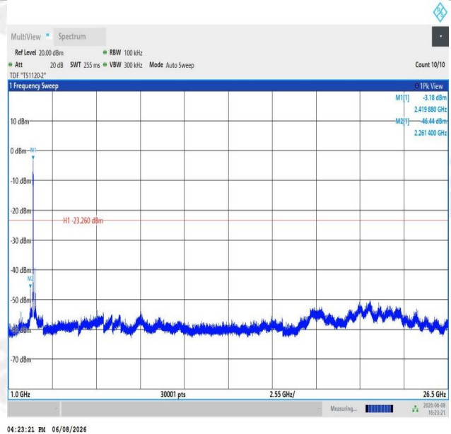
11AX40SISO-Ant1-2422-1000~26500-PASS
