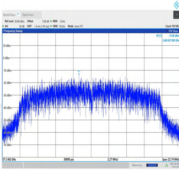
11N20SISO-Ant1-2462-PASS
