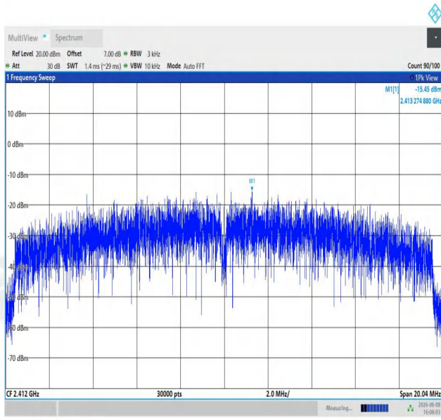
11AX20SISO-Ant1-2412-PASS
