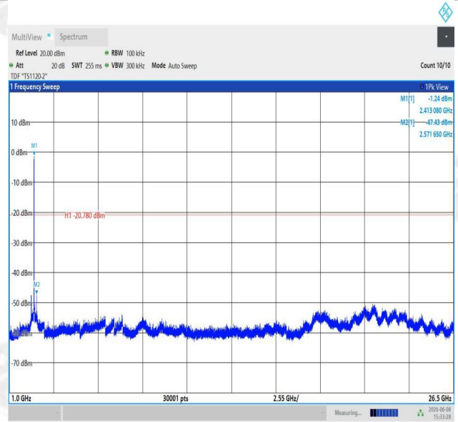
11G-Ant1-2412-0~Reference-PASS
