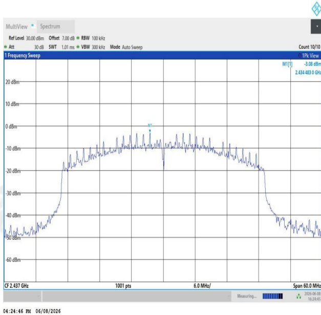
11AX40ISO-Ant1-2437-0~Reference-PASS
