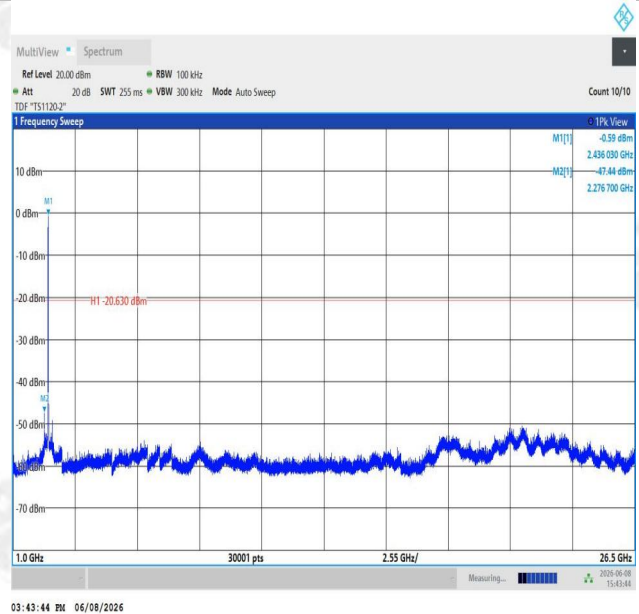
11N20SISO-Ant1-2437-1000~26500-PASS
