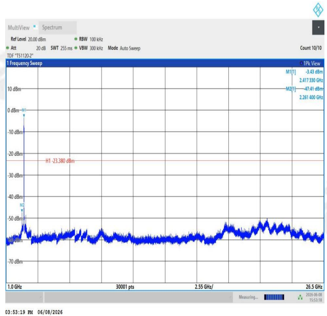
11N40SISO-Ant1-2422-1000~26500-PASS
