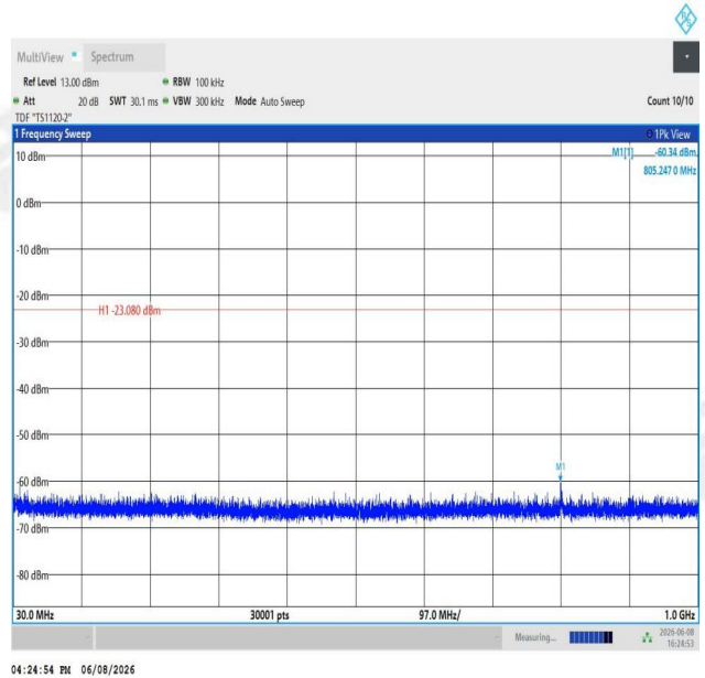
11AX40ISO-Ant1-2437-30~1000-PASS
