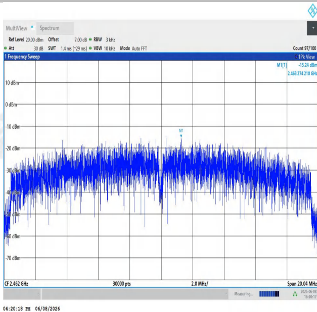
11AX20SISO-Ant1-2462-PASS
