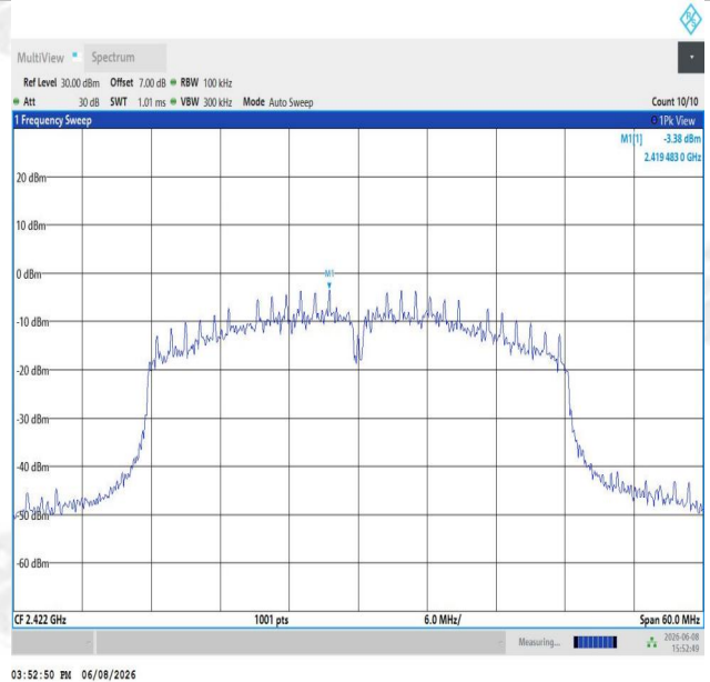
11N40SISO-Ant1-2422-0~Reference-PASS
