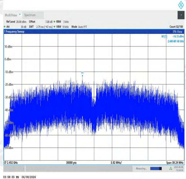
11N40SISO-Ant1-2452-PASS
