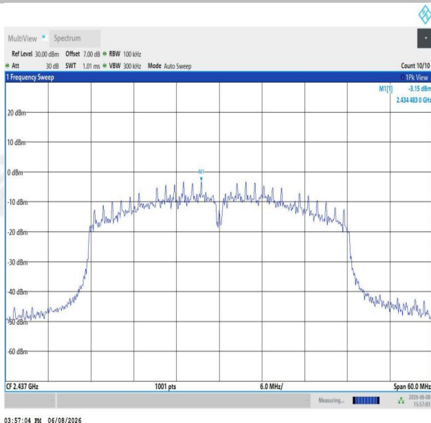
11N40SISO-Ant1-2437-0~Reference-PASS
