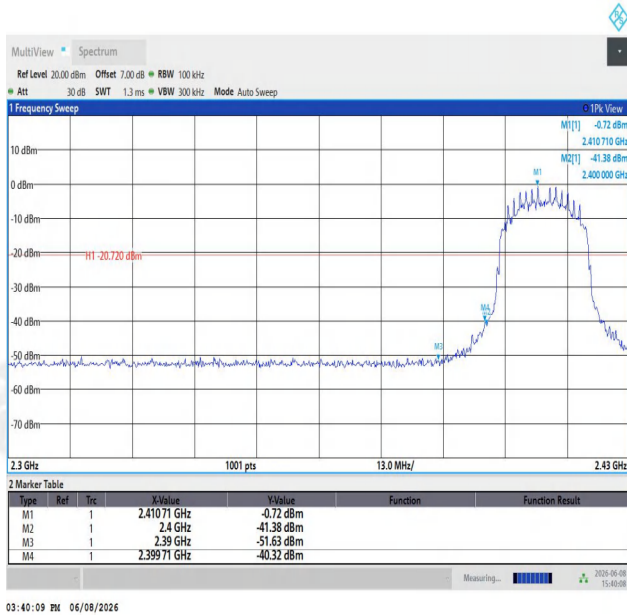
11N20SISO-Ant1-2412-PASS
