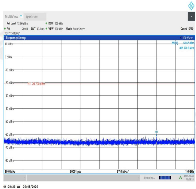
11AX20SISO-Ant1-2412-30~1000-PASS
