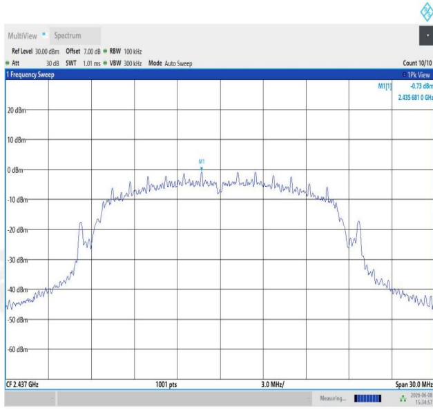
11G-Ant1-2437-0~Reference-PASS
