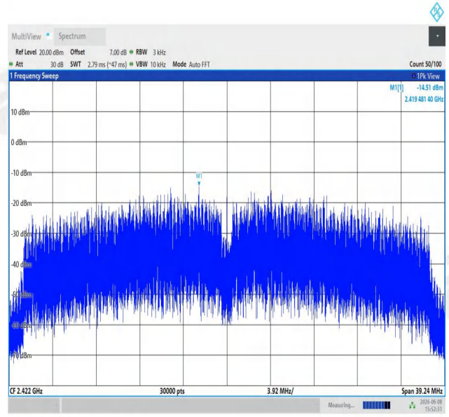
11N40SISO-Ant1-2422-PASS
