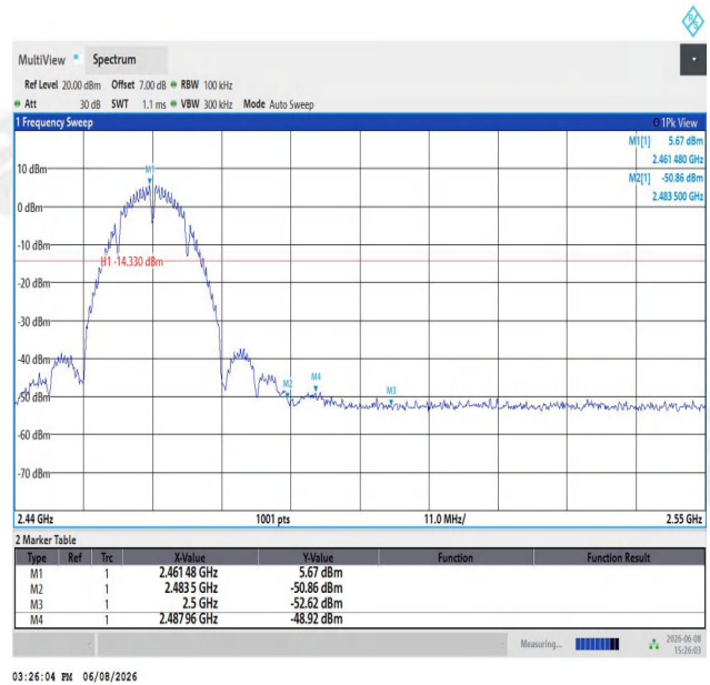
11B-Ant1-2462-PASS
