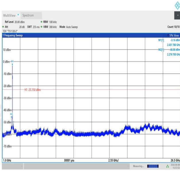
11N40SISO-Ant1-2437-1000~26500-PASS
