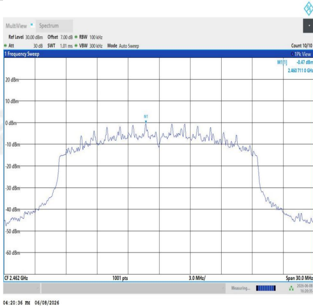
11AX20SISO-Ant1-2462-0~Reference-PASS
