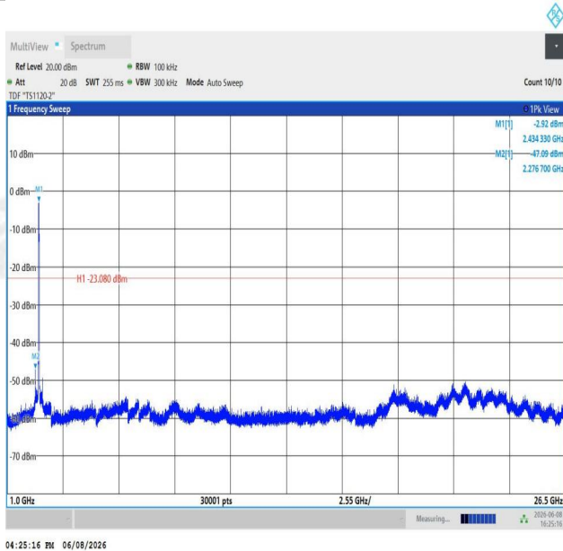
11AX40ISO-Ant1-2437-1000~26500-PASS
