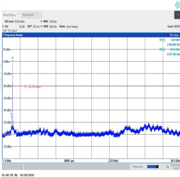
11N20SISO-Ant1-2462-1000~26500-PASS
