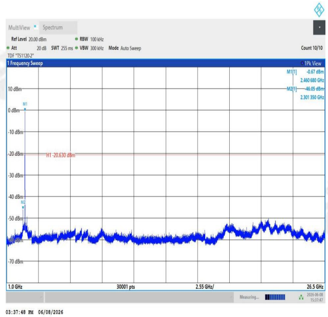
11G-Ant1-2462-1000~26500-PASS
