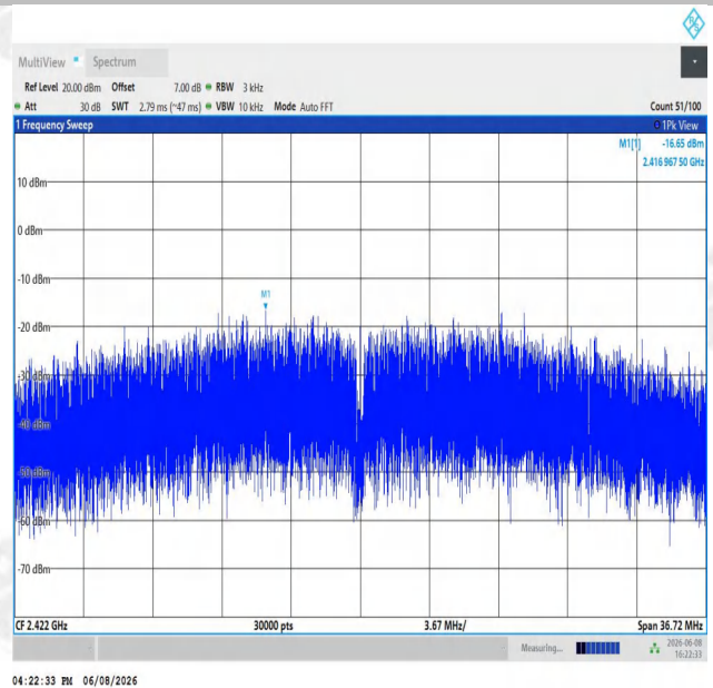
11AX40SISO-Ant1-2422-PASS
