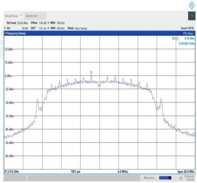
11G-Ant1-2412-0~Reference-PASS
