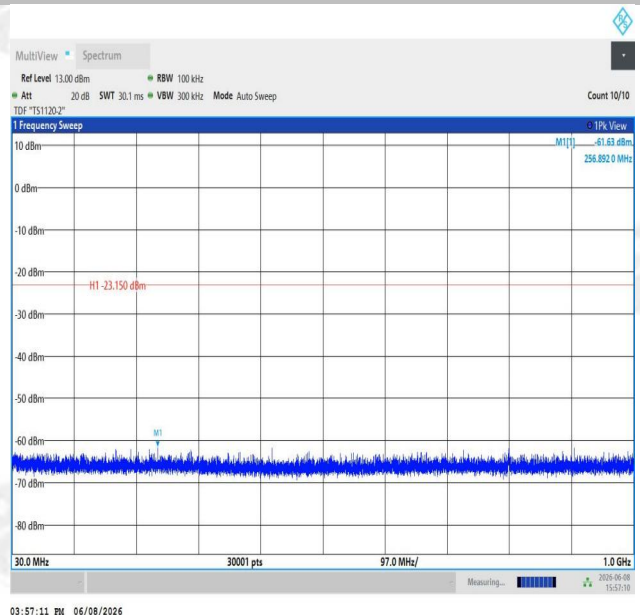
11N40SISO-Ant1-2437-30~1000-PASS
