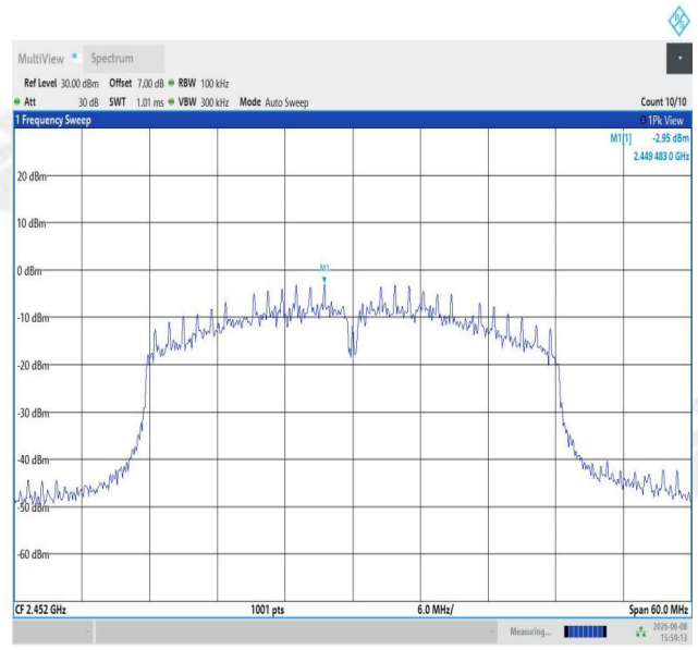
11N40SISO-Ant1-2452-0~Reference-PASS
