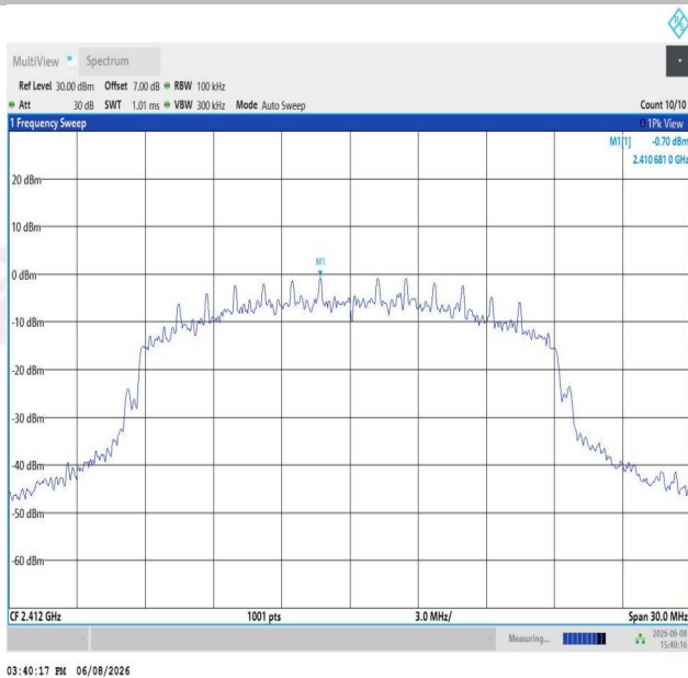
11N20SISO-Ant1-2412-0~Reference-PASS
