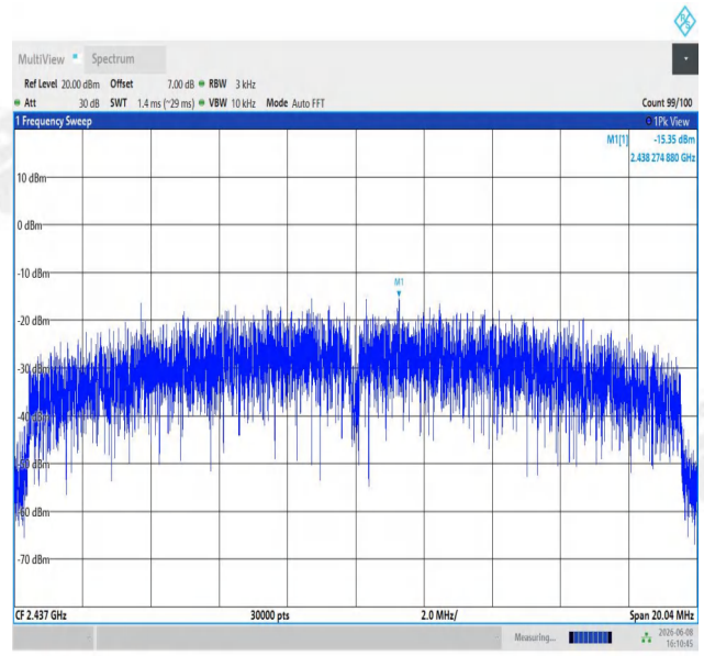
11AX20SISO-Ant1-2437-PASS
