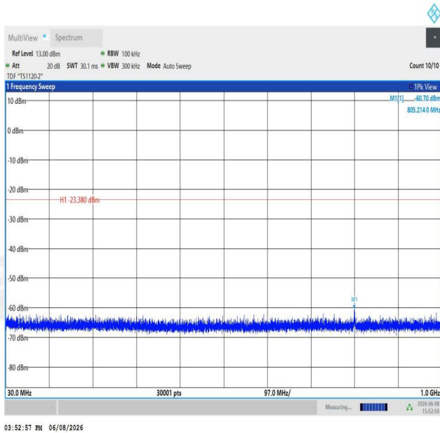
11N40SISO-Ant1-2422-30~1000-PASS
