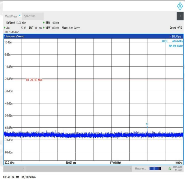
11N20SISO-Ant1-2412-30~1000-PASS
