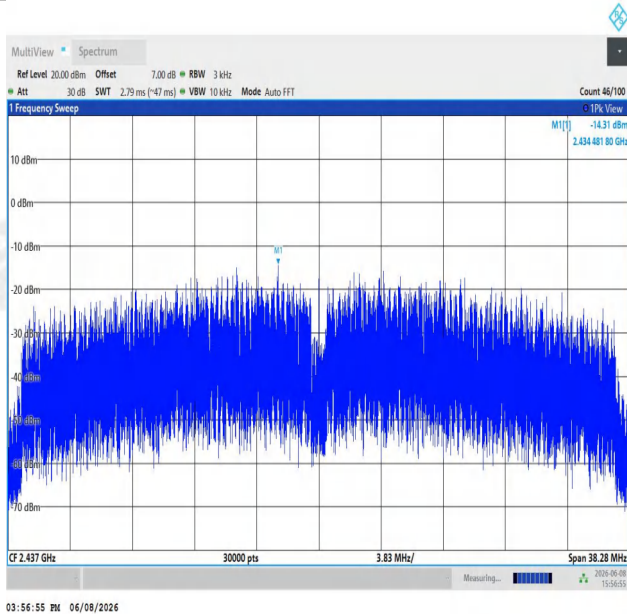
11N40SISO-Ant1-2437-PASS
