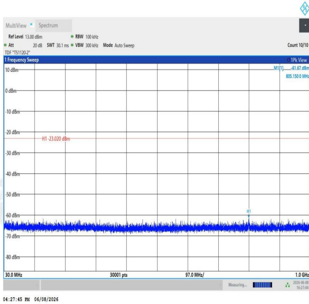
11AX40SISO-Ant1-2452-30~1000-PASS
