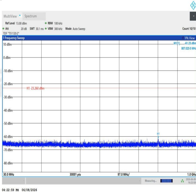
11AX40SISO-Ant1-2422-30~1000-PASS
