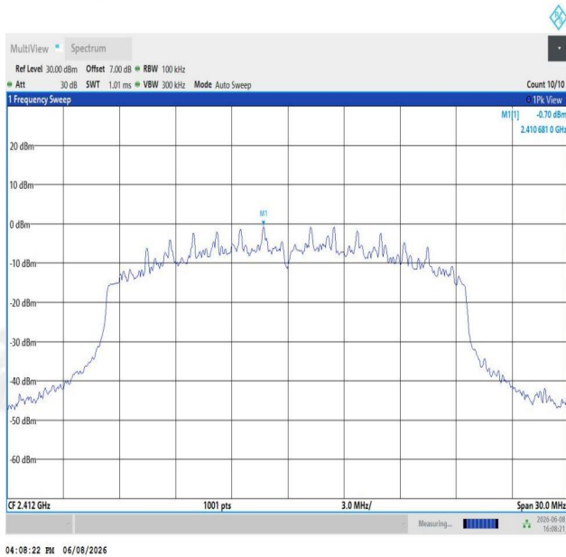
11AX20SISO-Ant1-2412-0~Reference-PASS
