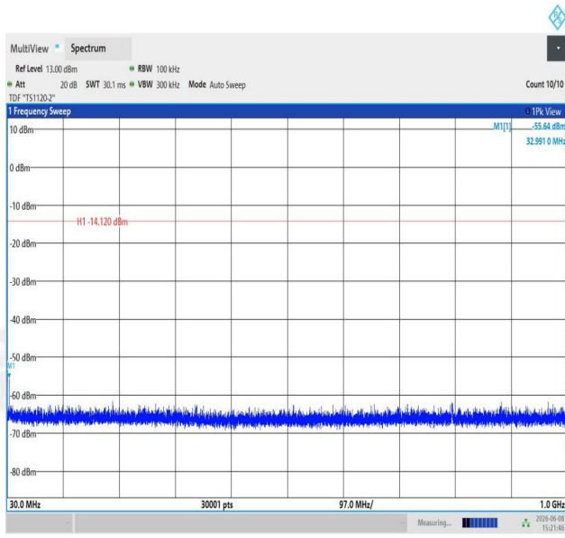
11B-Ant1-2437-30~1000-PASS
