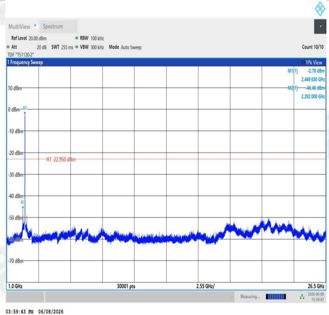
11N40SISO-Ant1-2452-1000~26500-PASS
