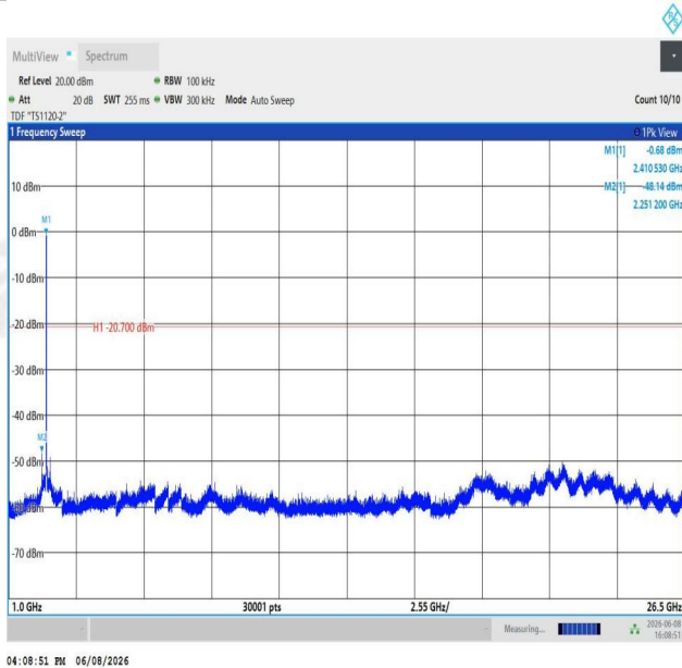
11AX20SISO-Ant1-2412-1000~26500-PASS
