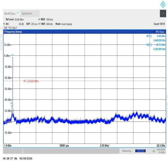
11AX40SISO-Ant1-2452-1000~26500-PASS
