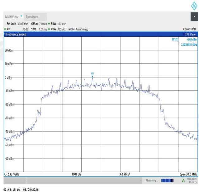
11N20SISO-Ant1-2437-0~Reference-PASS
