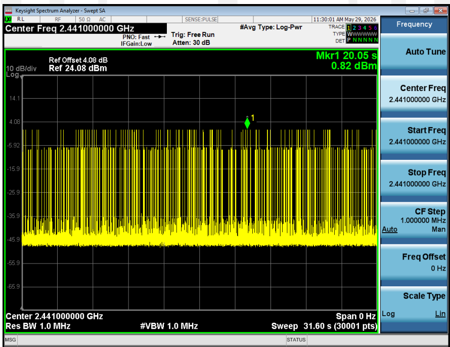
Dwell_Time_(Hopping)_NVNT_ANT1_1-DH5_2441_00_Accumulated
