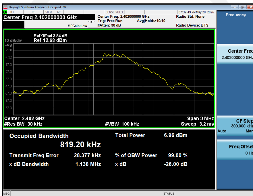
99%_Occupied_Bandwidth_NVNT_ANT1_1-DH1_2402_00
