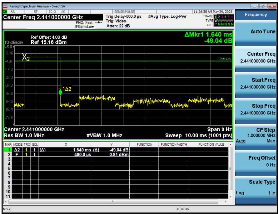
Dwell_Time_(Hopping)_NVNT_ANT1_1-DH3_2441_00_Accumulated
