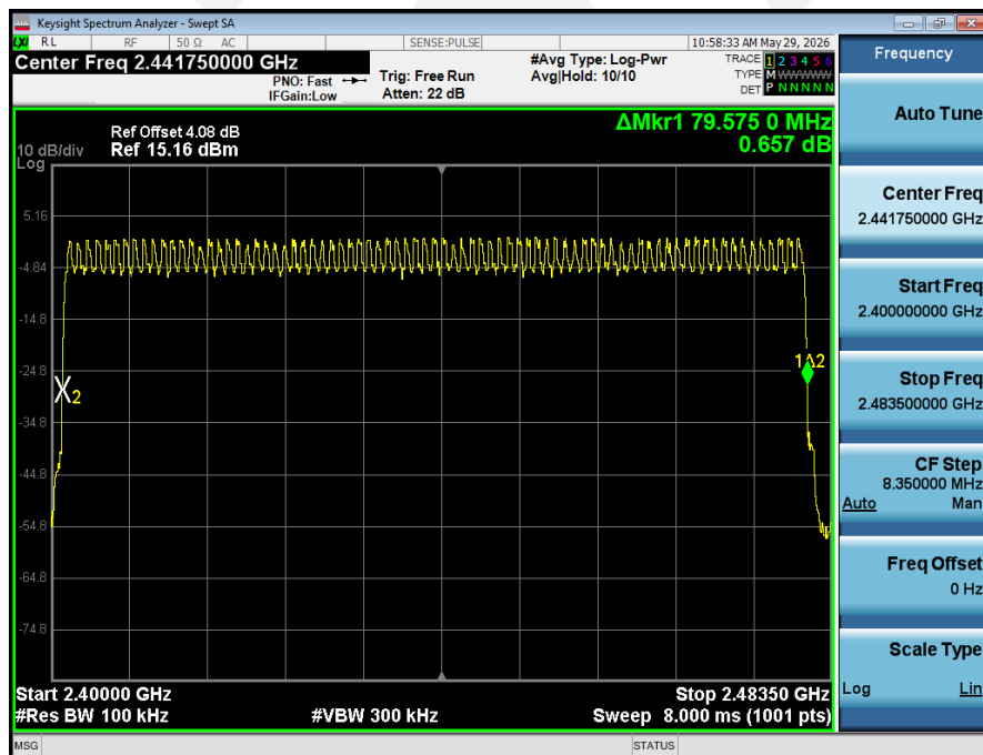
Number_of_Hopping_Channel_(Hopping)_NVNT_ANT1_2-DH1_Hopping
