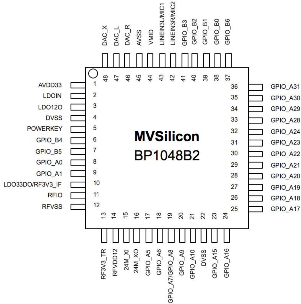
Figure 2. Pin Definition
