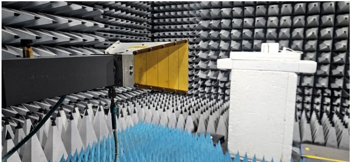
Radiated emissions 1GHz -10GHz
