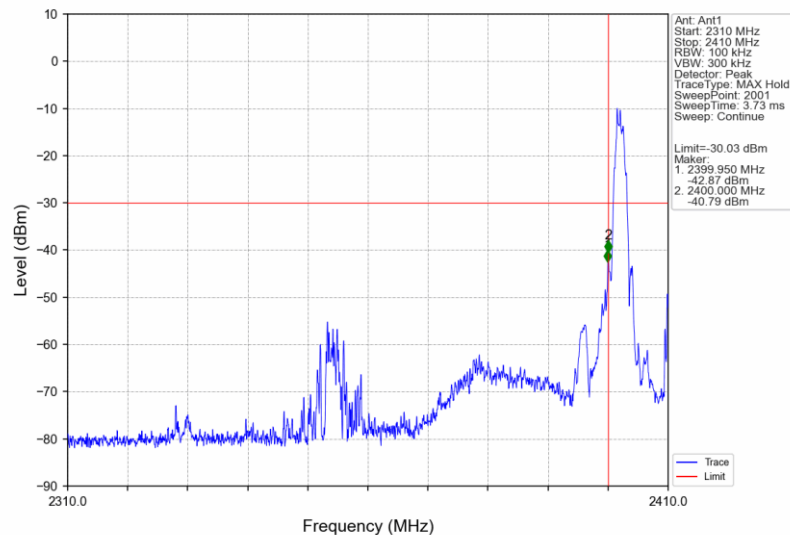
2M_LCH_2402MHz_Ant1_NTNV
