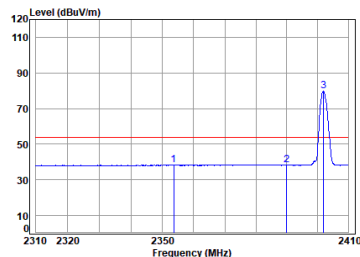
BLE_1M_TX_CH_00_Vertical-AVG
