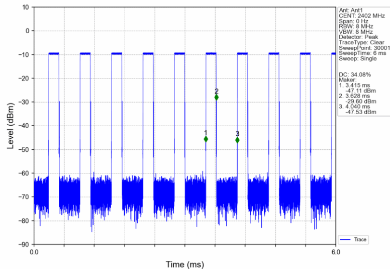
2M_LCH_2402MHz_Ant1_NTNV
