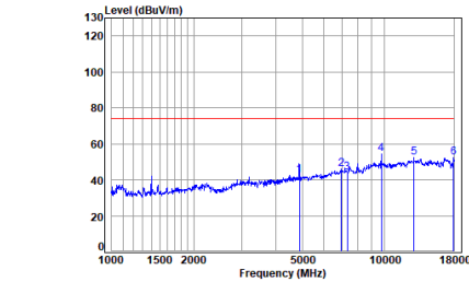
BLE_1M_TX_CH_19_Vertical-Peak
