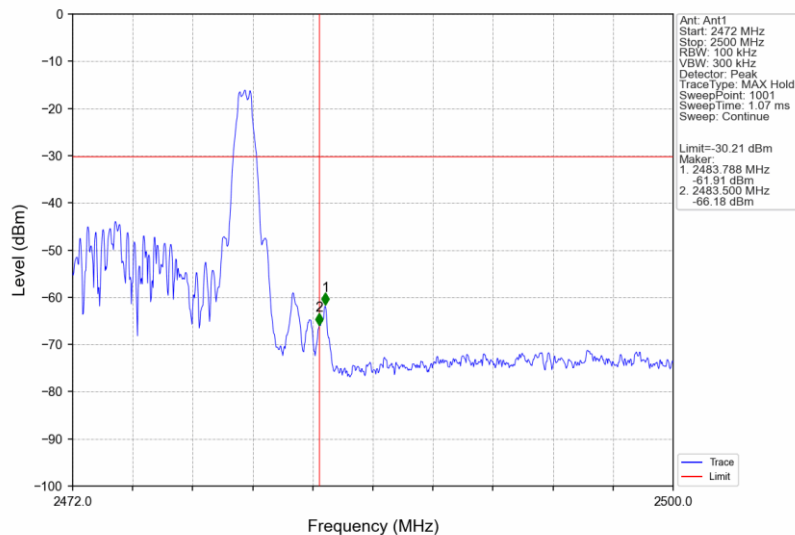
1M_HCH_2480MHz_Ant1_NTNV
