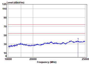
BLE_1M_TX_CH_39_Horizontal-Peak
