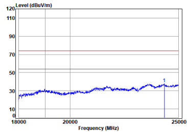
BLE_1M_TX_CH_39_Vertical-Peak
