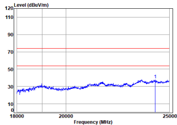
BLE_1M_TX_CH_39_Horizontal-Peak
