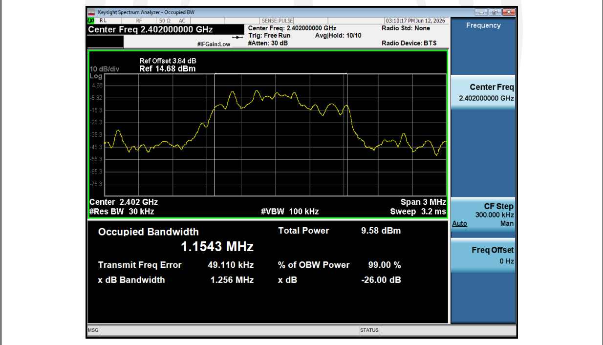
99%_Occupied_Bandwidth_NVNT_ANT1_2-DH1_2402_00
