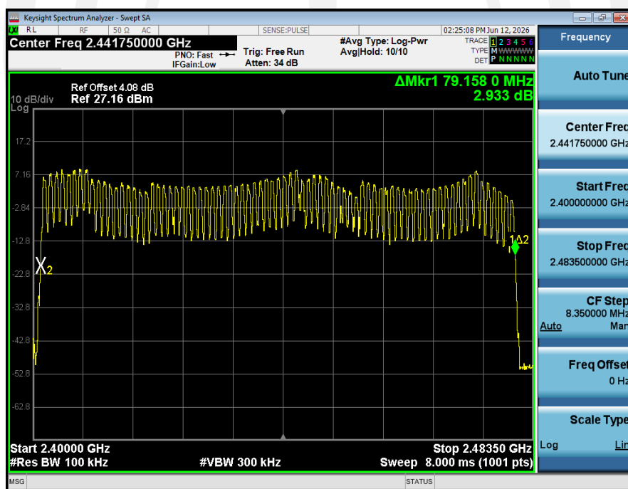
Number_of_Hopping_Channel_(Hopping)_NVNT_ANT1_1-DH1_Hopping
