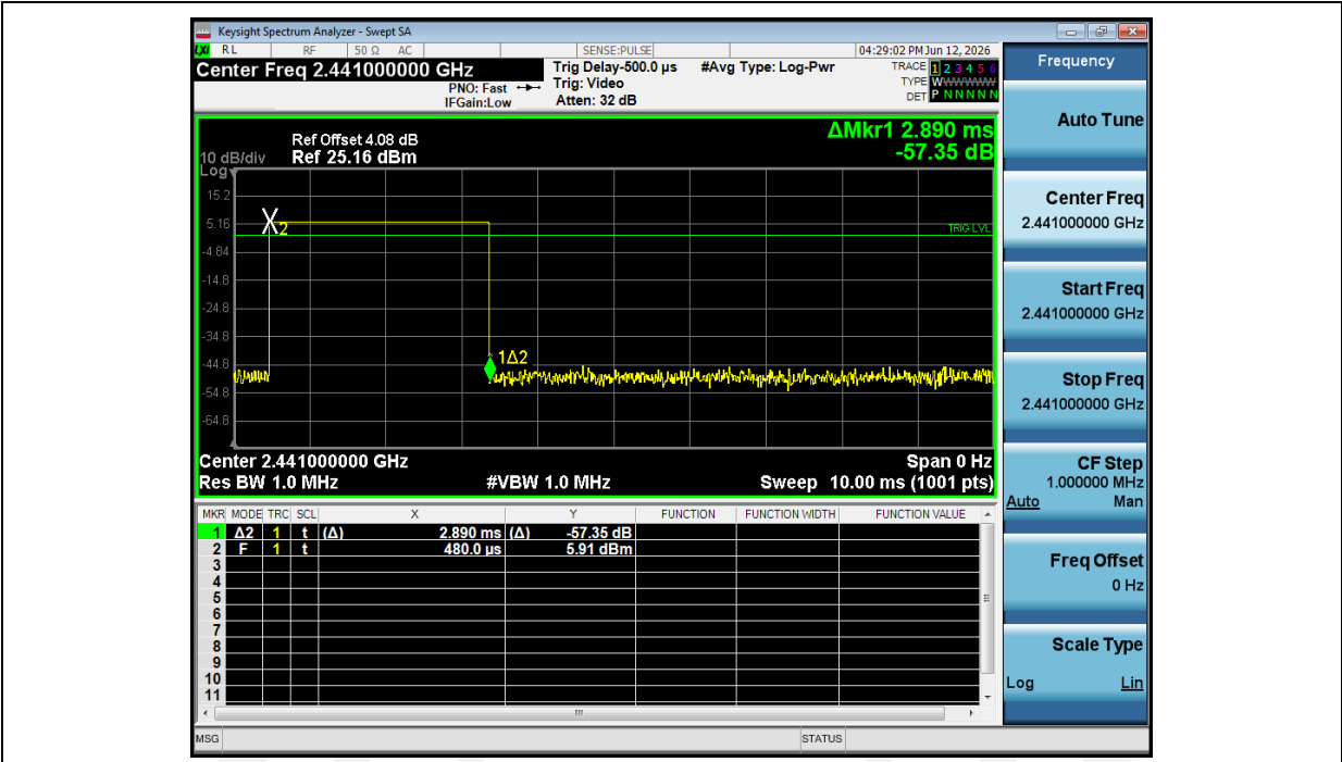
Dwell_Time_(Hopping)_NVNT_ANT1_2-DH5_2441_00_Accumulated
