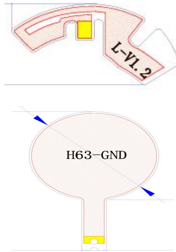
FPC Antenna picture & assembly picture
