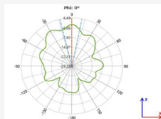
BT Passive Efficiency Field Pattern
