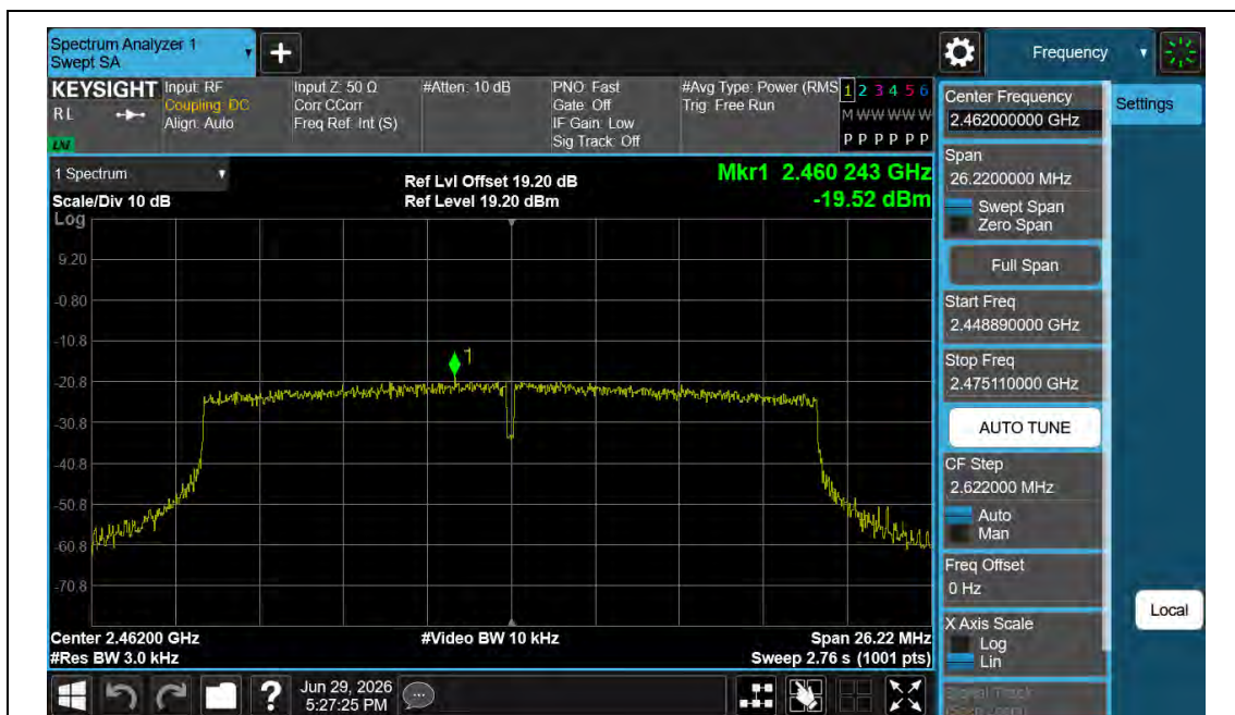
11AX20MIMO-Ant1-2462-PASS
