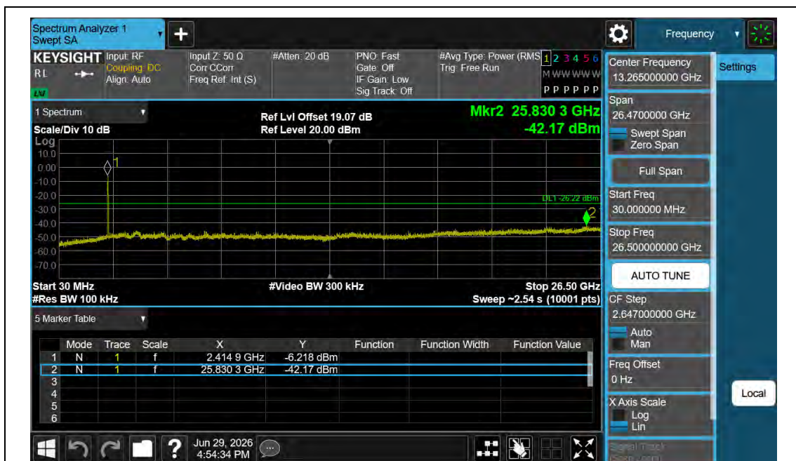
11N40MIMO-Ant1-2422-30~26500-PASS
