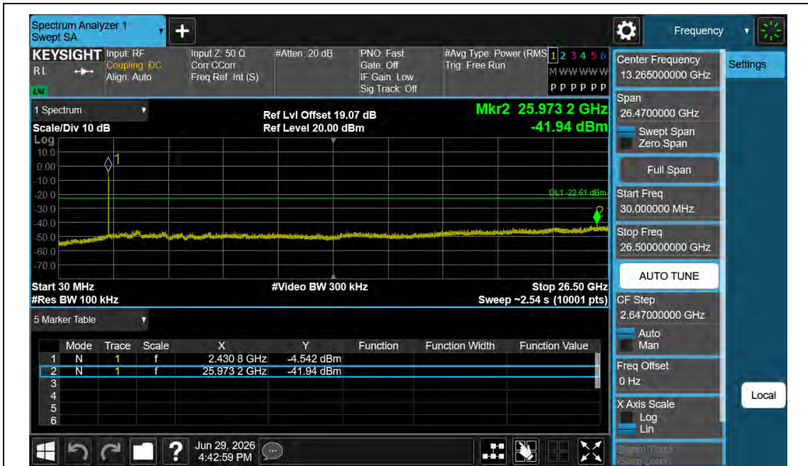
11N20MIMO-Ant1-2437-30~26500-PASS
