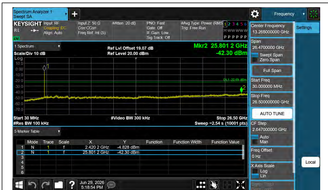
11AX20MIMO-Ant1-2412-30~26500-PASS
