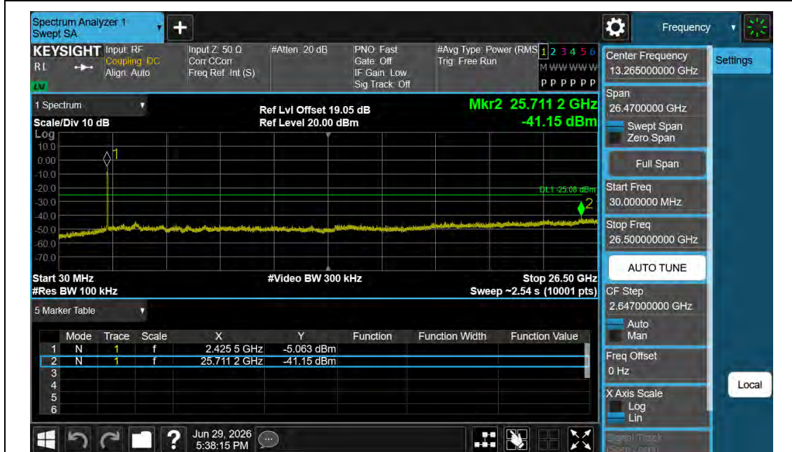
11AX40MIMO-Ant0-2437-30~26500-PASS
