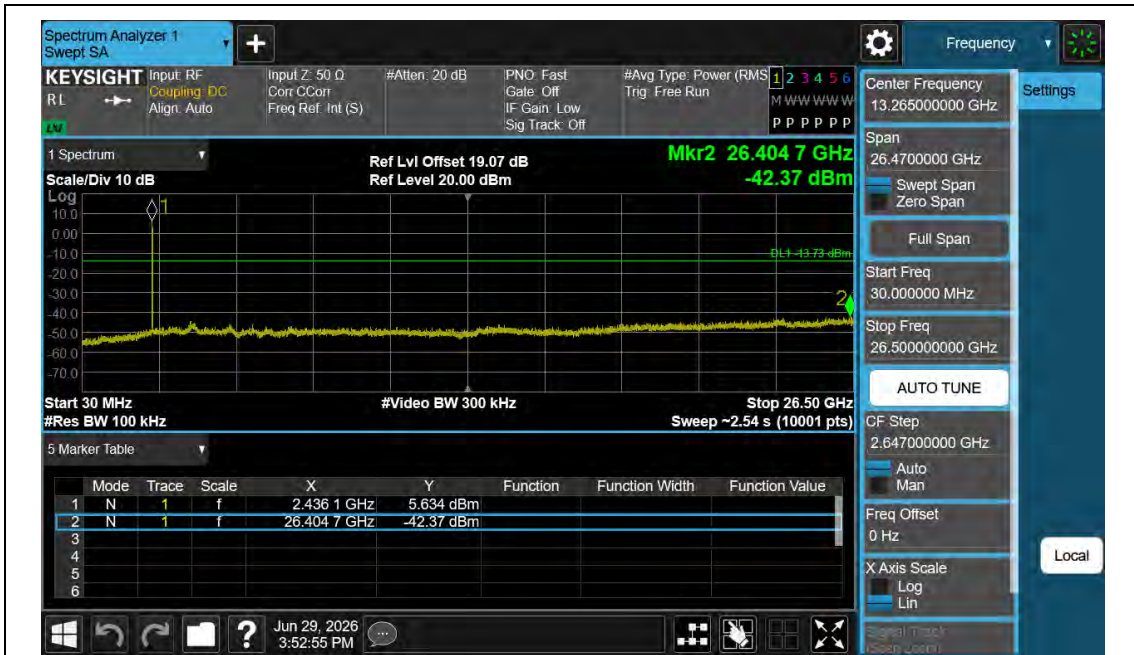
11B-Ant1-2437-30~26500-PASS
