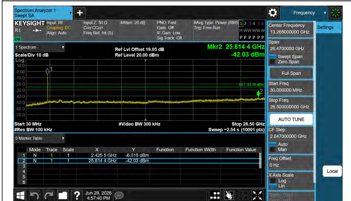
11N40MIMO-Ant0-2437-30~26500-PASS
