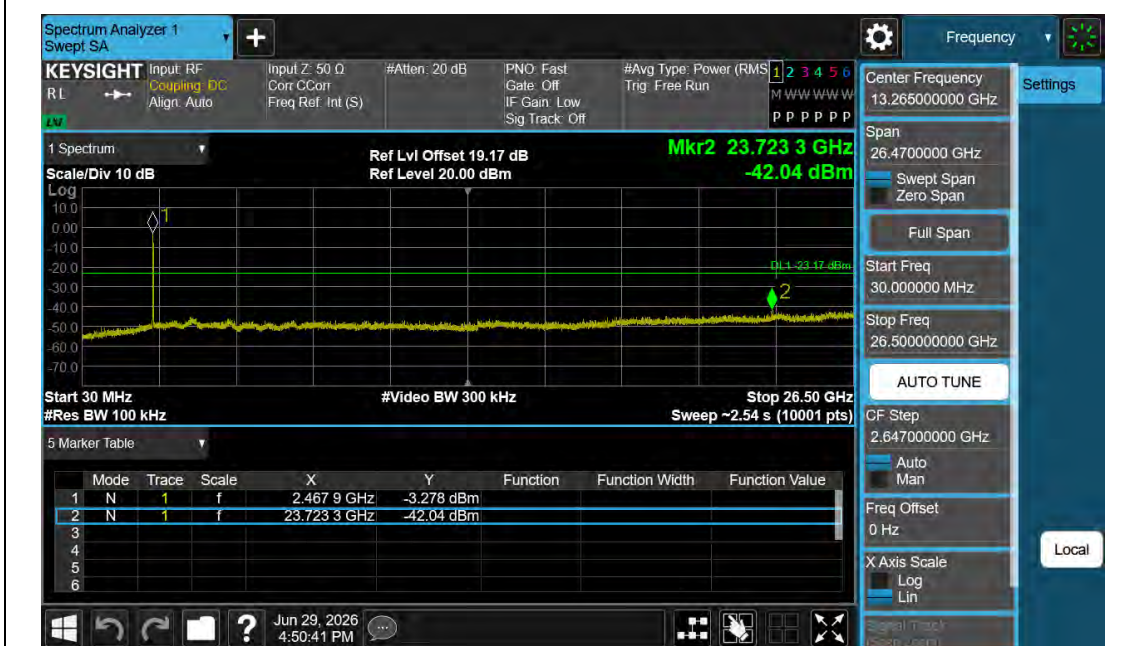
11N40MIMO-Ant0-2422-30~26500-PASS
