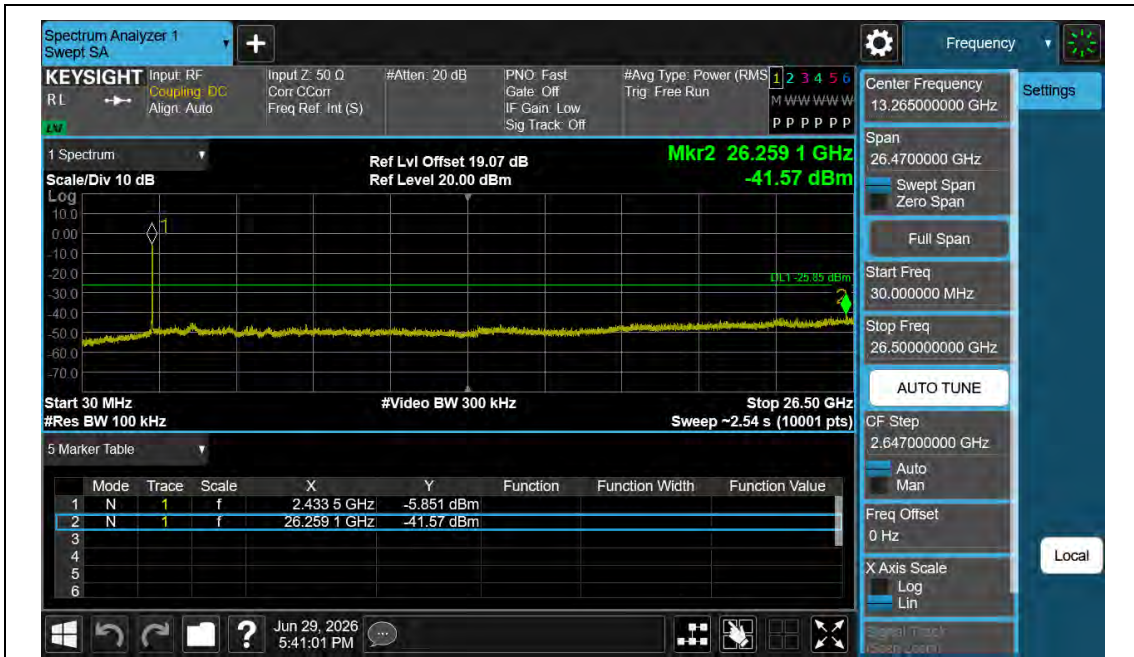
11AX40MIMO-Ant1-2437-30~26500-PASS
