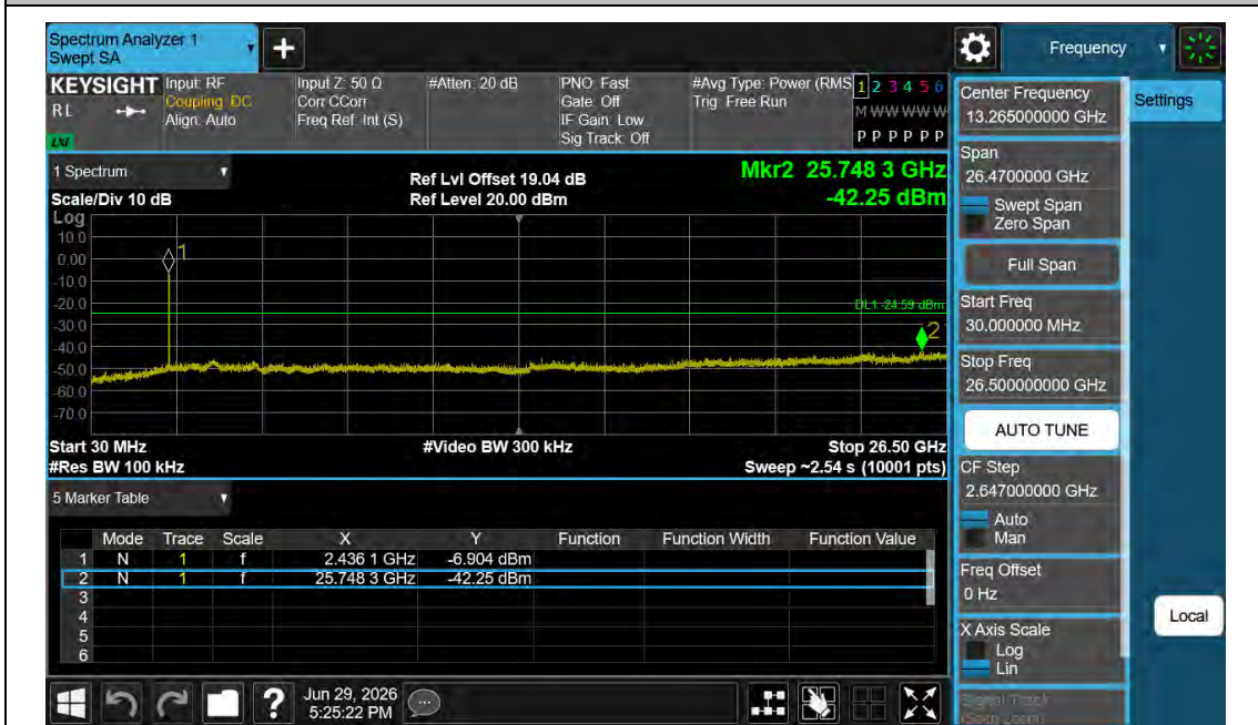
11AX20MIMO-Ant0-2462-30~26500-PASS
