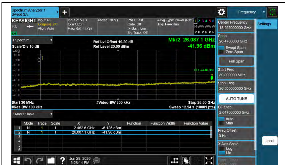
11AX20MIMO-Ant1-2462-30~26500-PASS
