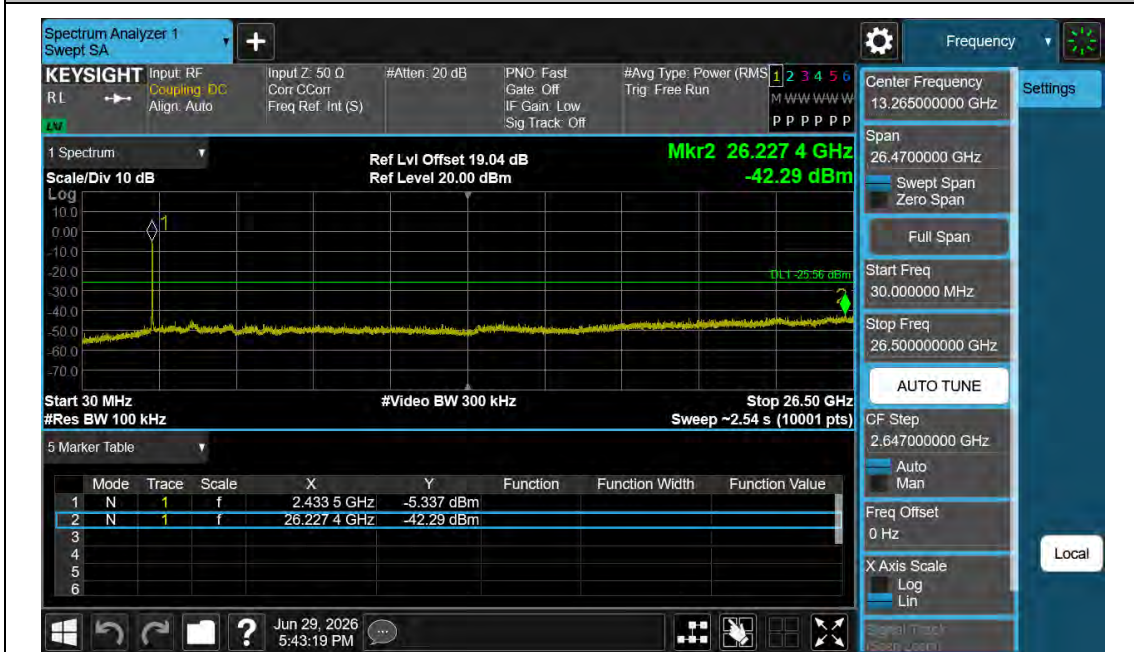
11AX40MIMO-Ant0-2452-30~26500-PASS
