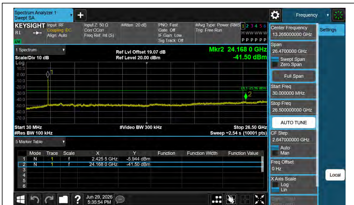
11AX40MIMO-Ant1-2422-30~26500-PASS
