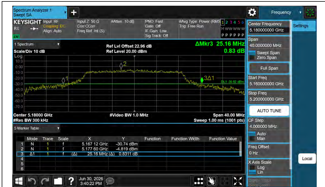
11AC20MIMO-Ant1-5180
