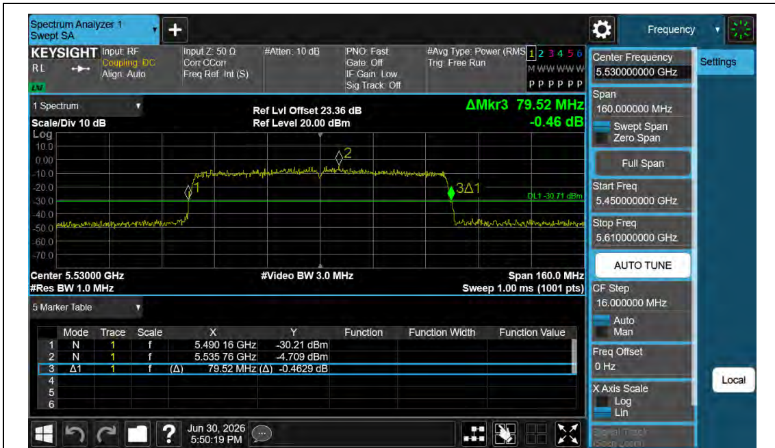
11AC80MIMO-Ant1-5530
