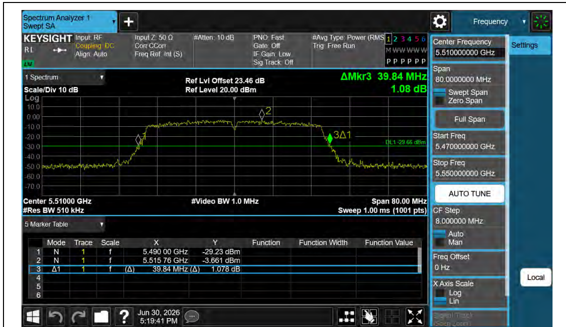
11AC40MIMO-Ant1-5510
