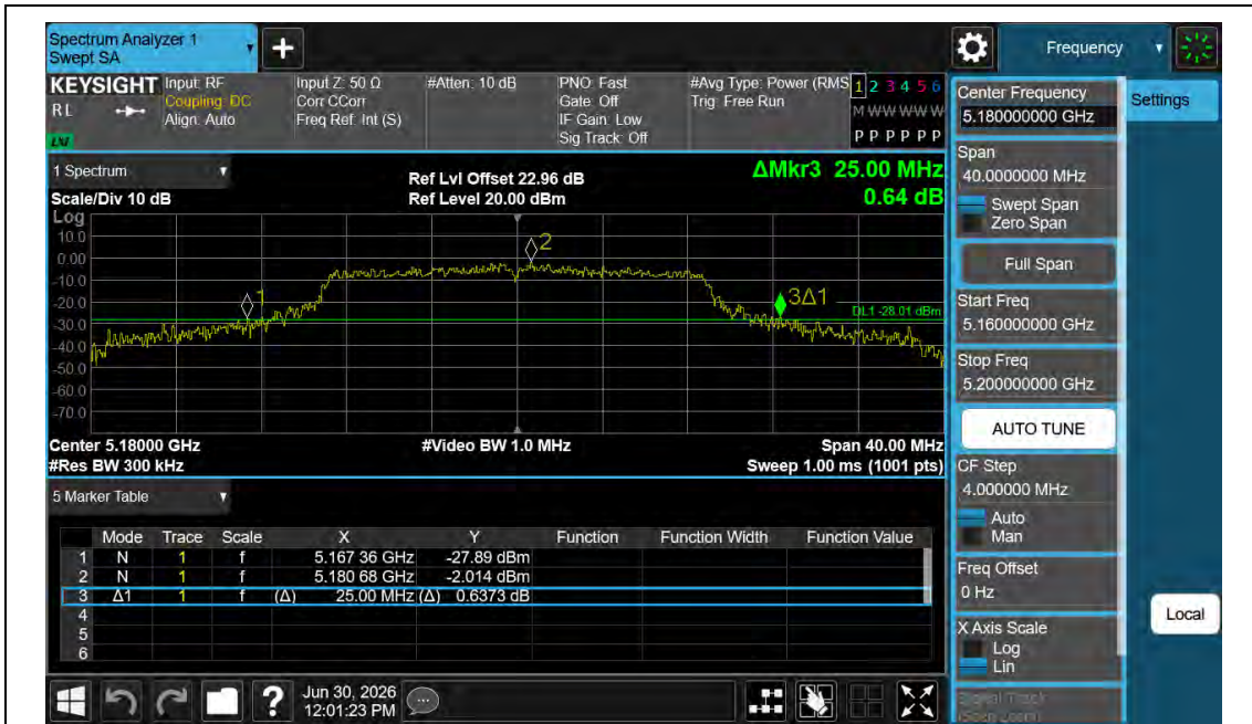
11N20MIMO-Ant1-5180
