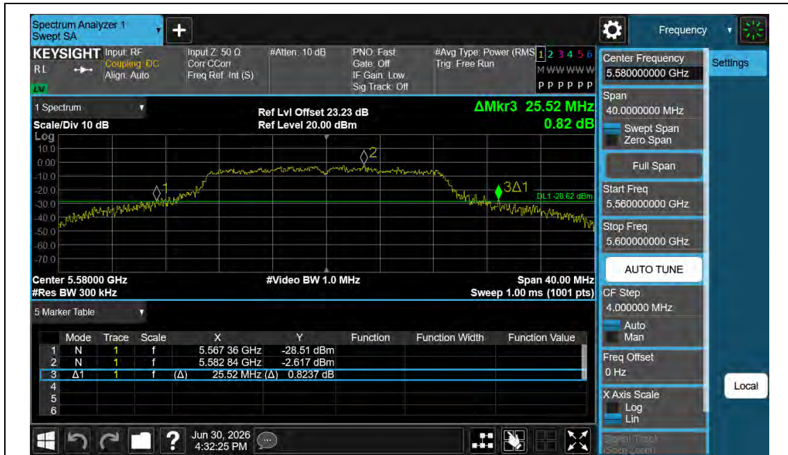
11AC20MIMO-Ant1-5580
