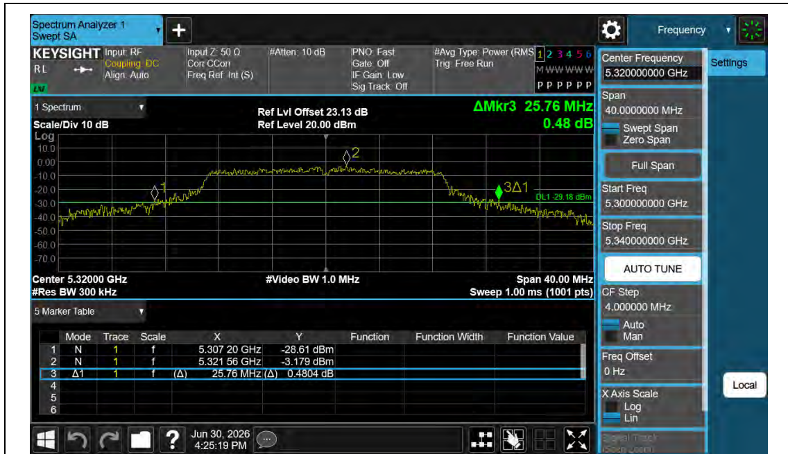
11AC20MIMO-Ant1-5320
