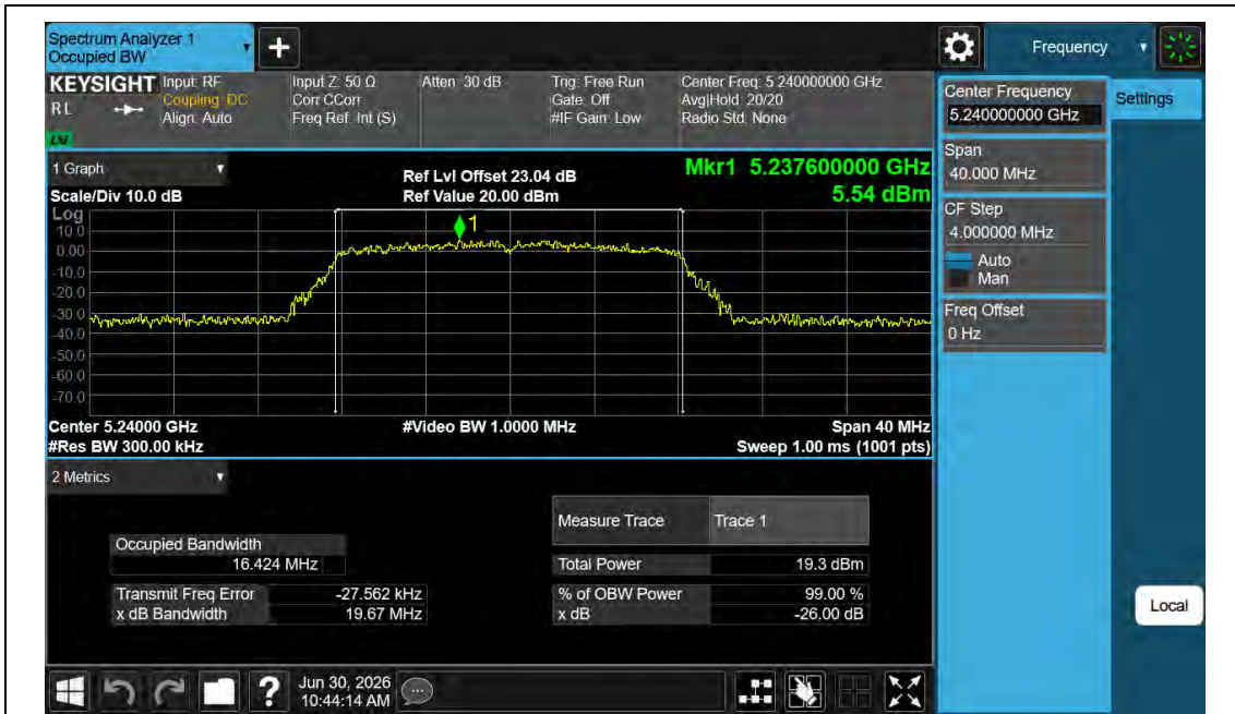
11A-Ant1-5240
