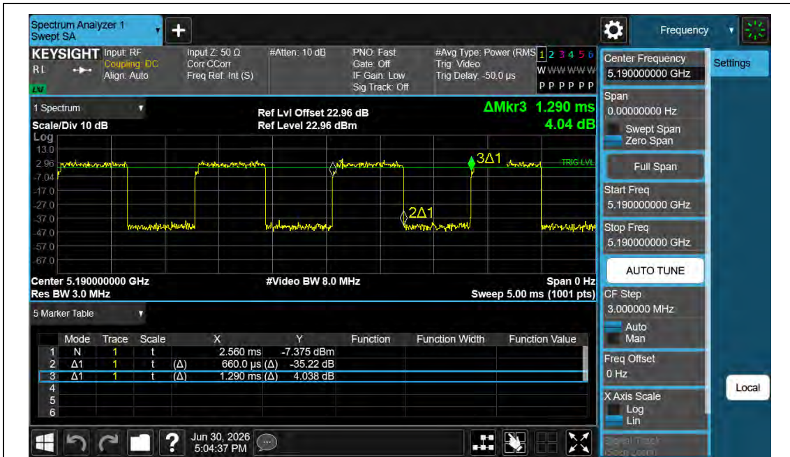
NTNV-11AC40MIMO-Ant1-5190
