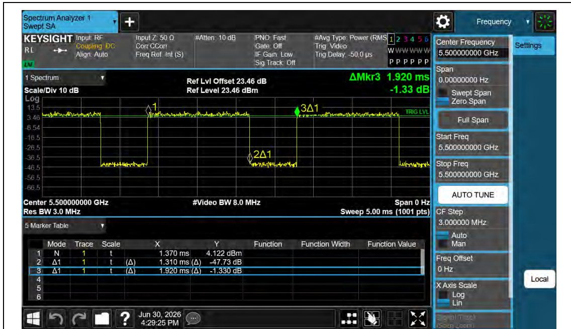
NTNV-11AC20MIMO-Ant1-5500
