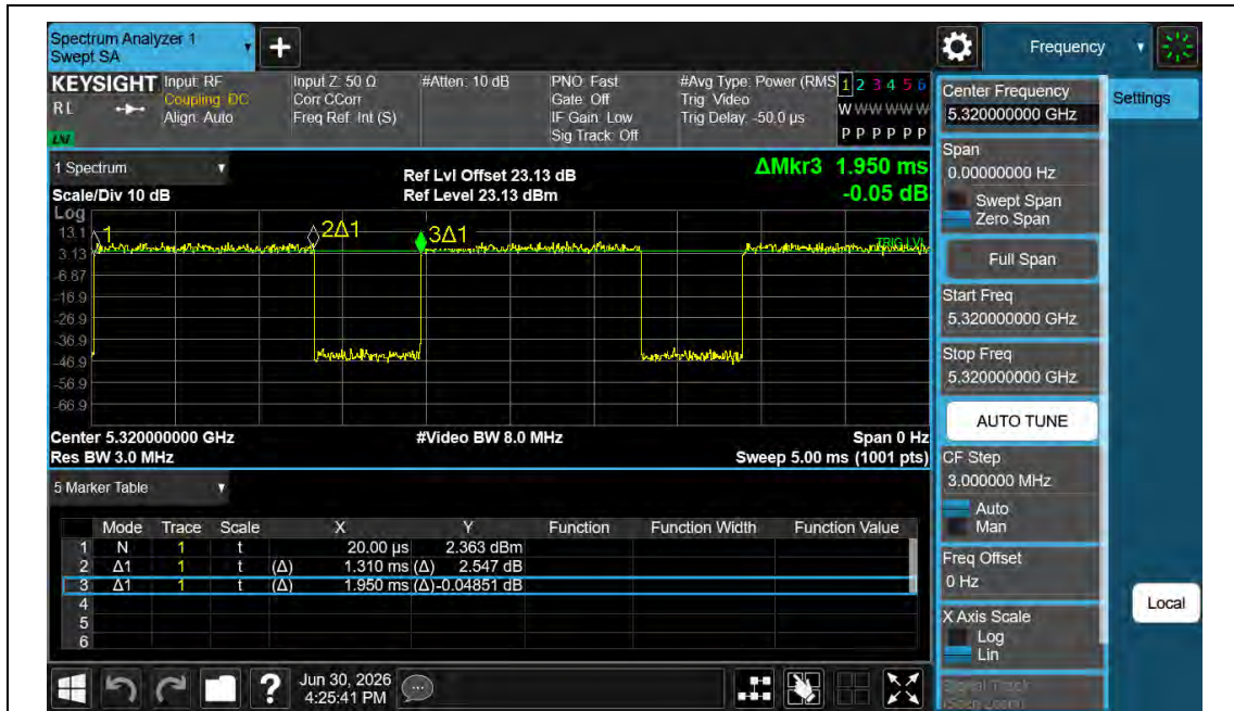
NTNV-11AC20MIMO-Ant1-5320
