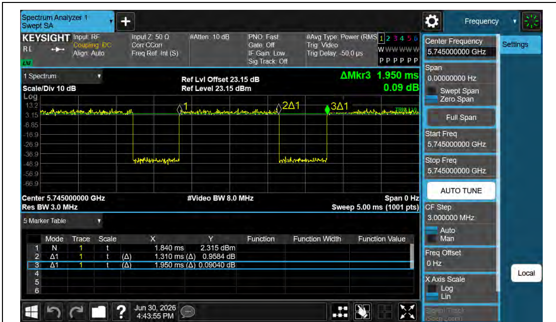
NTNV-11AC20MIMO-Ant1-5745
