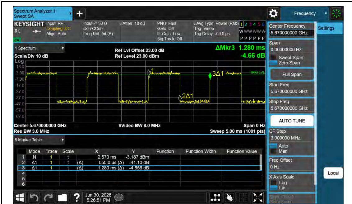
NTNV-11AC40MIMO-Ant1-5670
