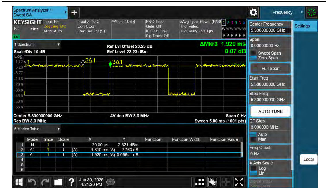
NTNV-11AC20MIMO-Ant1-5300
