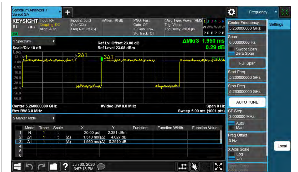
NTNV-11AC20MIMO-Ant1-5260
