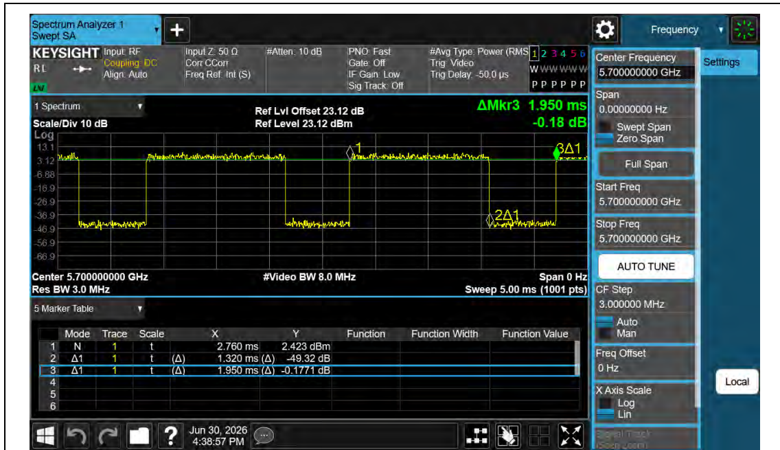
NTNV-11AC20MIMO-Ant1-5700
