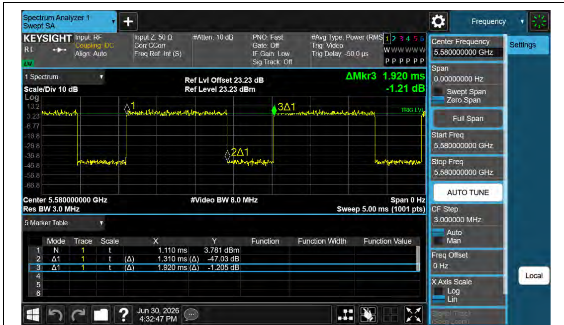
NTNV-11AC20MIMO-Ant1-5580
