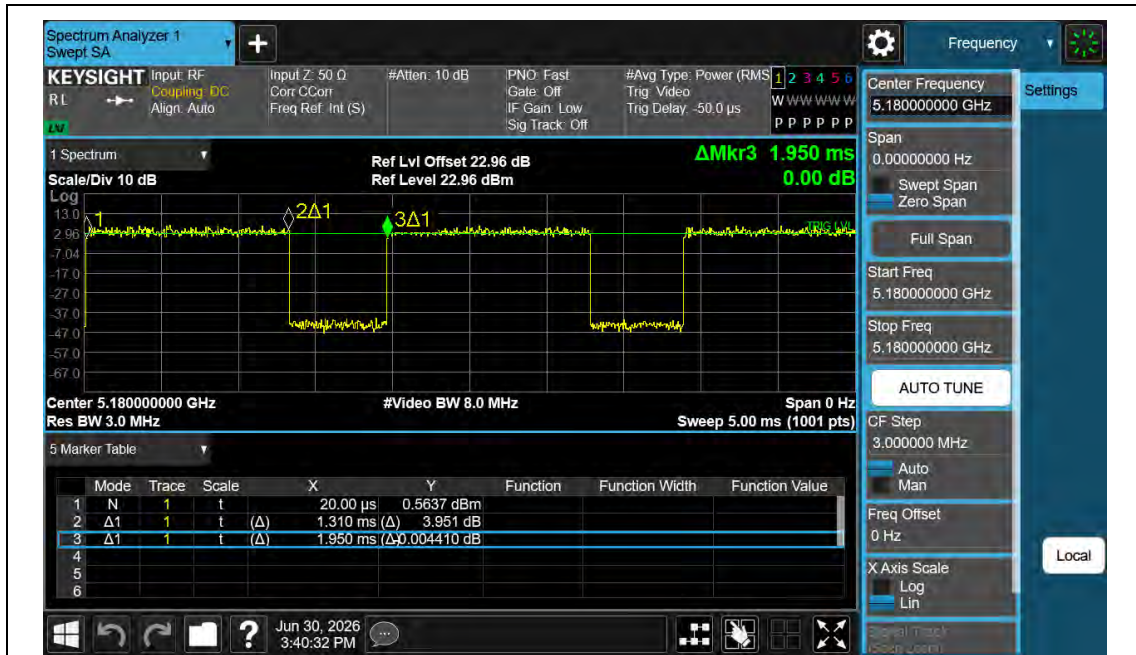
NTNV-11AC20MIMO-Ant1-5180
