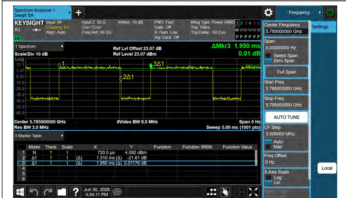
NTNV-11AC20MIMO-Ant0-5825
