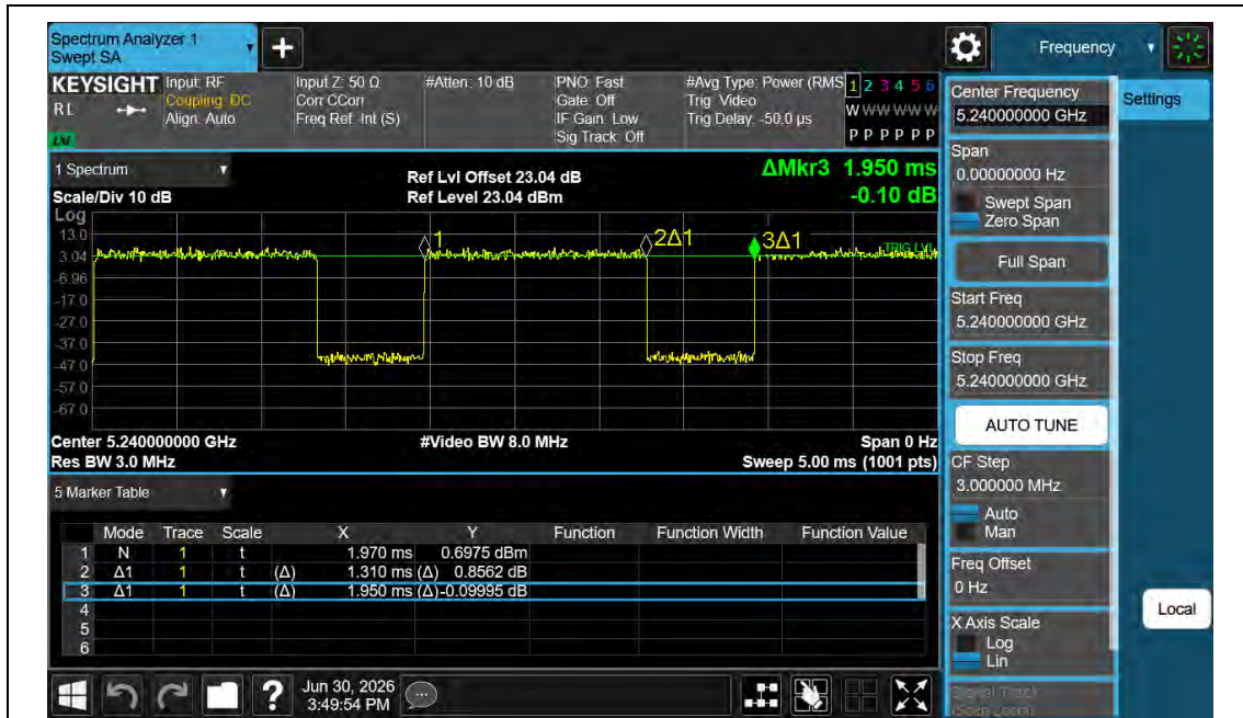
NTNV-11AC20MIMO-Ant1-5240
