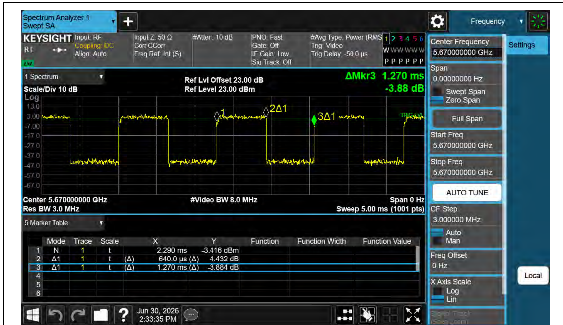
NTNV-11N40MIMO-Ant1-5670
