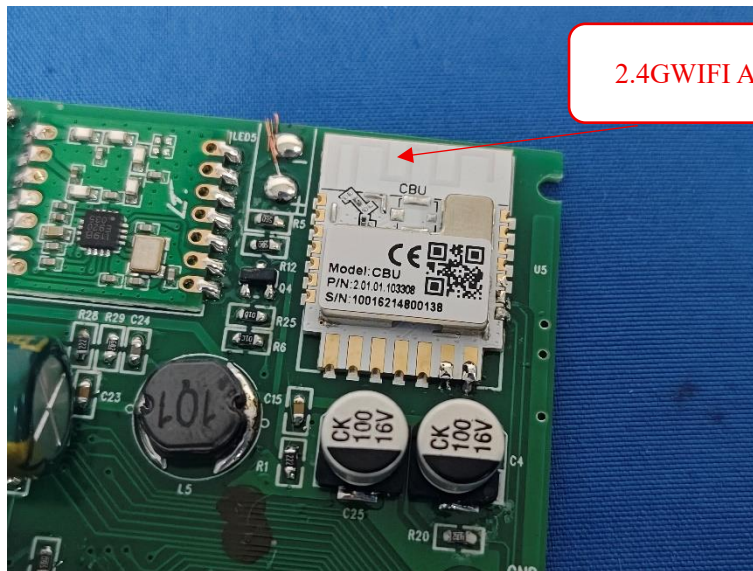
SRD Antenna
