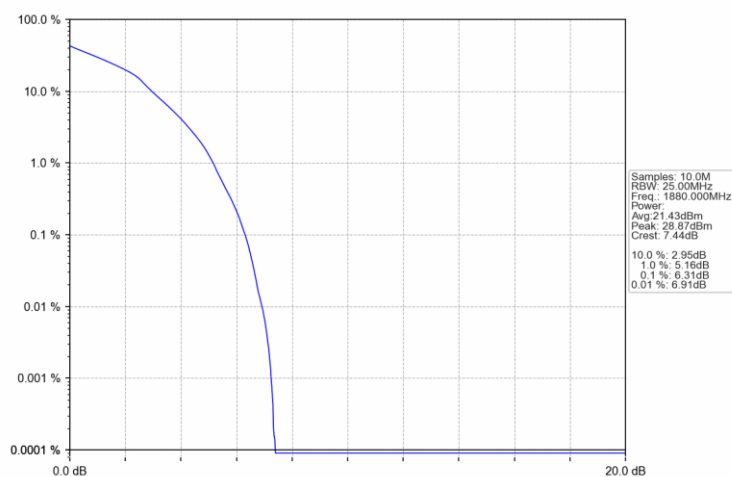
Band2_15MHz_16QAM_MCH_1880MHz_RB_27_0_NTNV
