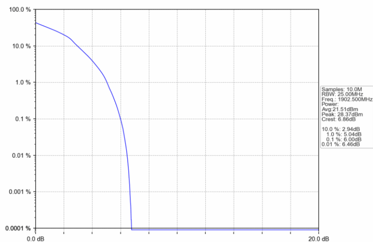
Band2_15MHz_16QAM_HCH_1902.5MHz_RB_27_48_NTNV
