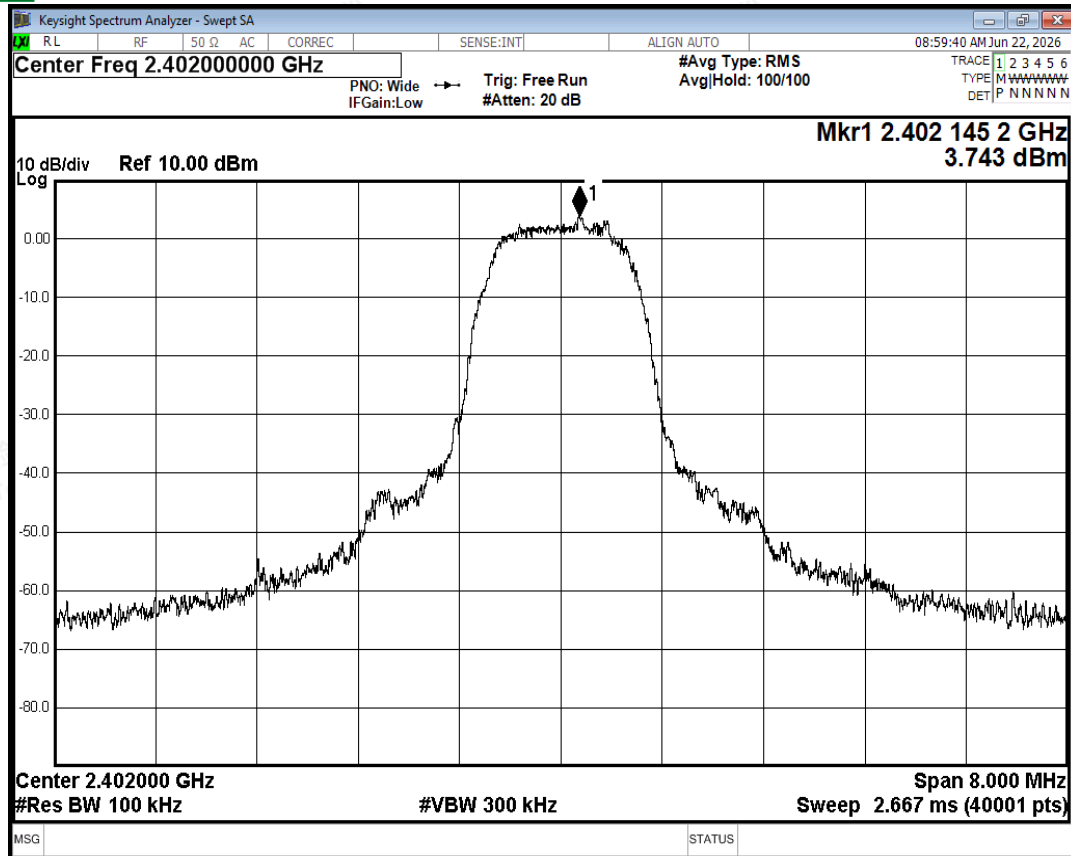
Tx. Spurious NVNT 3-DH5 2402MHz Ant2 Ref
