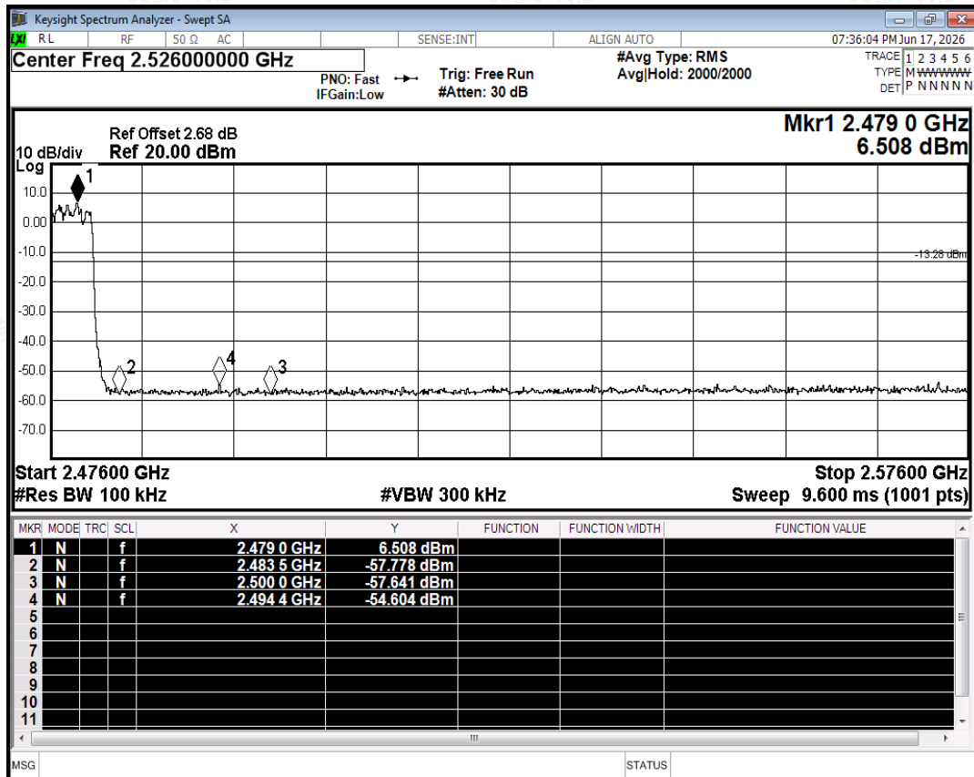
Band Edge(Hopping) NVNT 2-DH5 2480MHz Ant2 Hopping Emission
