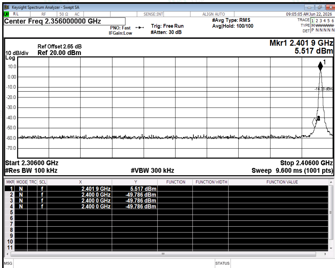
Band Edge NVNT 1-DH5 2402MHz Ant2 No-Hopping Emission
