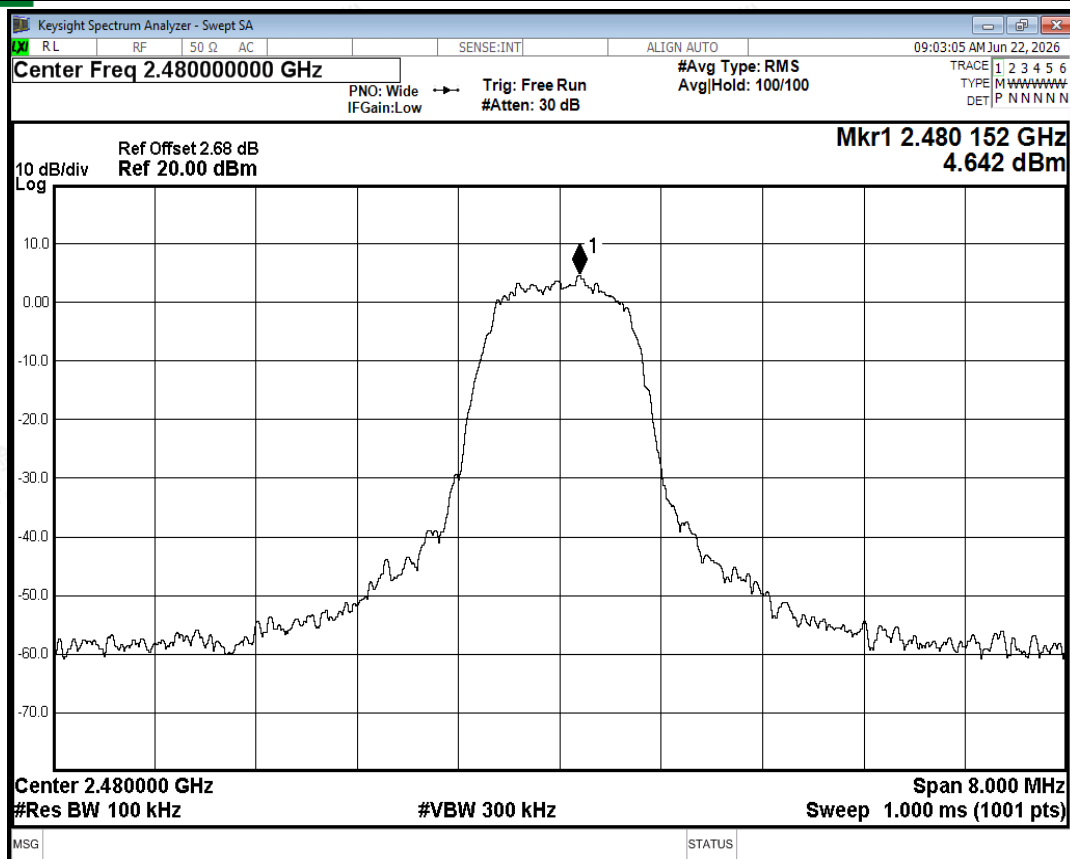
Band Edge NVNT 3-DH5 2480MHz Ant2 No-Hopping Ref
