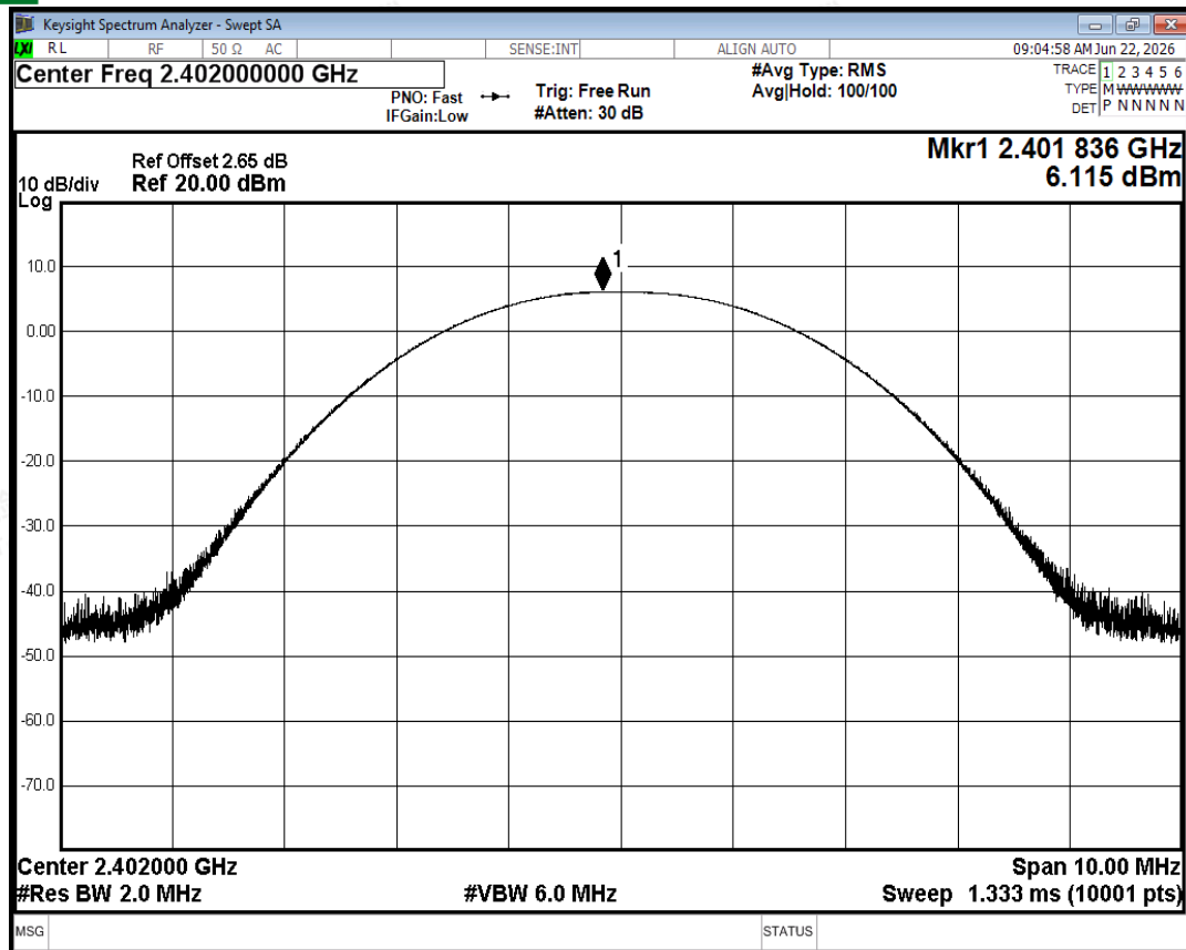
Peak Power NVNT 1-DH5 2402MHz Ant2
