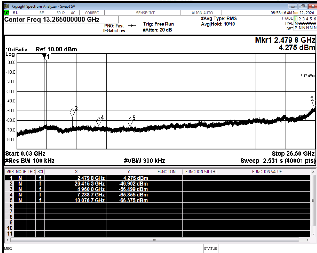
Tx. Spurious NVNT 2-DH5 2480MHz Ant2 Emission
