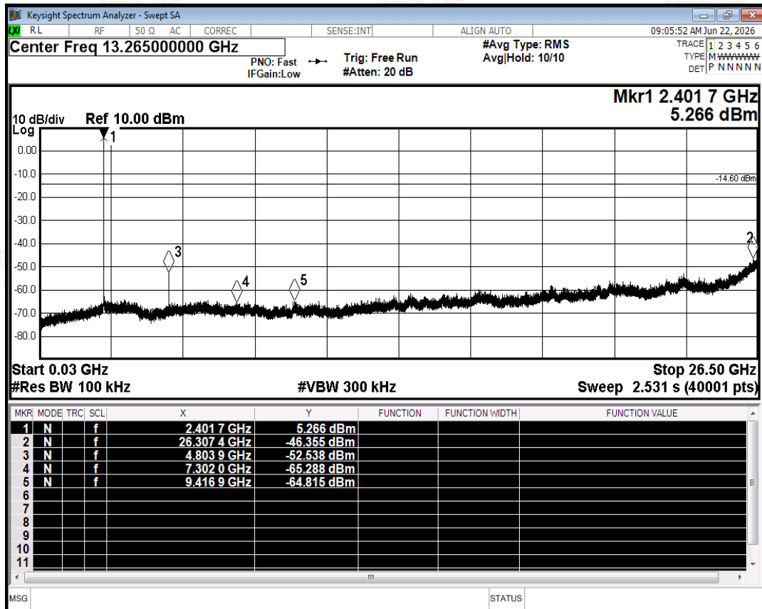
Tx. Spurious NVNT 1-DH5 2402MHz Ant2 Emission
