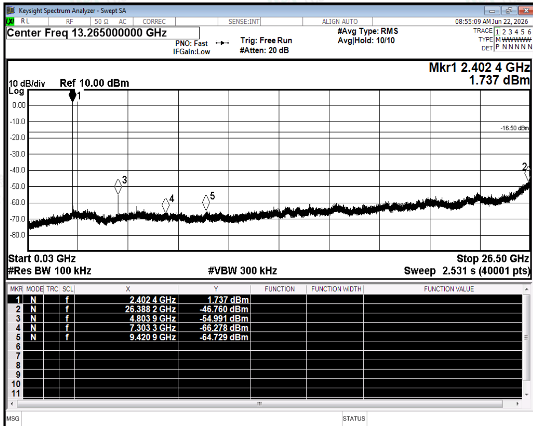
Tx. Spurious NVNT 2-DH5 2402MHz Ant2 Emission
