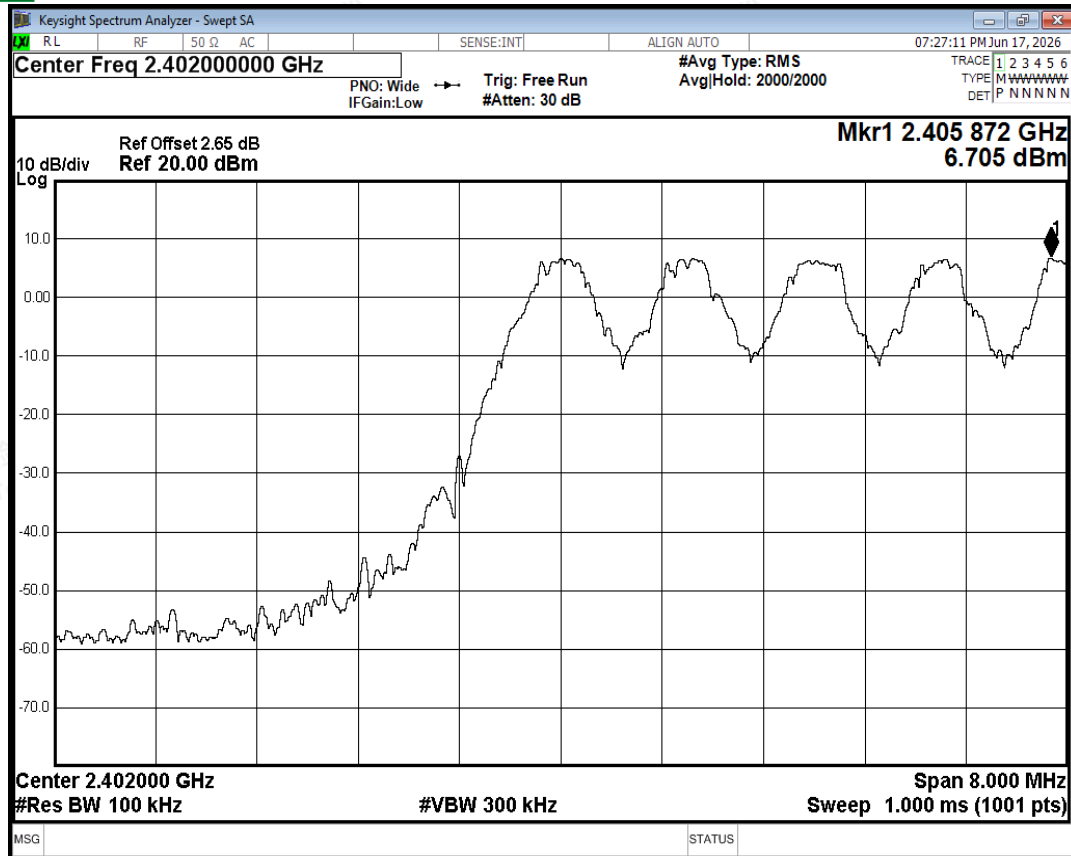
Band Edge(Hopping) NVNT 1-DH5 2402MHz Ant2 Hopping Ref
