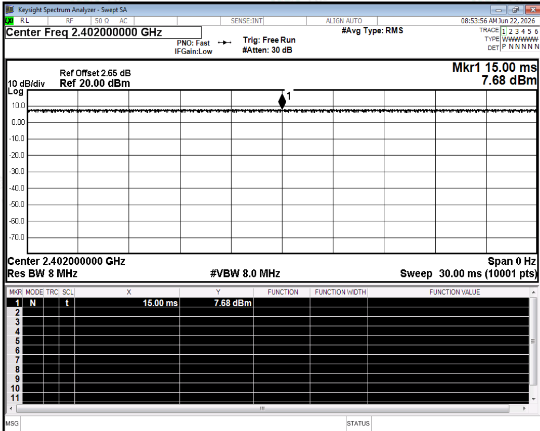
Duty Cycle NVNT 2-DH5 2402MHz Ant2
