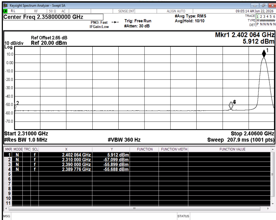
Restrict Band NVNT 1-DH5 2402MHz Ant2 No-Hopping Average
