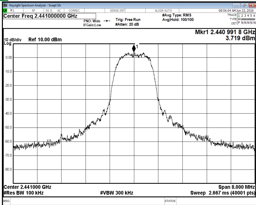
Tx. Spurious NVNT 2-DH5 2441MHz Ant2 Ref
