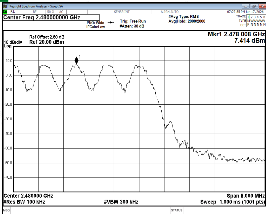
Band Edge(Hopping) NVNT 1-DH5 2480MHz Ant2 Hopping Ref
