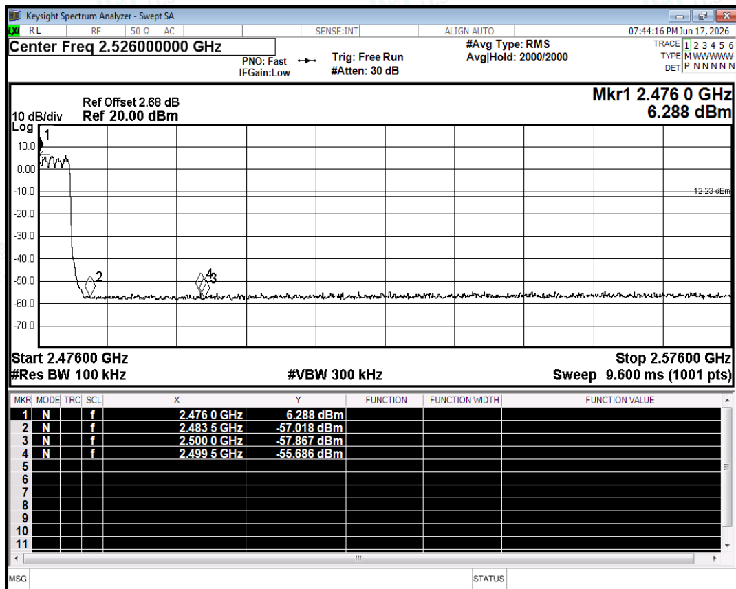
Band Edge(Hopping) NVNT 3-DH5 2480MHz Ant2 Hopping Emission
