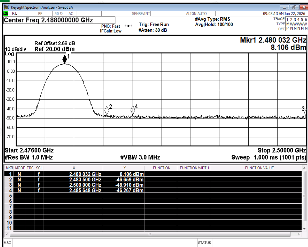
Restrict Band NVNT 3-DH5 2480MHz Ant2 No-Hopping Peak
