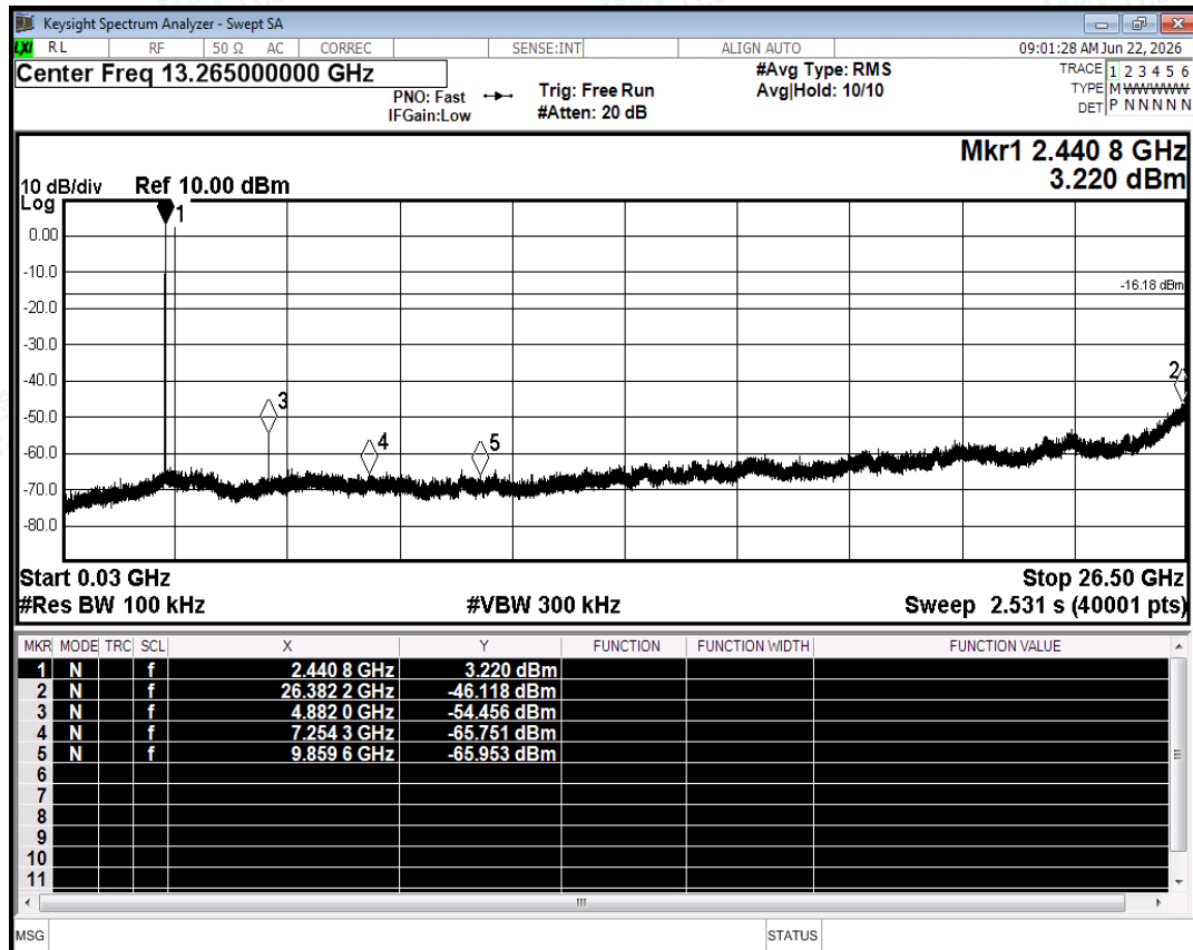
Tx. Spurious NVNT 3-DH5 2441MHz Ant2 Emission
