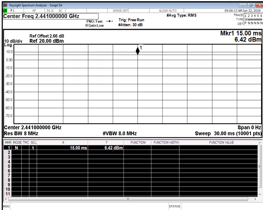
Duty Cycle NVNT 1-DH5 2441MHz Ant2
