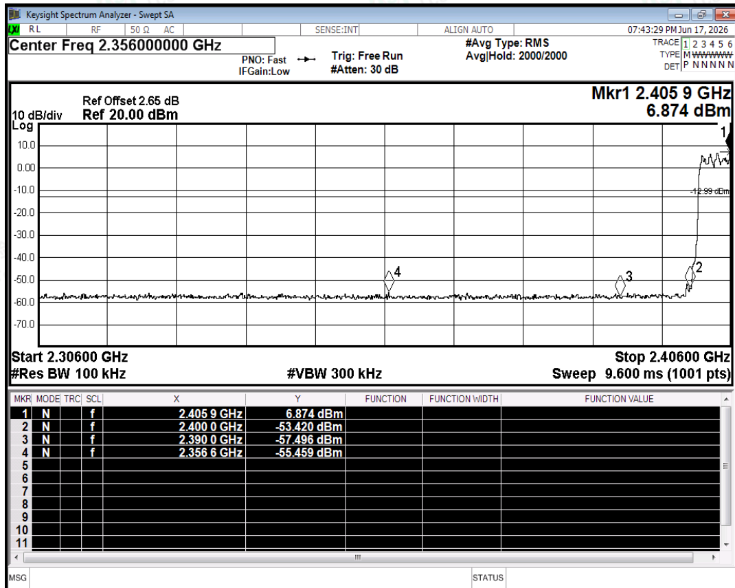
Band Edge(Hopping) NVNT 3-DH5 2402MHz Ant2 Hopping Emission
