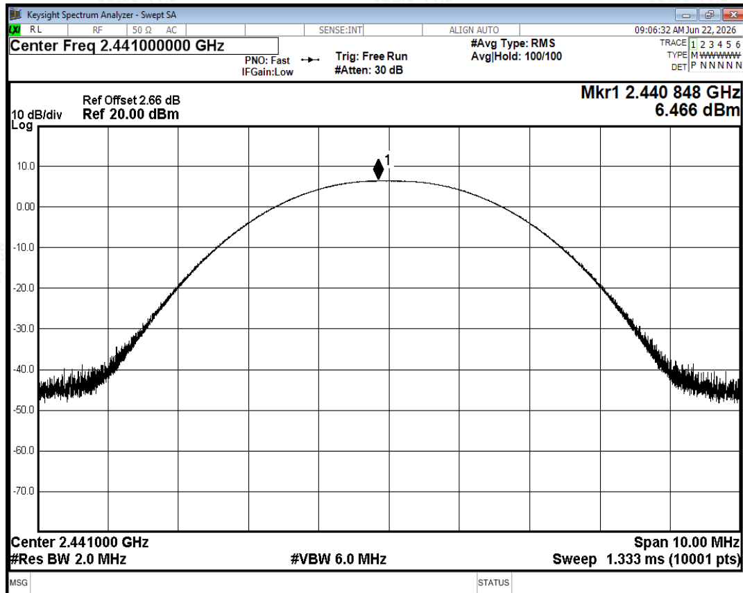
Peak Power NVNT 1-DH5 2441MHz Ant2
