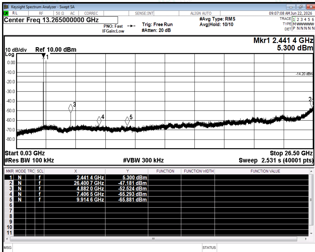
Tx. Spurious NVNT 1-DH5 2441MHz Ant2 Emission
