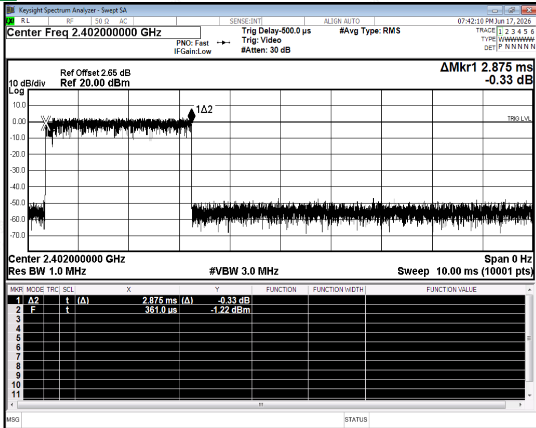
Dwell NVNT 3-DH5 2402MHz Ant2 One Burst
