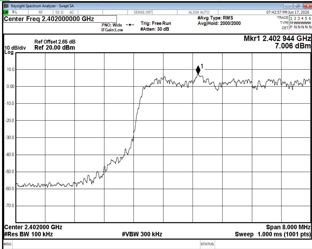
Band Edge(Hopping) NVNT 3-DH5 2402MHz Ant2 Hopping Ref
