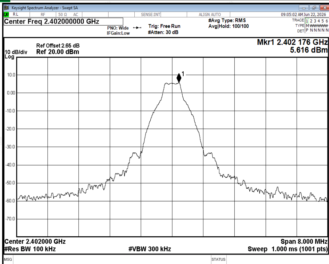
Band Edge NVNT 1-DH5 2402MHz Ant2 No-Hopping Ref
