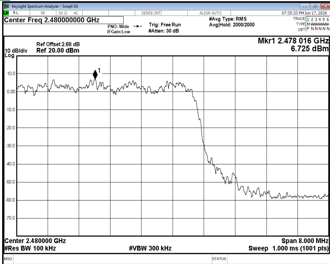
Band Edge(Hopping) NVNT 2-DH5 2480MHz Ant2 Hopping Ref
