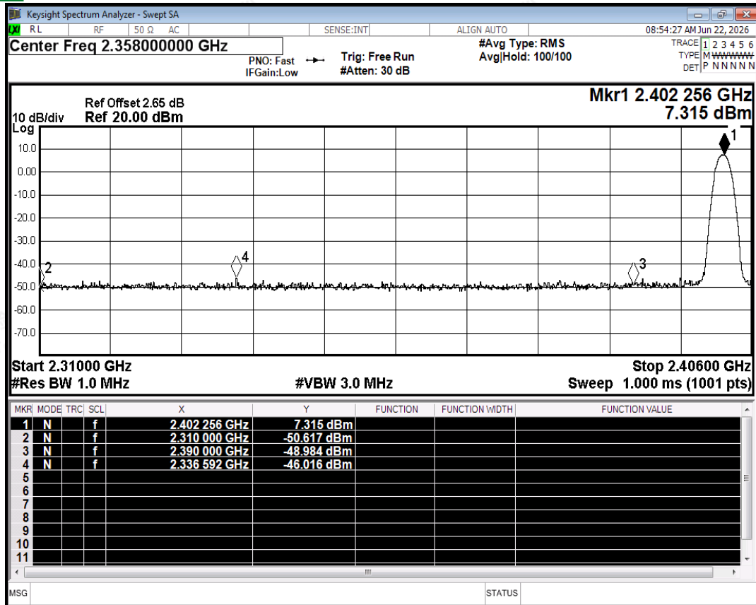
Restrict Band NVNT 2-DH5 2402MHz Ant2 No-Hopping Peak
