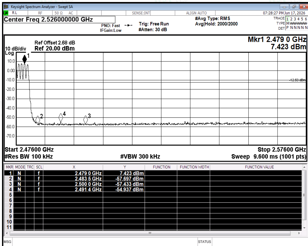
Band Edge(Hopping) NVNT 1-DH5 2480MHz Ant2 Hopping Emission
