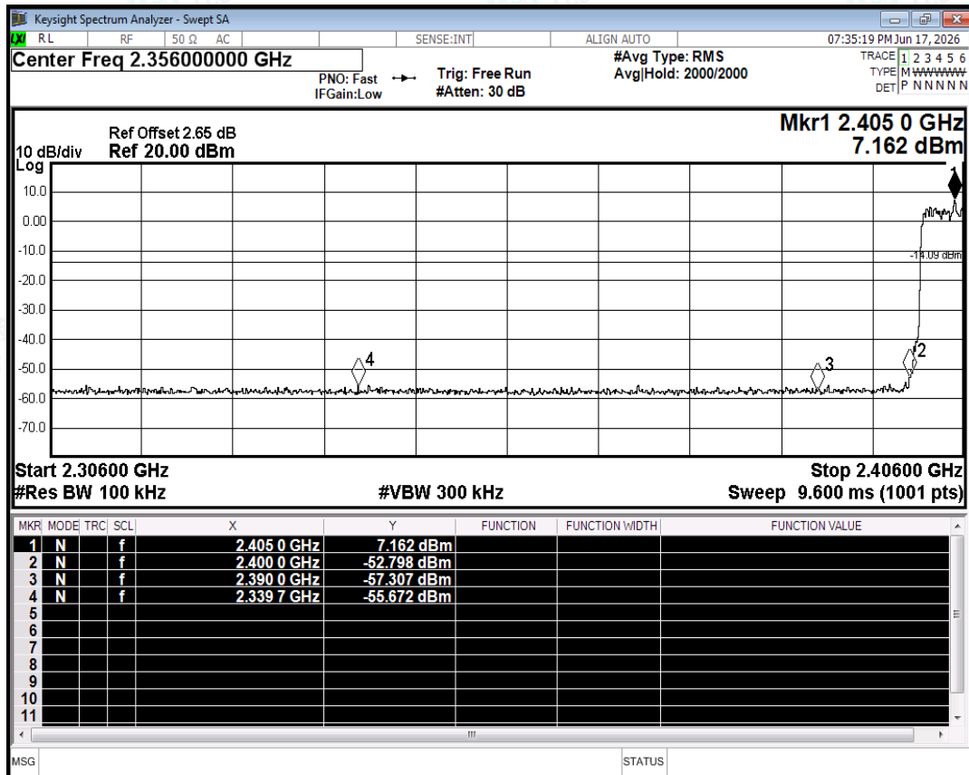
Band Edge(Hopping) NVNT 2-DH5 2402MHz Ant2 Hopping Emission
