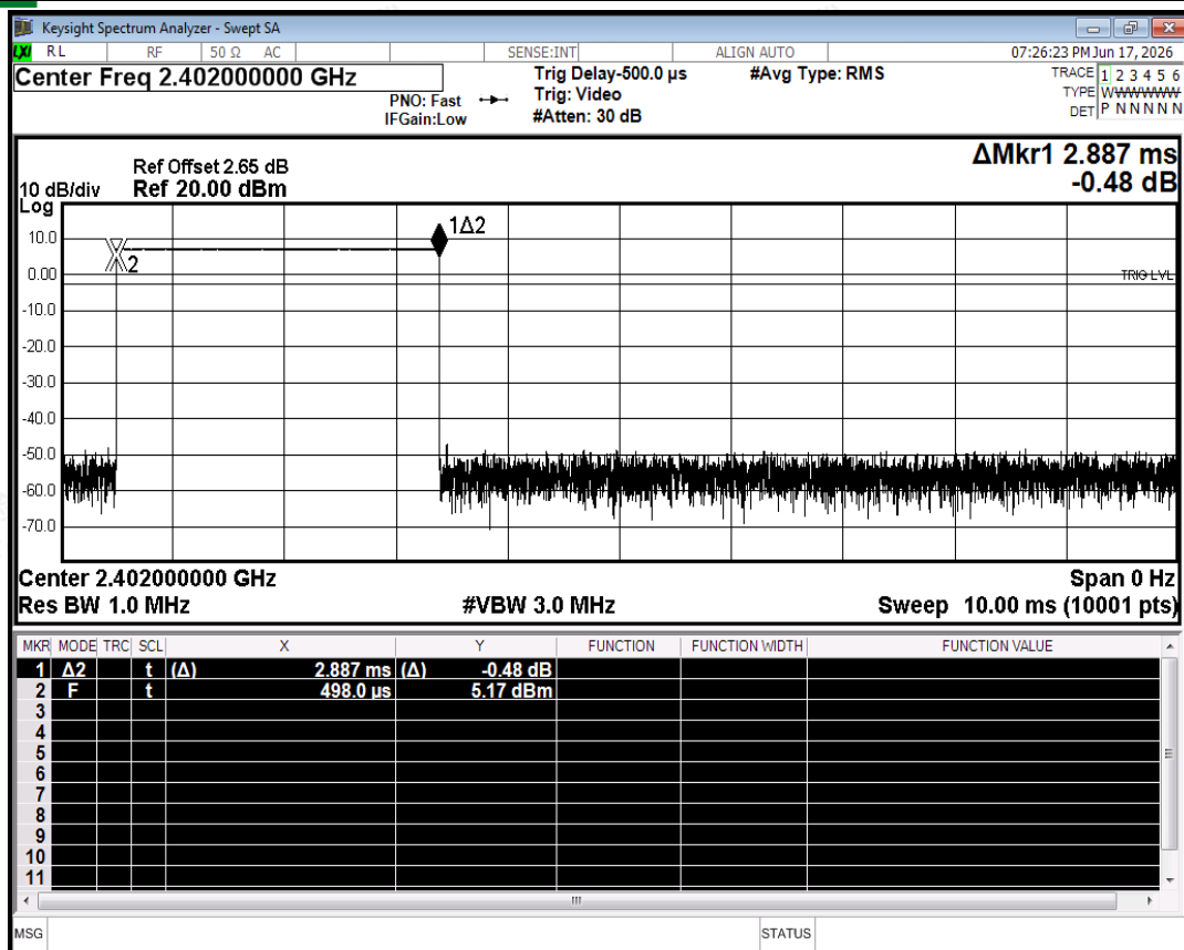
Dwell NVNT 1-DH5 2402MHz Ant2 One Burst
