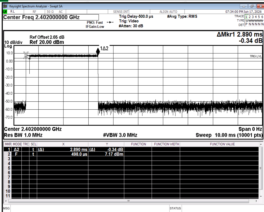
Dwell NVNT 2-DH5 2402MHz Ant2 One Burst
