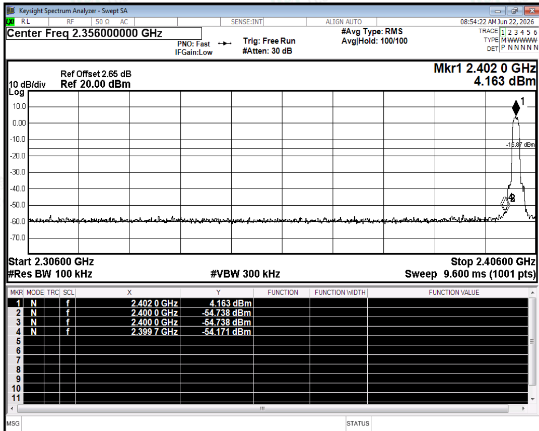
Band Edge NVNT 2-DH5 2402MHz Ant2 No-Hopping Emission
