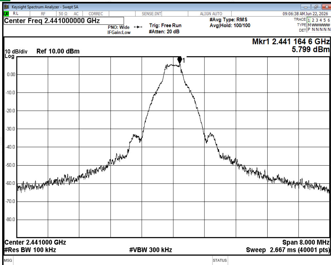
Tx. Spurious NVNT 1-DH5 2441MHz Ant2 Ref
