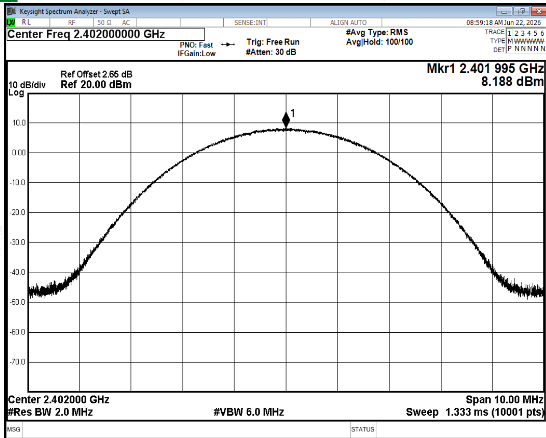
Peak Power NVNT 3-DH5 2402MHz Ant2
