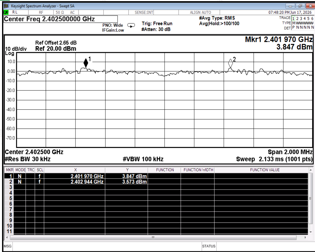
CFS NVNT 3-DH5 2402MHz Ant2
