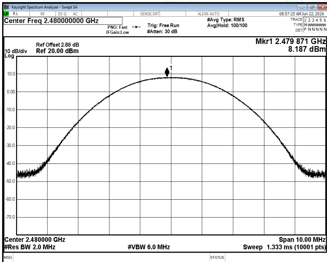
Peak Power NVNT 2-DH5 2480MHz Ant2
