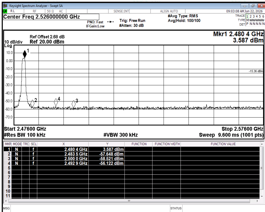
Band Edge NVNT 3-DH5 2480MHz Ant2 No-Hopping Emission
