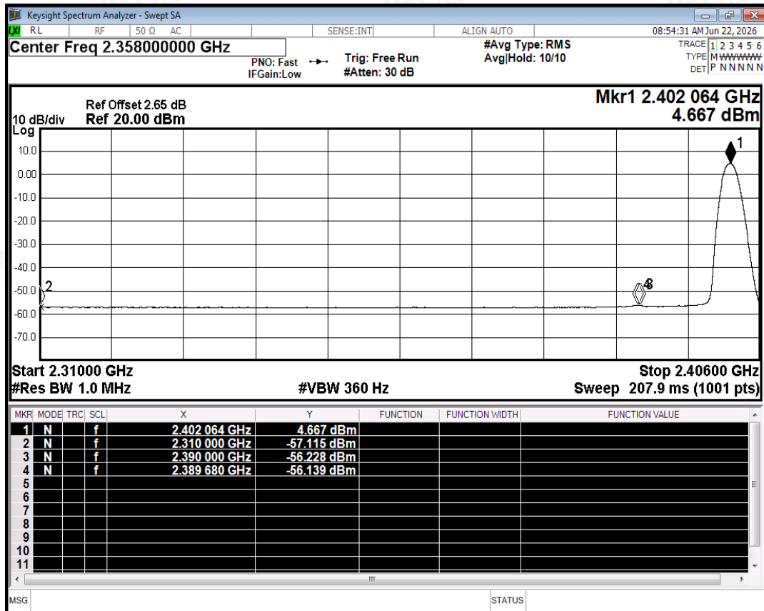
Restrict Band NVNT 2-DH5 2402MHz Ant2 No-Hopping Average
