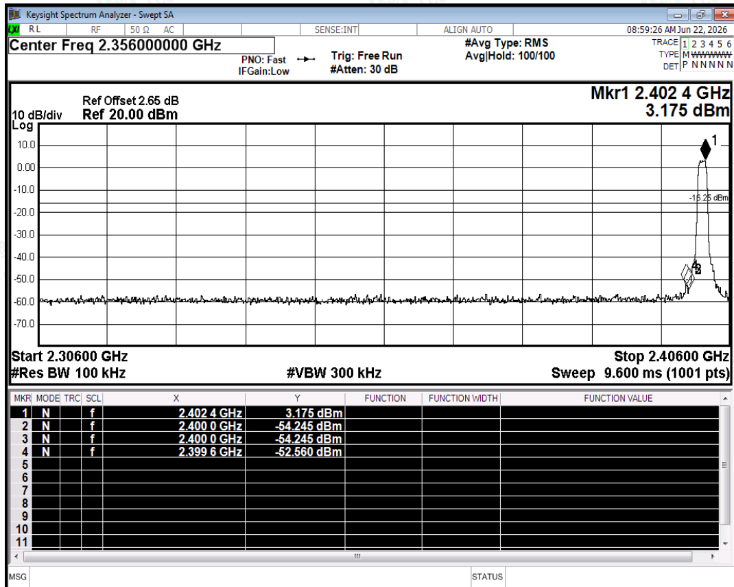
Band Edge NVNT 3-DH5 2402MHz Ant2 No-Hopping Emission
