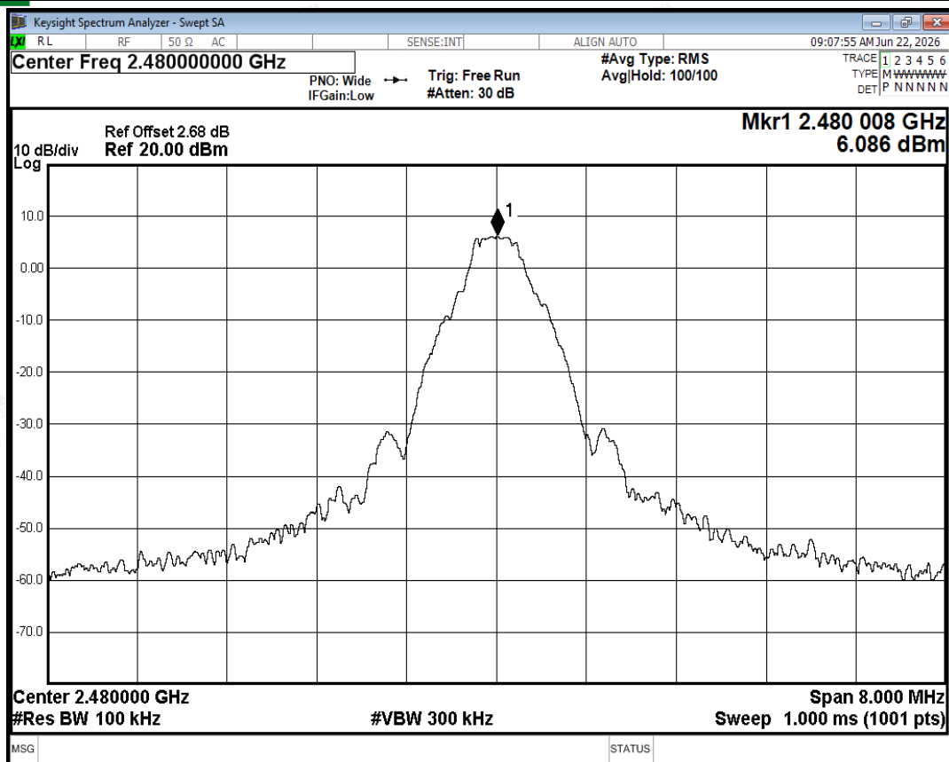
Band Edge NVNT 1-DH5 2480MHz Ant2 No-Hopping Ref
