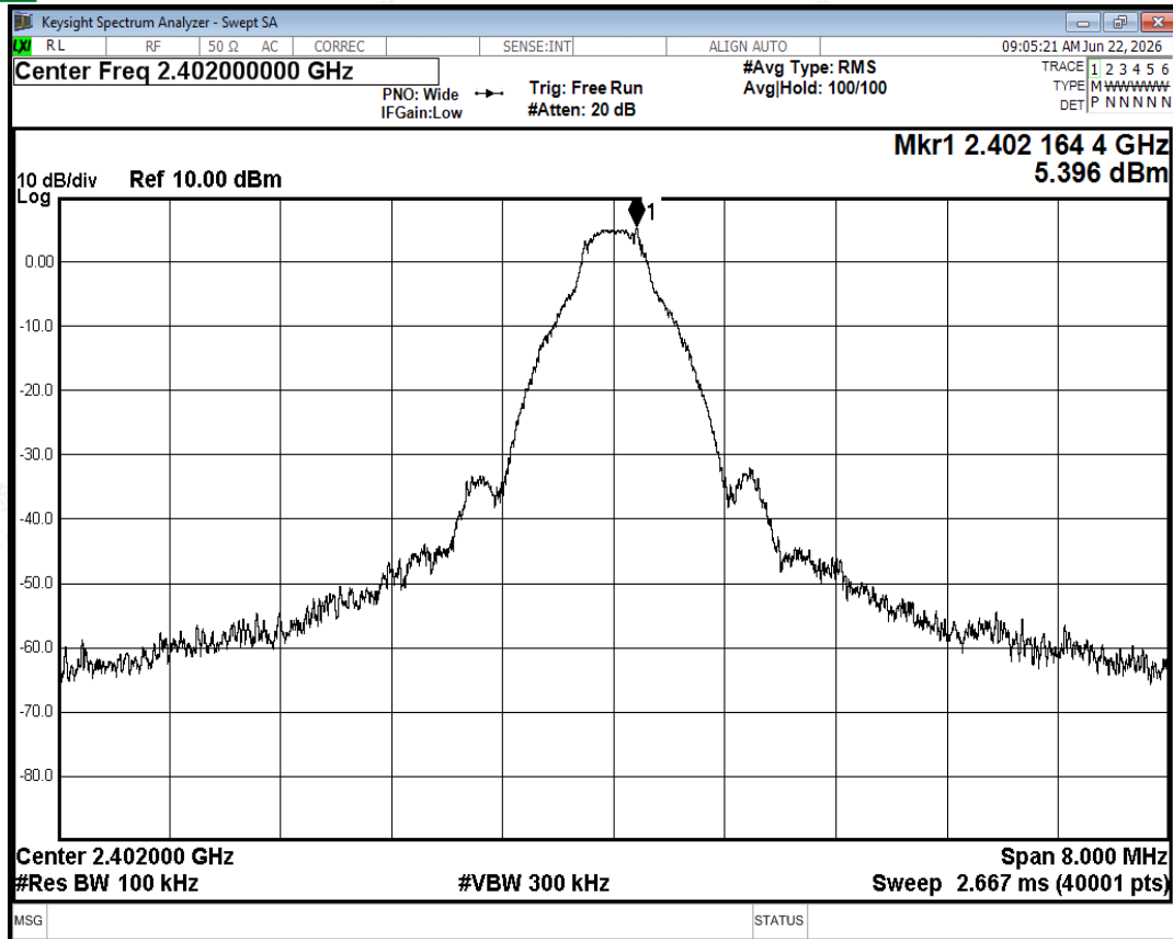
Tx. Spurious NVNT 1-DH5 2402MHz Ant2 Ref
