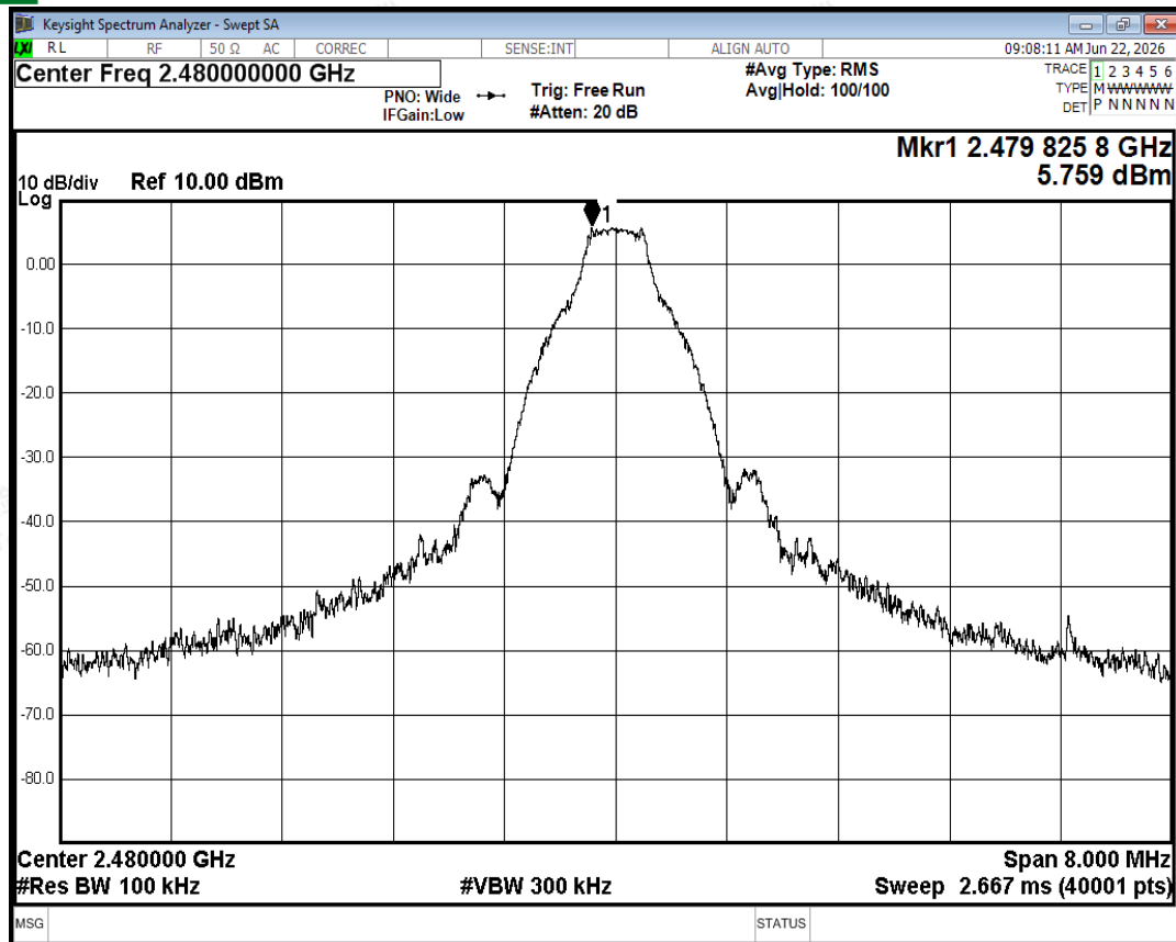
Tx. Spurious NVNT 1-DH5 2480MHz Ant2 Ref
