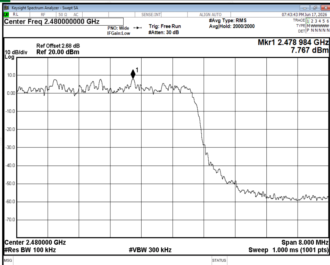
Band Edge(Hopping) NVNT 3-DH5 2480MHz Ant2 Hopping Ref
