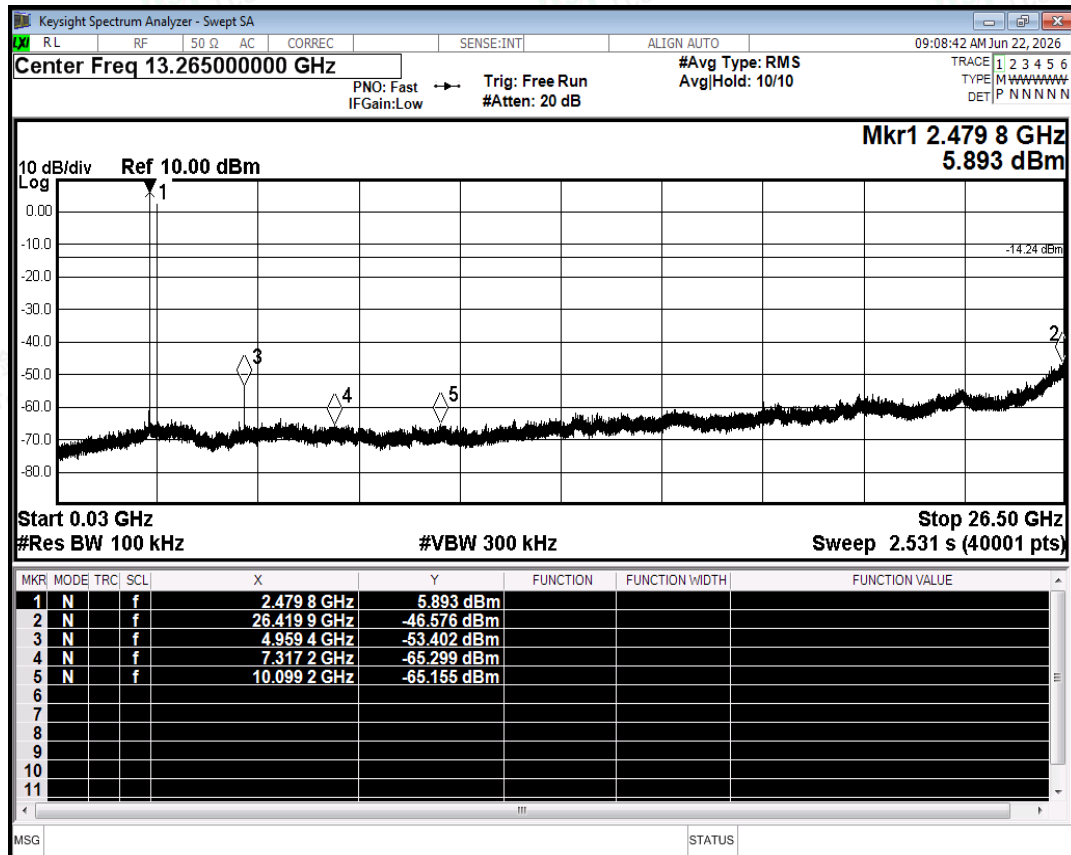
Tx. Spurious NVNT 1-DH5 2480MHz Ant2 Emission
