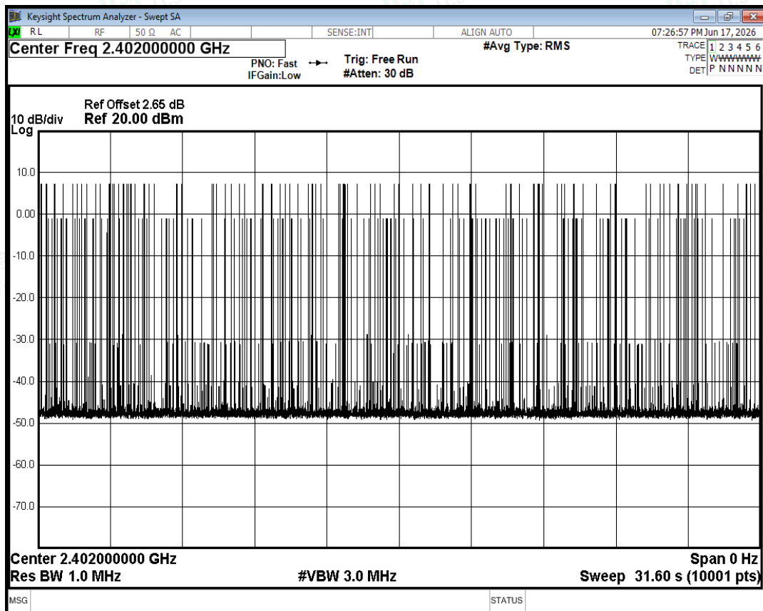
Dwell NVNT 1-DH5 2402MHz Ant2 Accumulated
