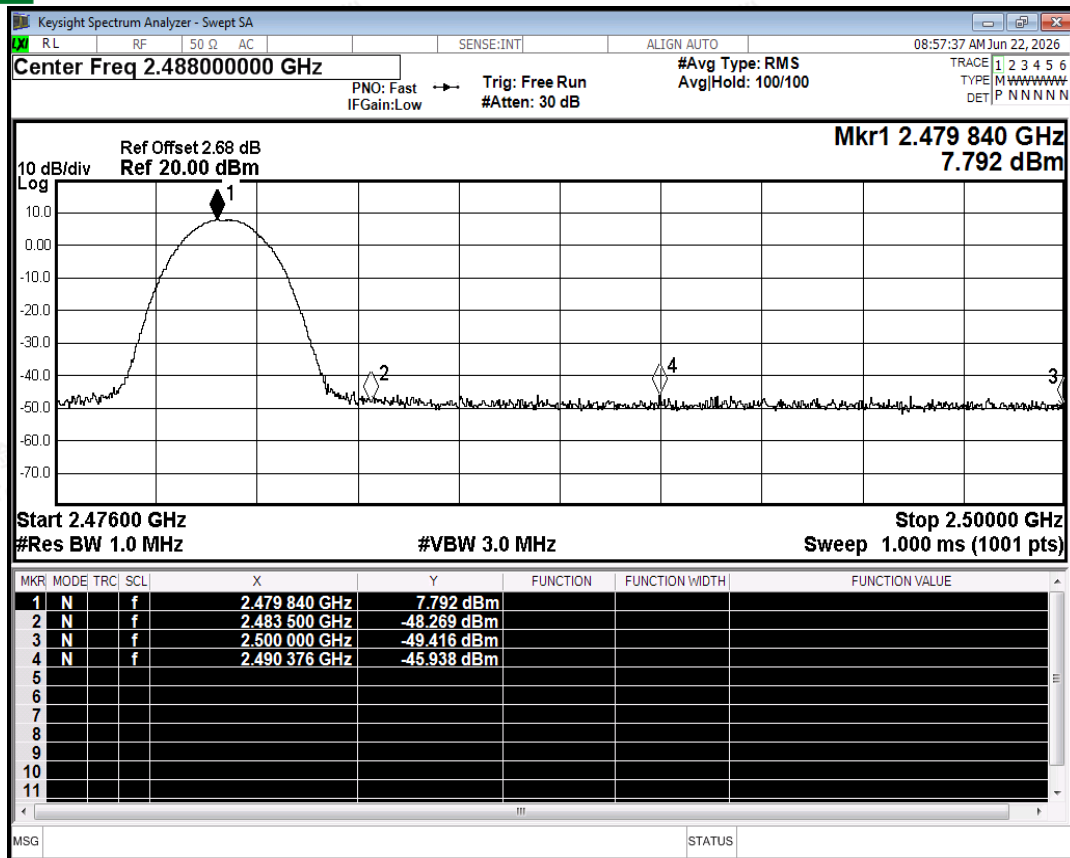
Restrict Band NVNT 2-DH5 2480MHz Ant2 No-Hopping Peak
