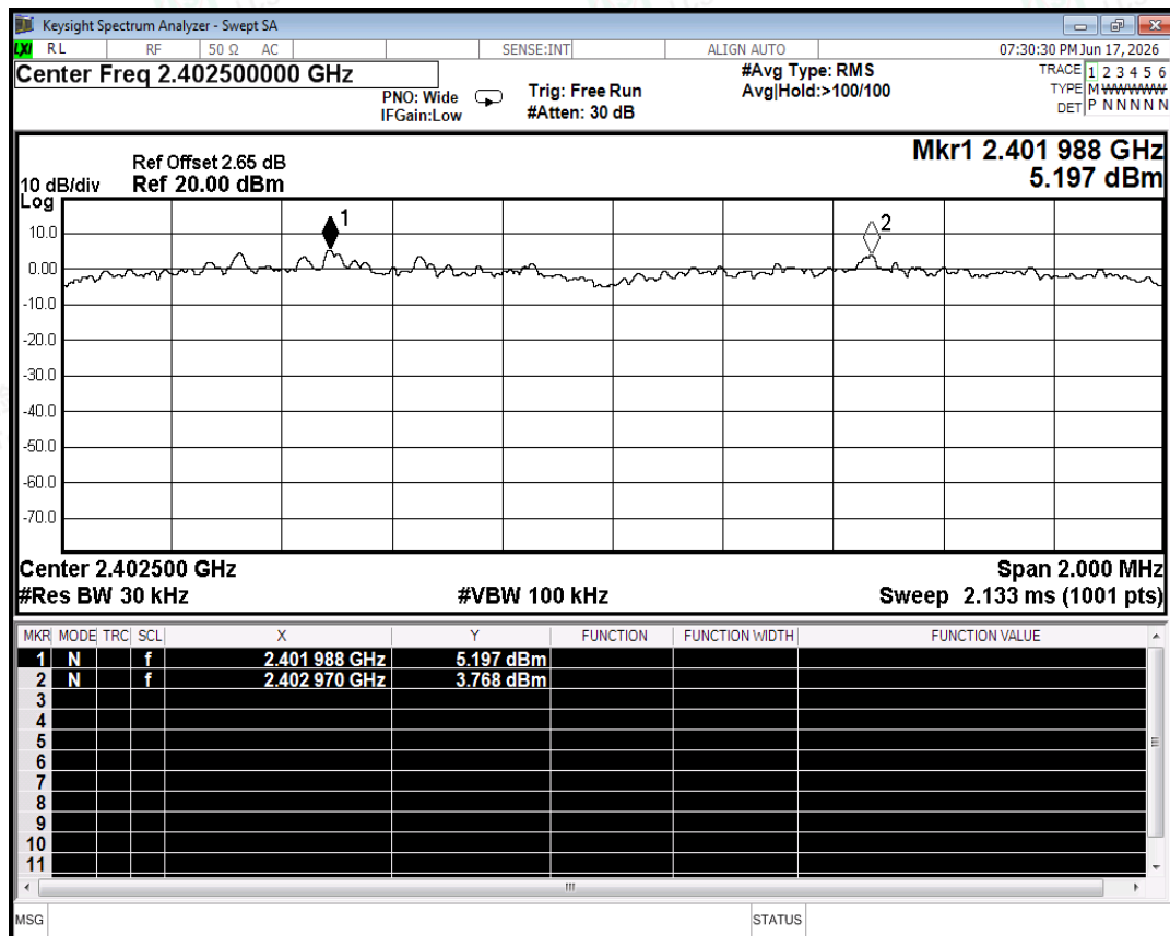
CFS NVNT 2-DH5 2402MHz Ant2
