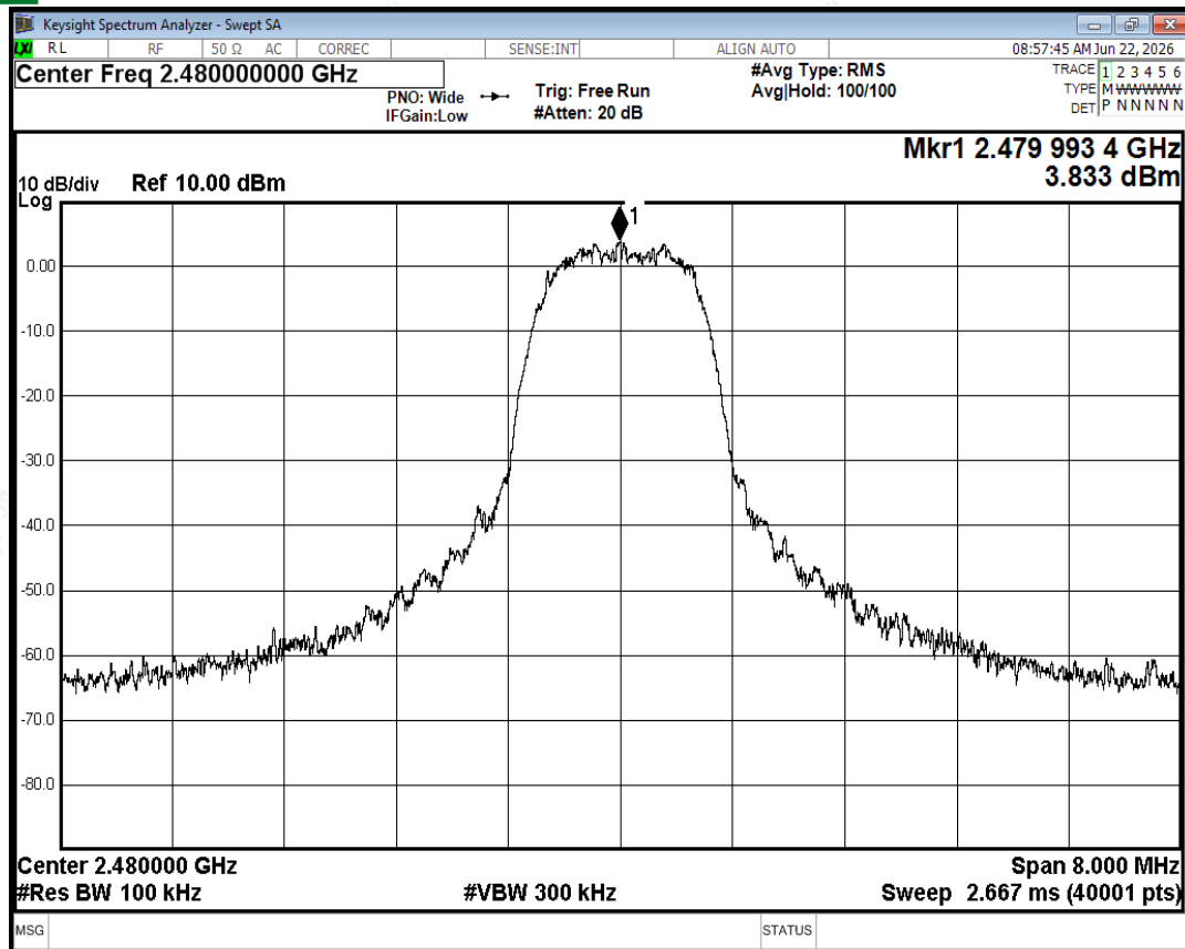
Tx. Spurious NVNT 2-DH5 2480MHz Ant2 Ref
