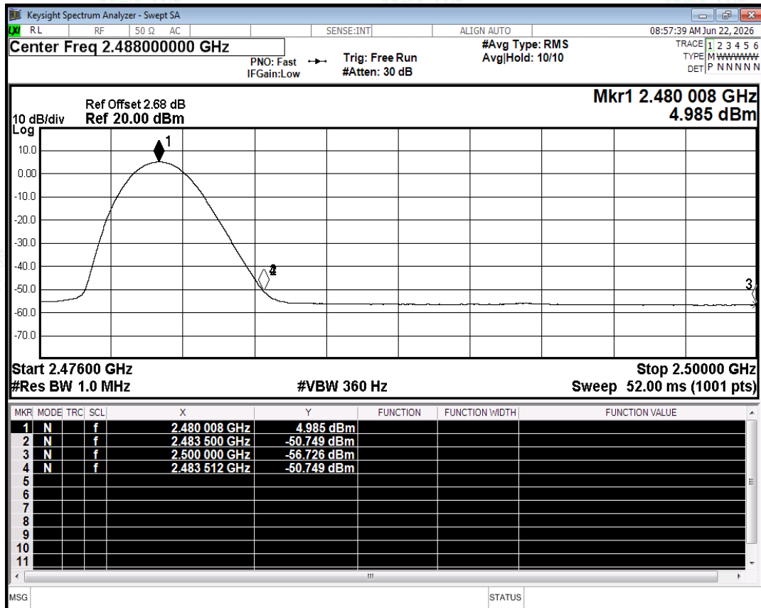
Restrict Band NVNT 2-DH5 2480MHz Ant2 No-Hopping Average
