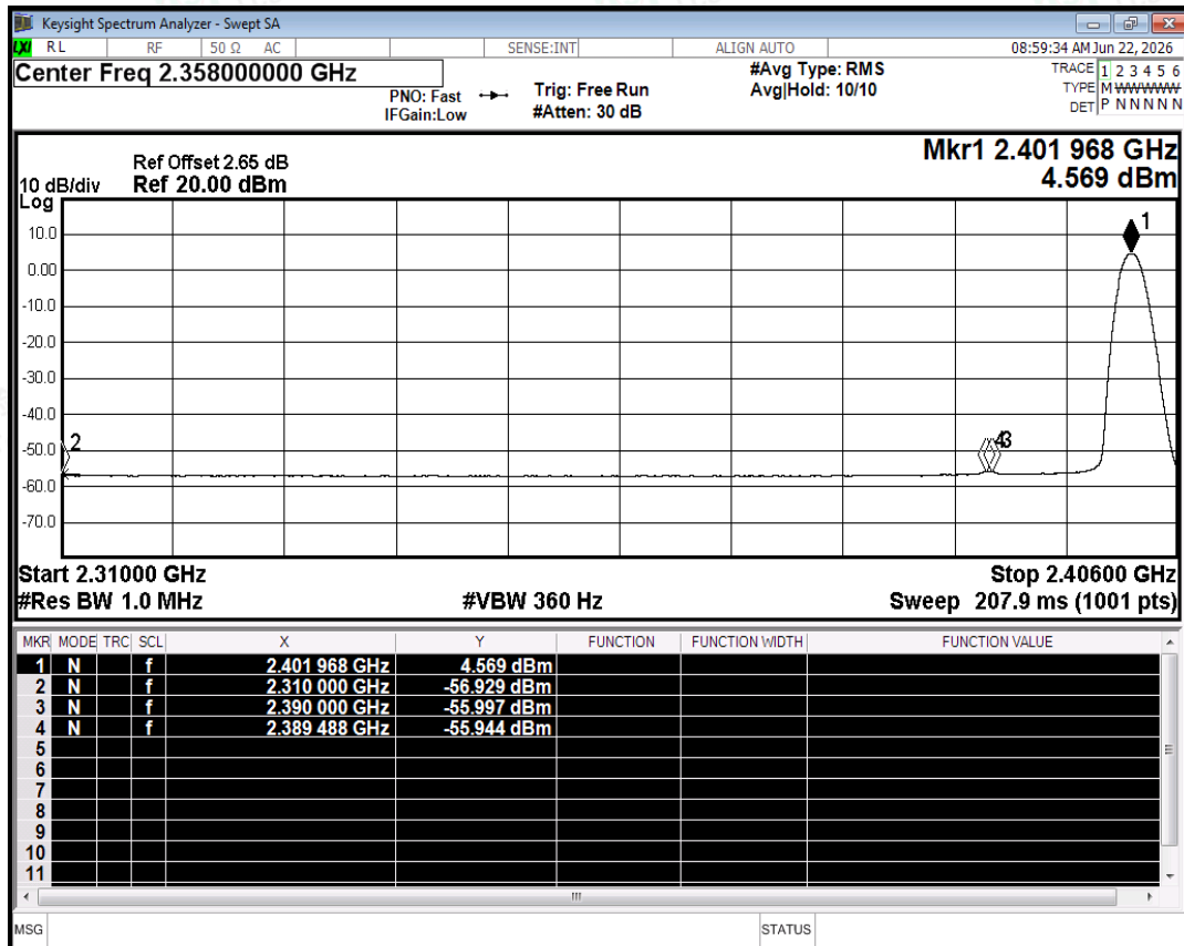
Restrict Band NVNT 3-DH5 2402MHz Ant2 No-Hopping Average
