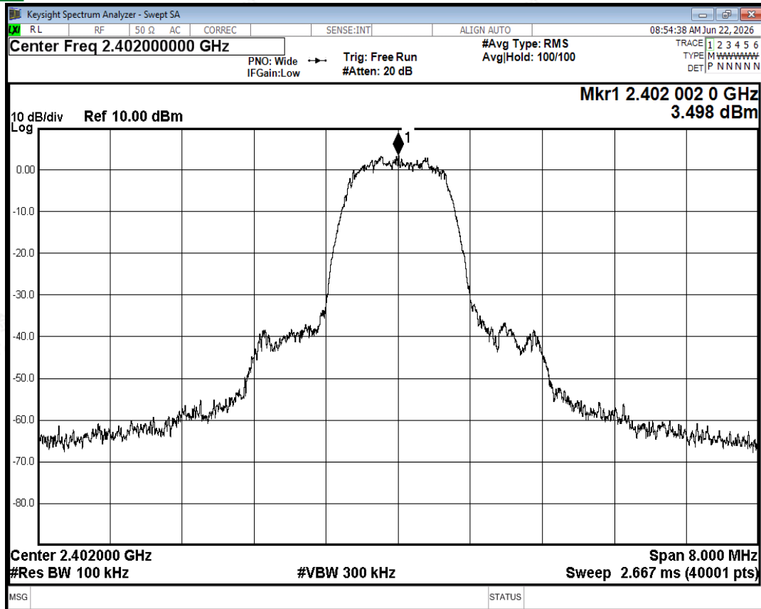
Tx. Spurious NVNT 2-DH5 2402MHz Ant2 Ref
