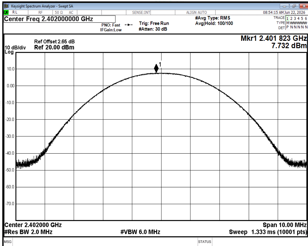
Peak Power NVNT 2-DH5 2402MHz Ant2
