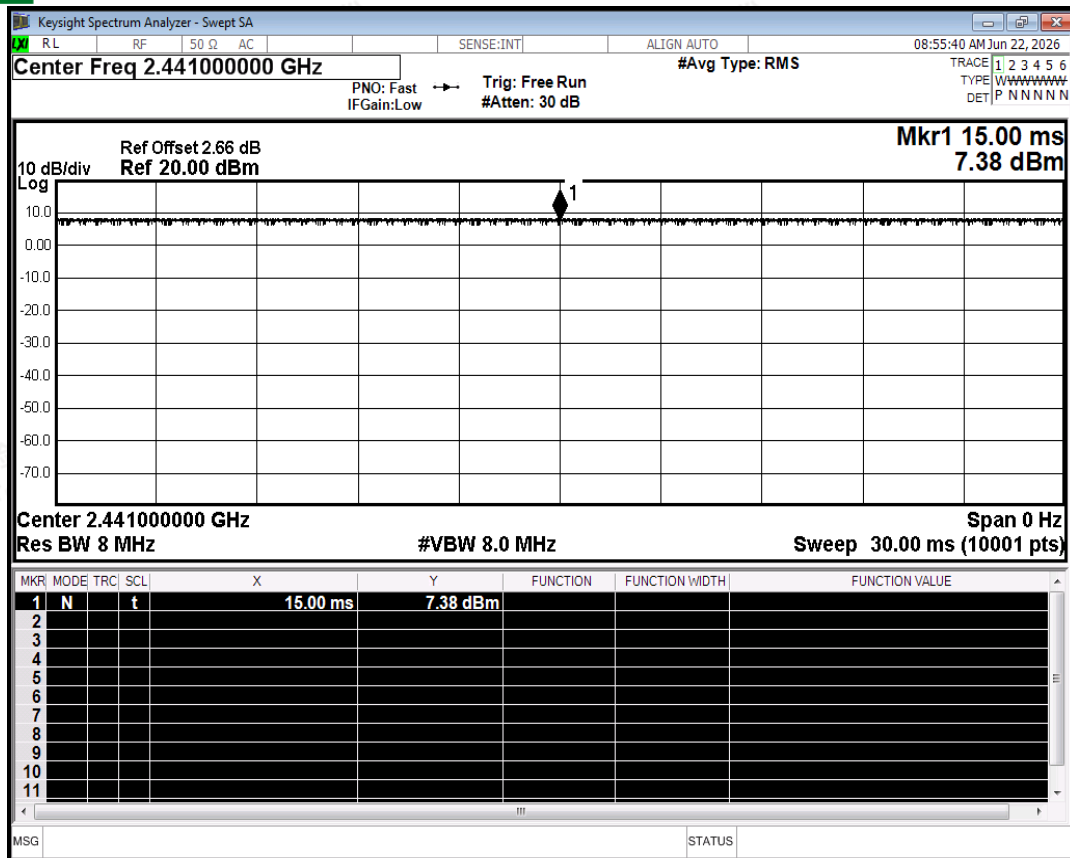
Duty Cycle NVNT 2-DH5 2441MHz Ant2
