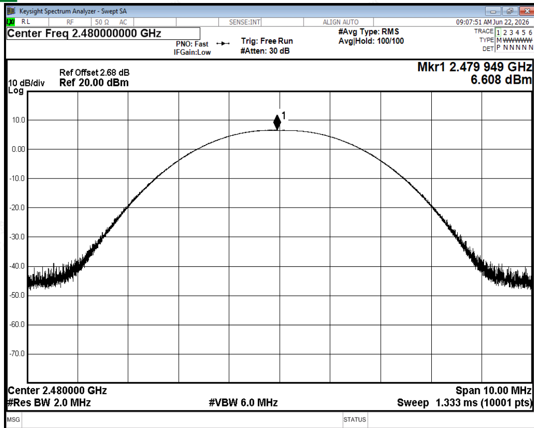
Peak Power NVNT 1-DH5 2480MHz Ant2
