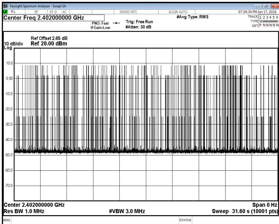
Dwell NVNT 2-DH5 2402MHz Ant2 Accumulated
