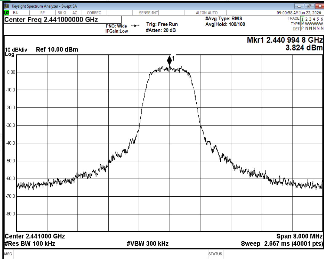
Tx. Spurious NVNT 3-DH5 2441MHz Ant2 Ref
