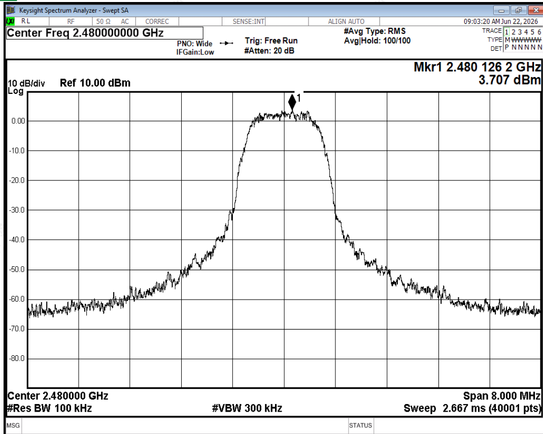
Tx. Spurious NVNT 3-DH5 2480MHz Ant2 Ref
