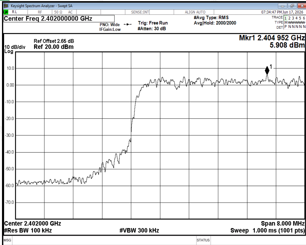
Band Edge(Hopping) NVNT 2-DH5 2402MHz Ant2 Hopping Ref
