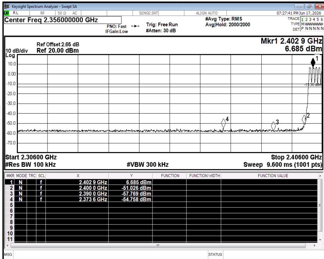
Band Edge(Hopping) NVNT 1-DH5 2402MHz Ant2 Hopping Emission
