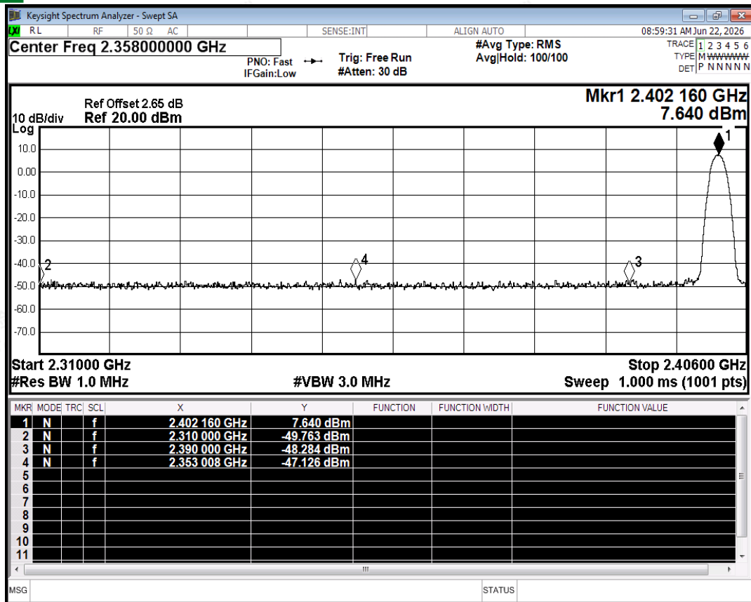
Restrict Band NVNT 3-DH5 2402MHz Ant2 No-Hopping Peak
