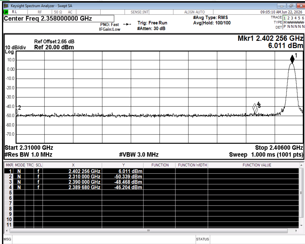
Restrict Band NVNT 1-DH5 2402MHz Ant2 No-Hopping Peak
