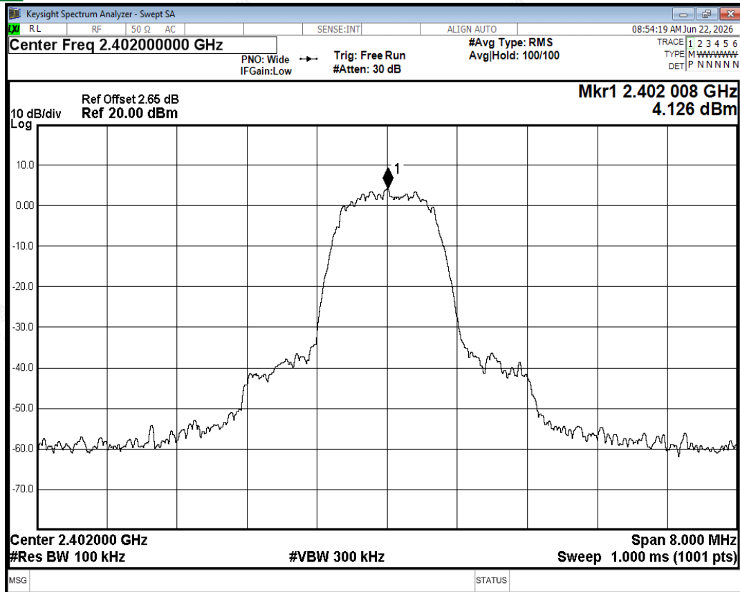
Band Edge NVNT 2-DH5 2402MHz Ant2 No-Hopping Ref
