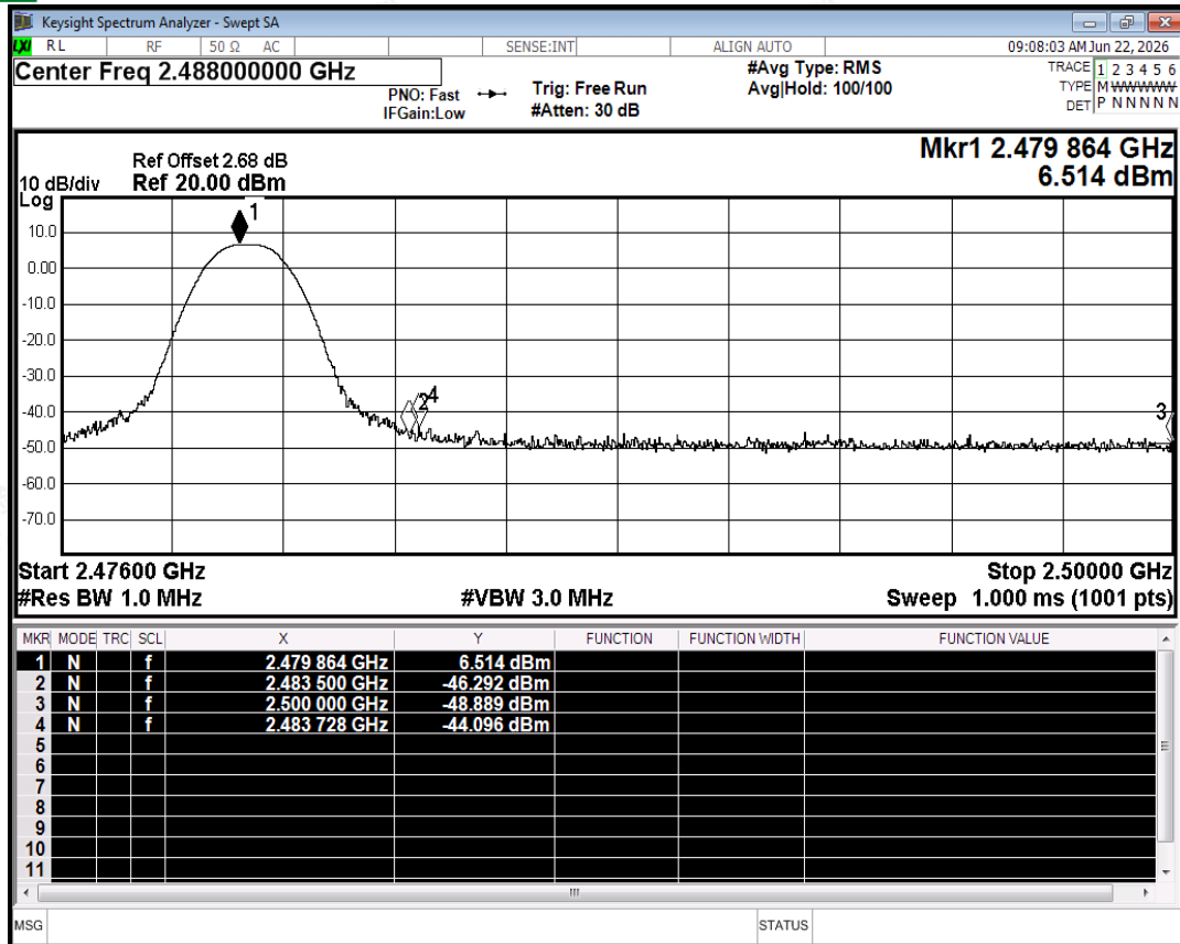
Restrict Band NVNT 1-DH5 2480MHz Ant2 No-Hopping Peak
