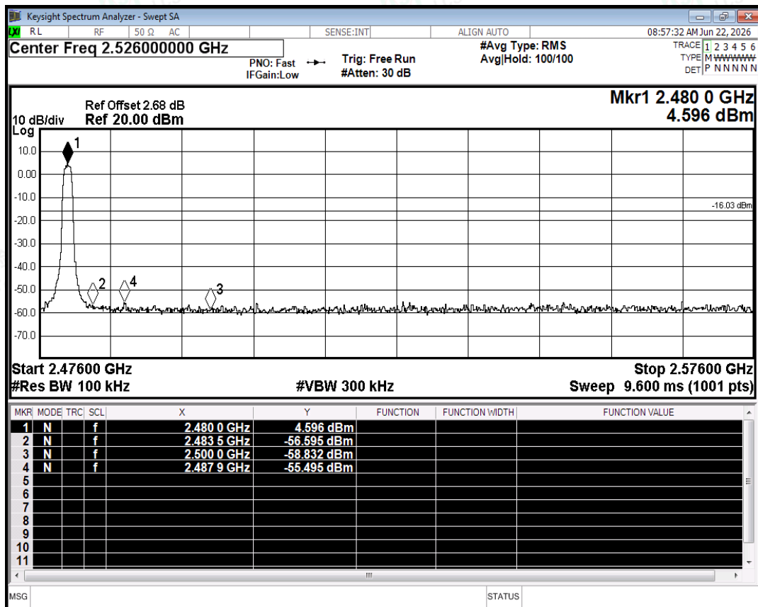
Band Edge NVNT 2-DH5 2480MHz Ant2 No-Hopping Emission
