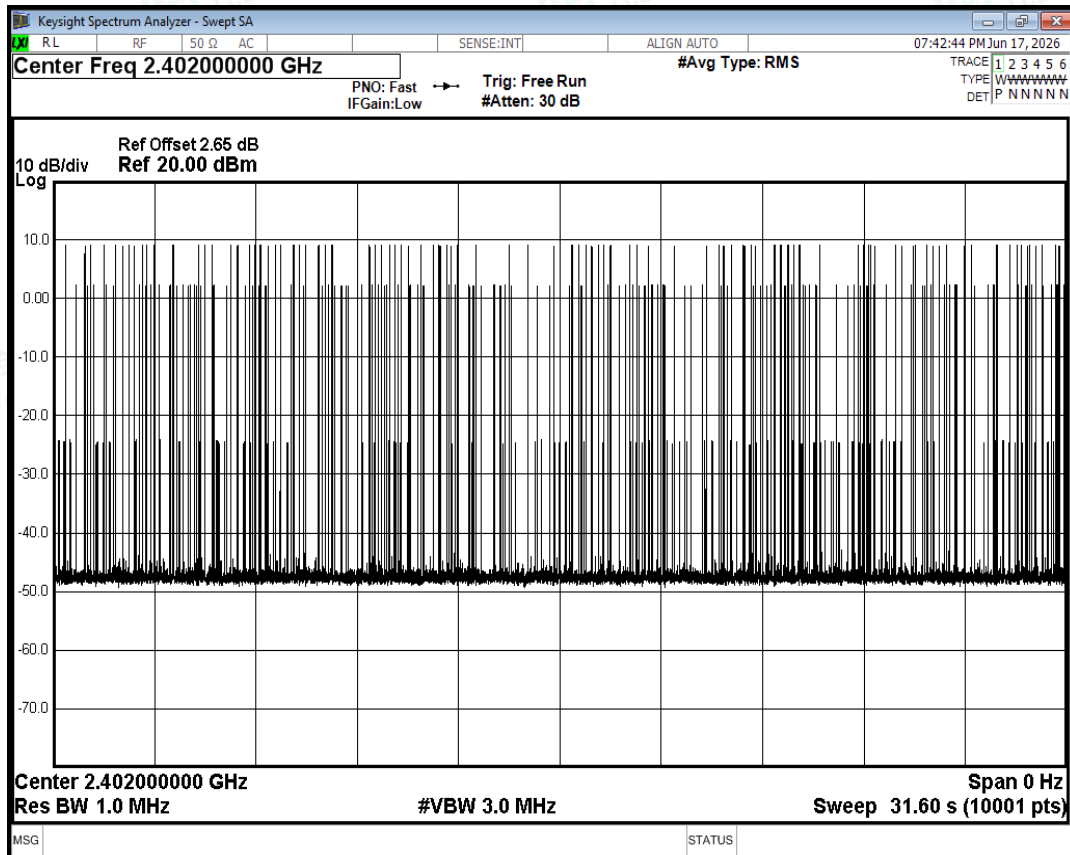
Dwell NVNT 3-DH5 2402MHz Ant2 Accumulated
