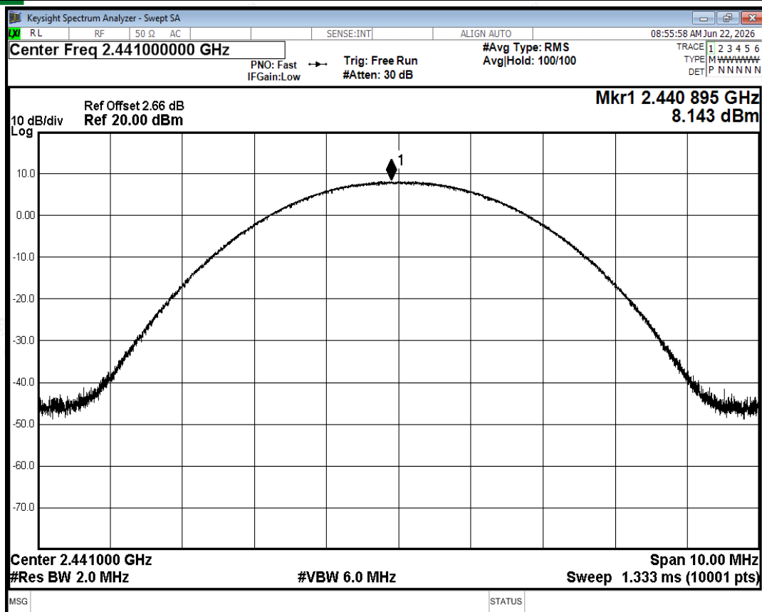
Peak Power NVNT 2-DH5 2441MHz Ant2
