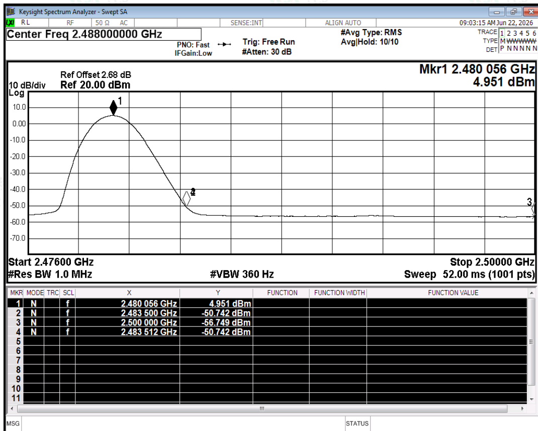
Restrict Band NVNT 3-DH5 2480MHz Ant2 No-Hopping Average
