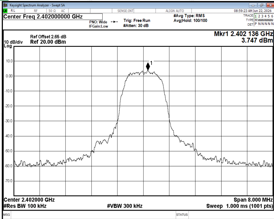
Band Edge NVNT 3-DH5 2402MHz Ant2 No-Hopping Ref
