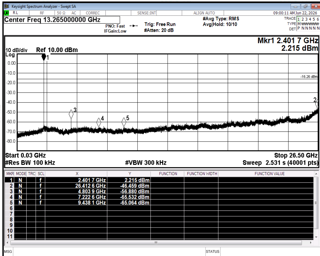
Tx. Spurious NVNT 3-DH5 2402MHz Ant2 Emission
