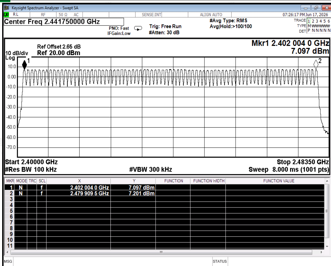
Hopping No. NVNT 1-DH5 2402MHz Ant2
