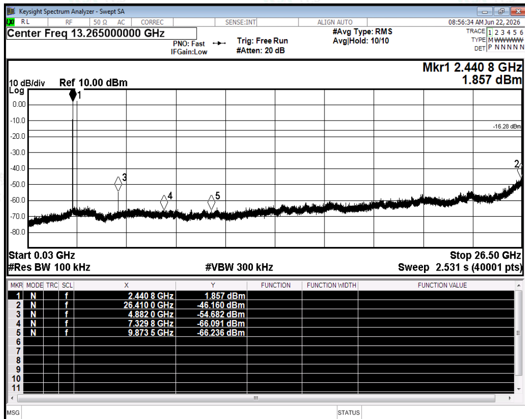
Tx. Spurious NVNT 2-DH5 2441MHz Ant2 Emission
