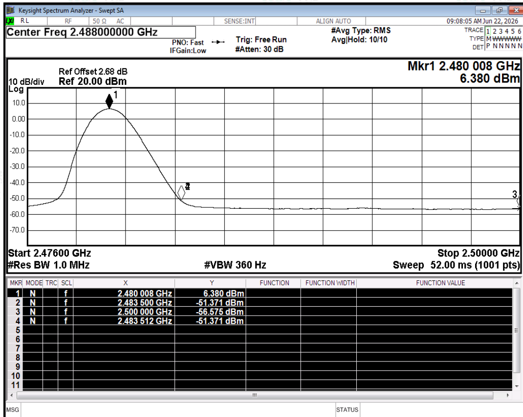
Restrict Band NVNT 1-DH5 2480MHz Ant2 No-Hopping Average
