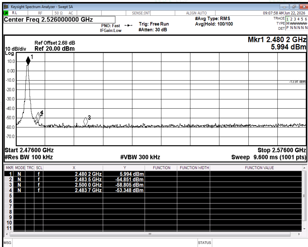
Band Edge NVNT 1-DH5 2480MHz Ant2 No-Hopping Emission
