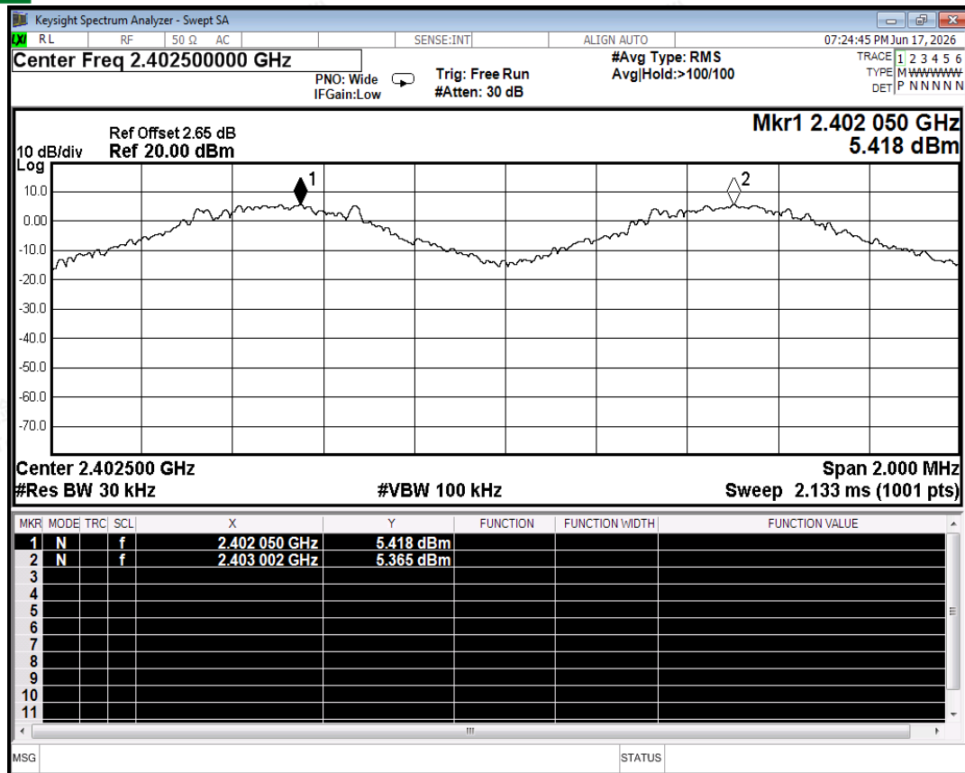
CFS NVNT 1-DH5 2402MHz Ant2
