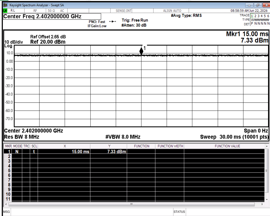
Duty Cycle NVNT 3-DH5 2402MHz Ant2
