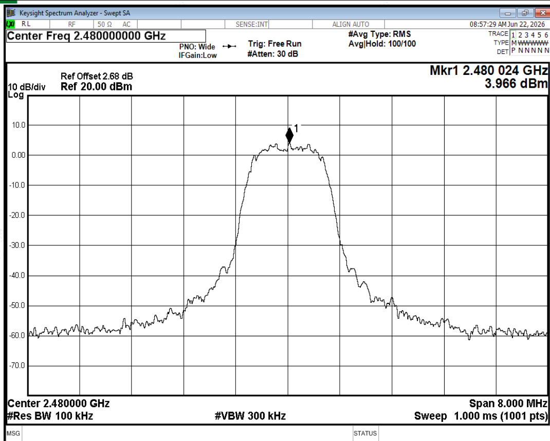
Band Edge NVNT 2-DH5 2480MHz Ant2 No-Hopping Ref
