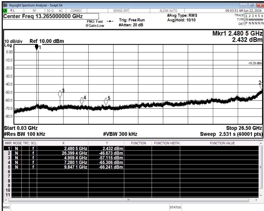
Tx. Spurious NVNT 3-DH5 2480MHz Ant2 Emission
