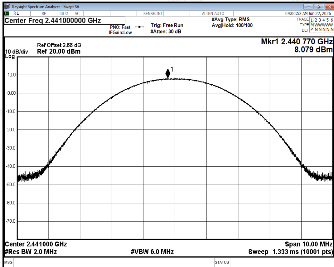
Peak Power NVNT 3-DH5 2441MHz Ant2
