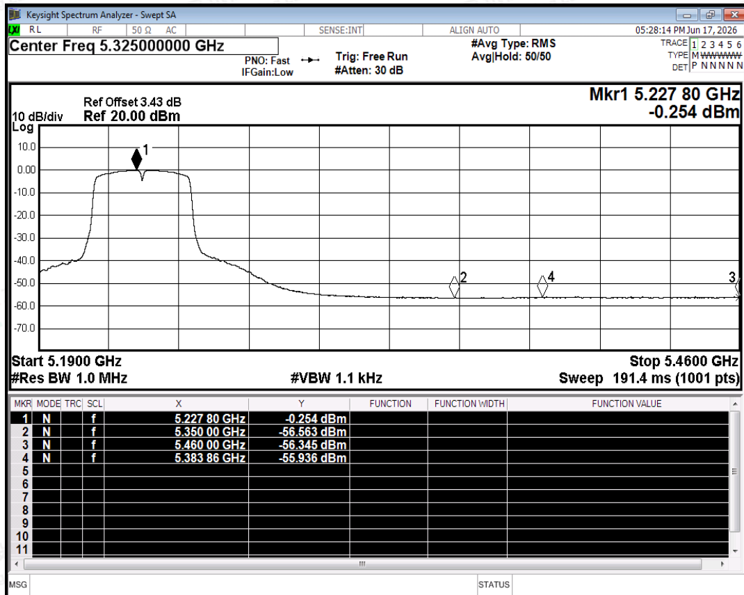
Restrict Band NVNT ac40 5230MHz Ant0 Average
