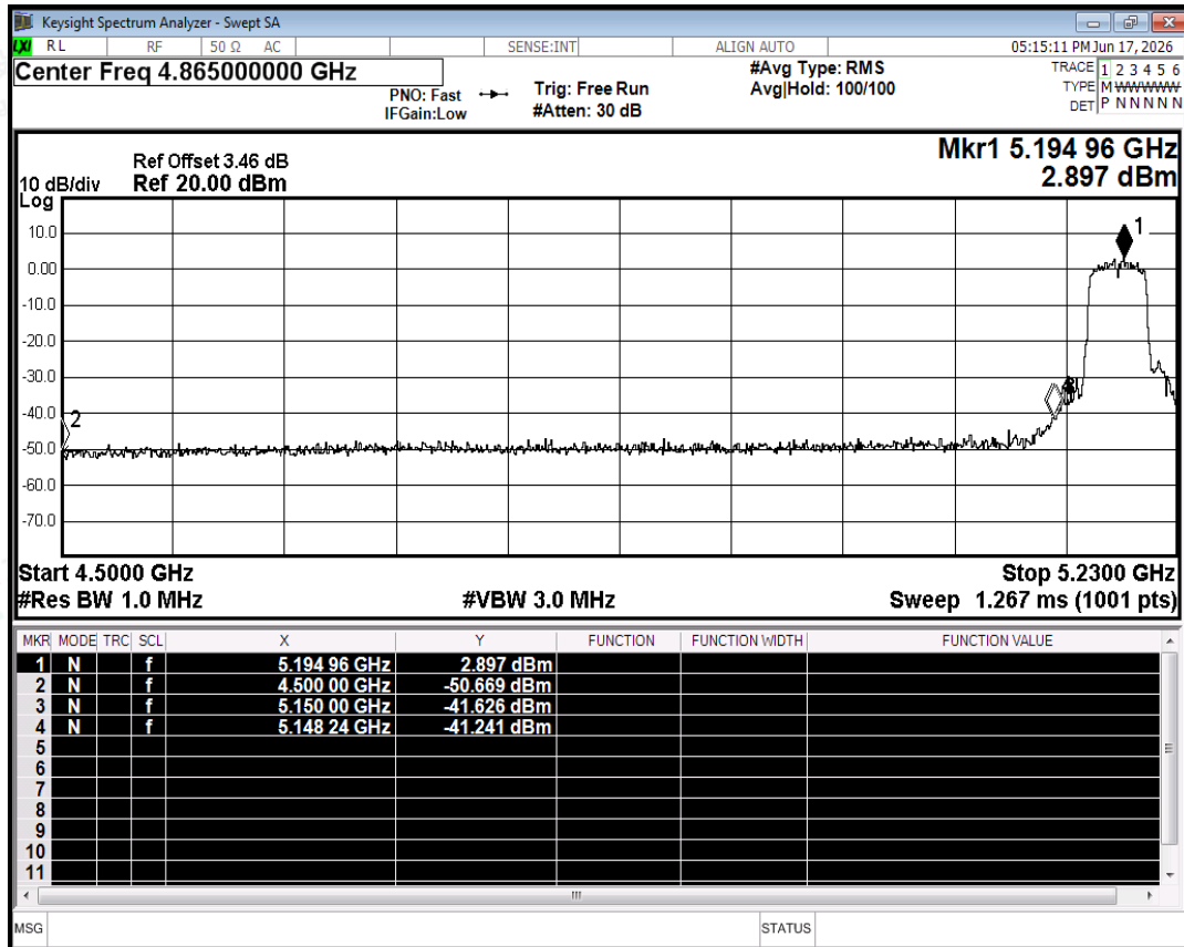
Restrict Band NVNT n40 5190MHz Ant0 Peak
