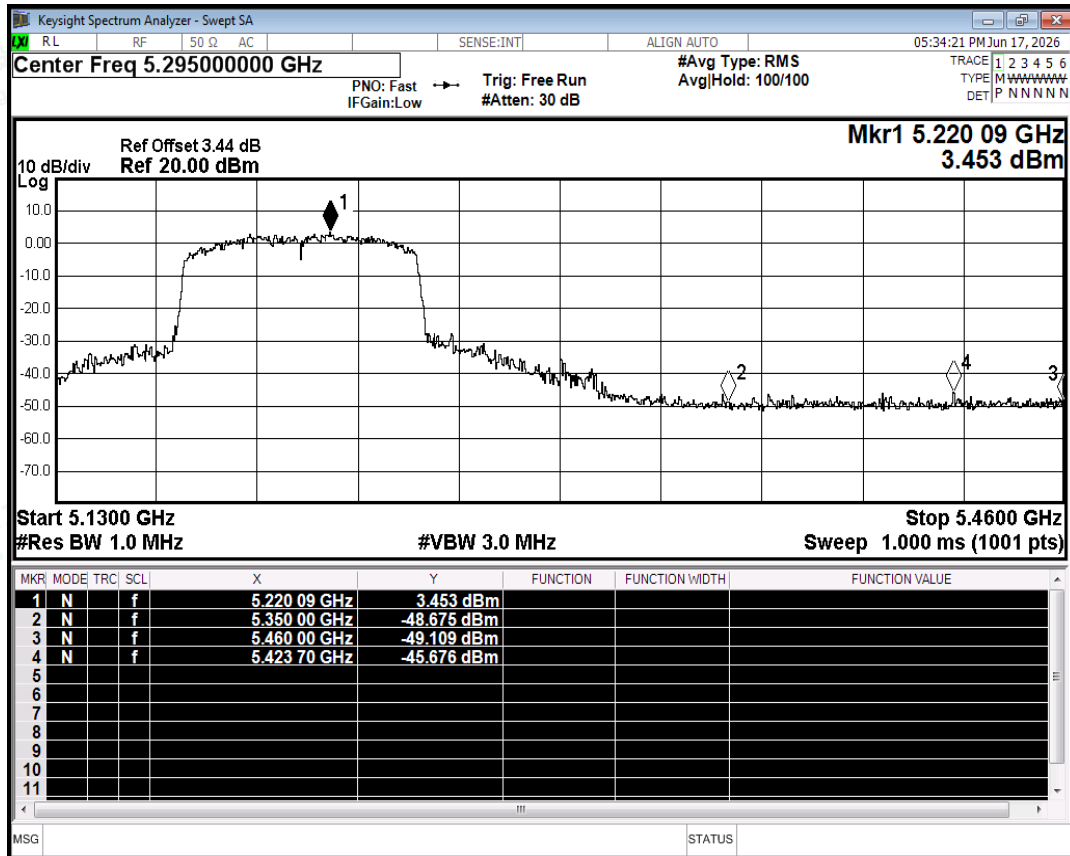
Restrict Band NVNT ac80 5210MHz Ant0 Peak
