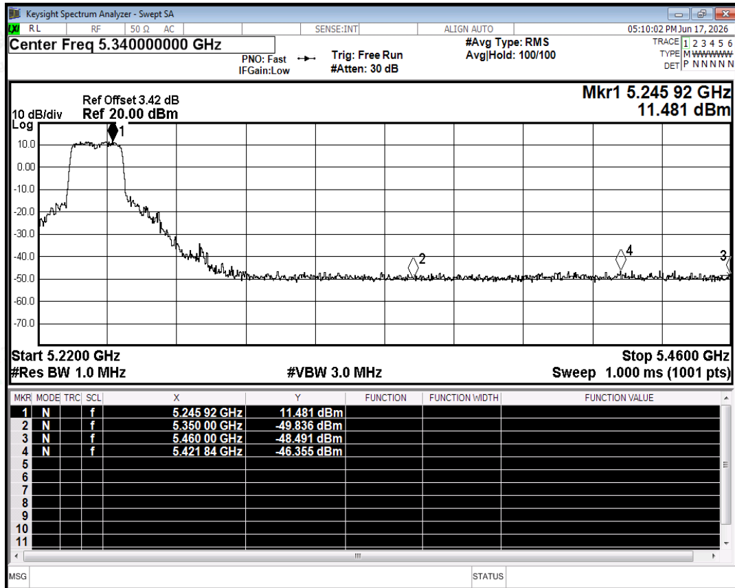
Restrict Band NVNT ac20 5240MHz Ant0 Peak
