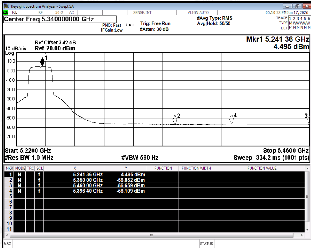
Restrict Band NVNT ac20 5240MHz Ant0 Average
