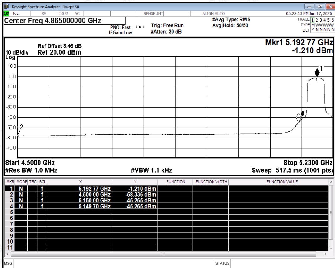
Restrict Band NVNT ac40 5190MHz Ant0 Average
