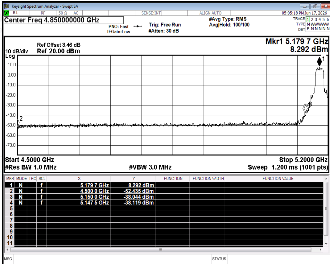
Restrict Band NVNT ac20 5180MHz Ant0 Peak
