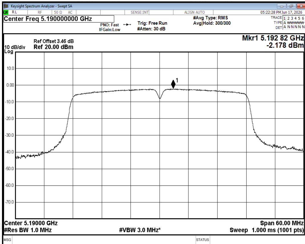
PSD NVNT ac40 5190MHz Ant0
