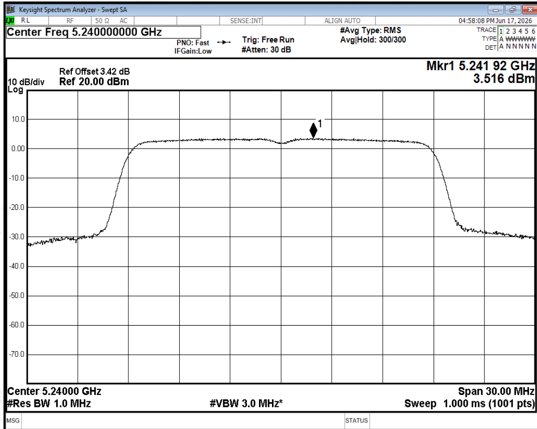
PSD NVNT n20 5240MHz Ant0
