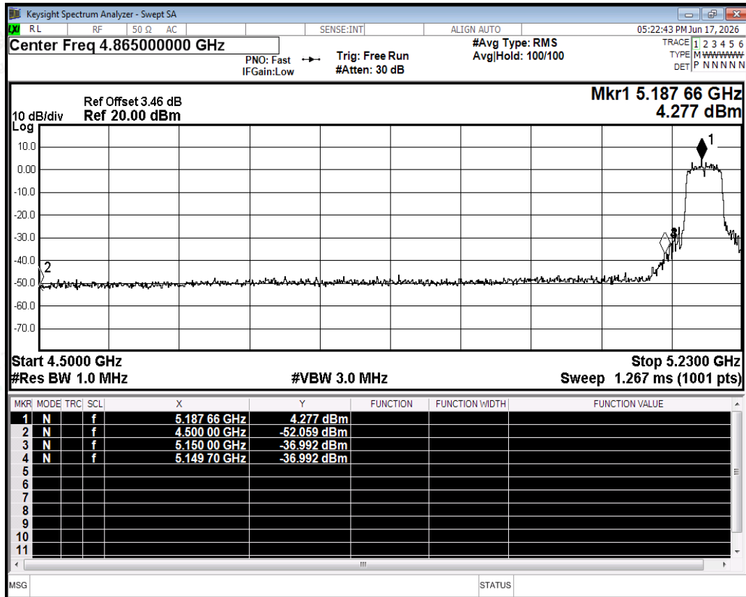
Restrict Band NVNT ac40 5190MHz Ant0 Peak
