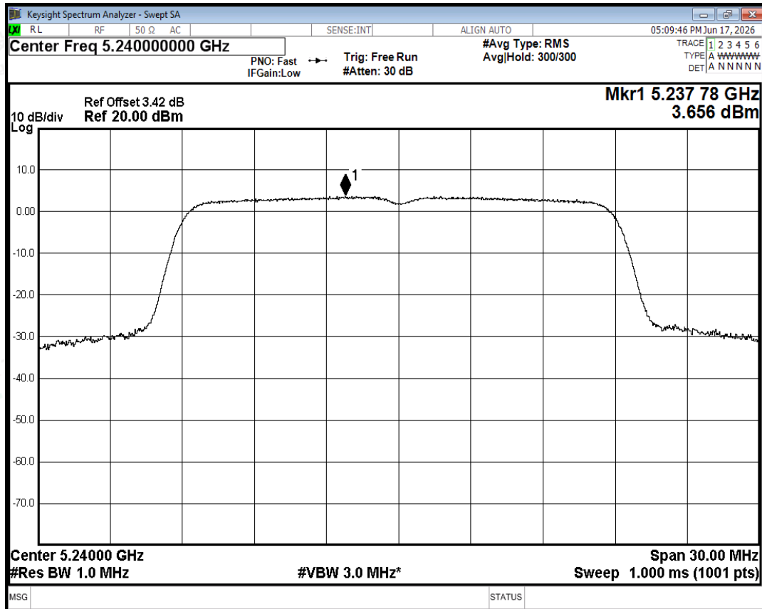
PSD NVNT ac20 5240MHz Ant0
