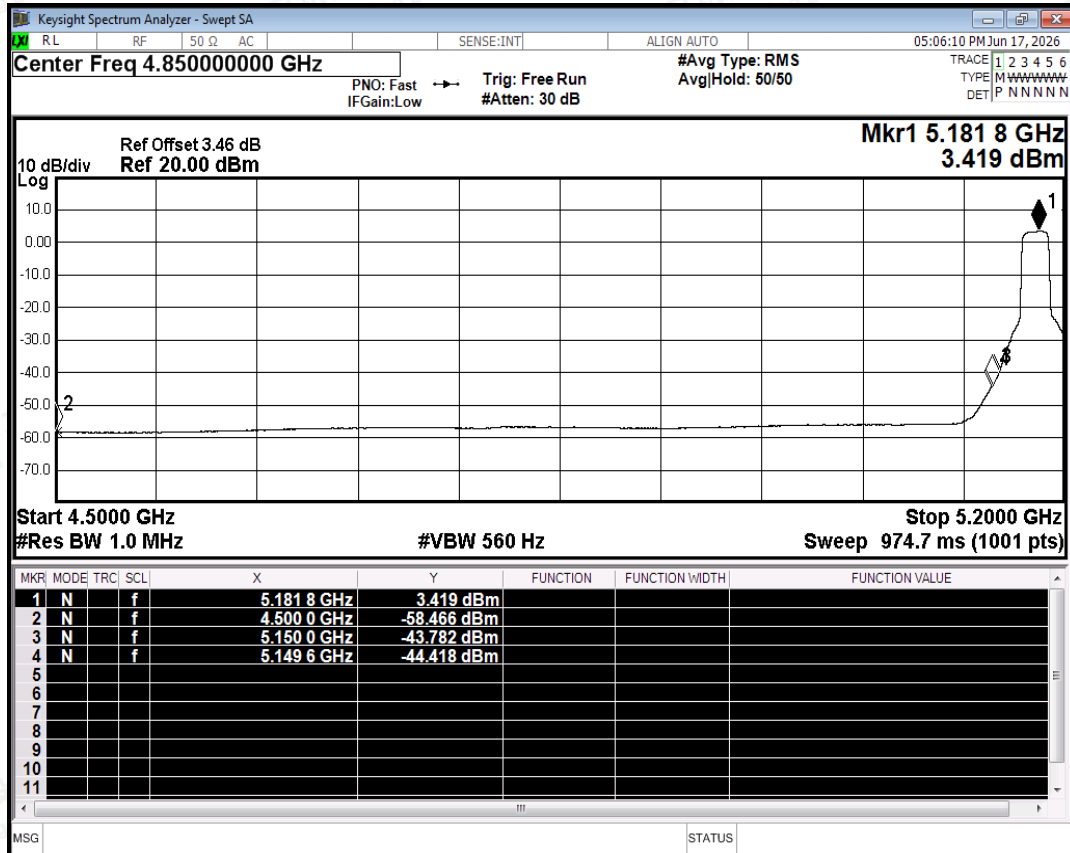
Restrict Band NVNT ac20 5180MHz Ant0 Average
