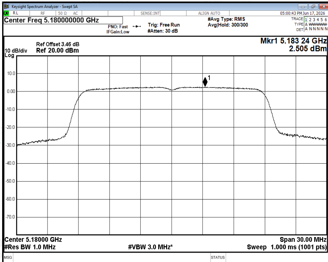
PSD NVNT n20 5180MHz Ant0
