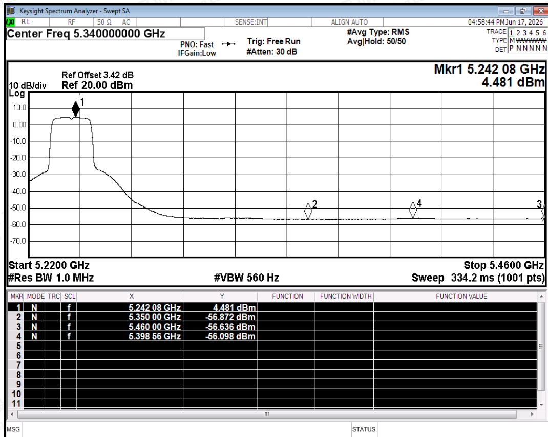
Restrict Band NVNT n20 5240MHz Ant0 Average
