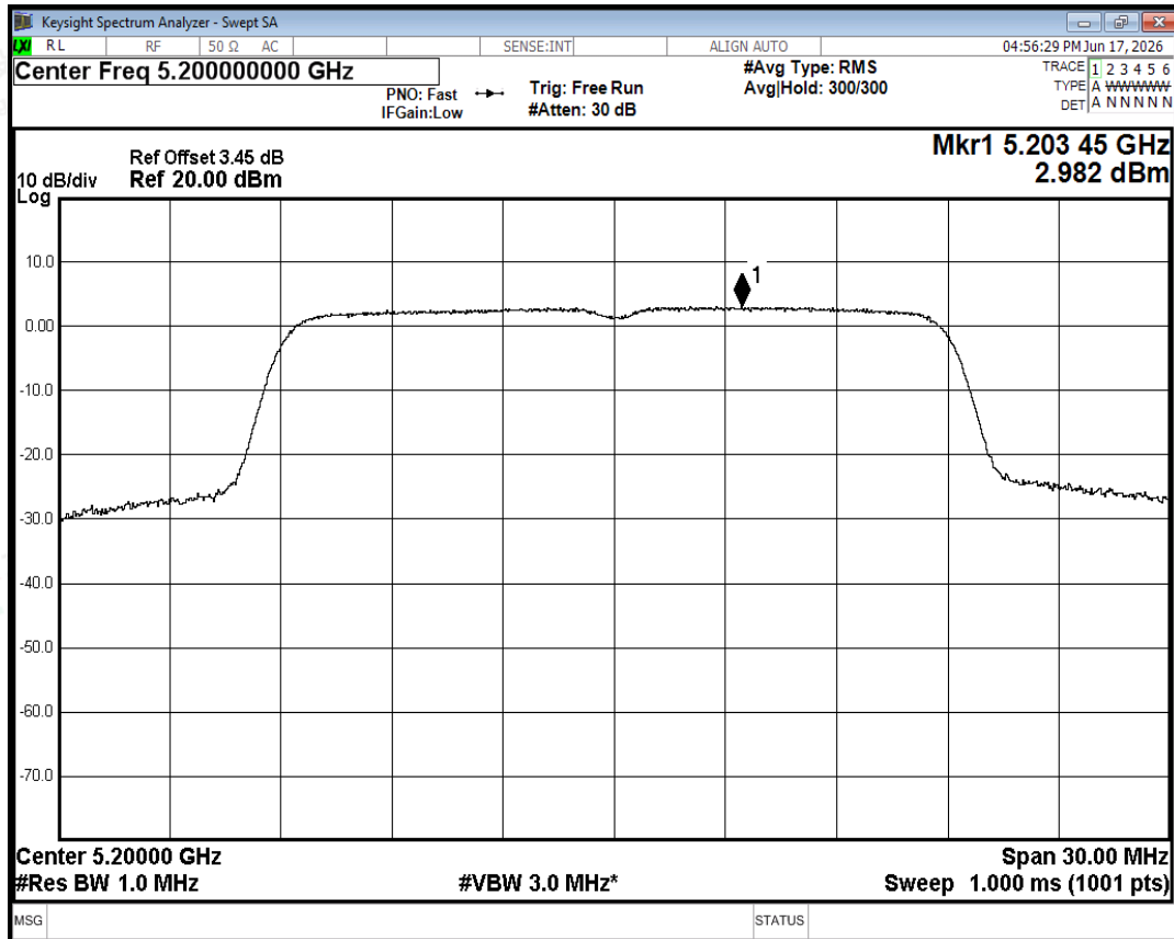
PSD NVNT n20 5200MHz Ant0
