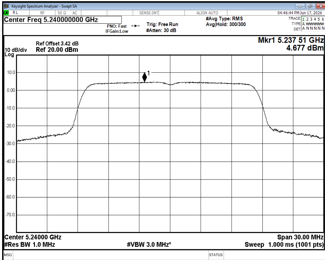
PSD NVNT a 5240MHz Ant0
