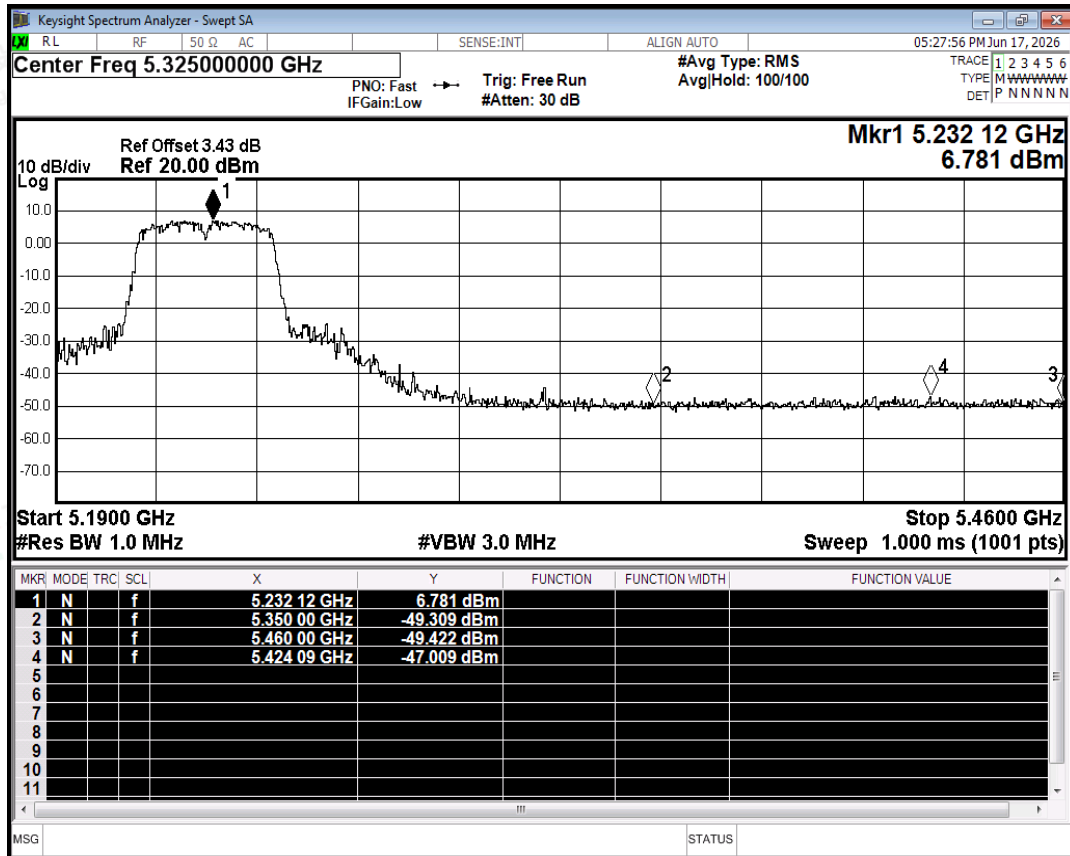
Restrict Band NVNT ac40 5230MHz Ant0 Peak
