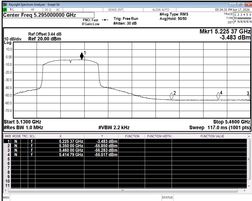
Restrict Band NVNT ac80 5210MHz Ant0 Average
