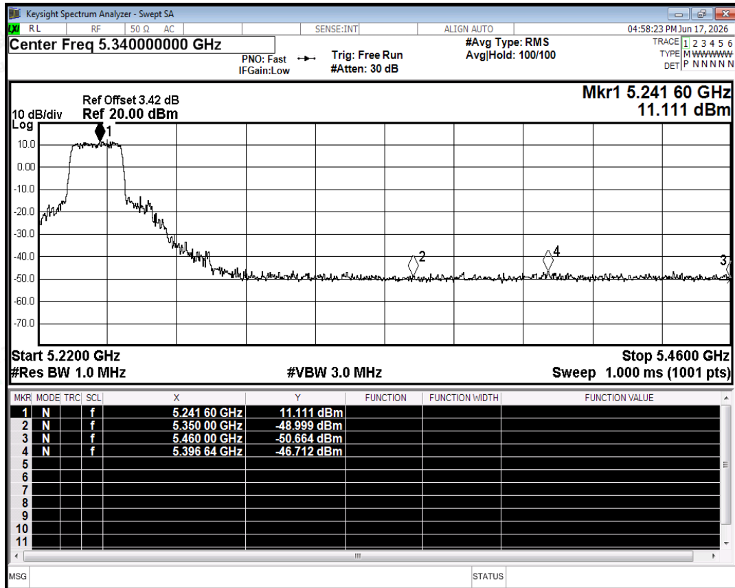
Restrict Band NVNT n20 5240MHz Ant0 Peak
