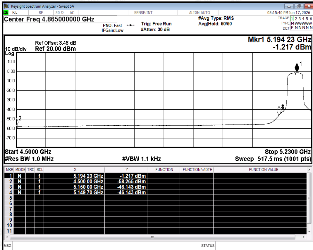
Restrict Band NVNT n40 5190MHz Ant0 Average
