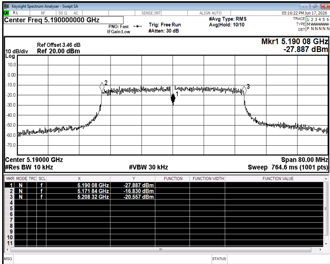
Freq. Stability NVNT n40 5190MHz Ant0
