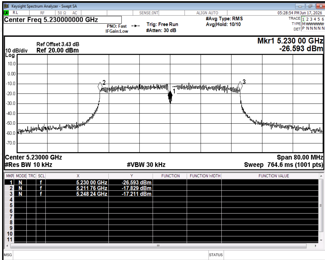
Freq. Stability NVNT ac40 5230MHz Ant0
