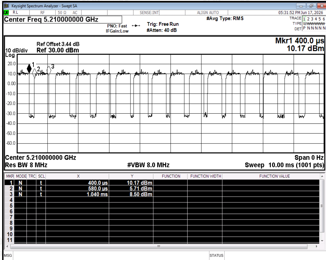
Duty Cycle NVNT ac80 5210MHz Ant0
