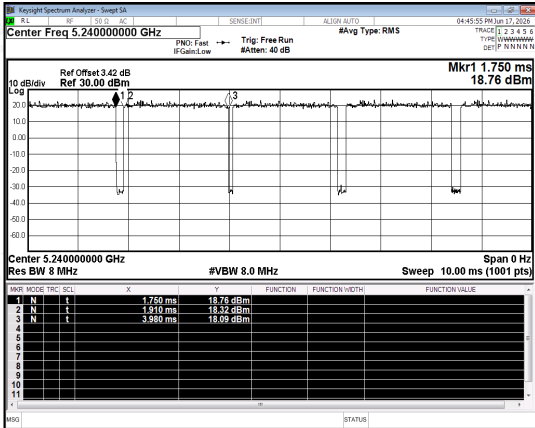
Duty Cycle NVNT a 5240MHz Ant0
