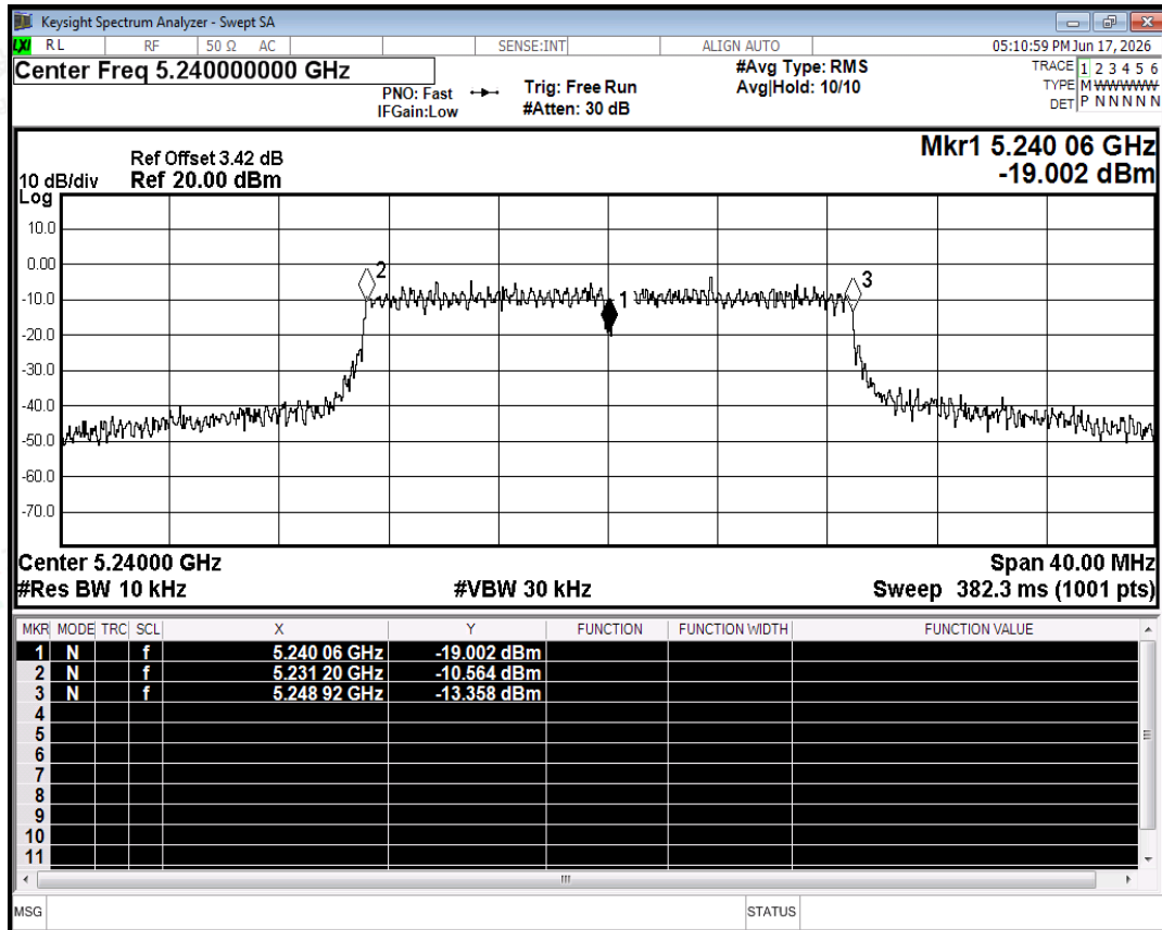
Freq. Stability NVNT ac20 5240MHz Ant0
