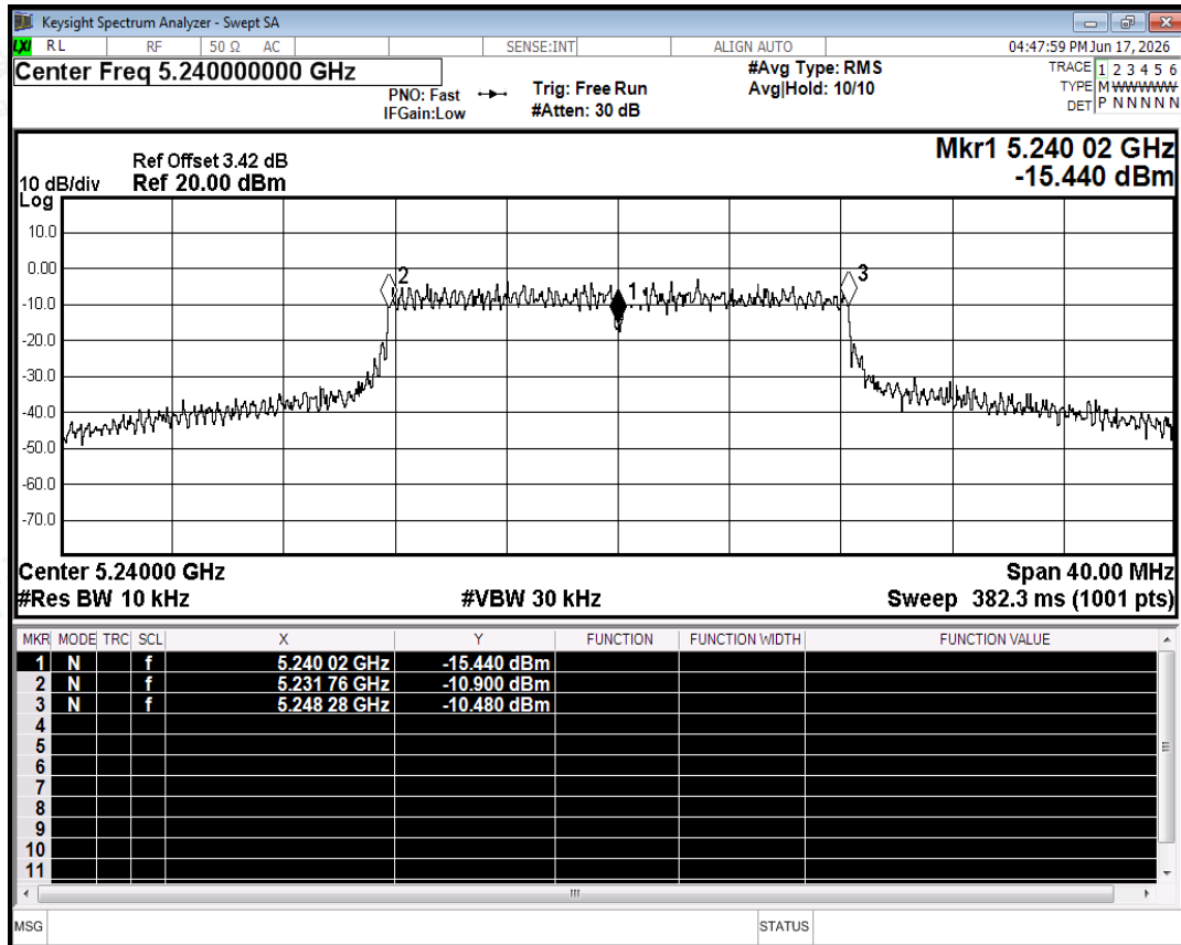
Freq. Stability NVNT a 5240MHz Ant0
