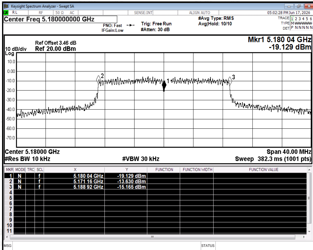
Freq. Stability NVNT n20 5180MHz Ant0
