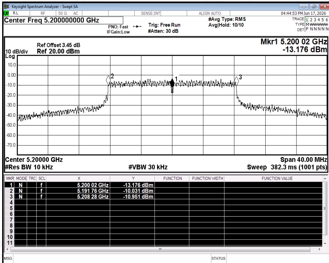
Freq. Stability NVNT a 5200MHz Ant0
