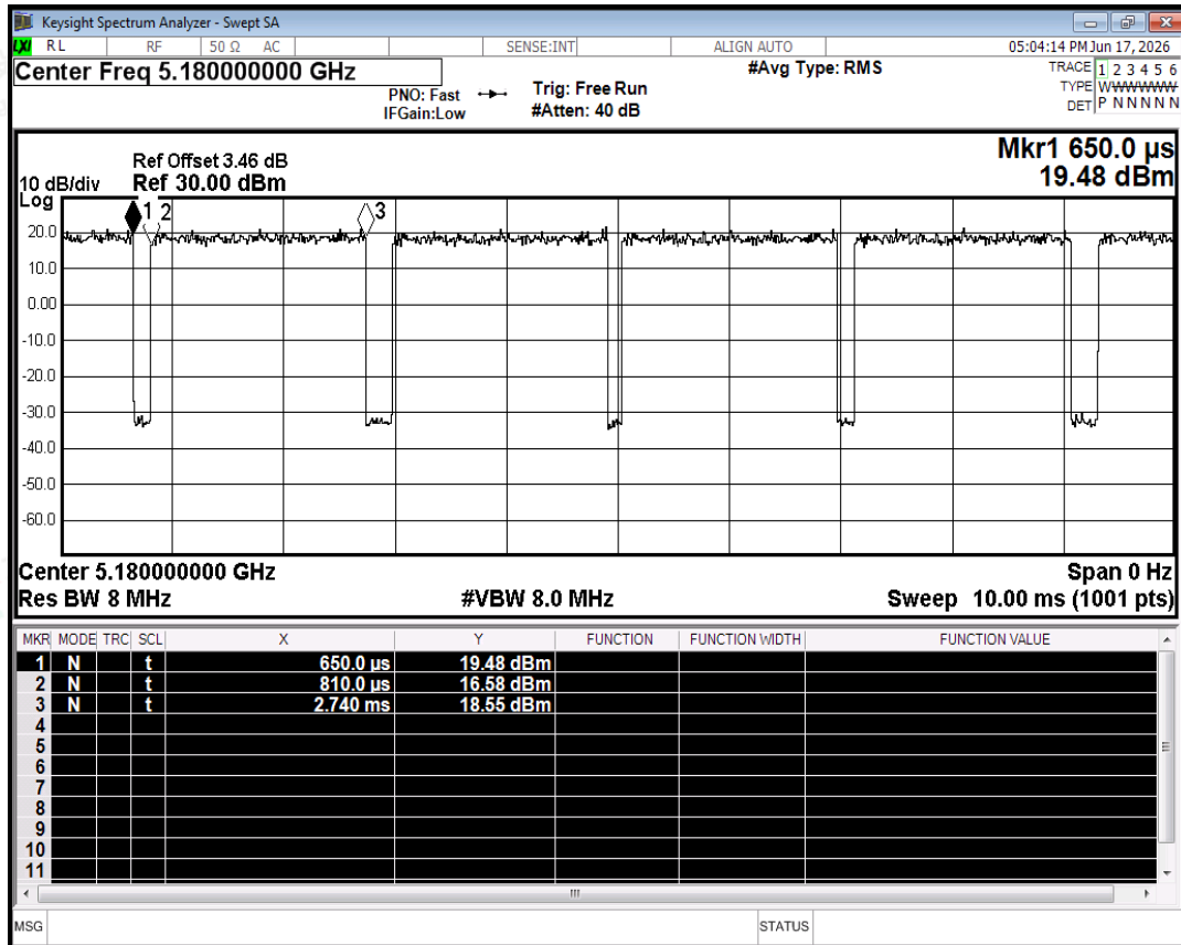
Duty Cycle NVNT ac20 5180MHz Ant0
