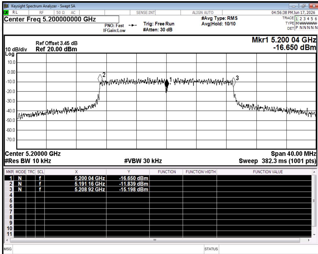
Freq. Stability NVNT n20 5200MHz Ant0
