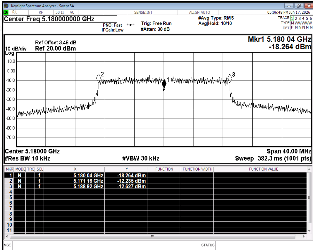
Freq. Stability NVNT ac20 5180MHz Ant0
