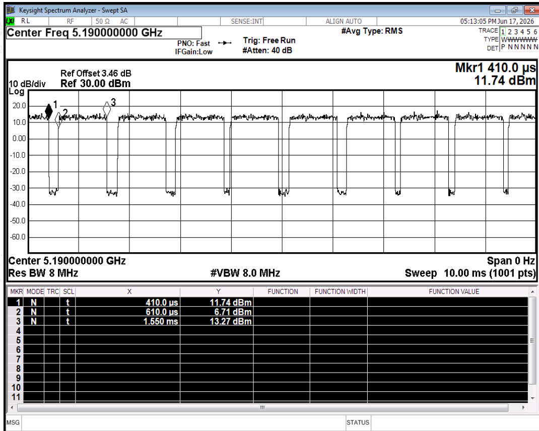
Duty Cycle NVNT n40 5190MHz Ant0
