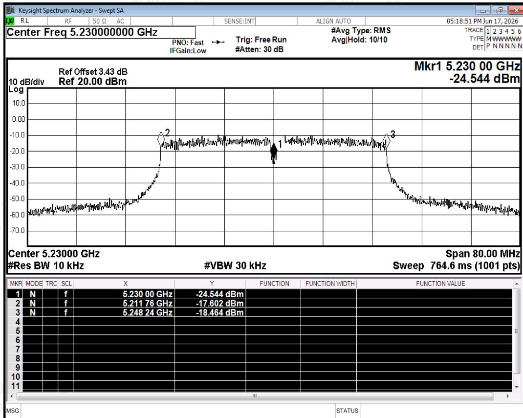
Freq. Stability NVNT n40 5230MHz Ant0
