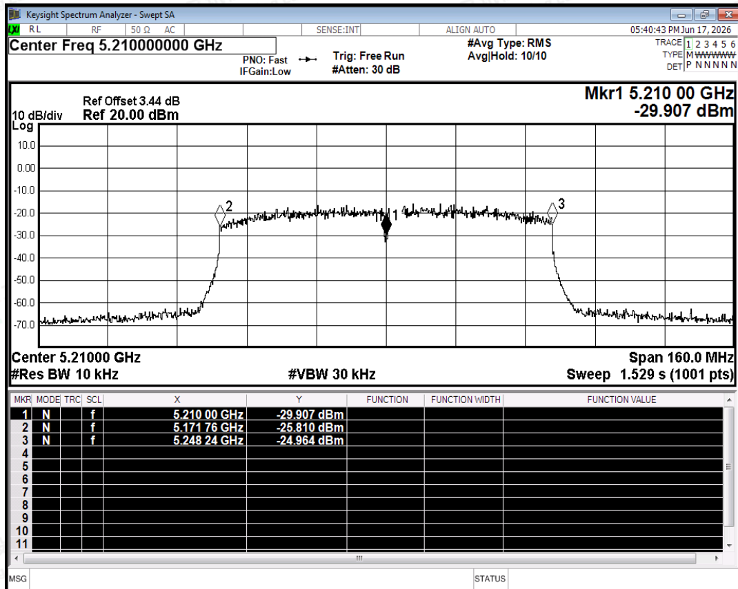
Freq. Stability NVNT ac80 5210MHz Ant0
