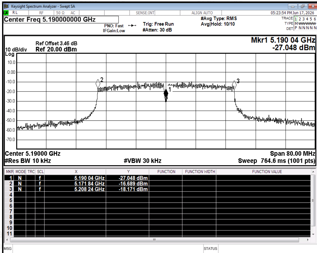
Freq. Stability NVNT ac40 5190MHz Ant0
