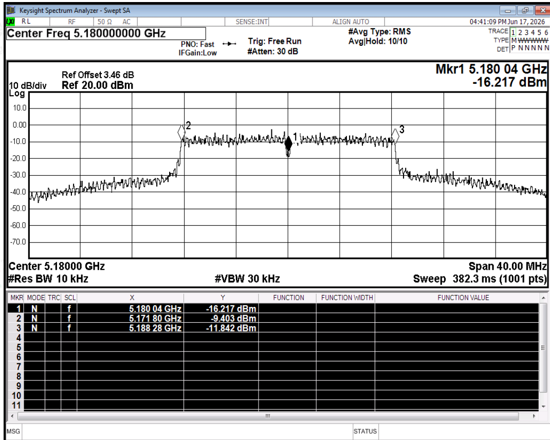
Freq. Stability NVNT a 5180MHz Ant0
