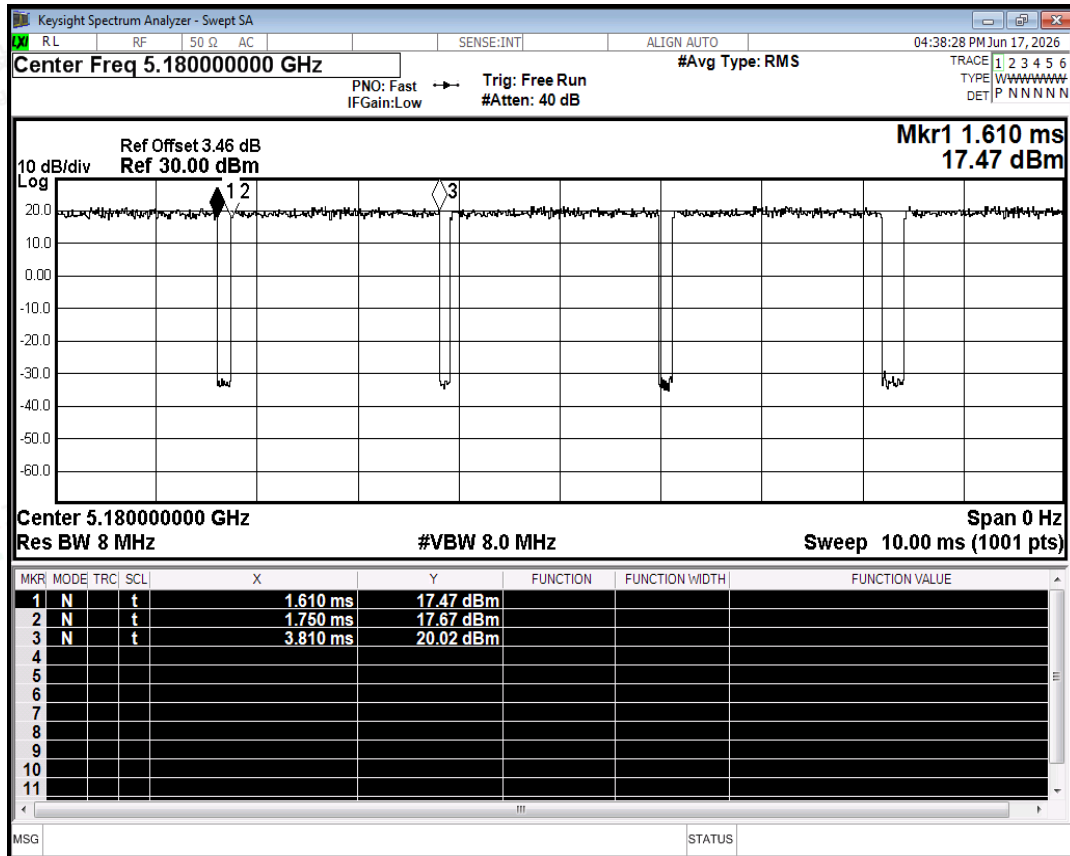
Duty Cycle NVNT a 5180MHz Ant0
