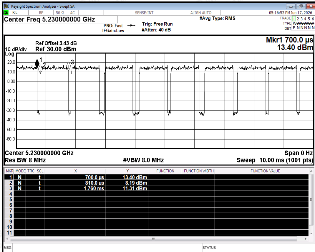
Duty Cycle NVNT n40 5230MHz Ant0
