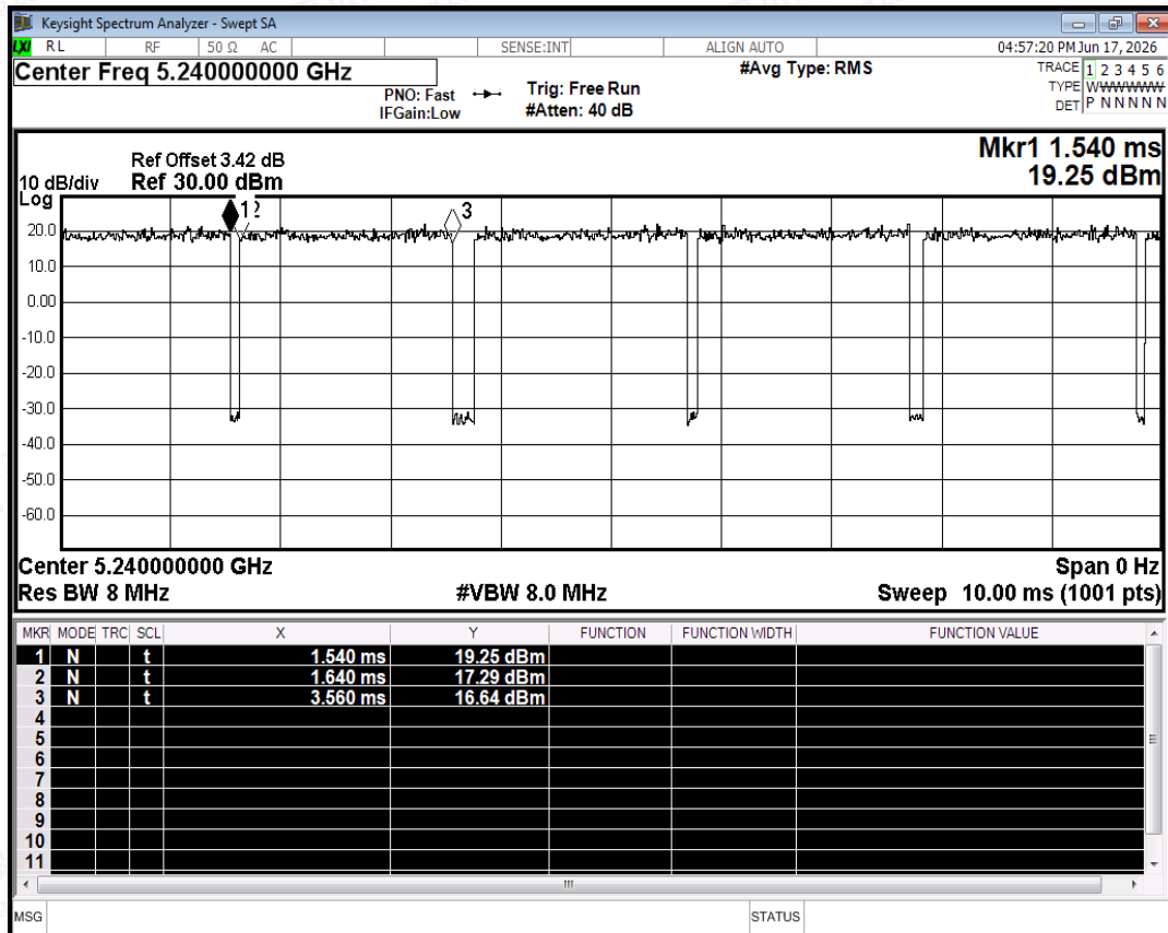
Duty Cycle NVNT n20 5240MHz Ant0
