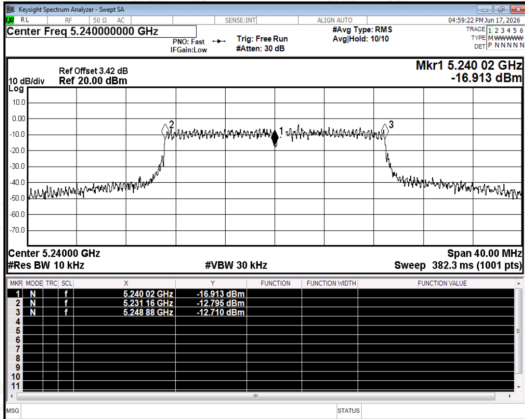
Freq. Stability NVNT n20 5240MHz Ant0
