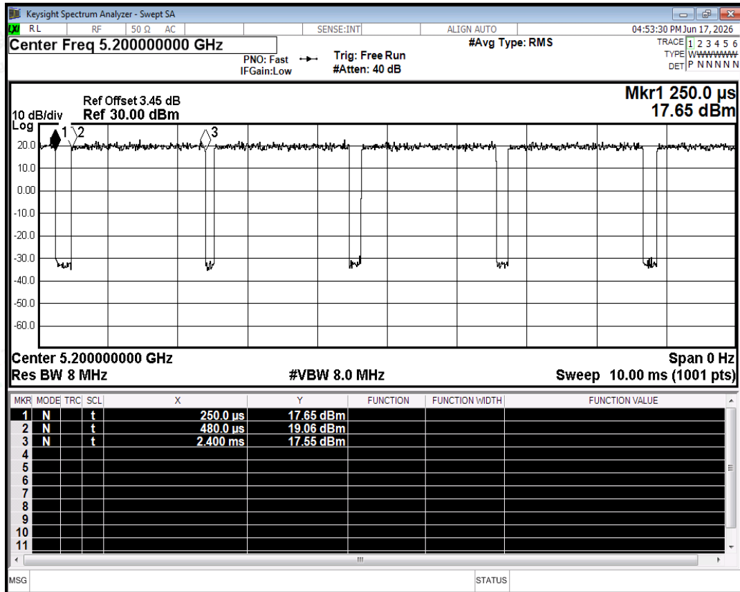
Duty Cycle NVNT n20 5200MHz Ant0
