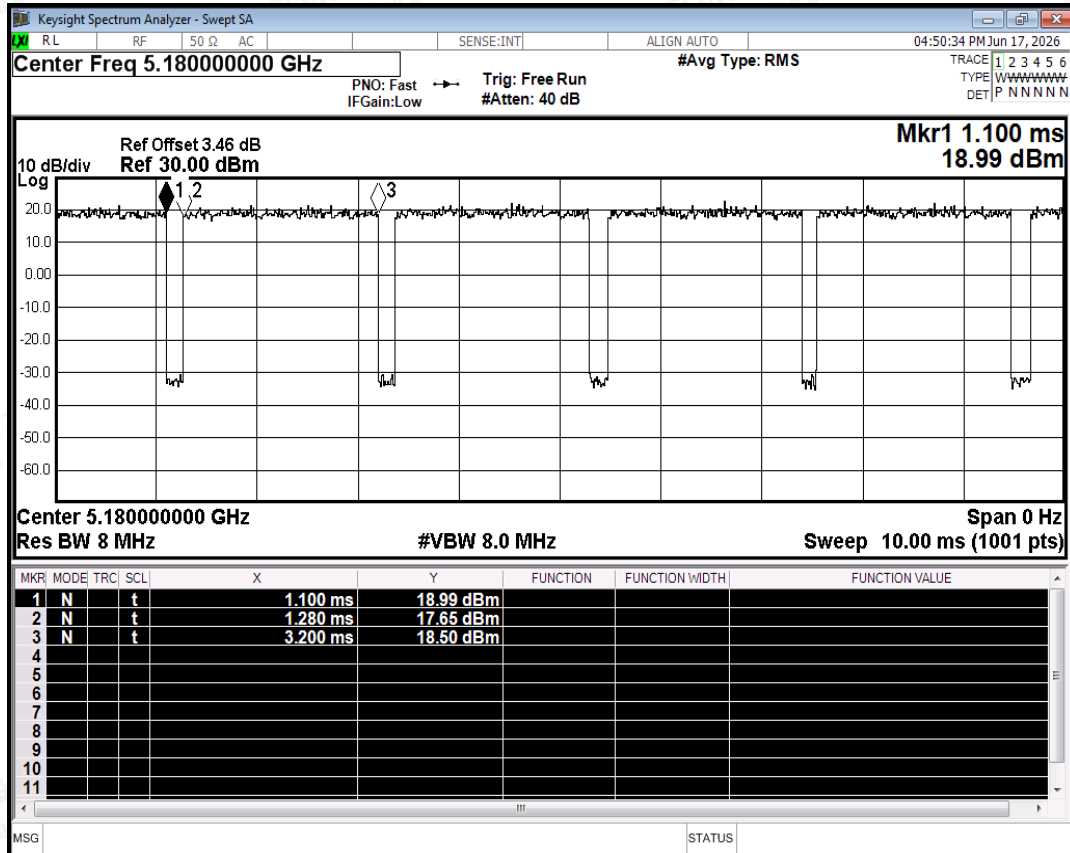
Duty Cycle NVNT n20 5180MHz Ant0
