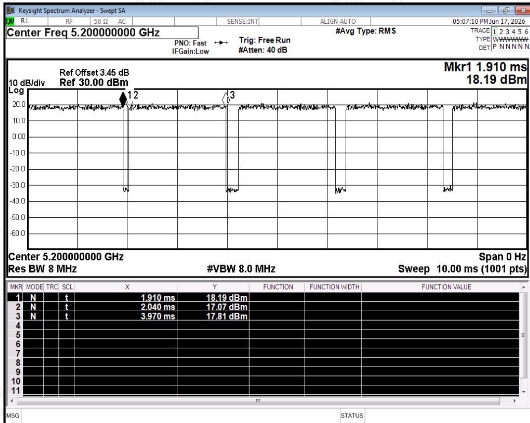
Duty Cycle NVNT ac20 5200MHz Ant0
