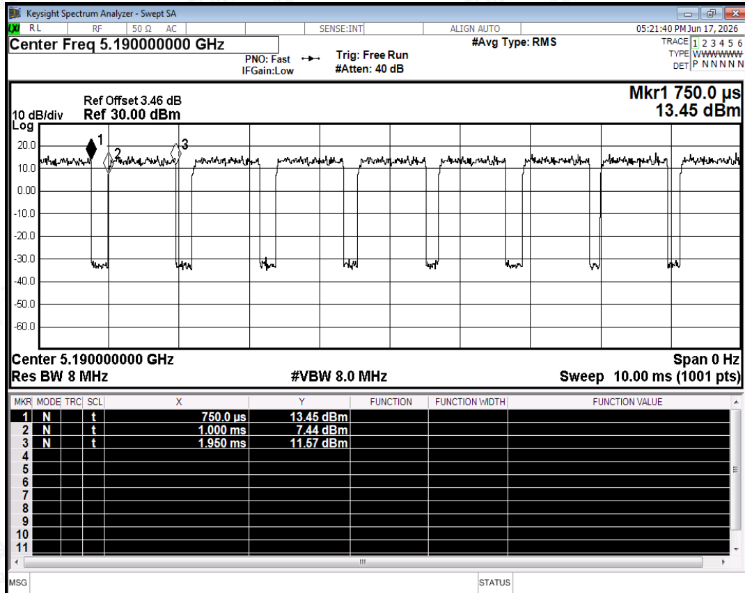
Duty Cycle NVNT ac40 5190MHz Ant0
