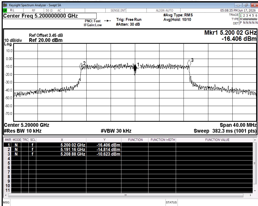
Freq. Stability NVNT ac20 5200MHz Ant0
