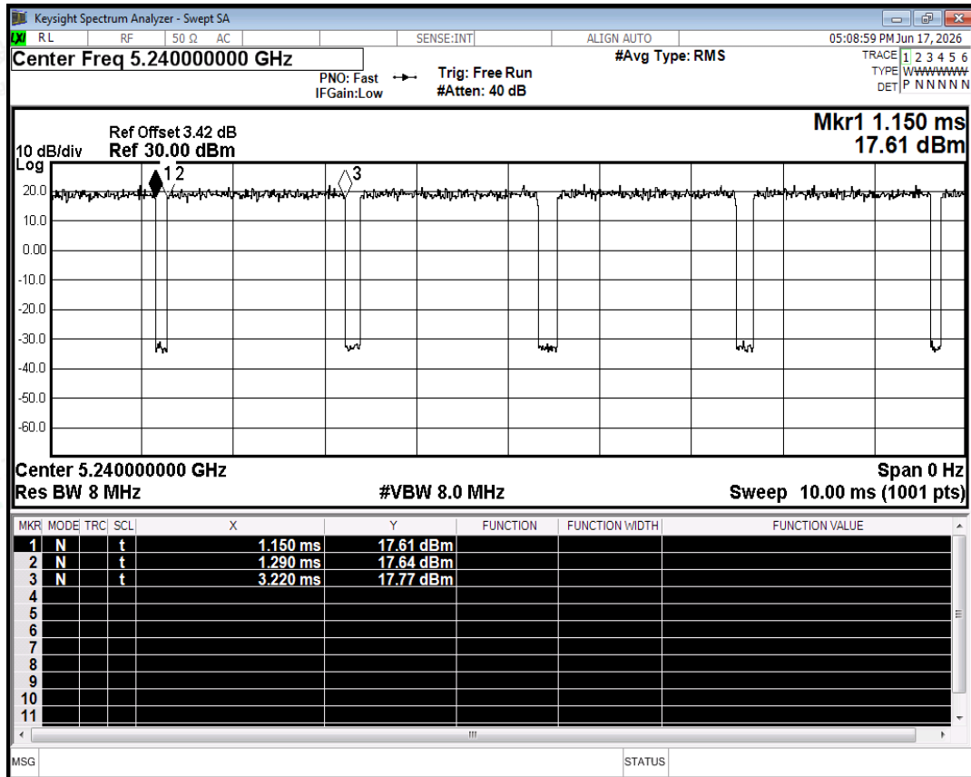
Duty Cycle NVNT ac20 5240MHz Ant0
