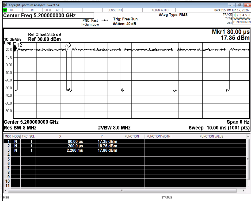
Duty Cycle NVNT a 5200MHz Ant0
