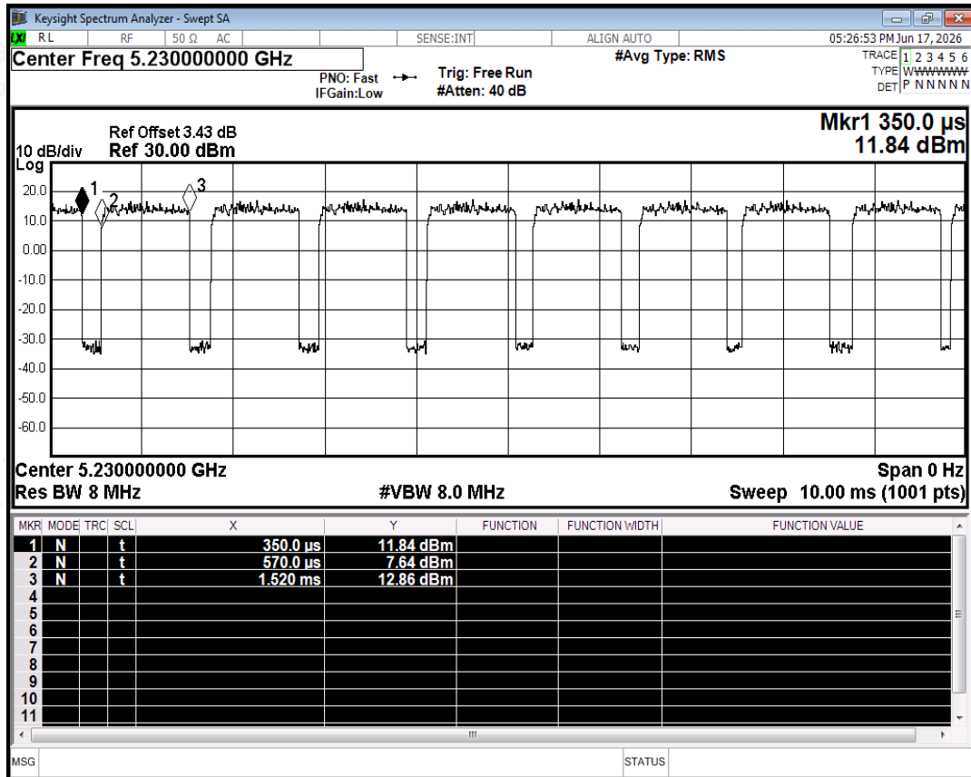
Duty Cycle NVNT ac40 5230MHz Ant0
