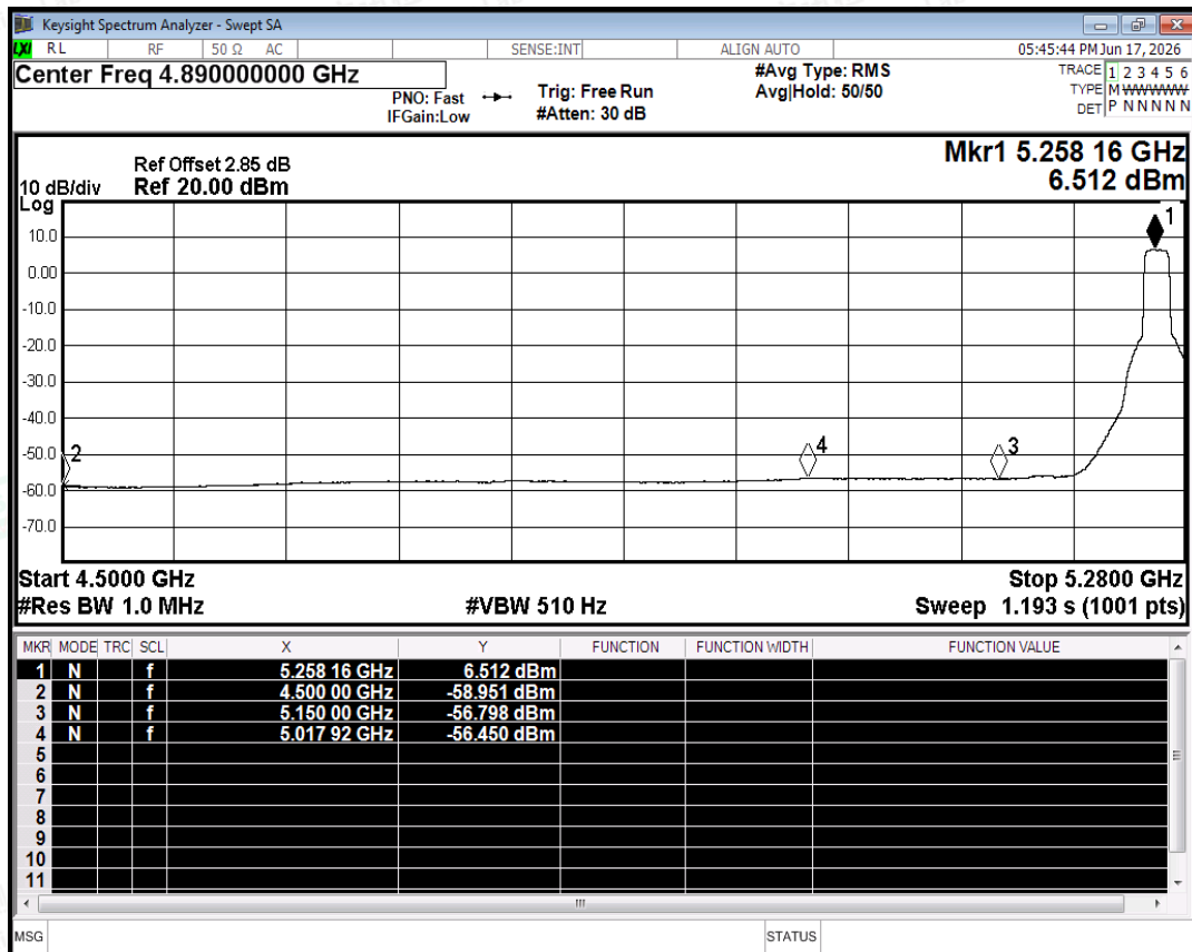
Restrict Band NVNT a 5260MHz Ant0 Average
