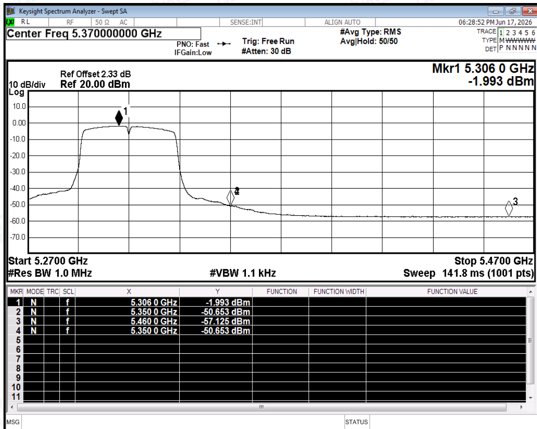
Restrict Band NVNT n40 5310MHz Ant0 Average
