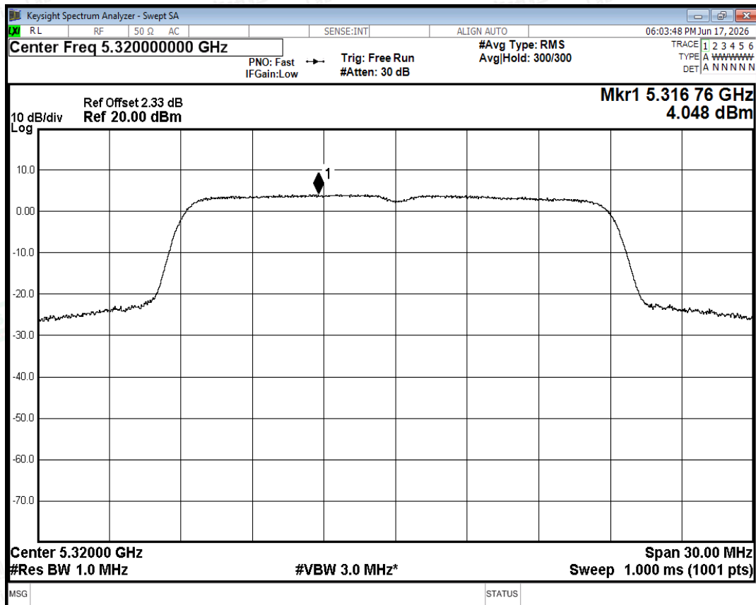
PSD NVNT n20 5320MHz Ant0
