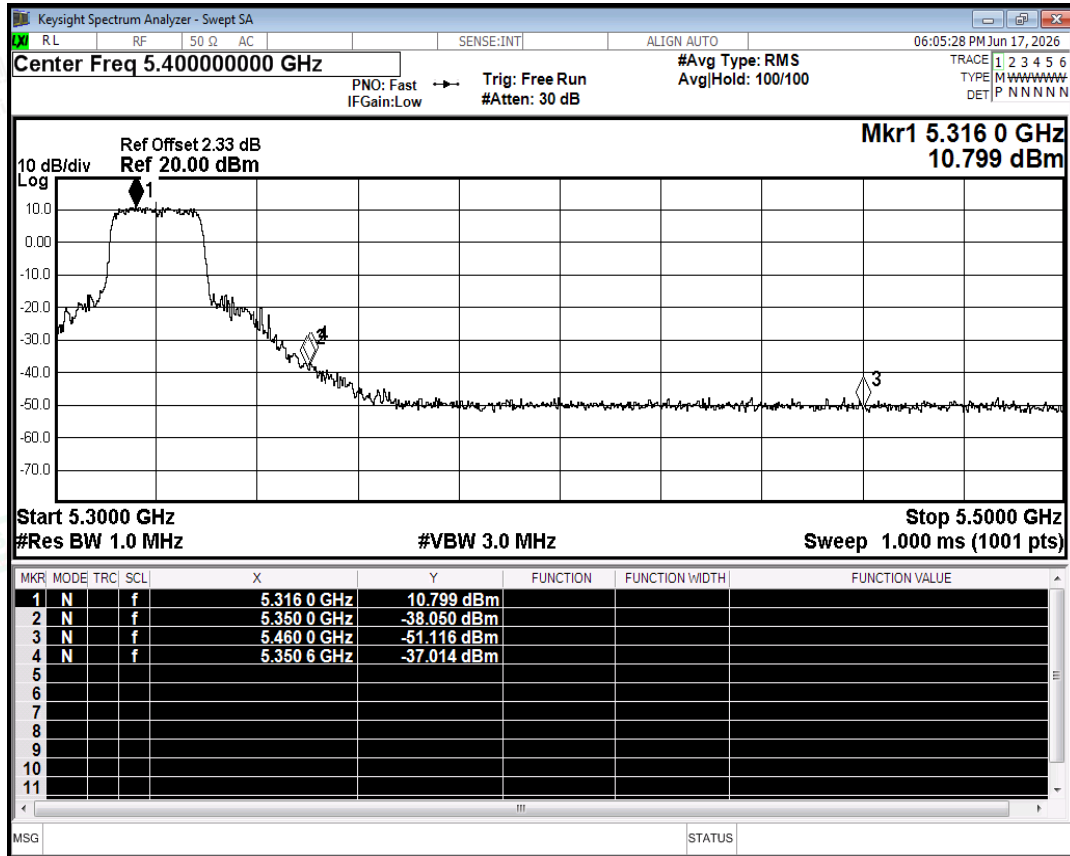
Restrict Band NVNT n20 5320MHz Ant0 Peak
