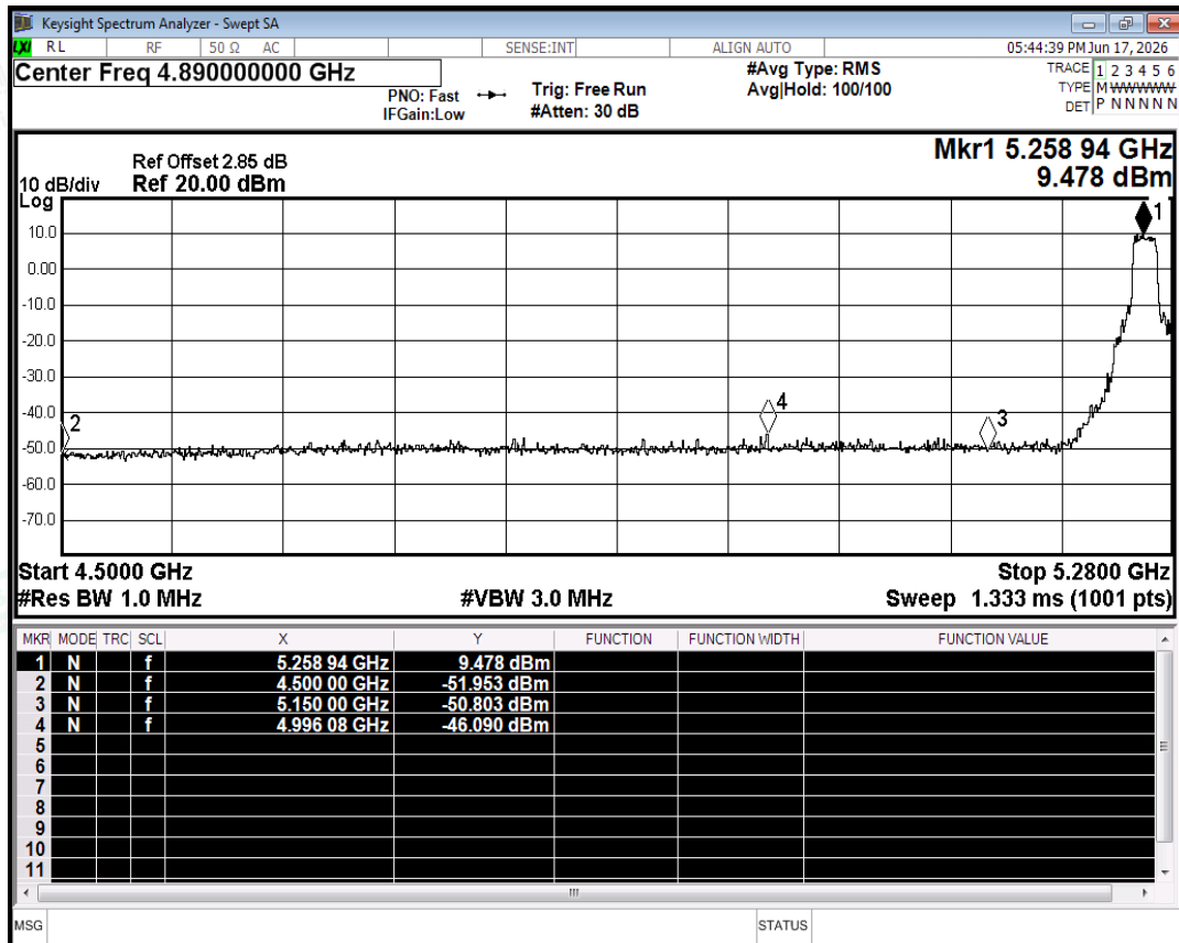
Restrict Band NVNT a 5260MHz Ant0 Peak
