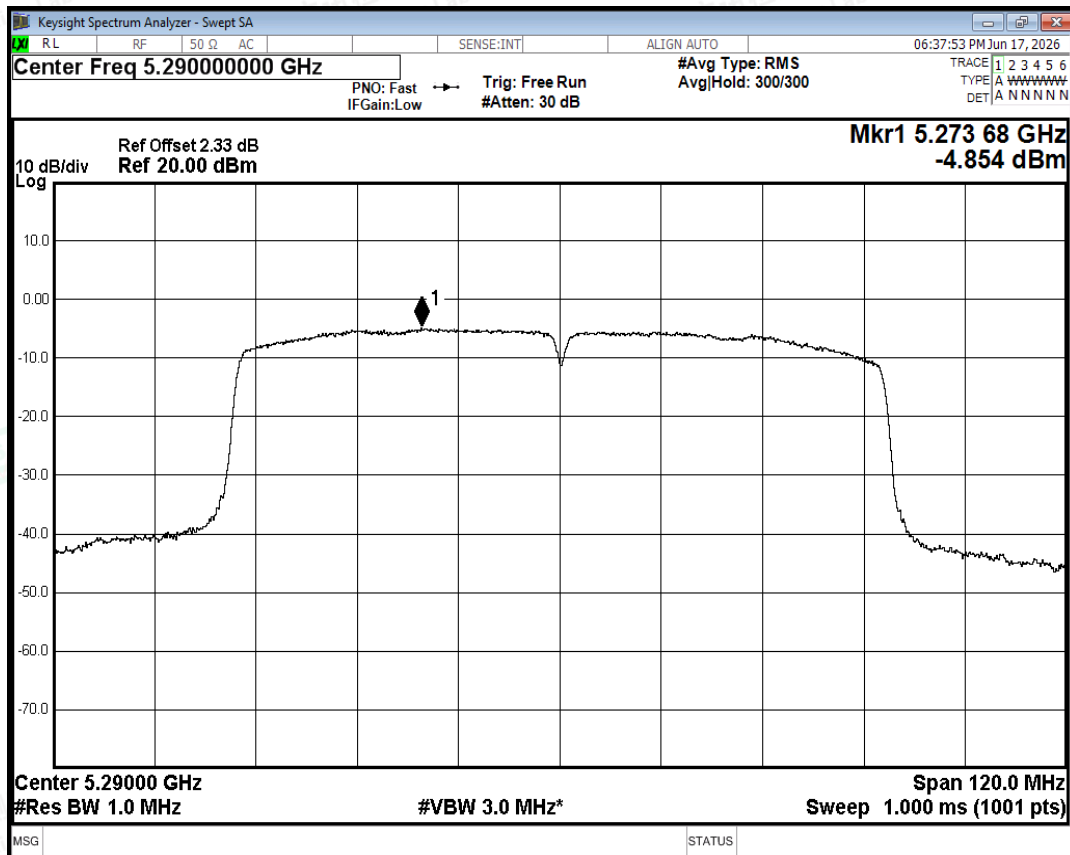
PSD NVNT ac80 5290MHz Ant0
