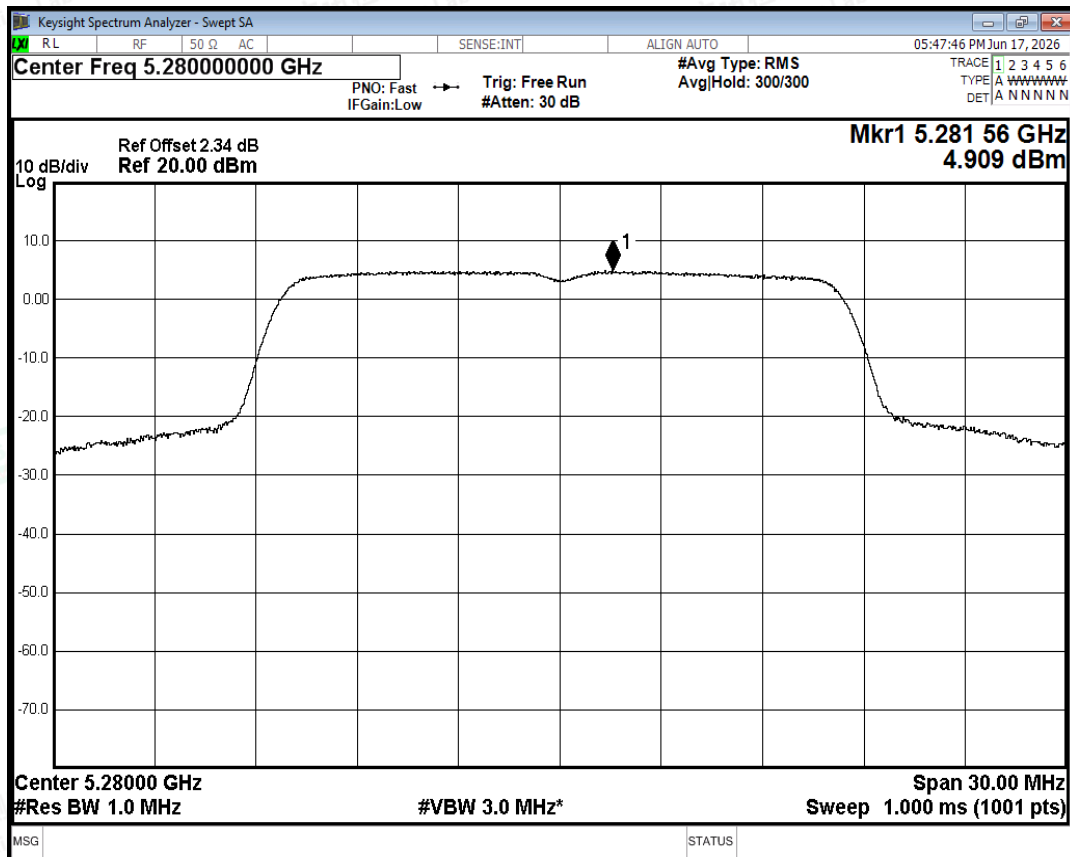
PSD NVNT a 5280MHz Ant0
