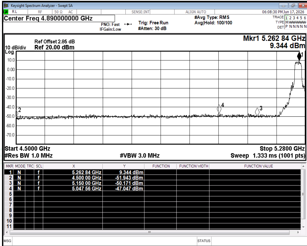
Restrict Band NVNT ac20 5260MHz Ant0 Peak
