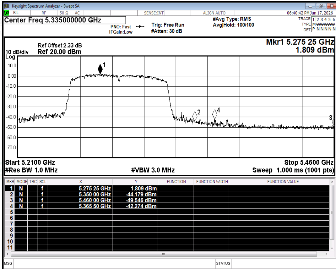
Restrict Band NVNT ac80 5290MHz Ant0 Peak
