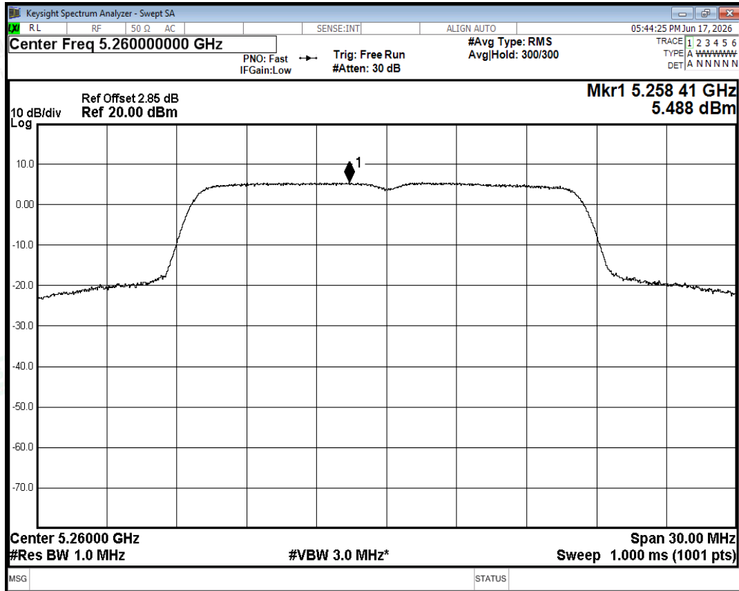
PSD NVNT a 5260MHz Ant0
