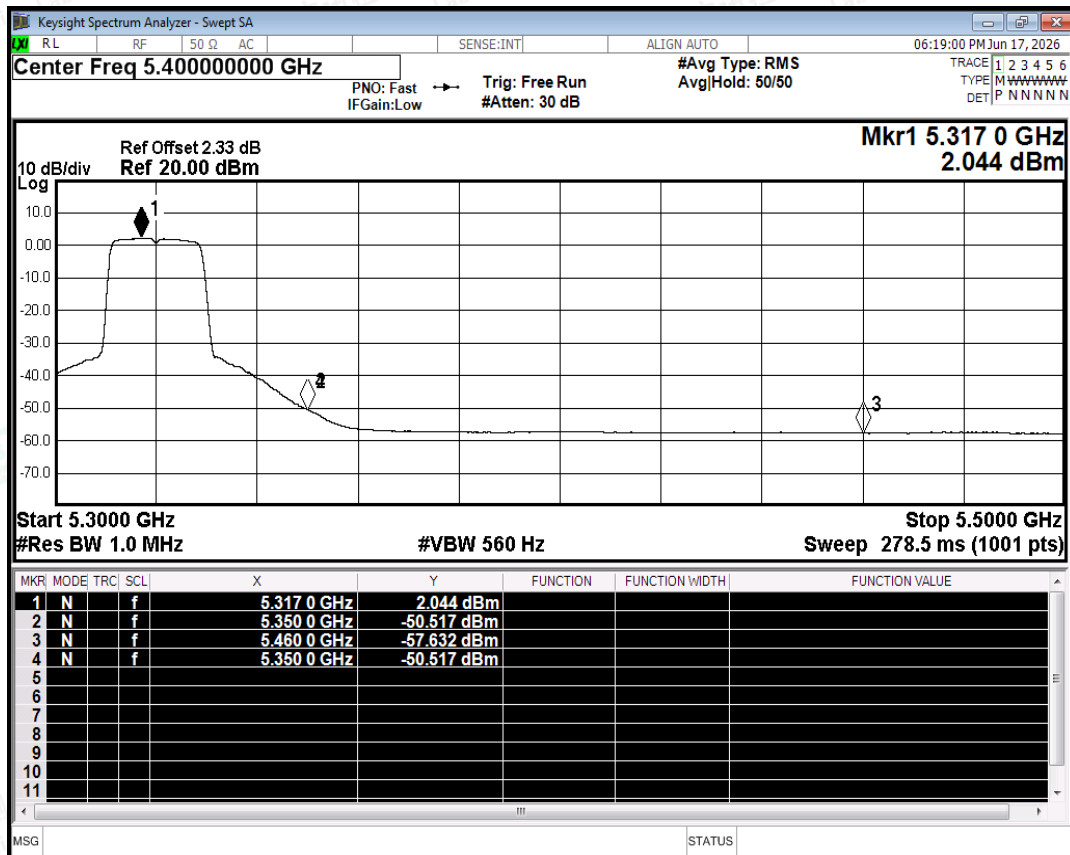
Restrict Band NVNT ac20 5320MHz Ant0 Average
