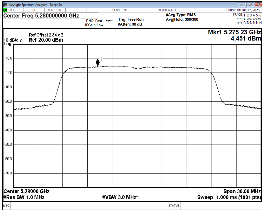
PSD NVNT n20 5280MHz Ant0
