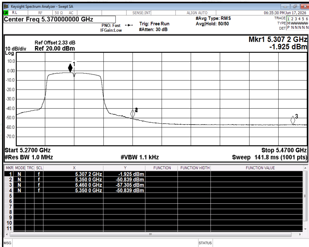
Restrict Band NVNT ac40 5310MHz Ant0 Average
