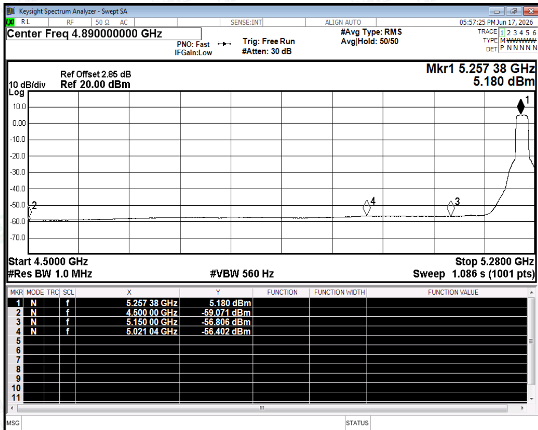
Restrict Band NVNT n20 5260MHz Ant0 Average
