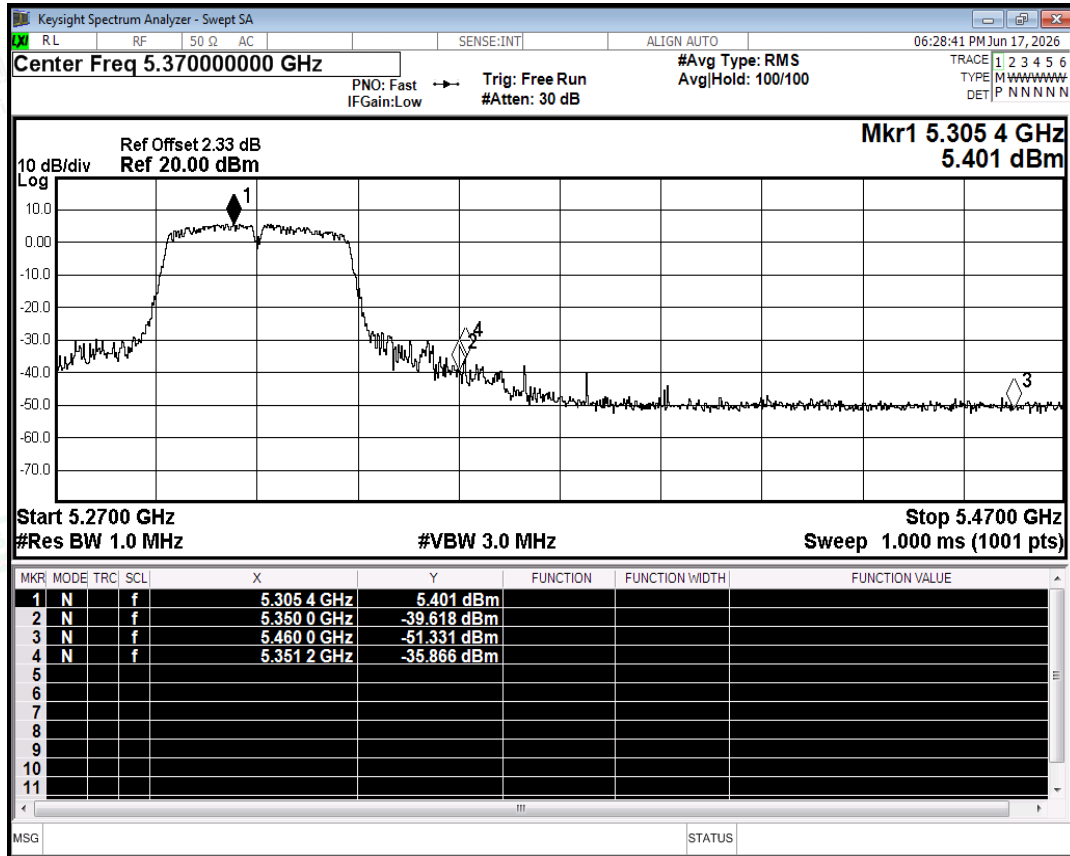
Restrict Band NVNT n40 5310MHz Ant0 Peak
