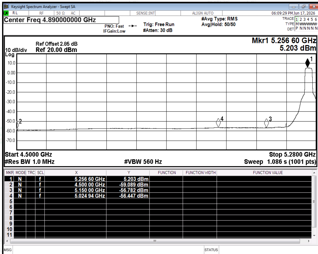
Restrict Band NVNT ac20 5260MHz Ant0 Average
