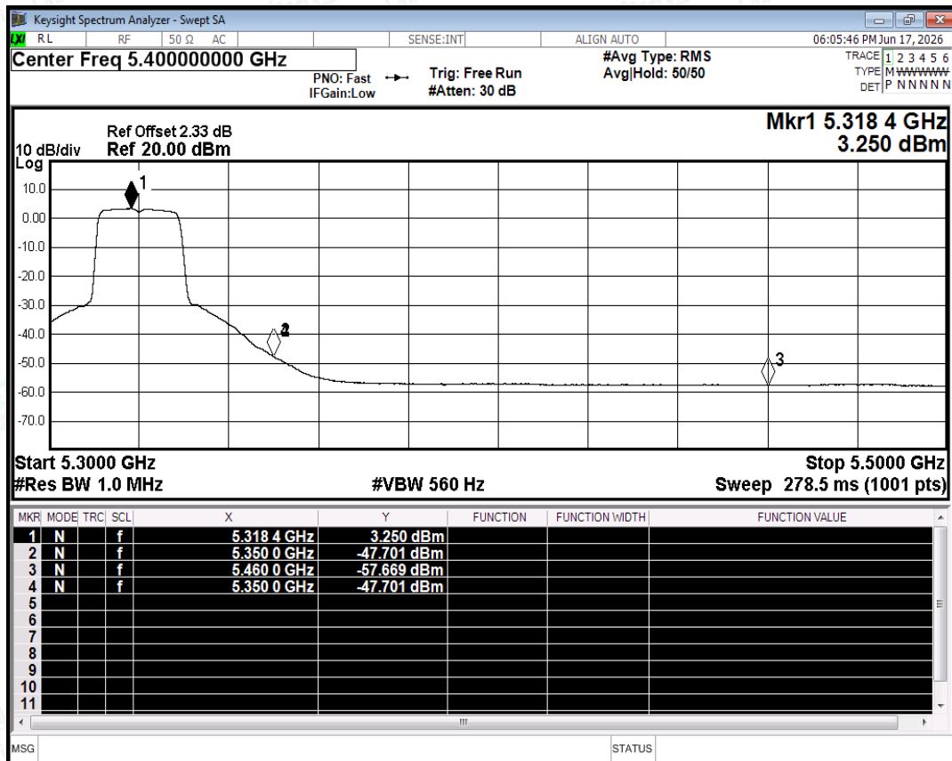
Restrict Band NVNT n20 5320MHz Ant0 Average
