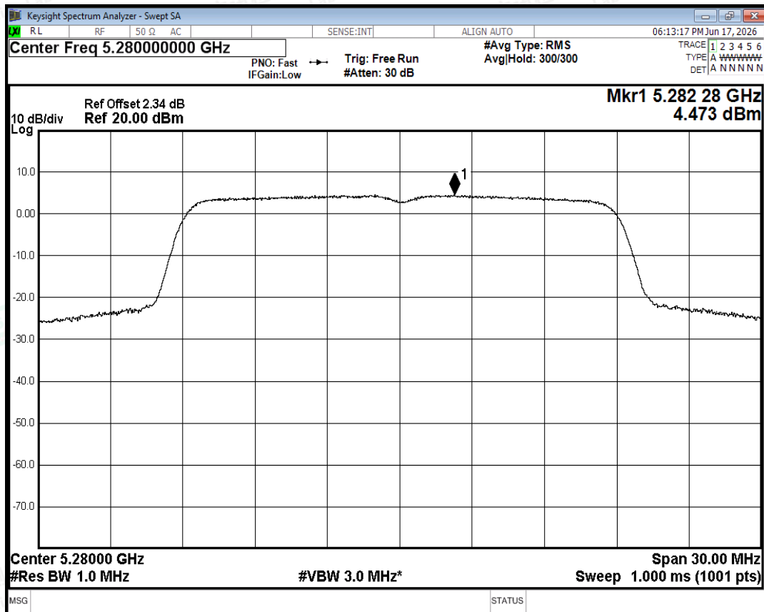
PSD NVNT ac20 5280MHz Ant0
