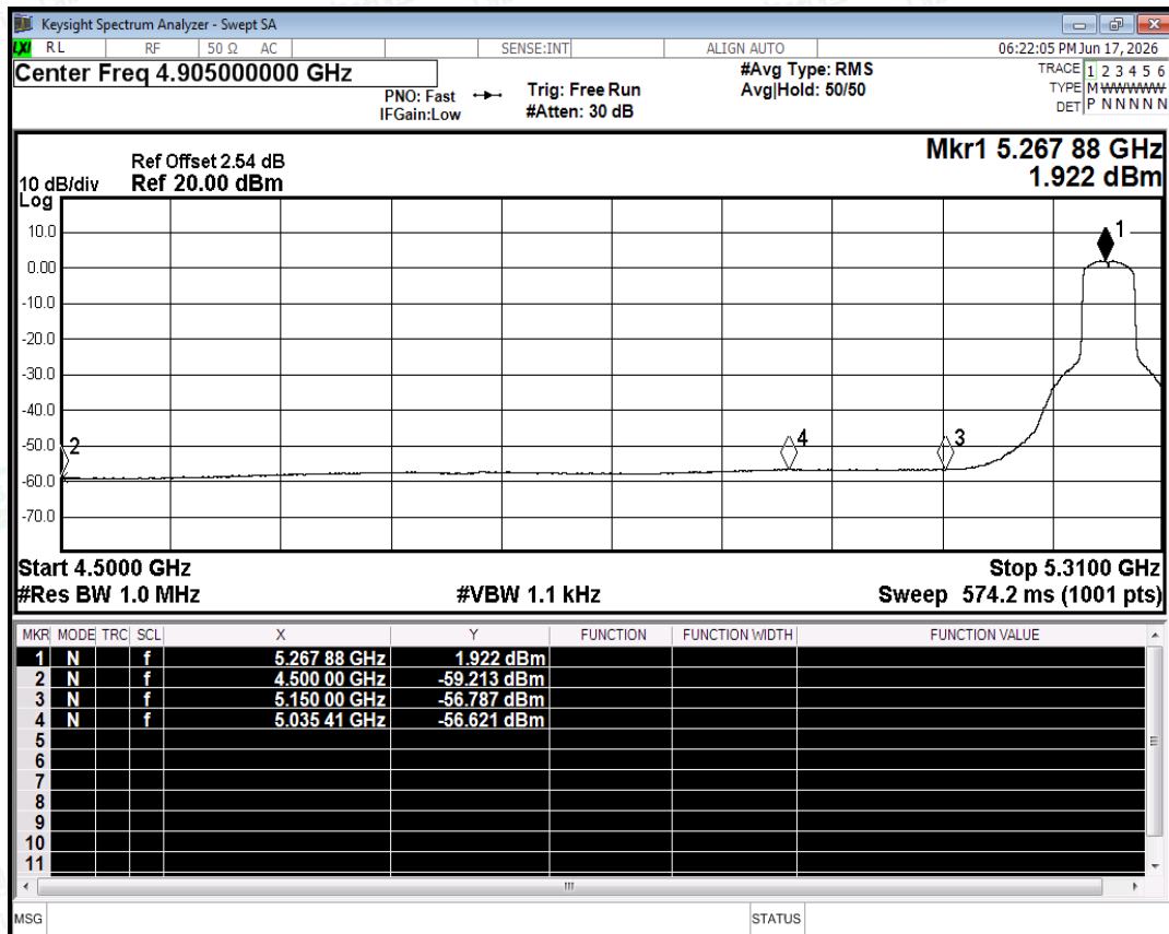
Restrict Band NVNT n40 5270MHz Ant0 Average
