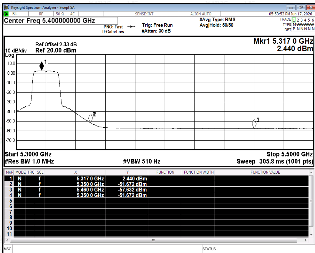
Restrict Band NVNT a 5320MHz Ant0 Average
