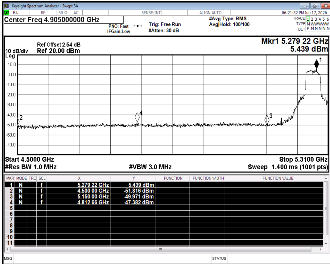
Restrict Band NVNT n40 5270MHz Ant0 Peak
