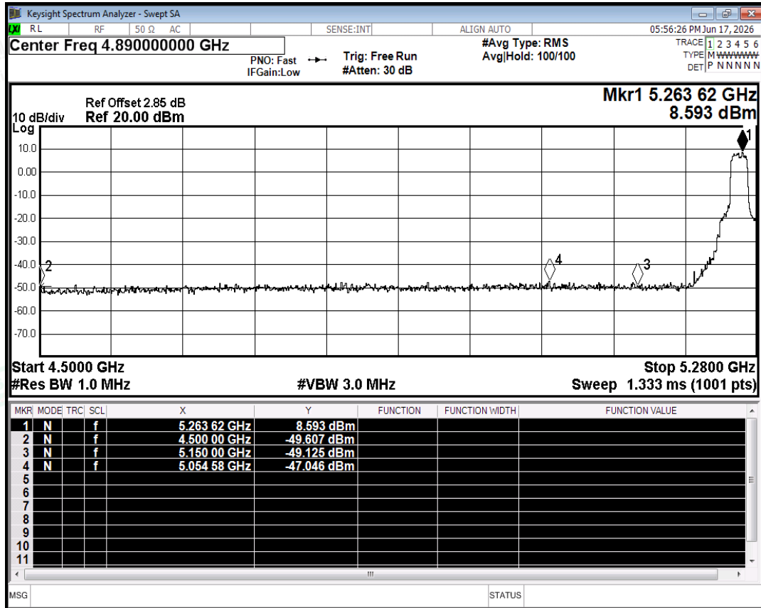
Restrict Band NVNT n20 5260MHz Ant0 Peak
