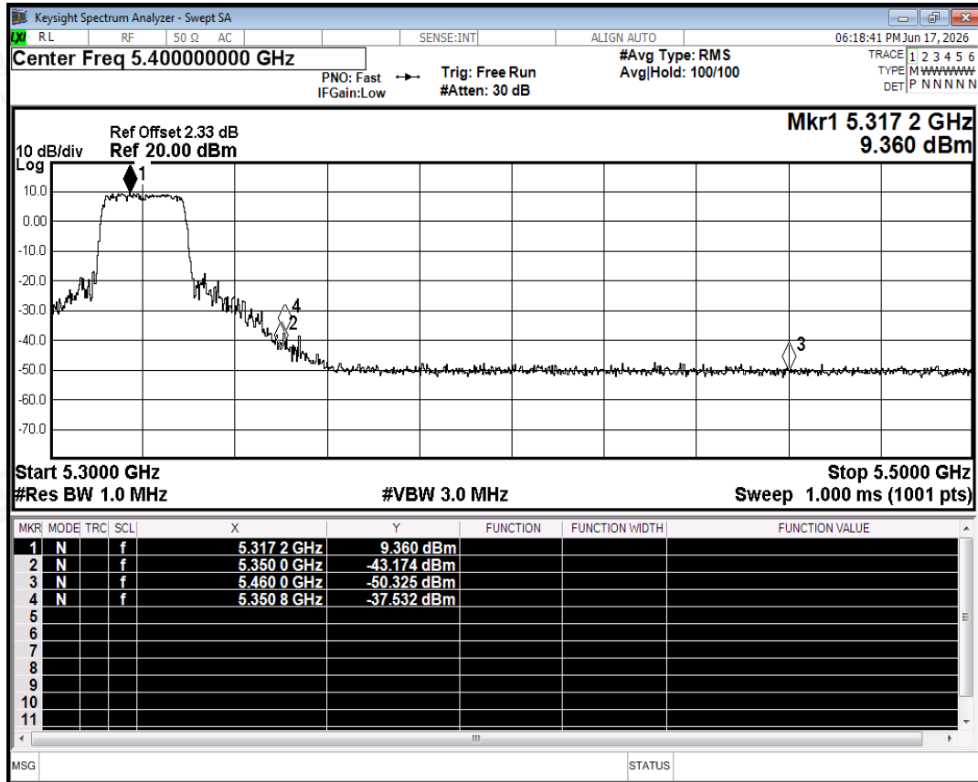
Restrict Band NVNT ac20 5320MHz Ant0 Peak
