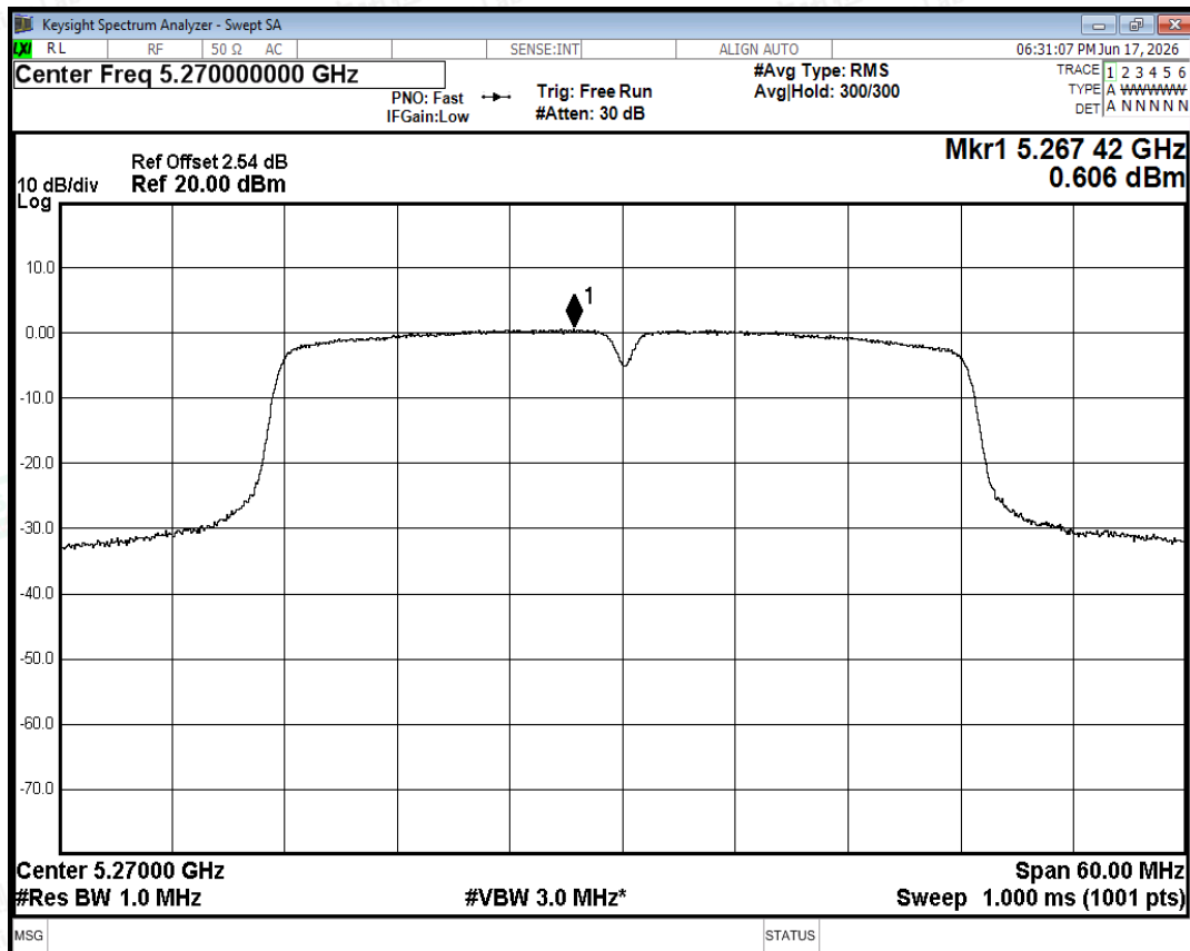
PSD NVNT ac40 5270MHz Ant0
