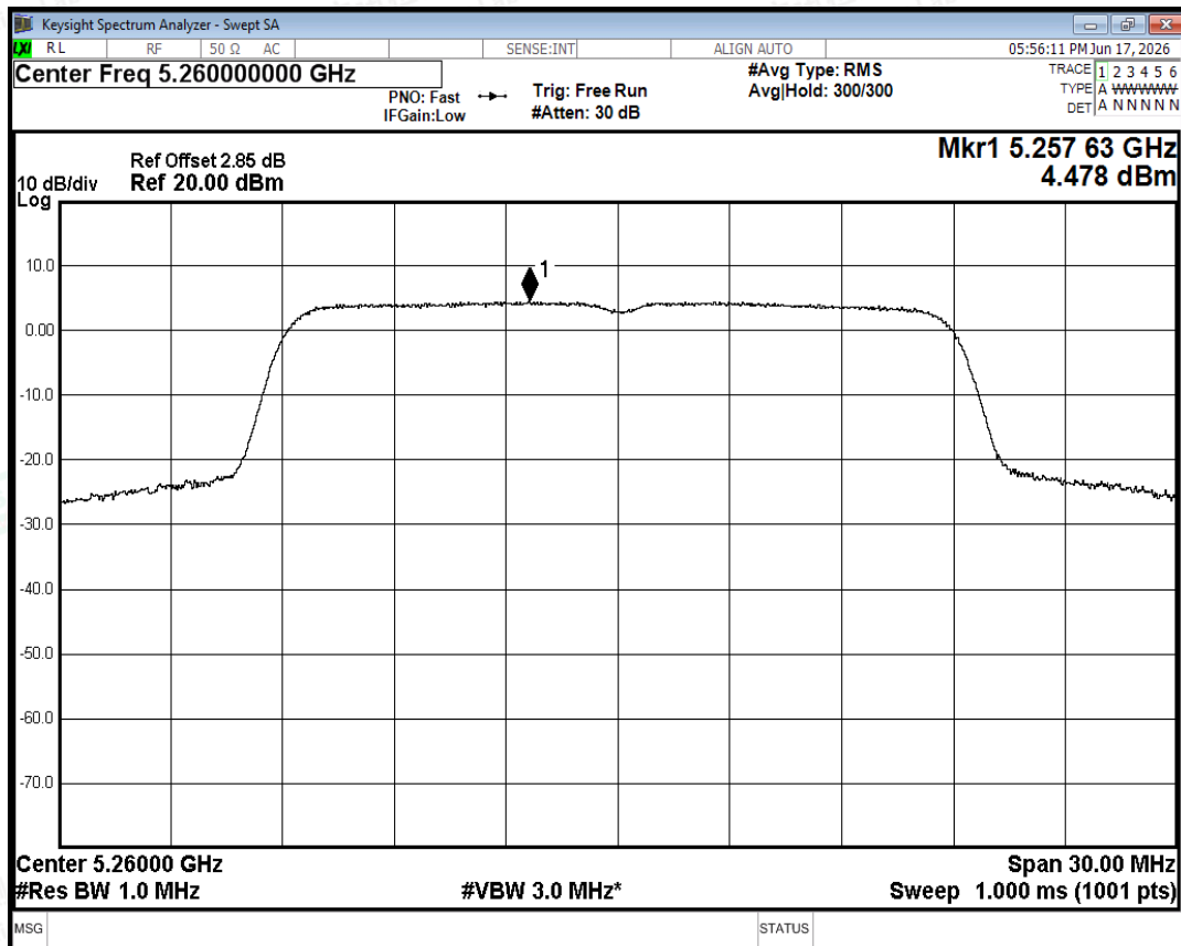
PSD NVNT n20 5260MHz Ant0
