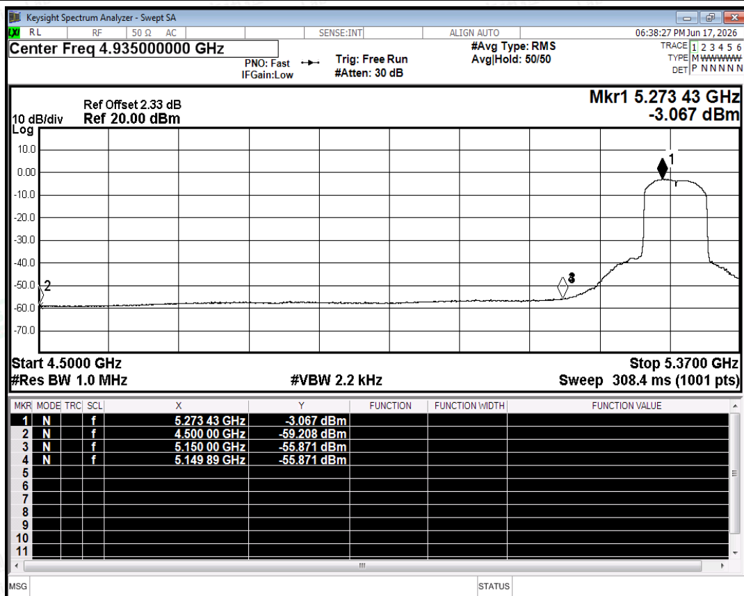
Restrict Band NVNT ac80 5290MHz Ant0 Average
