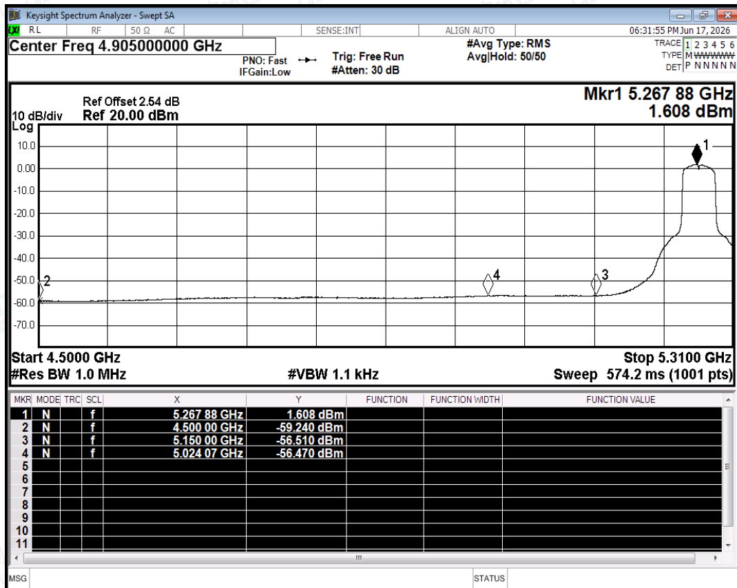
Restrict Band NVNT ac40 5270MHz Ant0 Average
