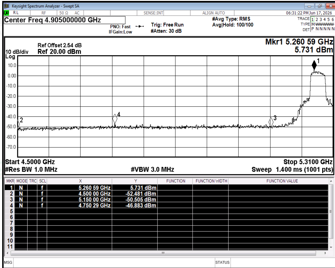
Restrict Band NVNT ac40 5270MHz Ant0 Peak
