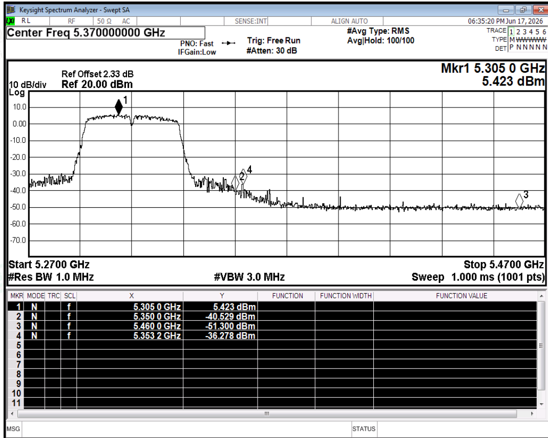
Restrict Band NVNT ac40 5310MHz Ant0 Peak
