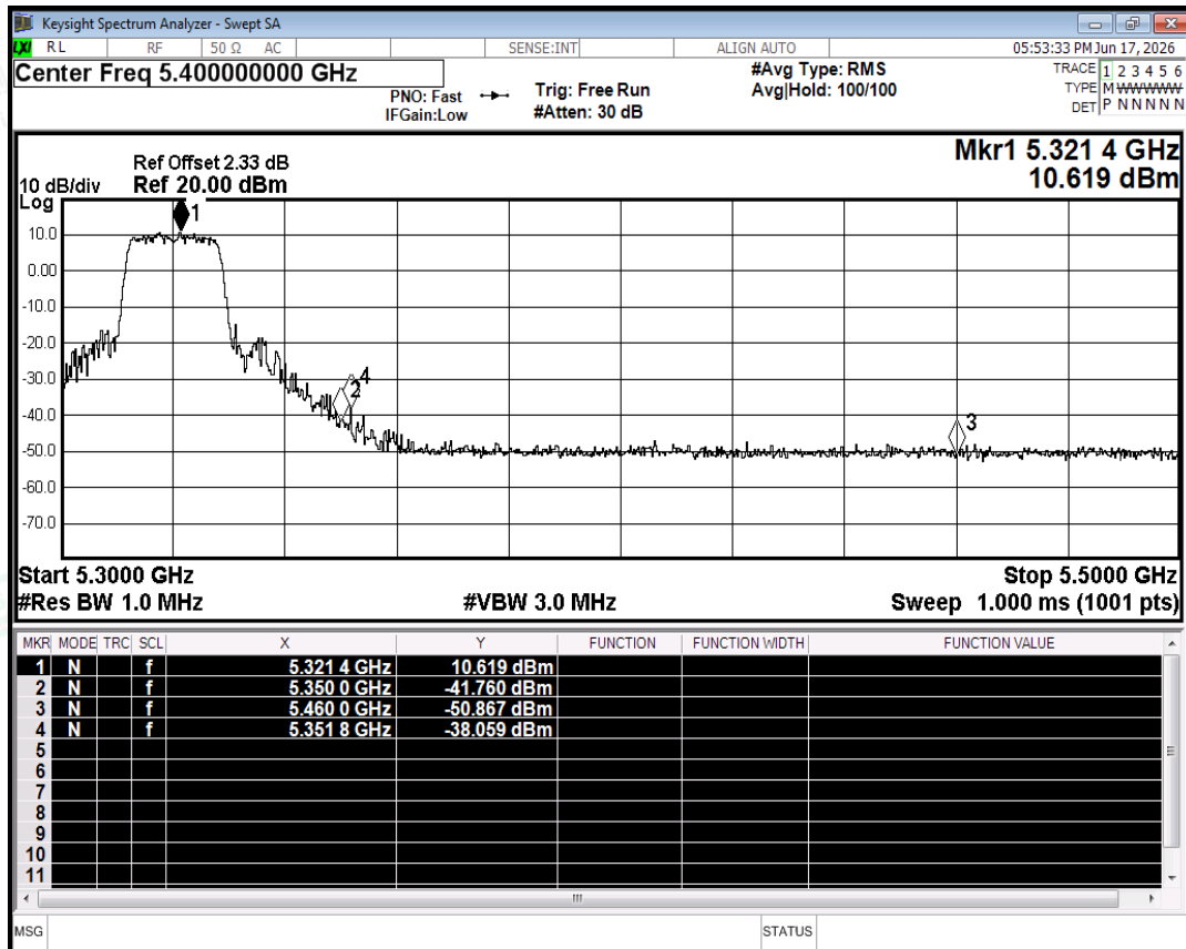
Restrict Band NVNT a 5320MHz Ant0 Peak
