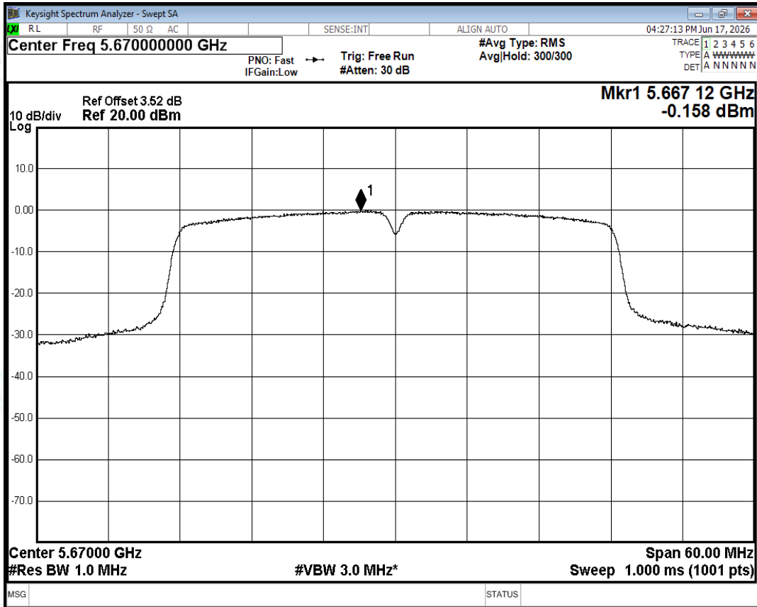
PSD NVNT ac40 5670MHz Ant0
