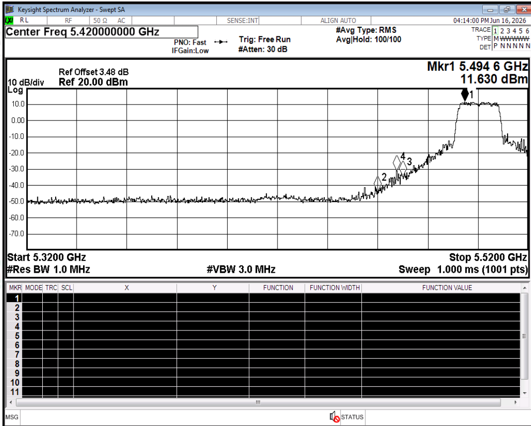
Restrict Band NVNT a 5500MHz Ant1 Peak
