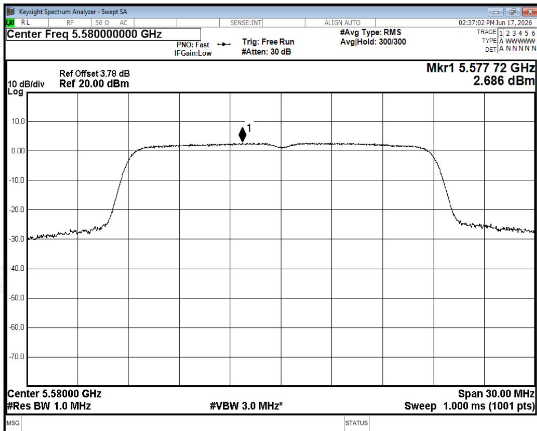
PSD NVNT ac20 5580MHz Ant0
