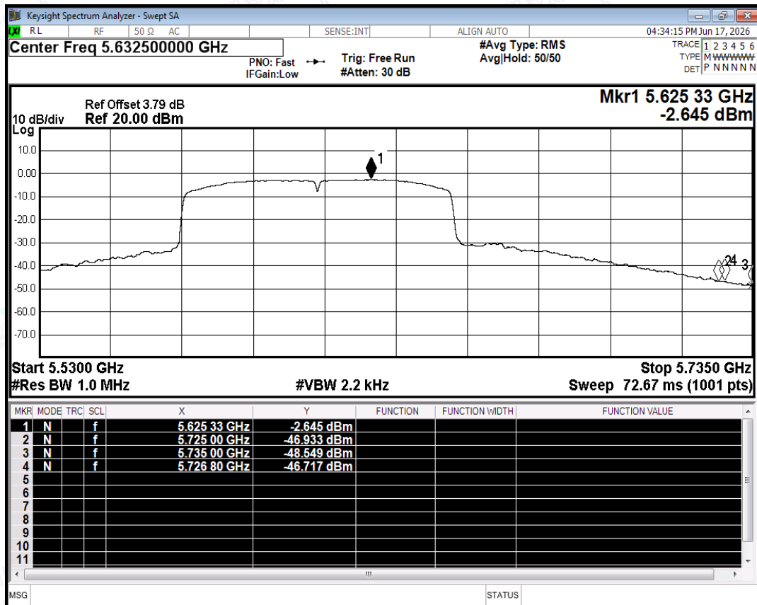
Restrict Band NVNT ac80 5610MHz Ant0 Average
