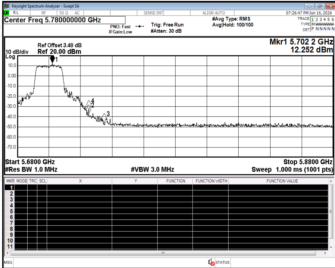
Restrict Band NVNT a 5700MHz Ant0 Peak
