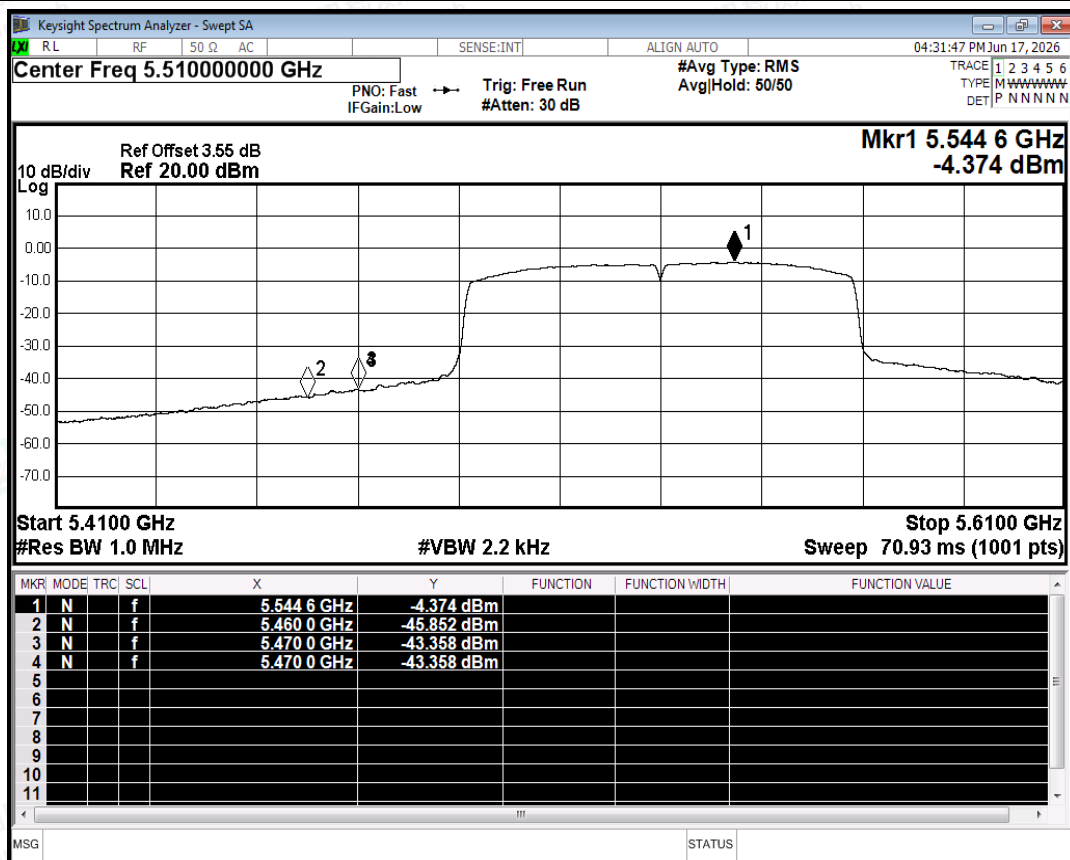
Restrict Band NVNT ac80 5530MHz Ant0 Average
