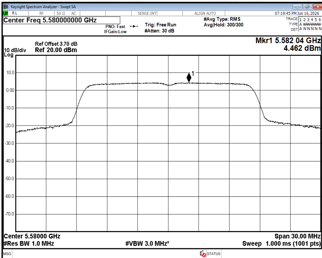
PSD NVNT a 5580MHz Ant0
