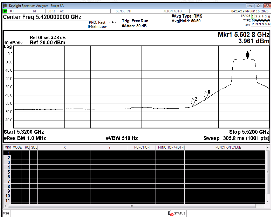
Restrict Band NVNT a 5500MHz Ant1 Average
