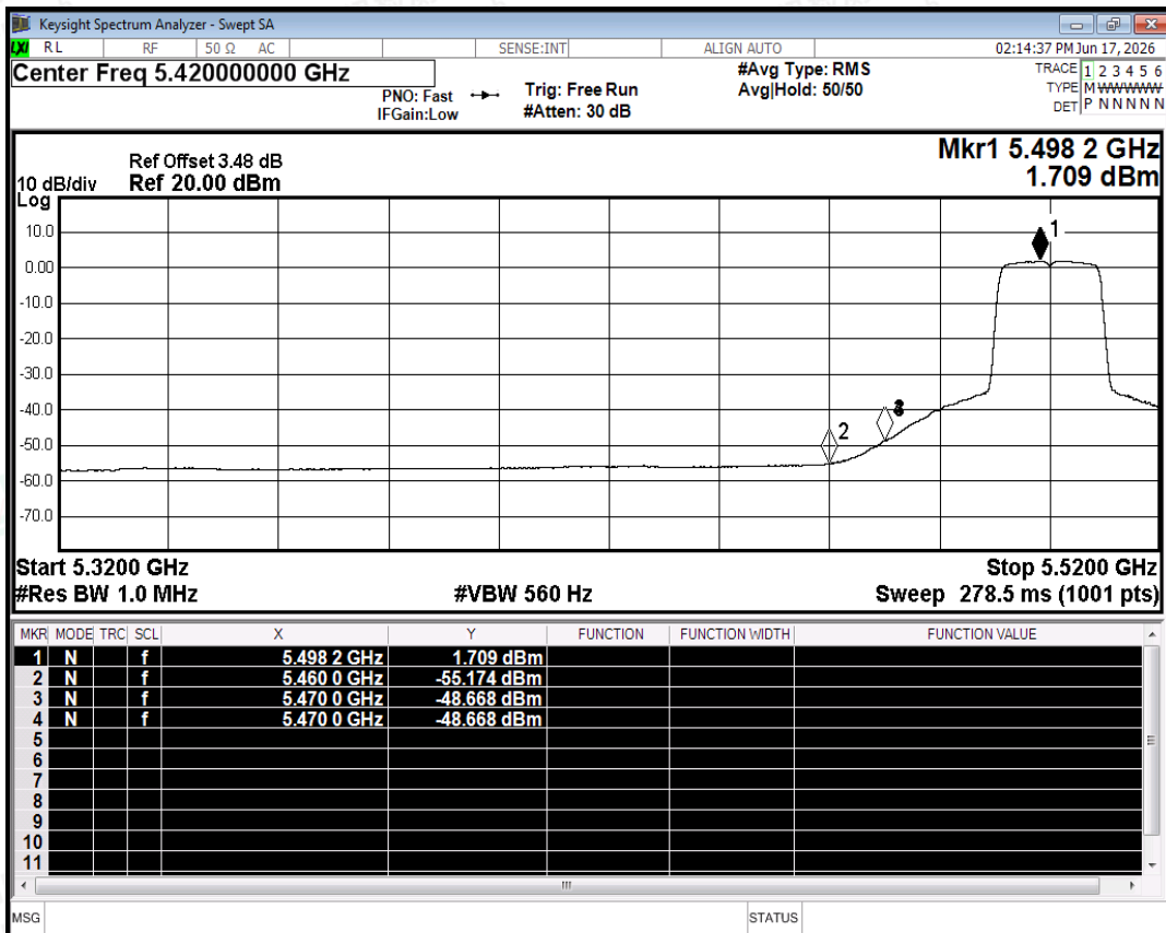
Restrict Band NVNT n20 5500MHz Ant0 Average
