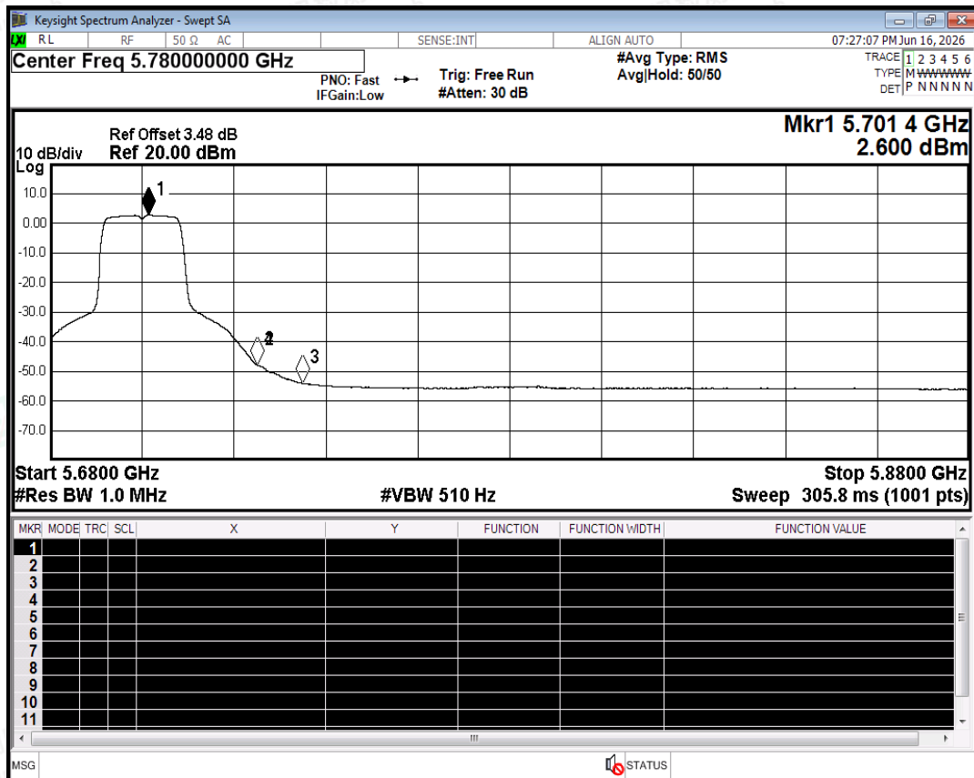
Restrict Band NVNT a 5700MHz Ant0 Average
