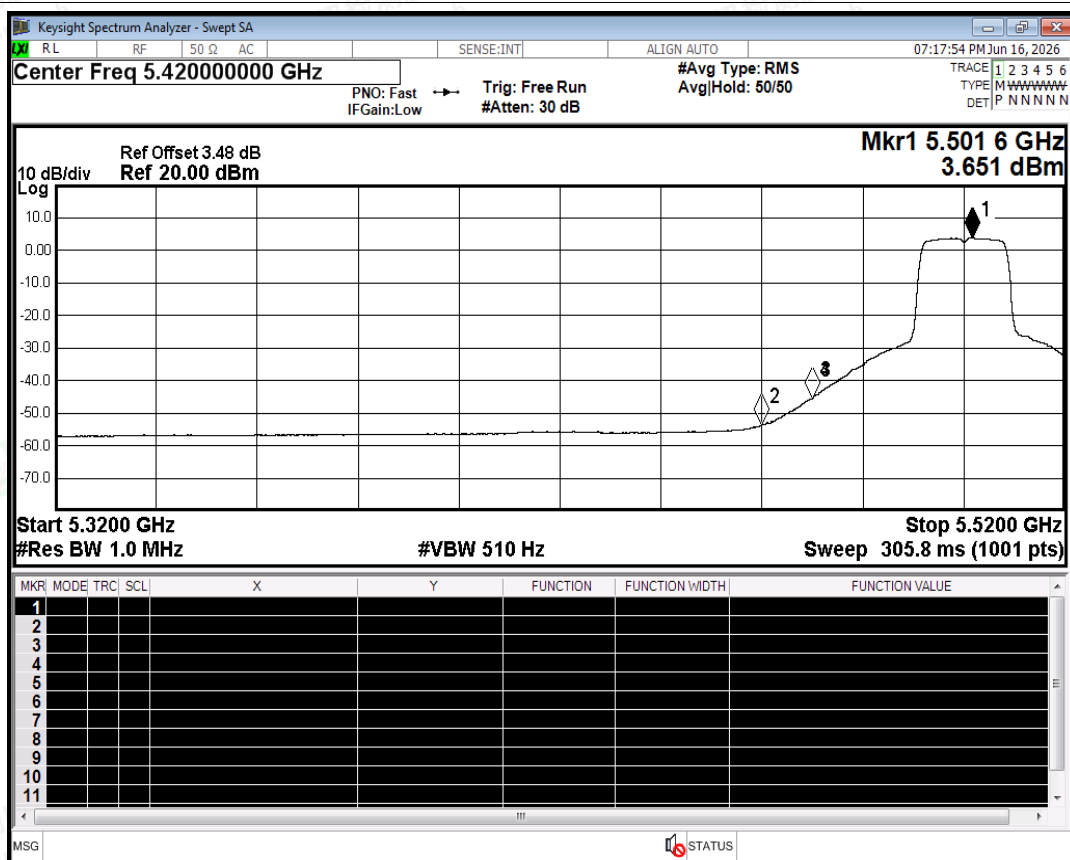
Restrict Band NVNT a 5500MHz Ant0 Average
