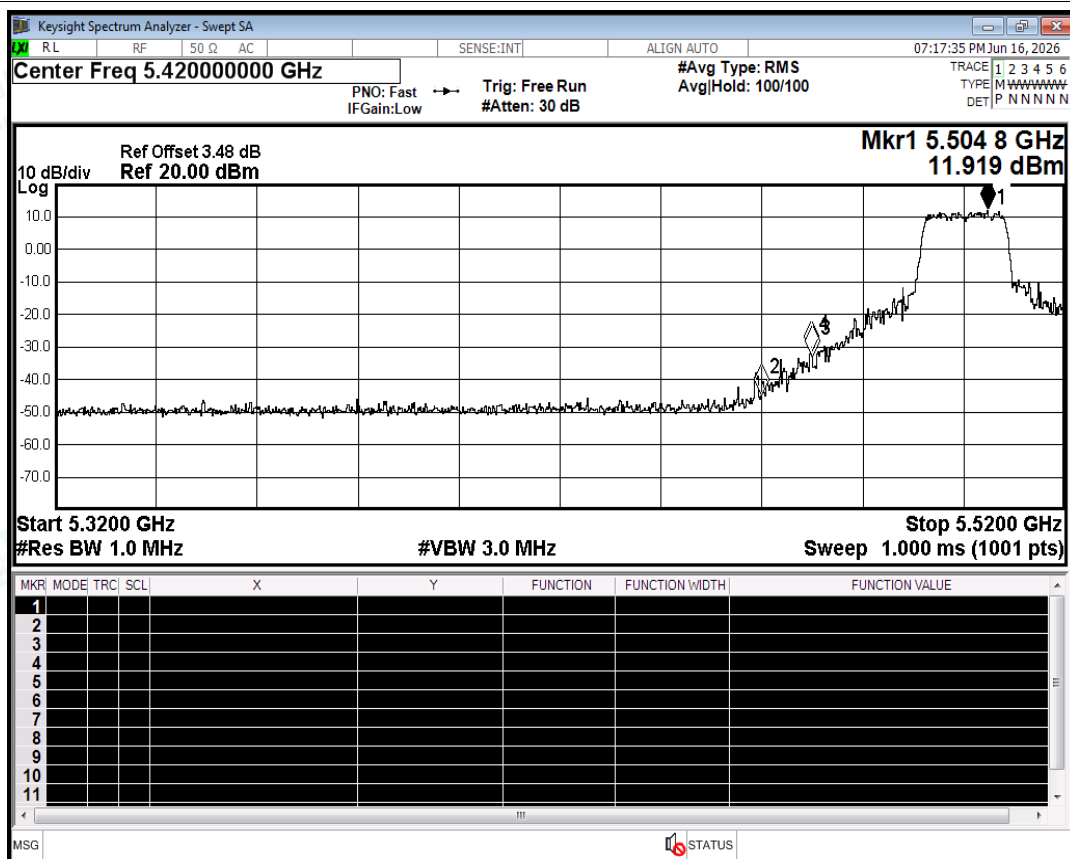
Restrict Band NVNT a 5500MHz Ant0 Peak
