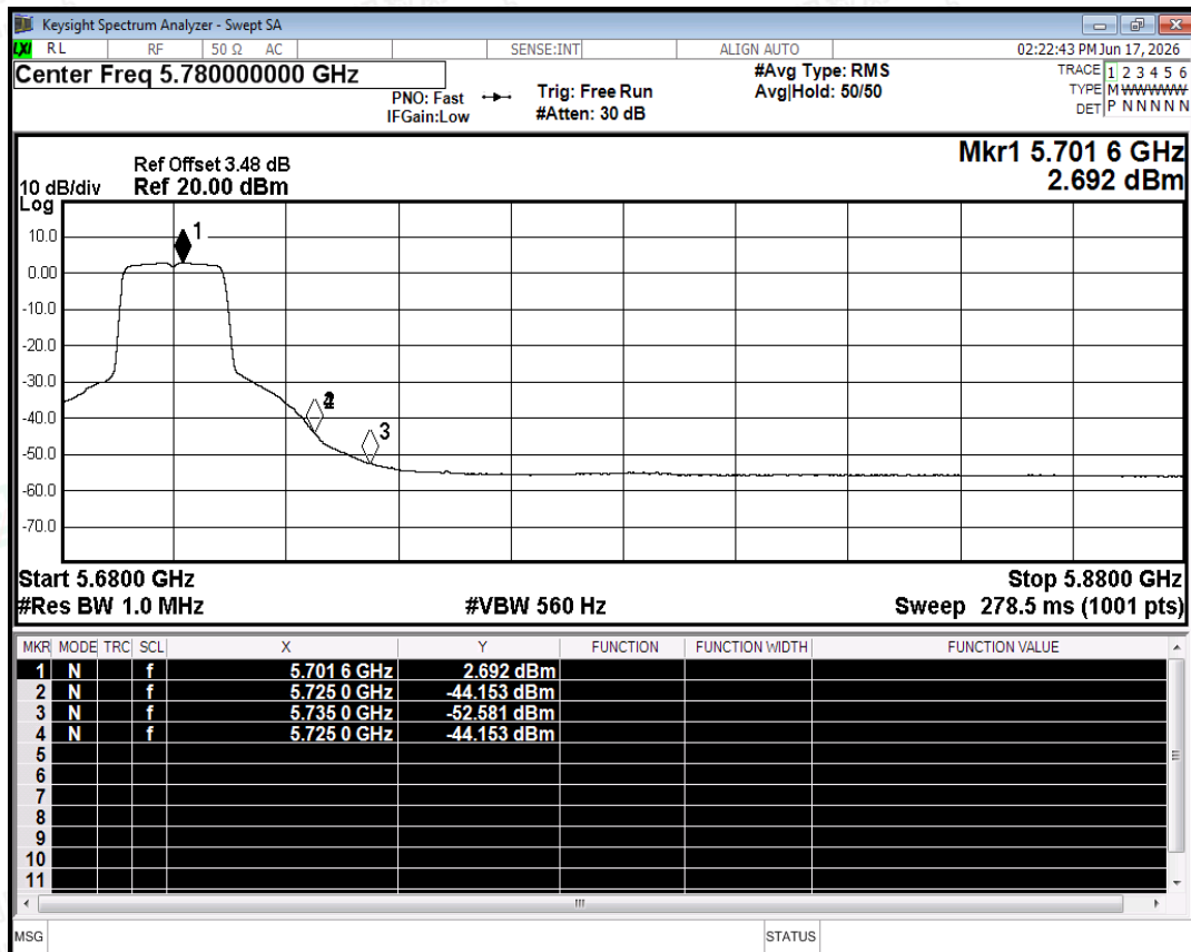
Restrict Band NVNT n20 5700MHz Ant0 Average
