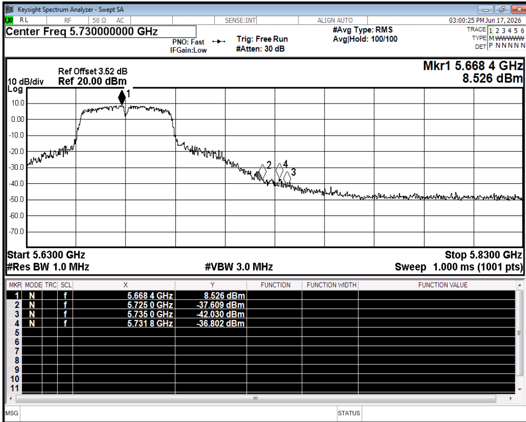
Restrict Band NVNT n40 5670MHz Ant0 Peak
