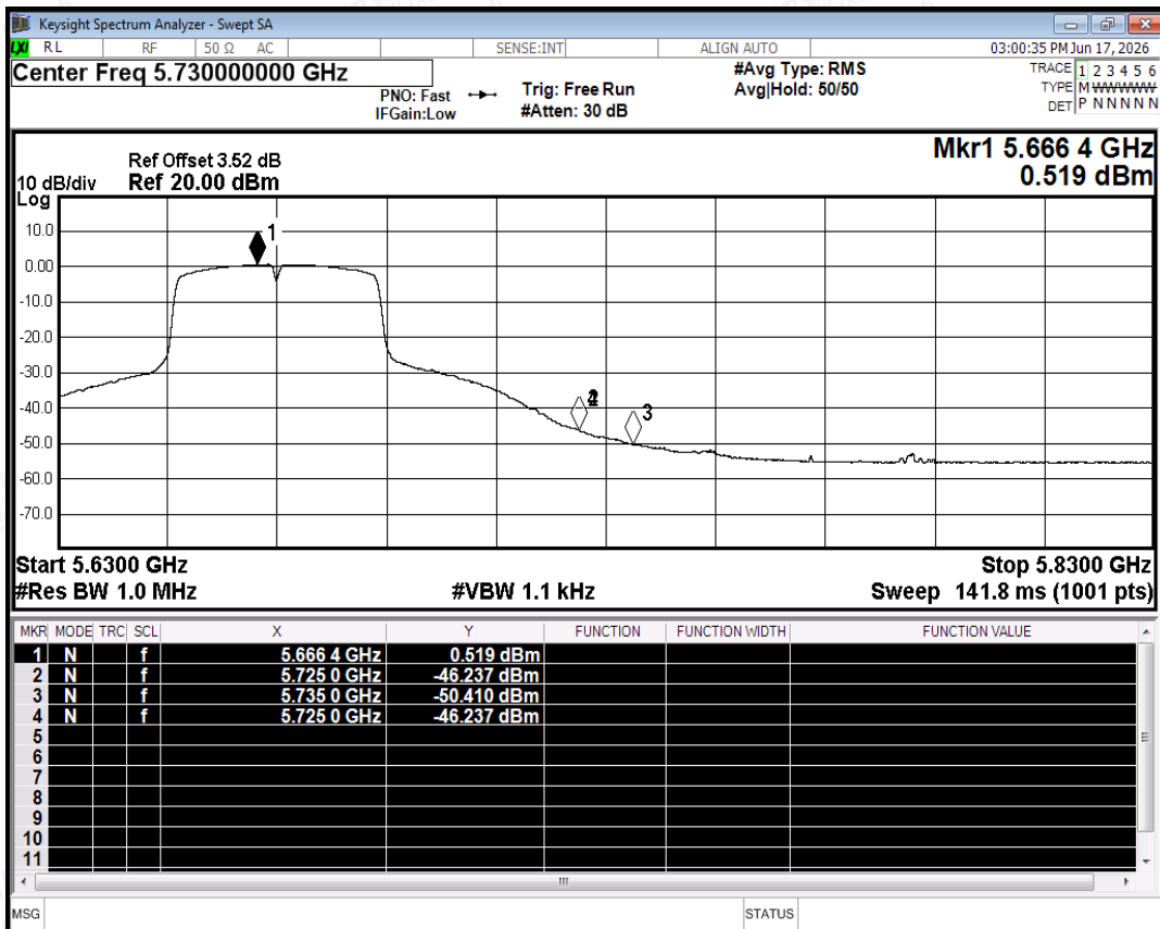
Restrict Band NVNT n40 5670MHz Ant0 Average
