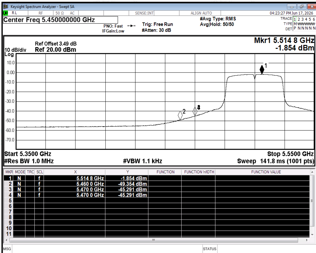
Restrict Band NVNT ac40 5510MHz Ant0 Average
