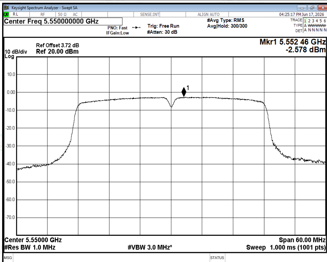
PSD NVNT ac40 5550MHz Ant0
