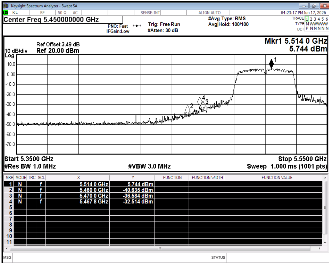
Restrict Band NVNT ac40 5510MHz Ant0 Peak
