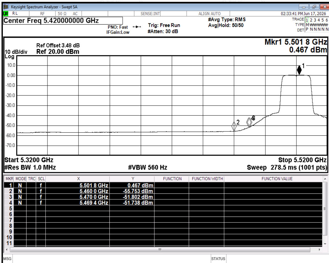
Restrict Band NVNT ac20 5500MHz Ant0 Average
