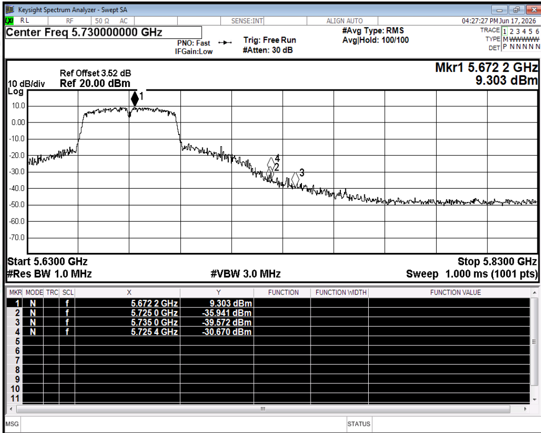
Restrict Band NVNT ac40 5670MHz Ant0 Peak
