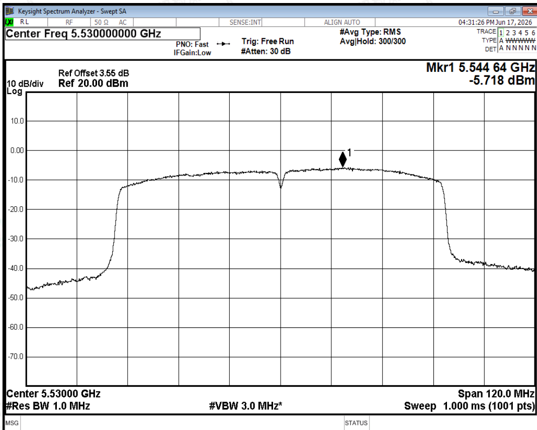
PSD NVNT ac80 5530MHz Ant0
