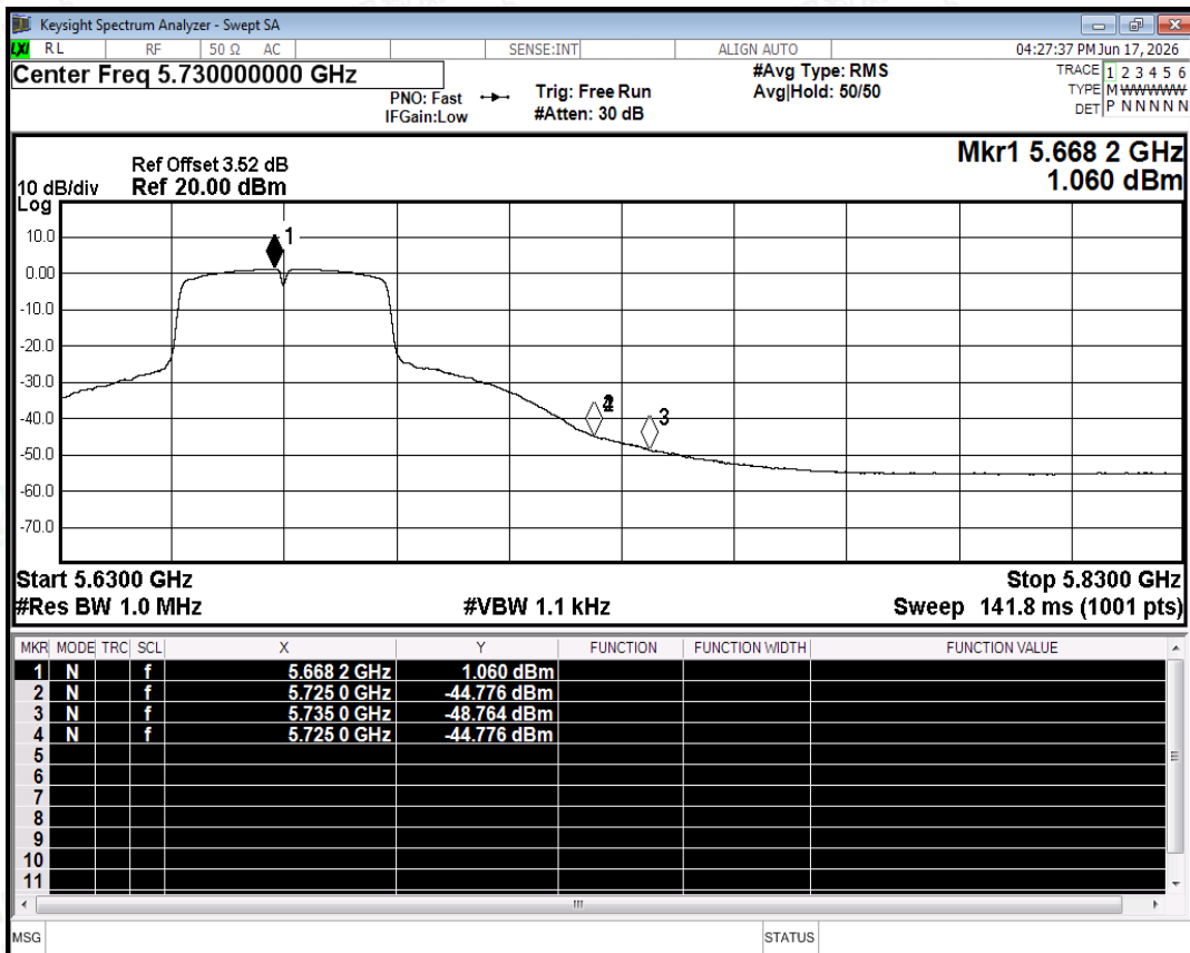
Restrict Band NVNT ac40 5670MHz Ant0 Average
