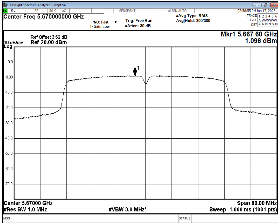
PSD NVNT n40 5670MHz Ant0
