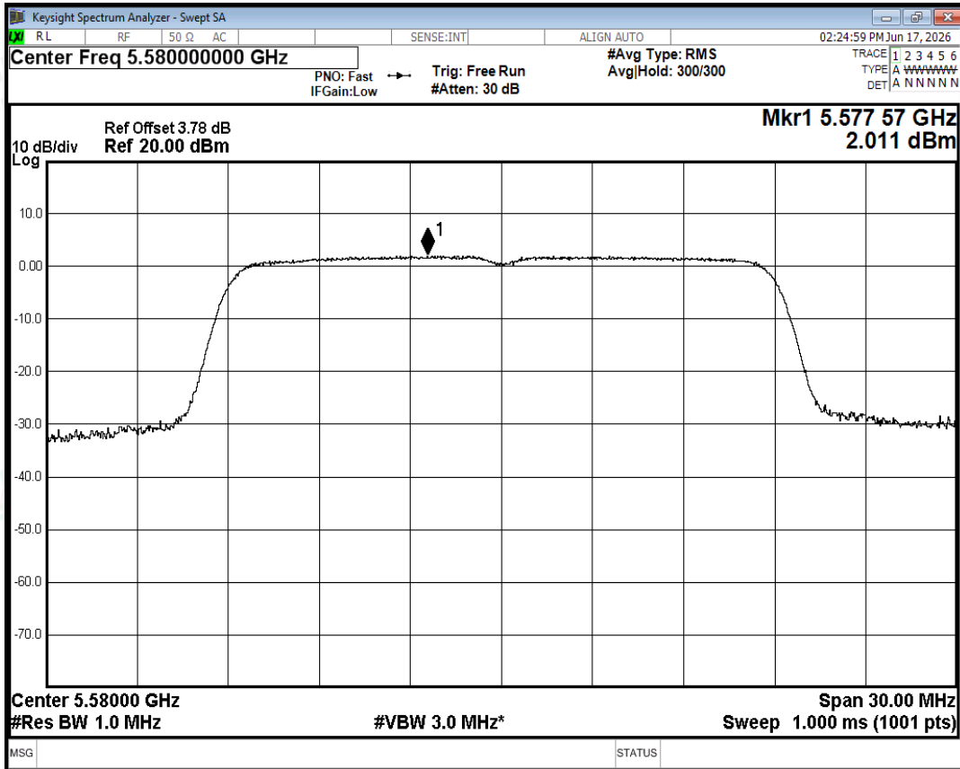
PSD NVNT n20 5580MHz Ant0
