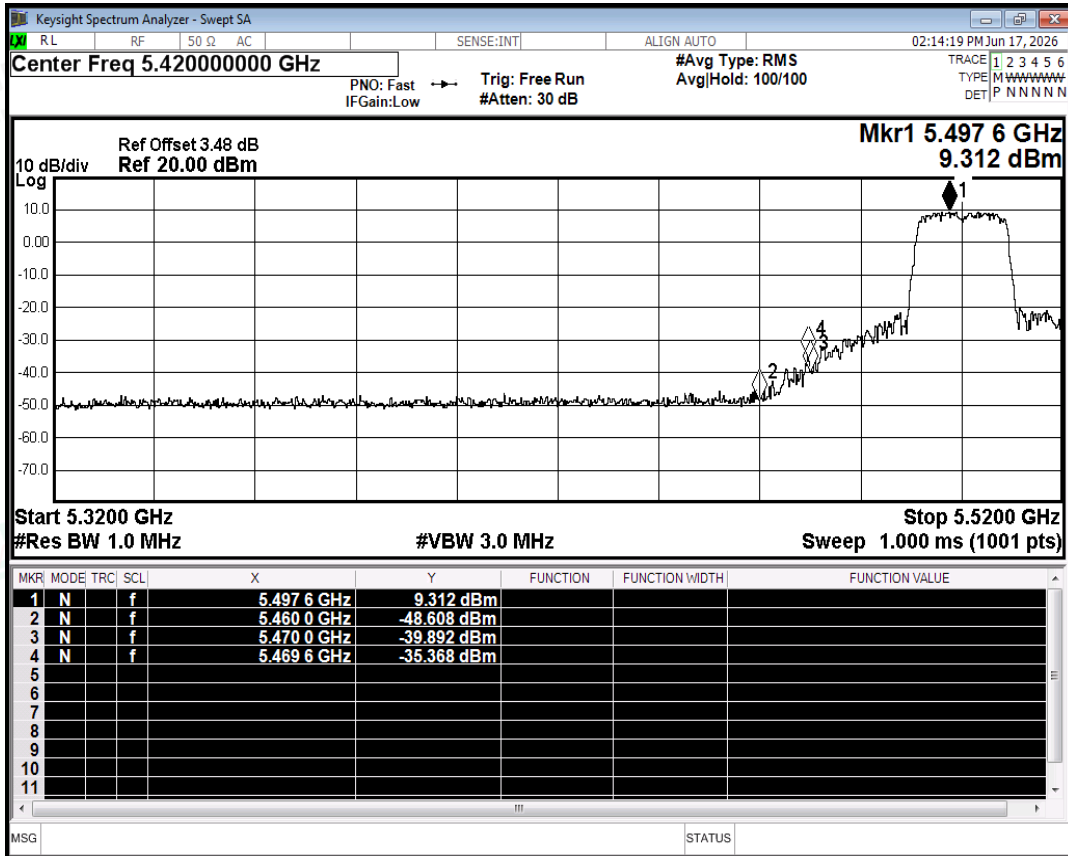
Restrict Band NVNT n20 5500MHz Ant0 Peak
