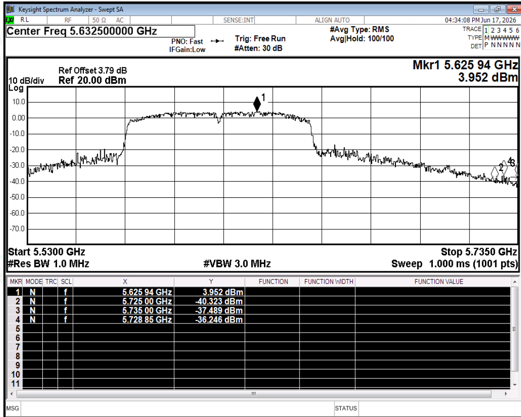
Restrict Band NVNT ac80 5610MHz Ant0 Peak
