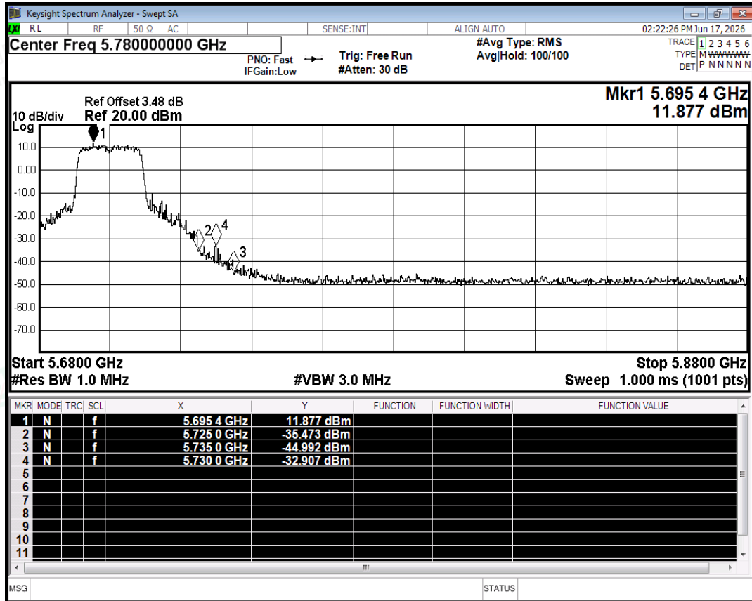
Restrict Band NVNT n20 5700MHz Ant0 Peak
