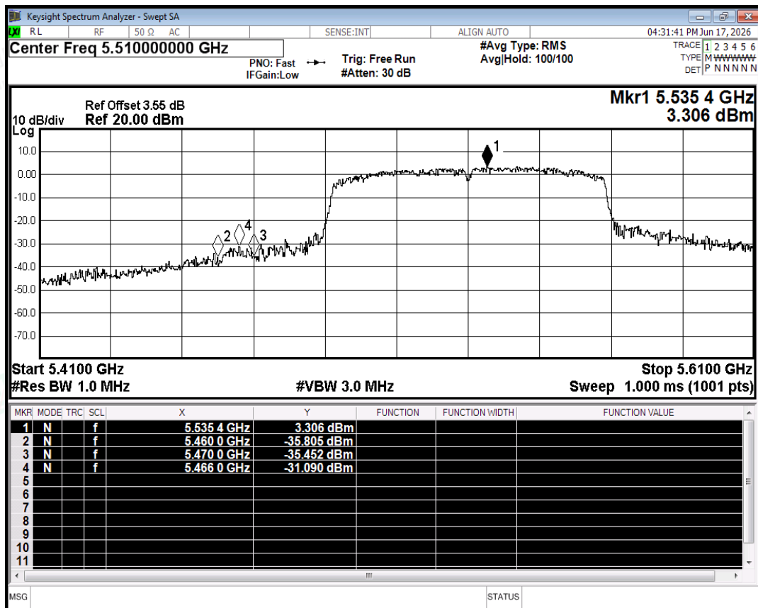
Restrict Band NVNT ac80 5530MHz Ant0 Peak
