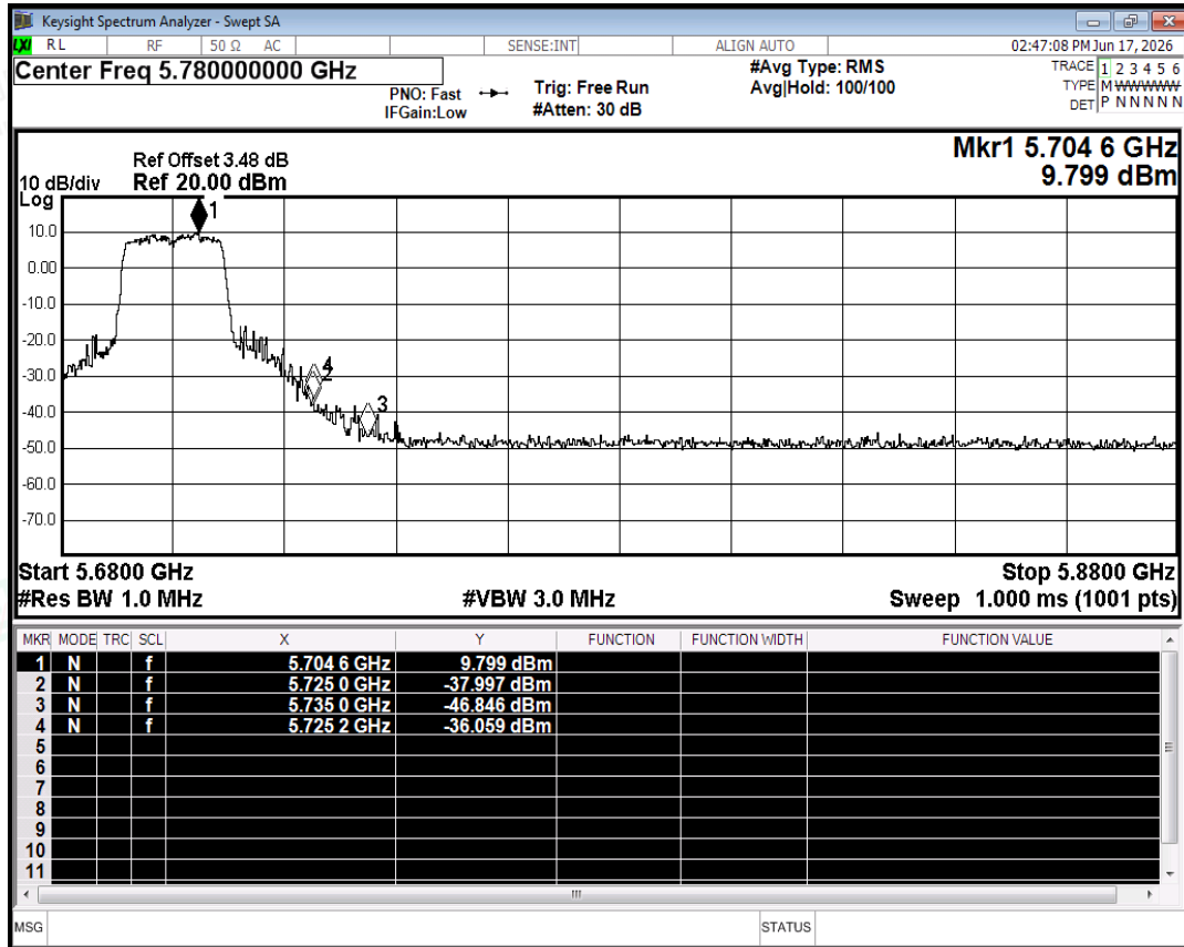
Restrict Band NVNT ac20 5700MHz Ant0 Peak
