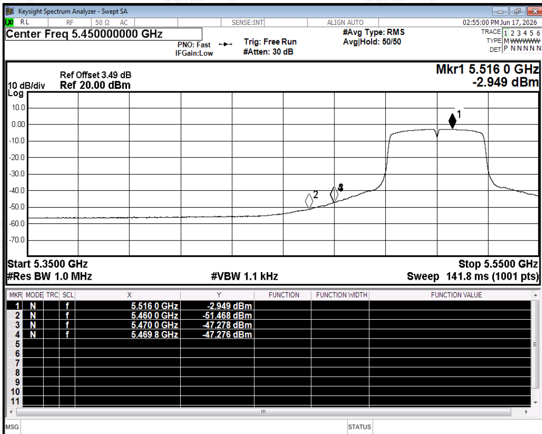
Restrict Band NVNT n40 5510MHz Ant0 Average
