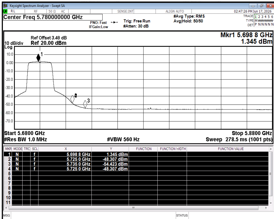
Restrict Band NVNT ac20 5700MHz Ant0 Average
