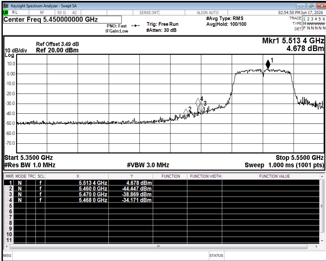
Restrict Band NVNT n40 5510MHz Ant0 Peak
