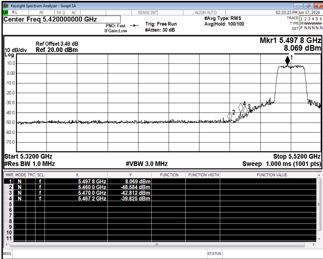
Restrict Band NVNT ac20 5500MHz Ant0 Peak
