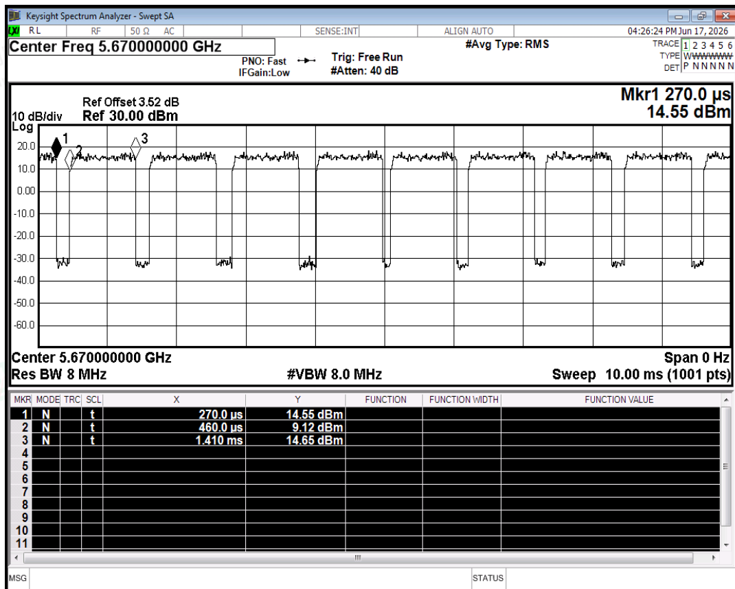
Duty Cycle NVNT ac40 5670MHz Ant0
