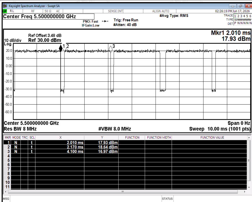
Duty Cycle NVNT ac20 5500MHz Ant0
