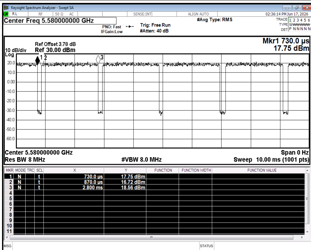
Duty Cycle NVNT ac20 5580MHz Ant0
