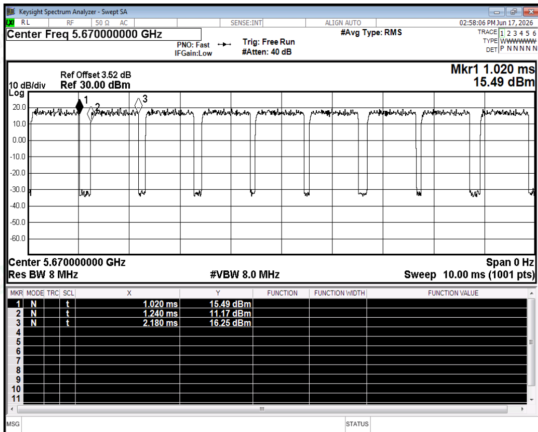
Duty Cycle NVNT n40 5670MHz Ant0
