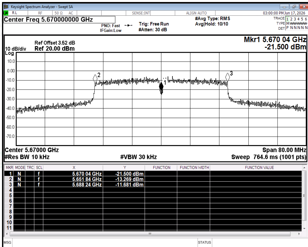
Freq. Stability NVNT n40 5670MHz Ant0
