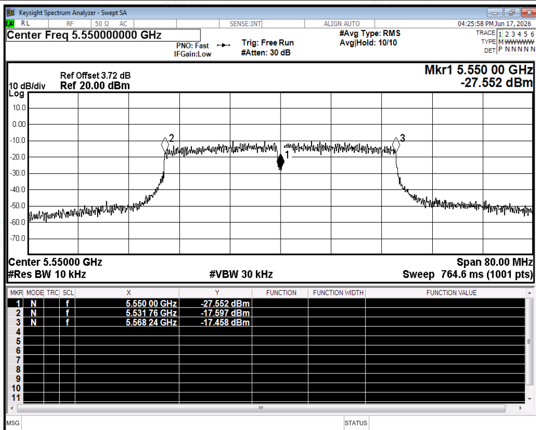
Freq. Stability NVNT ac40 5550MHz Ant0
