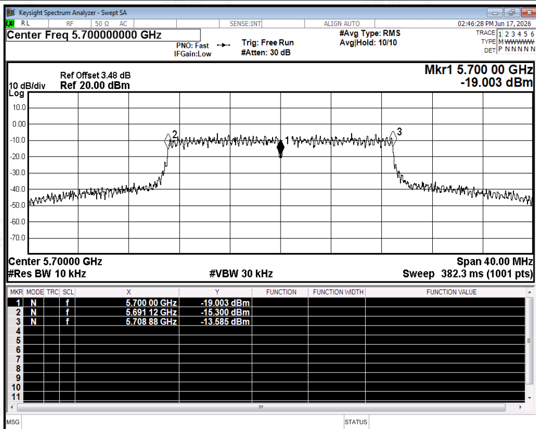
Freq. Stability NVNT ac20 5700MHz Ant0
