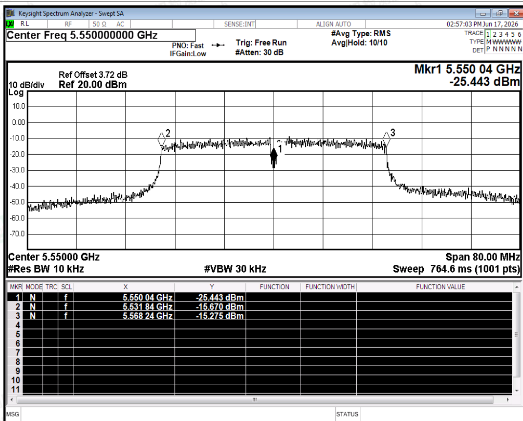
Freq. Stability NVNT n40 5550MHz Ant0
