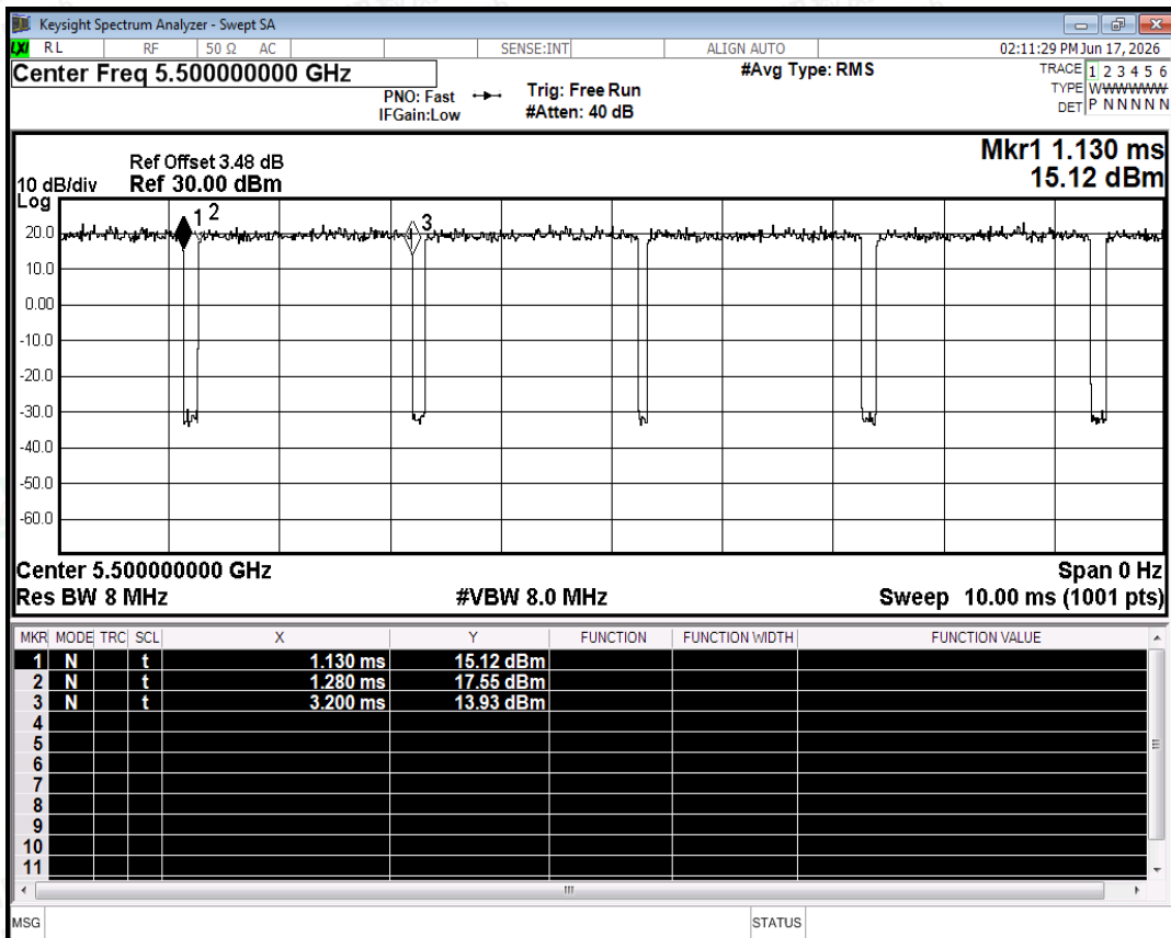
Duty Cycle NVNT n20 5500MHz Ant0
