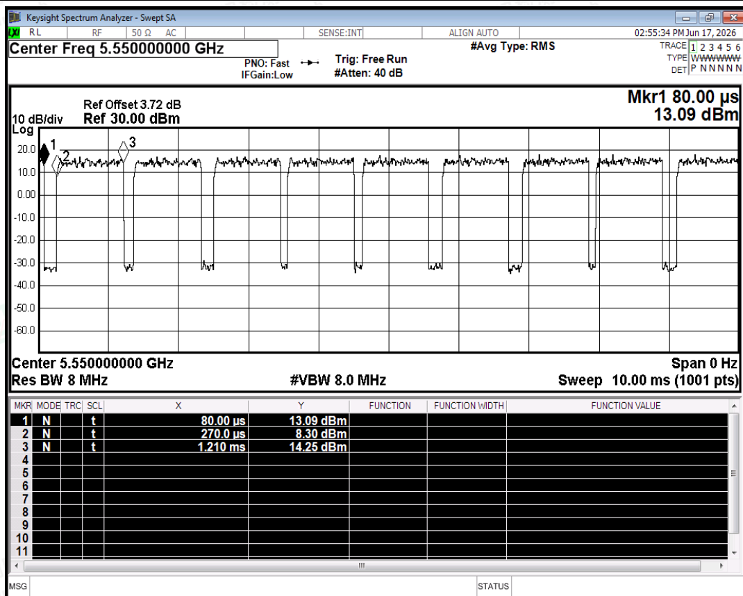
Duty Cycle NVNT n40 5550MHz Ant0
