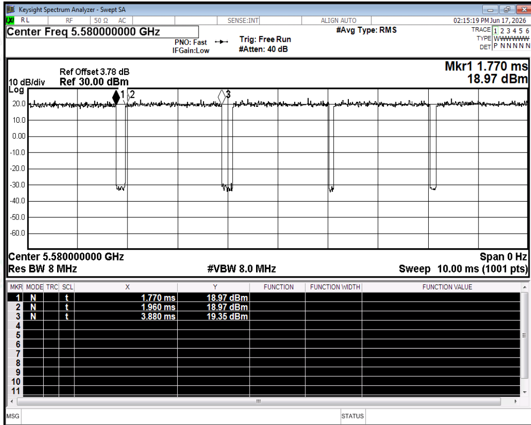
Duty Cycle NVNT n20 5580MHz Ant0
