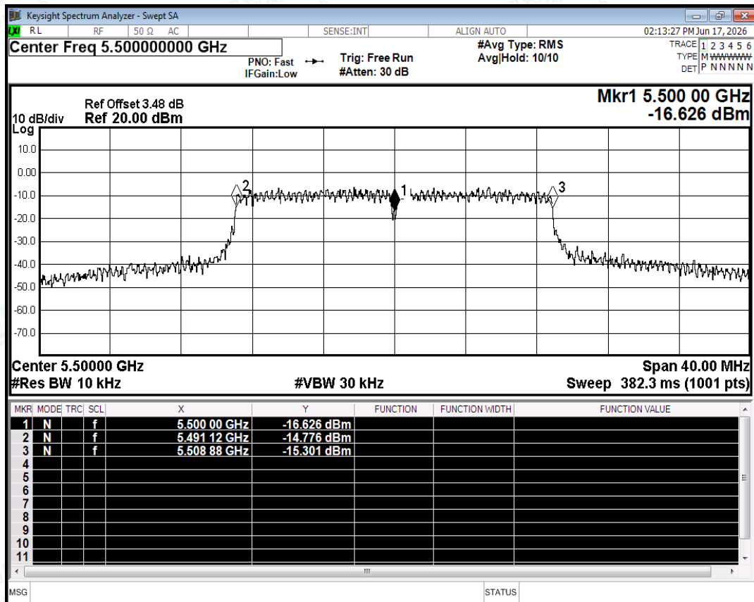
Freq. Stability NVNT n20 5500MHz Ant0
