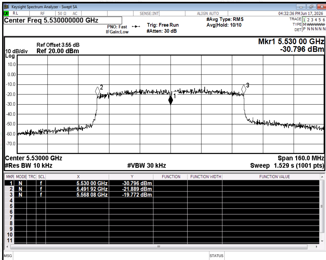
Freq. Stability NVNT ac80 5530MHz Ant0
