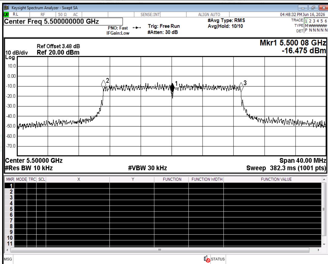
Freq. Stability NVNT ac20 5500MHz Ant1
