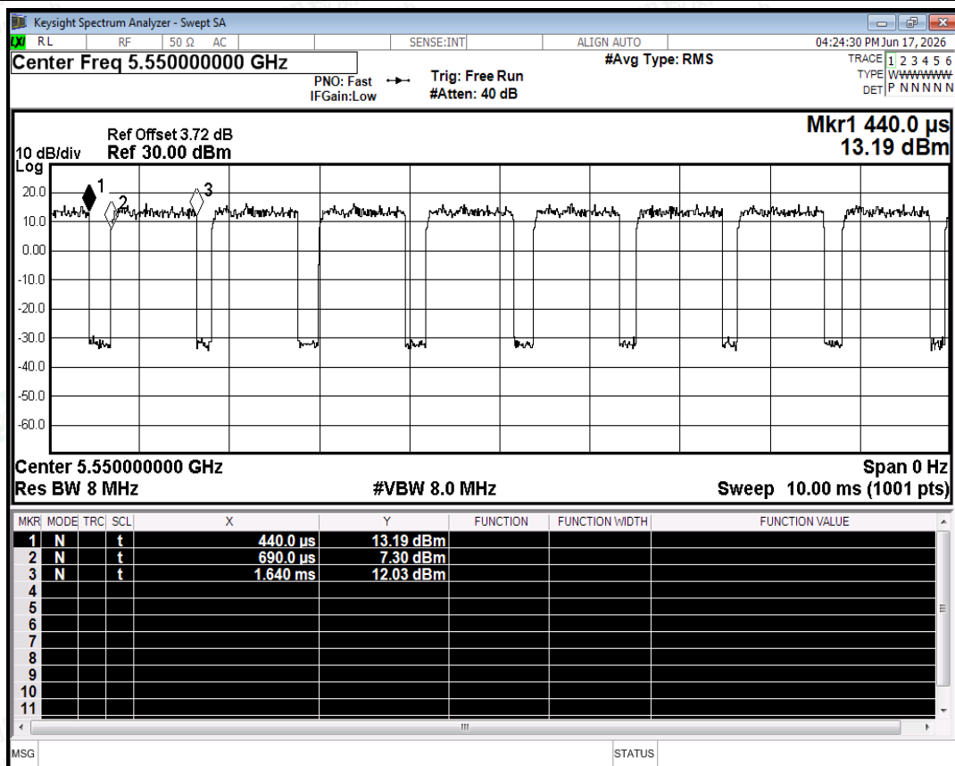
Duty Cycle NVNT ac40 5550MHz Ant0
