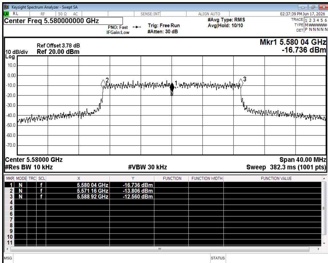
Freq. Stability NVNT ac20 5580MHz Ant0
