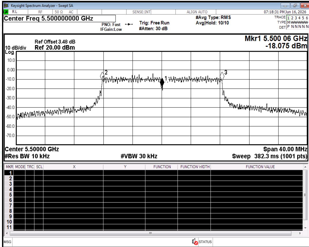
Freq. Stability NVNT a 5500MHz Ant0
