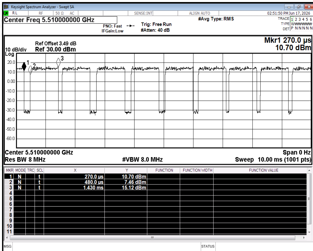
Duty Cycle NVNT n40 5510MHz Ant0
