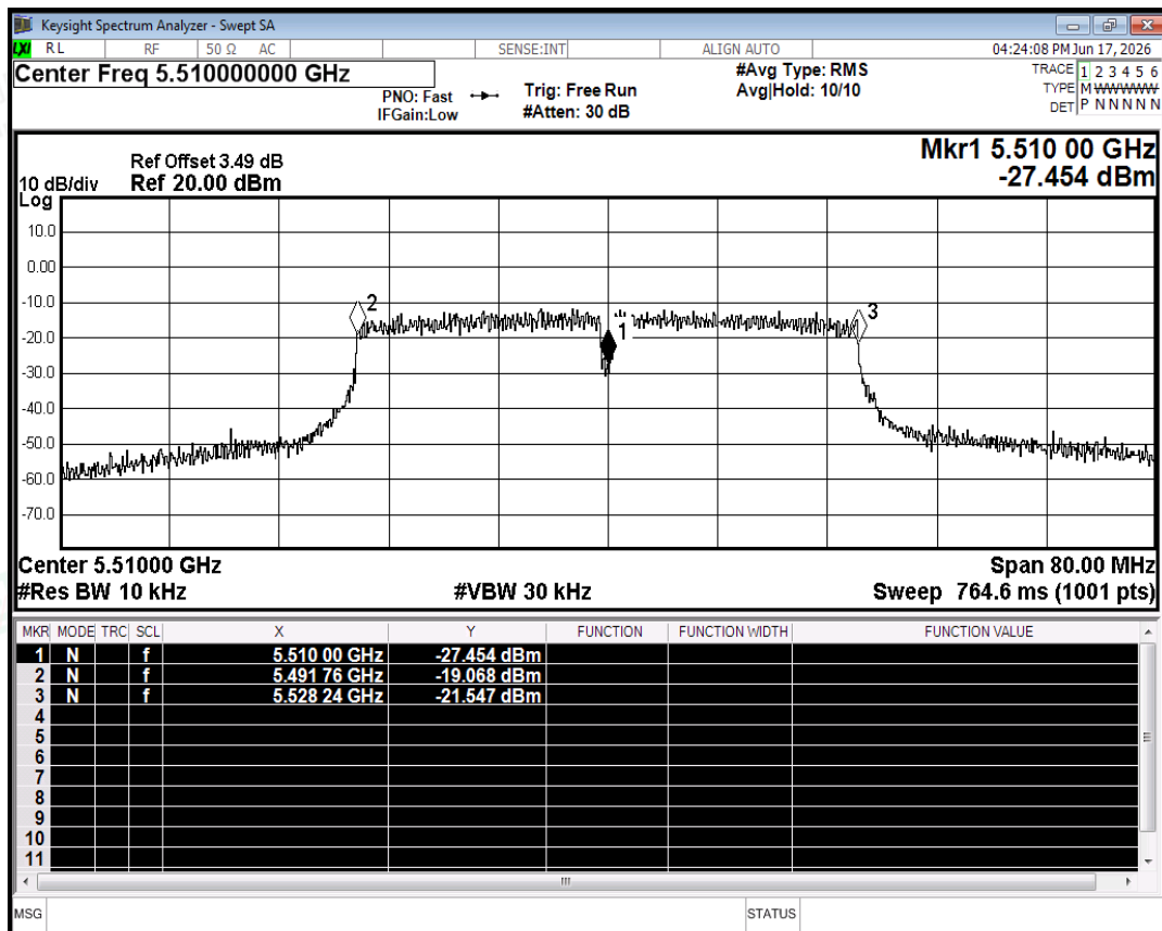
Freq. Stability NVNT ac40 5510MHz Ant0
