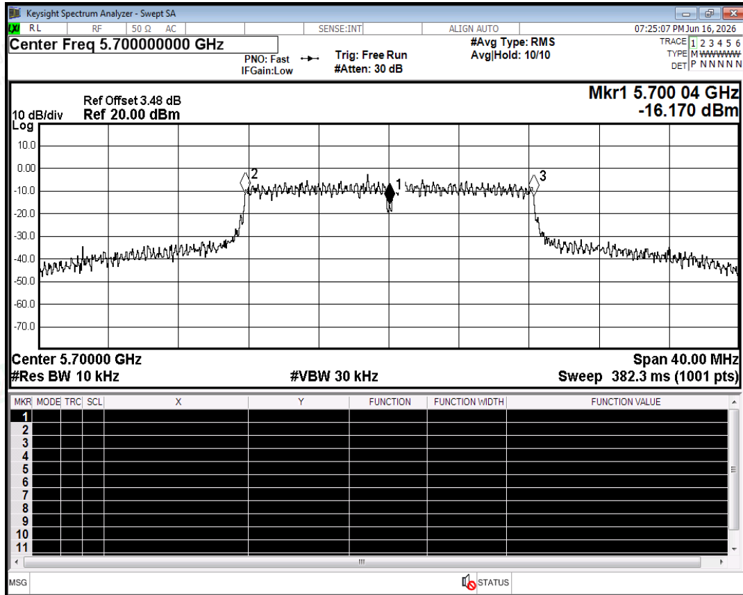
Freq. Stability NVNT a 5700MHz Ant0
