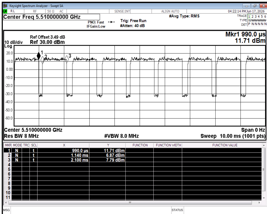
Duty Cycle NVNT ac40 5510MHz Ant0
