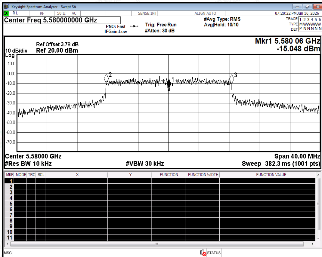
Freq. Stability NVNT a 5580MHz Ant0
