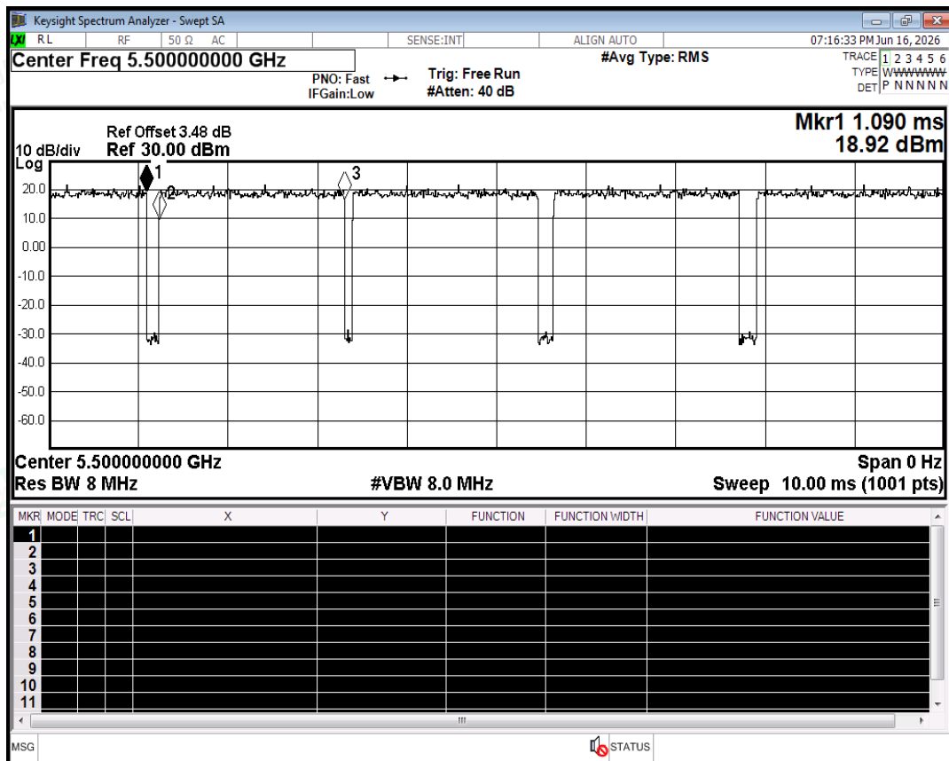
Duty Cycle NVNT a 5500MHz Ant0
