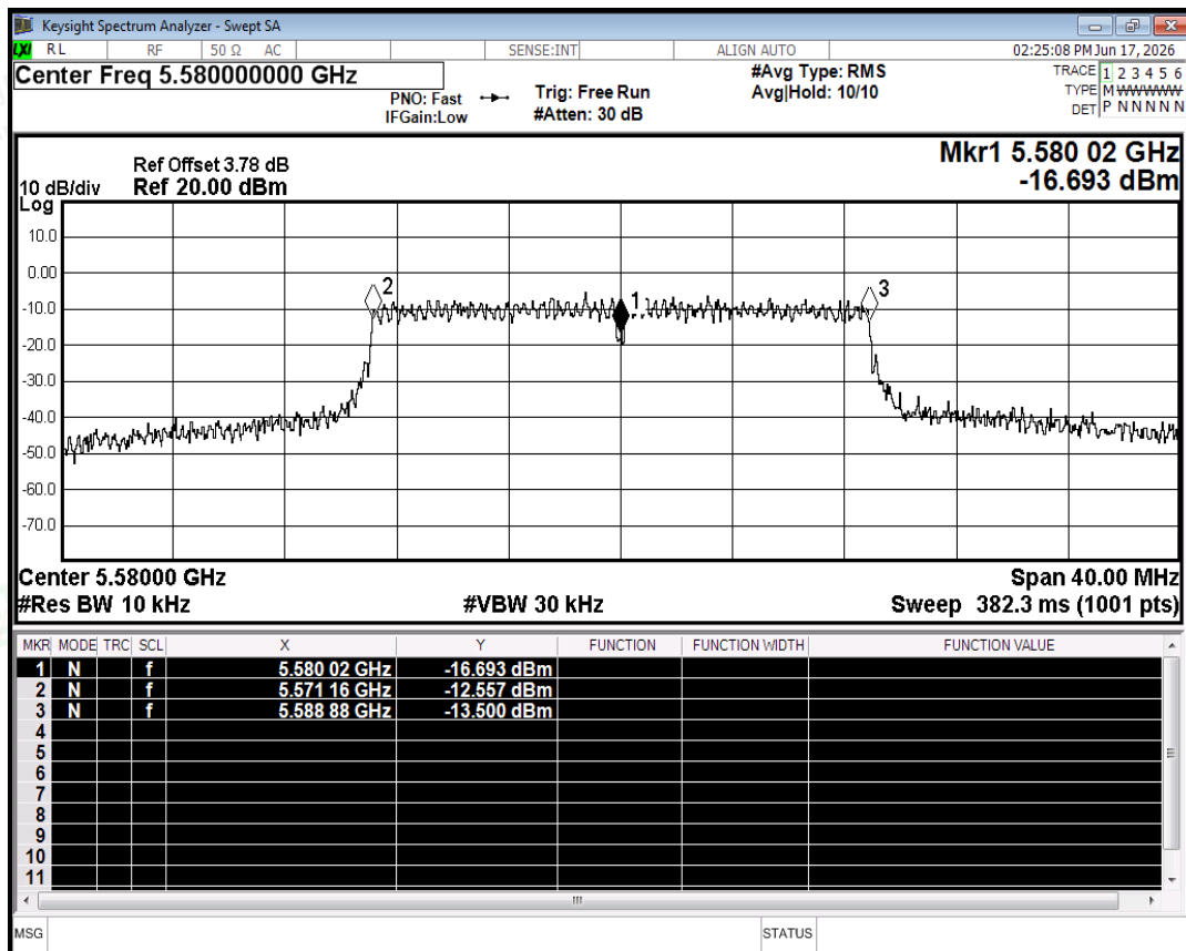
Freq. Stability NVNT n20 5580MHz Ant0
