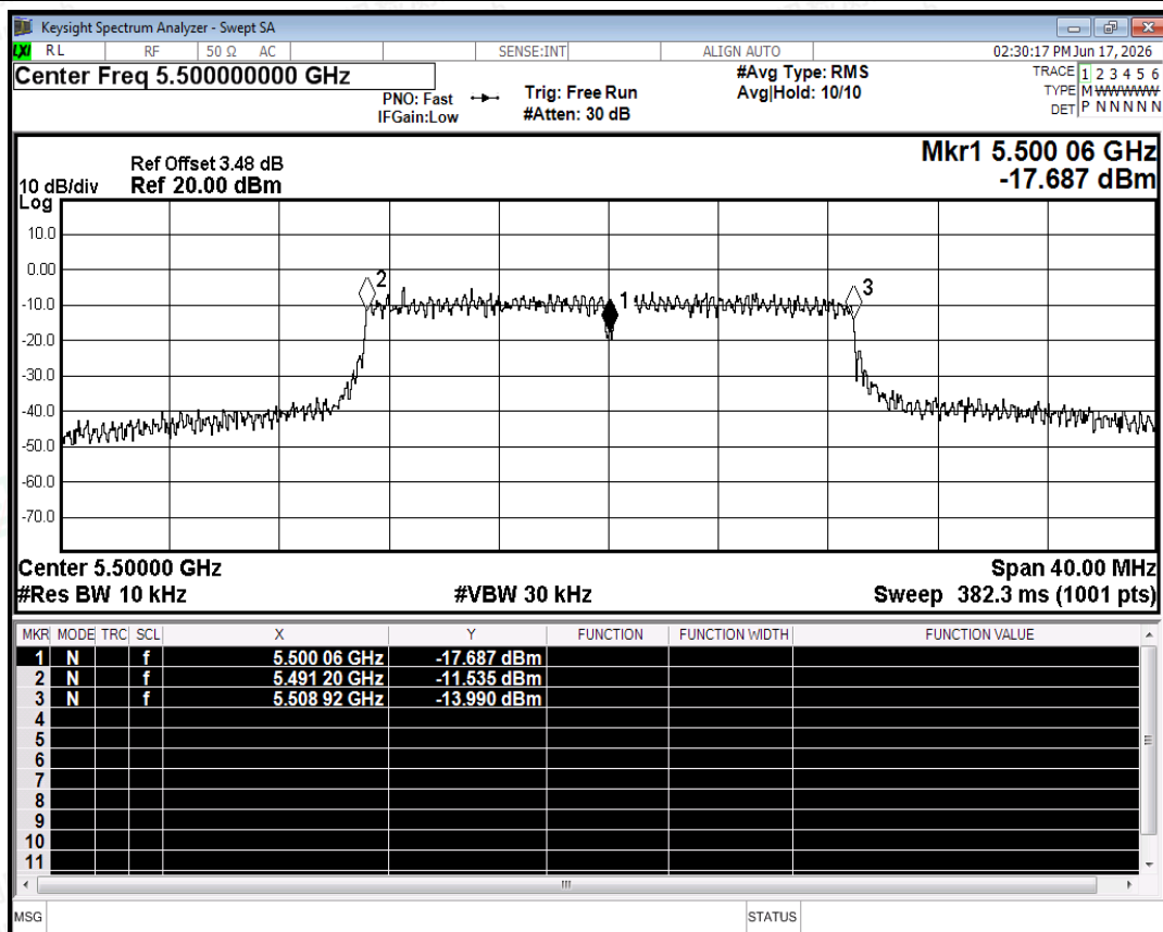
Freq. Stability NVNT ac20 5500MHz Ant0
