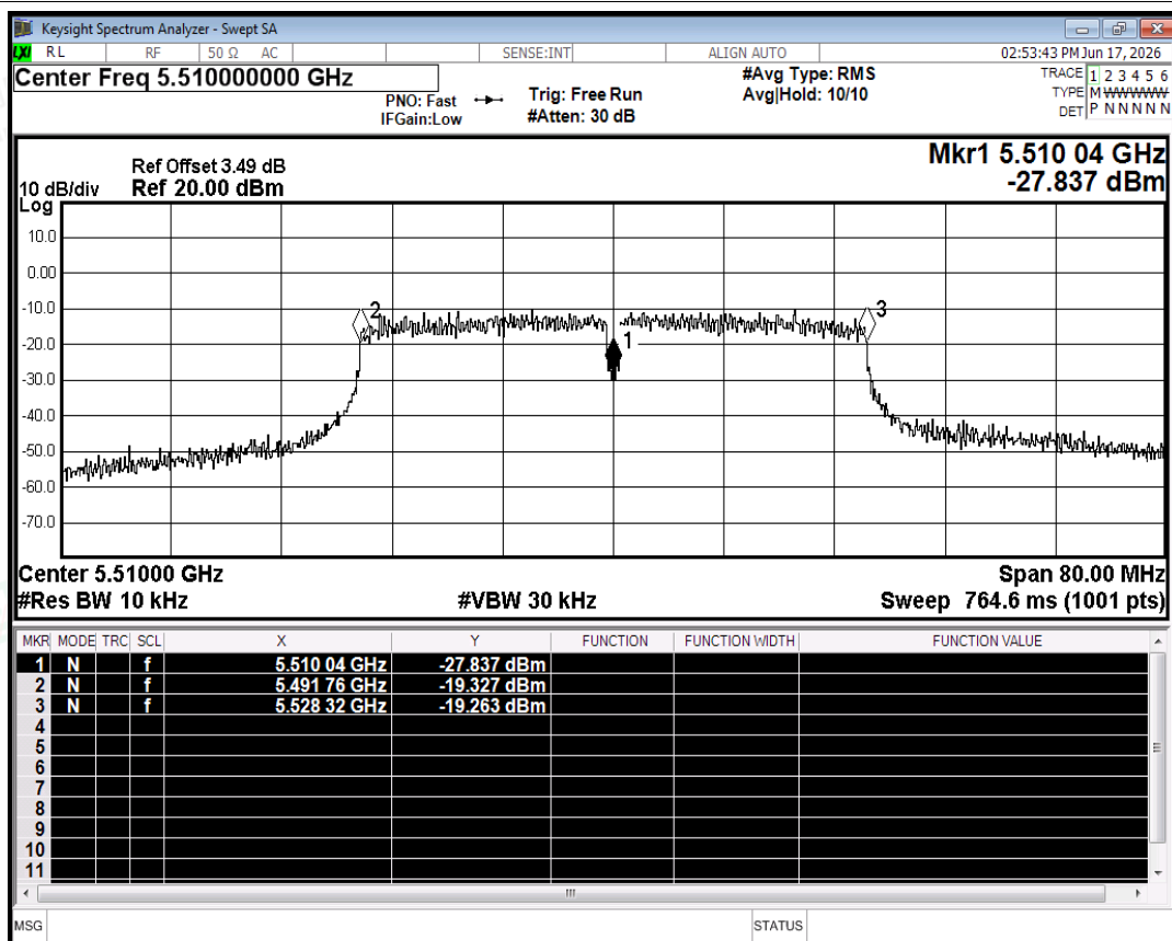
Freq. Stability NVNT n40 5510MHz Ant0
