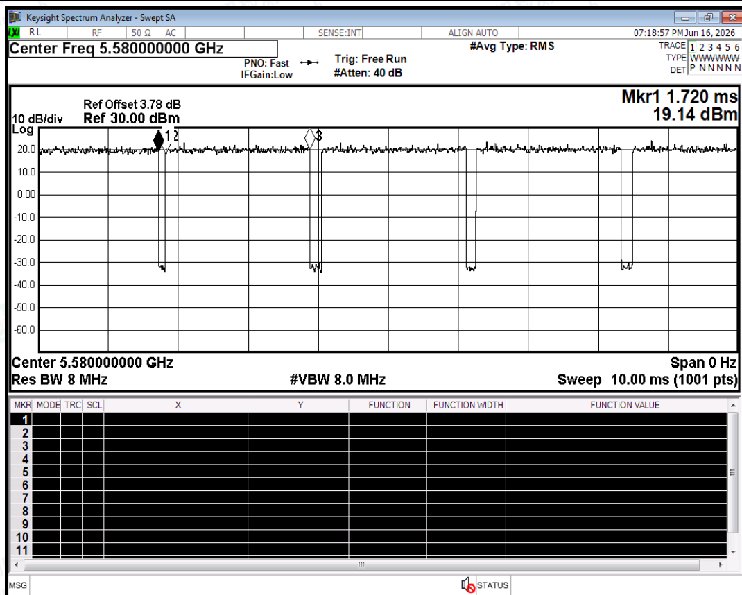
Duty Cycle NVNT a 5580MHz Ant0
