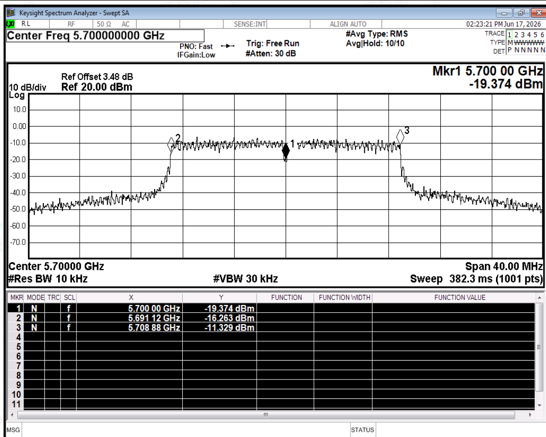
Freq. Stability NVNT n20 5700MHz Ant0
