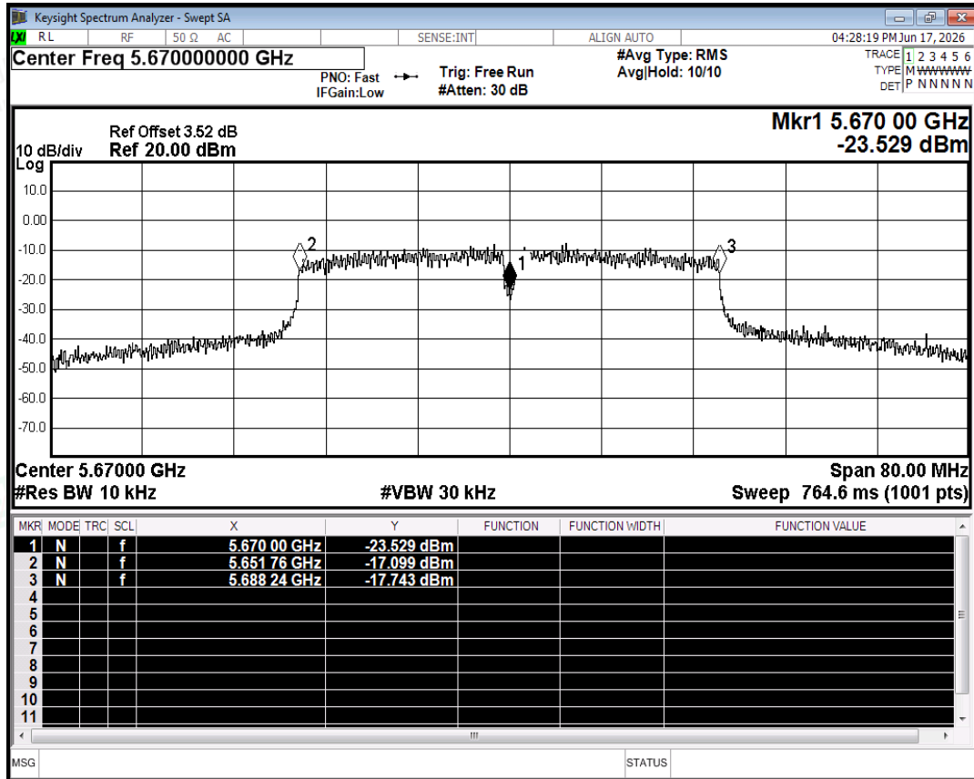
Freq. Stability NVNT ac40 5670MHz Ant0
