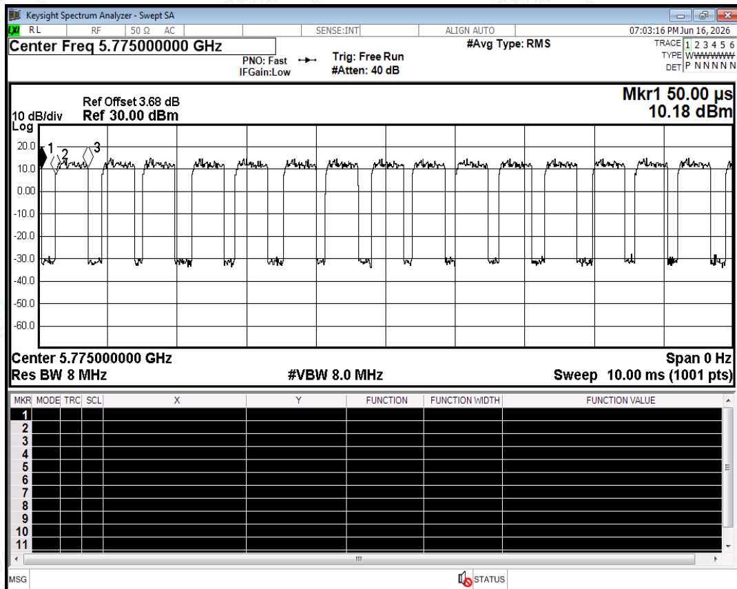
Duty Cycle NVNT ac80 5775MHz Ant0
