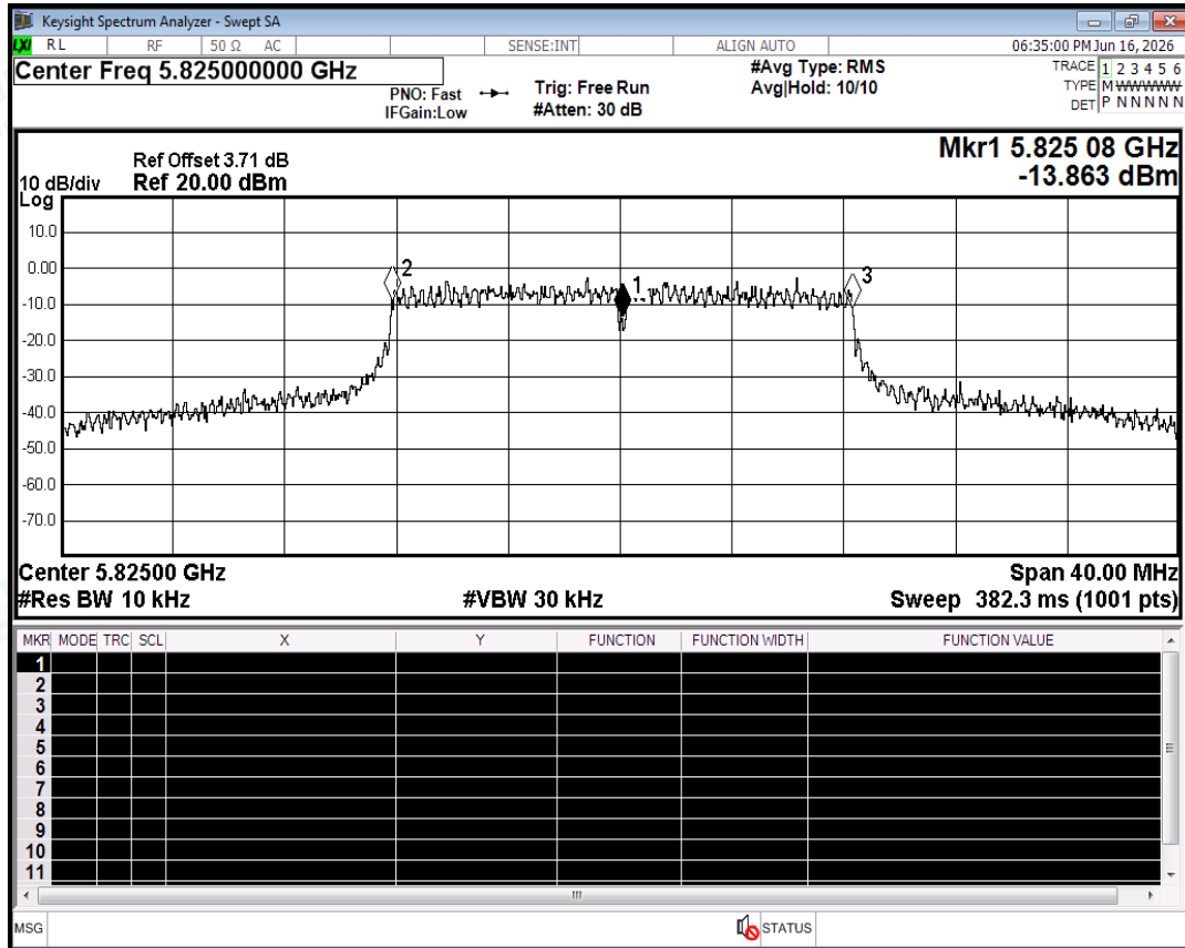
Freq. Stability NVNT a 5825MHz Ant0
