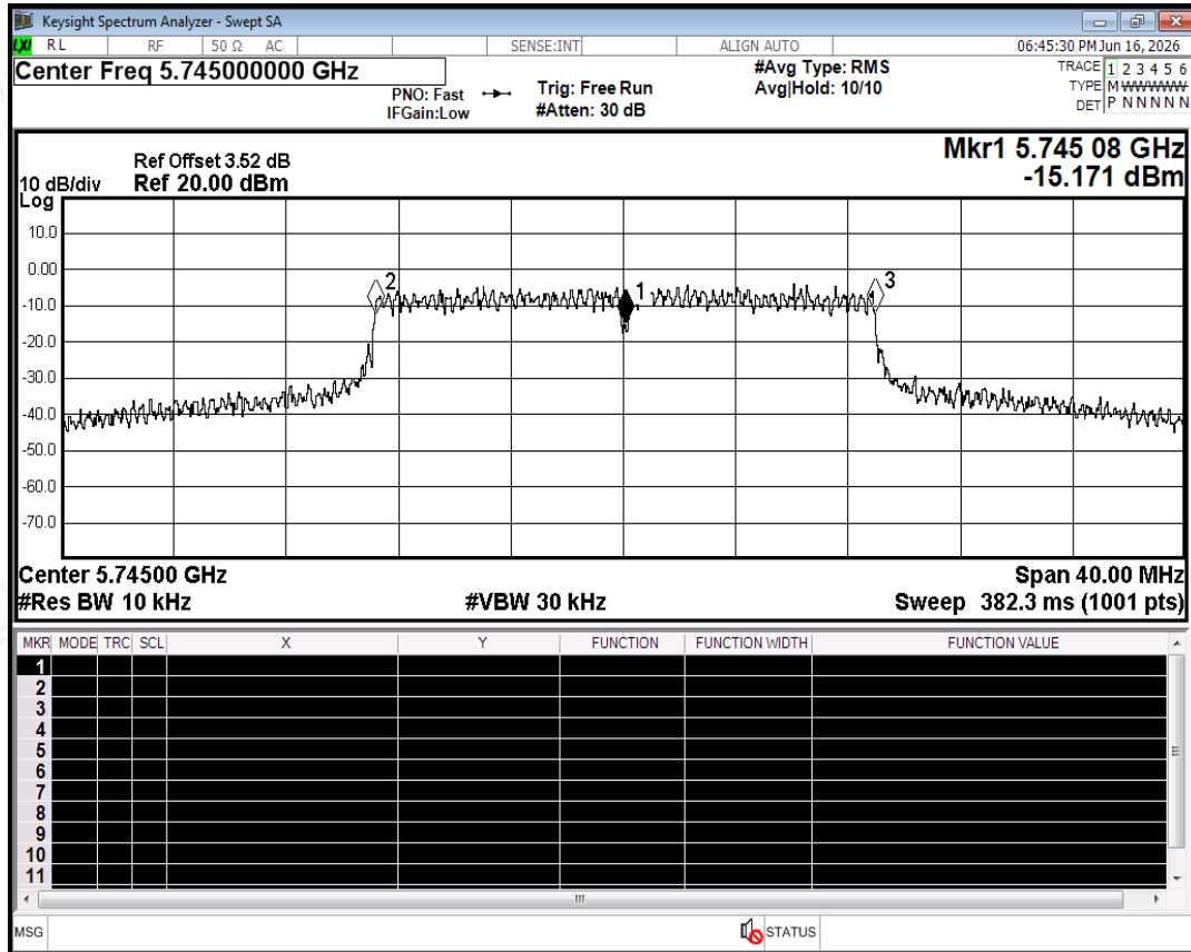
Freq. Stability NVNT ac20 5745MHz Ant0
