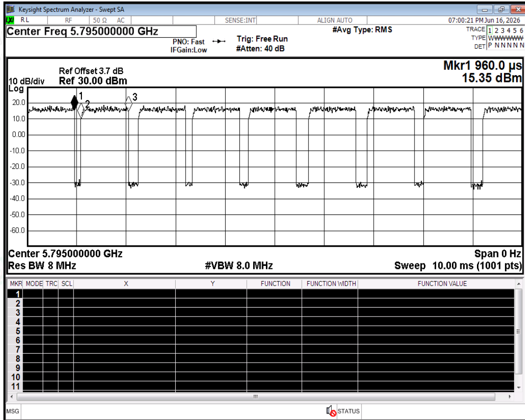
Duty Cycle NVNT ac40 5795MHz Ant0
