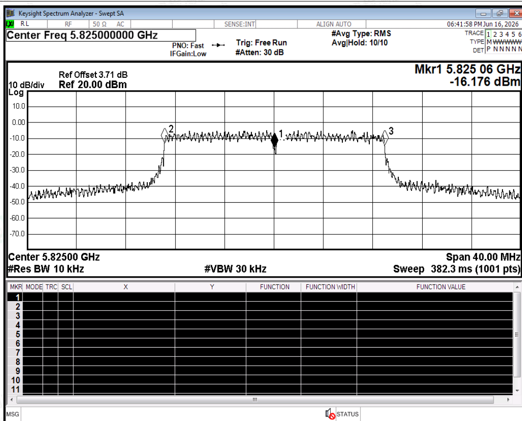
Freq. Stability NVNT n20 5825MHz Ant0
