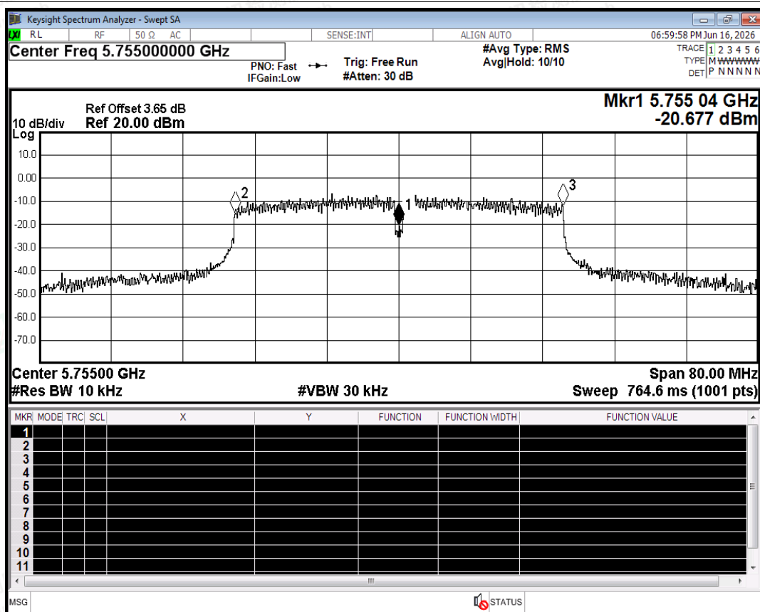
Freq. Stability NVNT ac40 5755MHz Ant0
