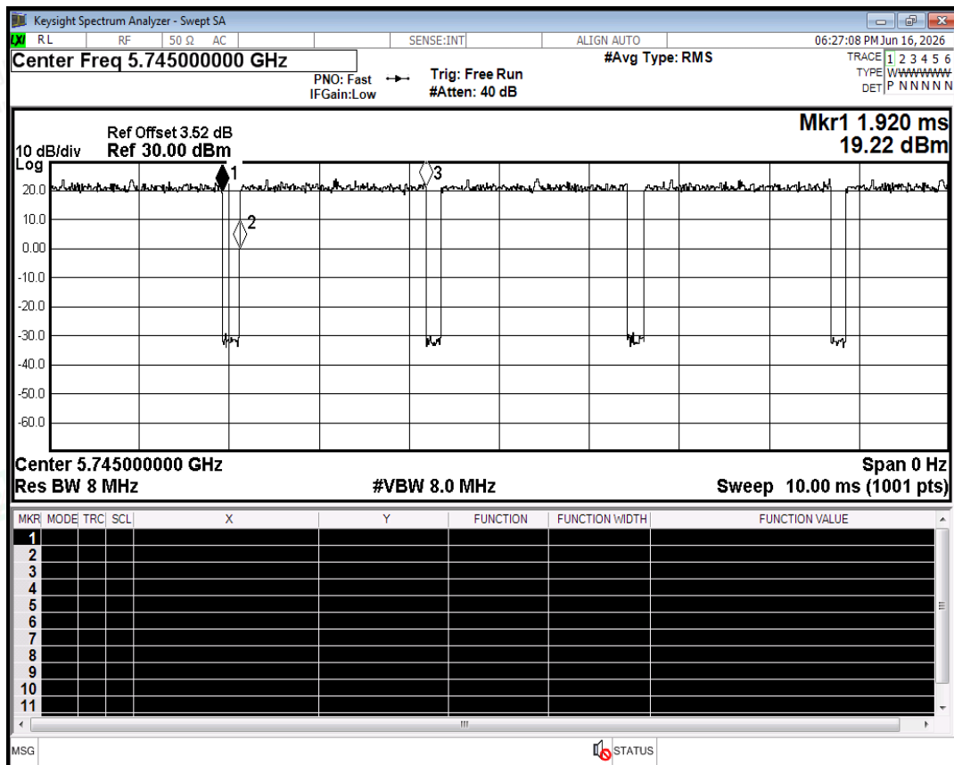
Duty Cycle NVNT a 5745MHz Ant0
