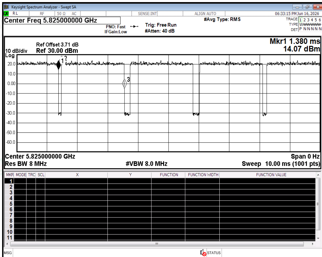
Duty Cycle NVNT a 5825MHz Ant0
