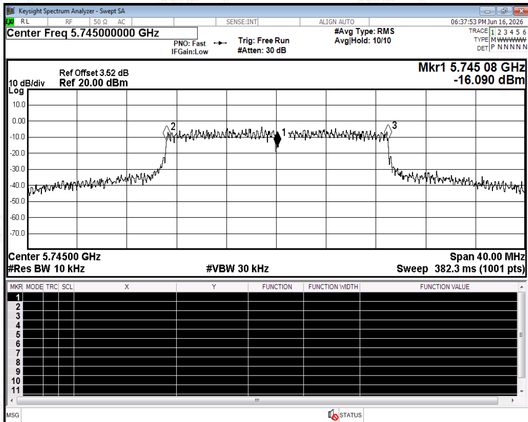
Freq. Stability NVNT n20 5745MHz Ant0
