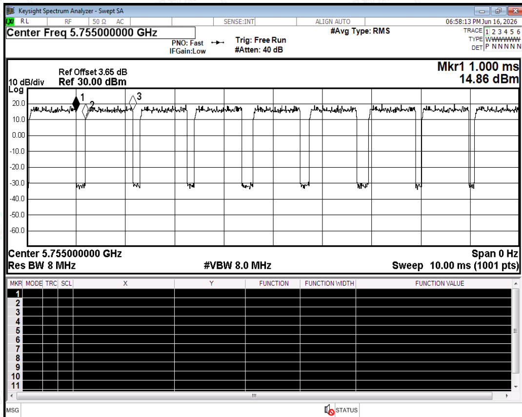
Duty Cycle NVNT ac40 5755MHz Ant0
