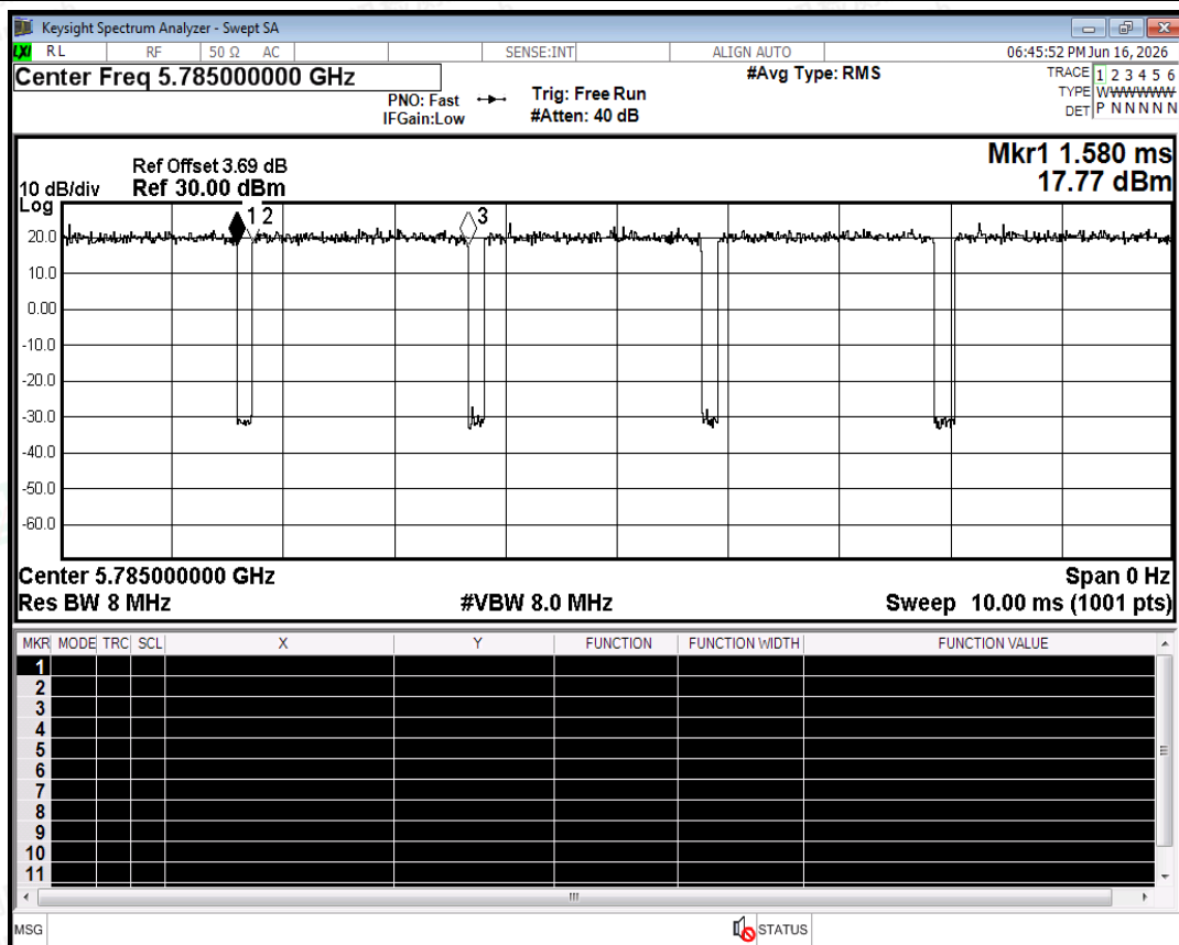
Duty Cycle NVNT ac20 5785MHz Ant0
