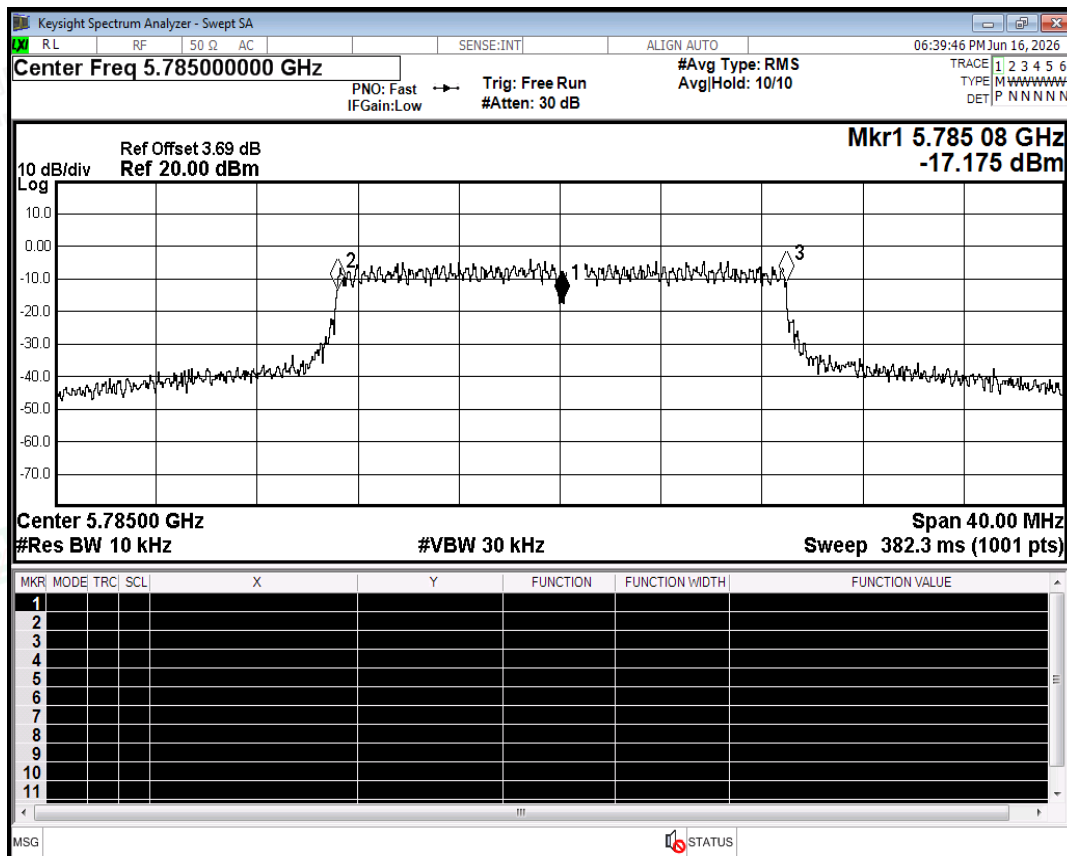
Freq. Stability NVNT n20 5785MHz Ant0
