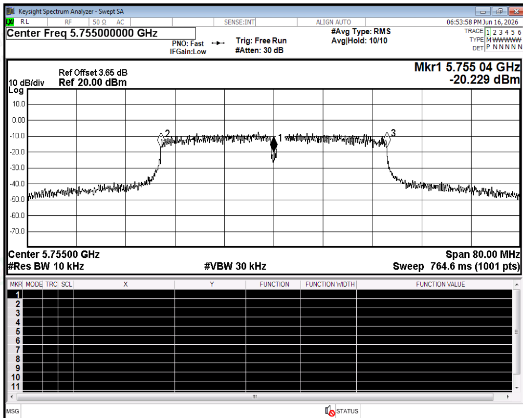
Freq. Stability NVNT n40 5755MHz Ant0
