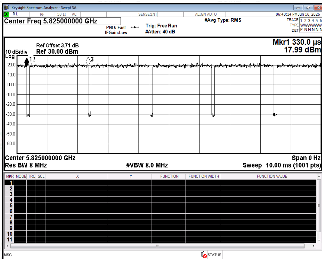
Duty Cycle NVNT n20 5825MHz Ant0
