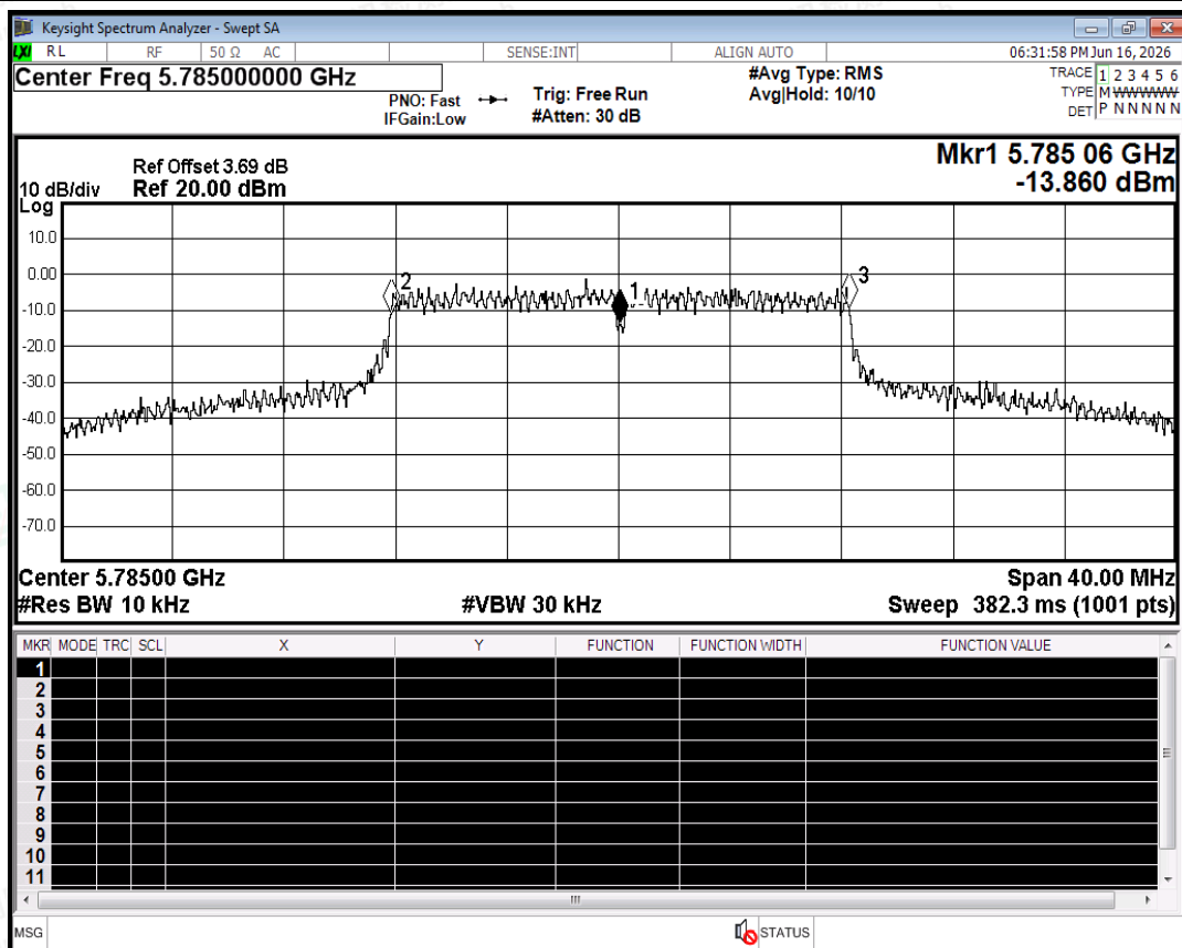
Freq. Stability NVNT a 5785MHz Ant0
