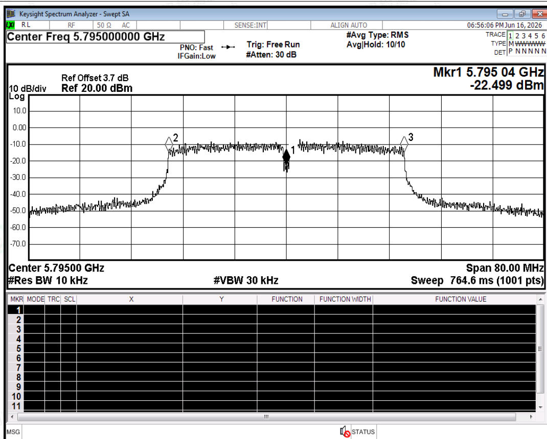
Freq. Stability NVNT n40 5795MHz Ant0
