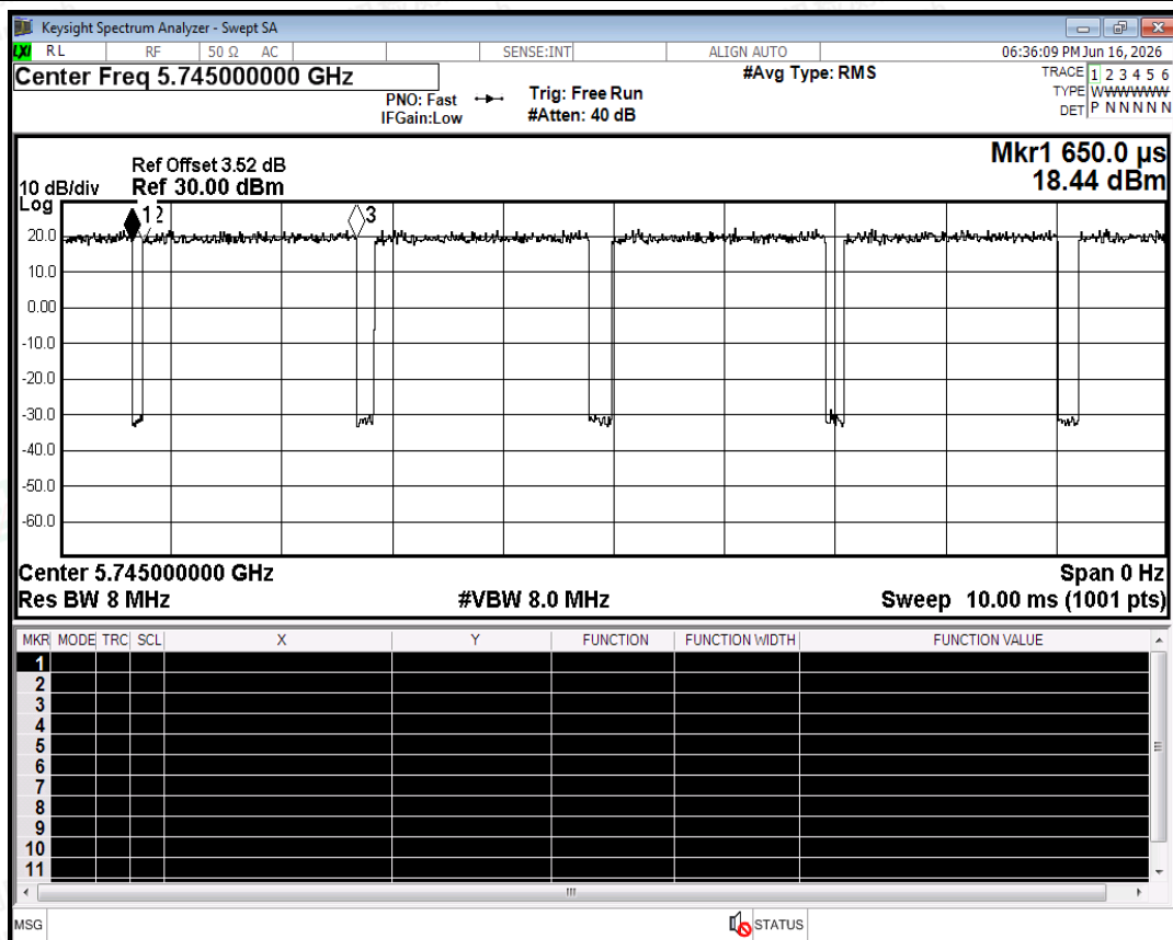
Duty Cycle NVNT n20 5745MHz Ant0
