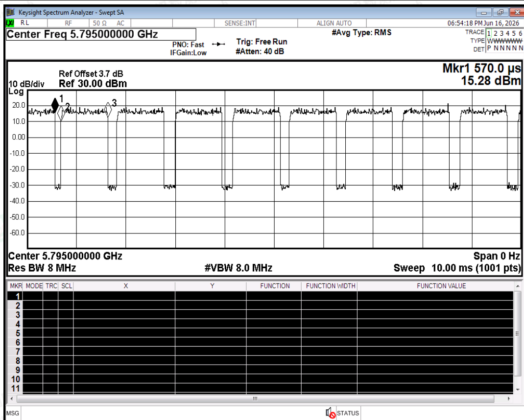
Duty Cycle NVNT n40 5795MHz Ant0
