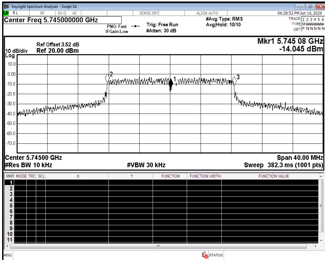
Freq. Stability NVNT a 5745MHz Ant0
