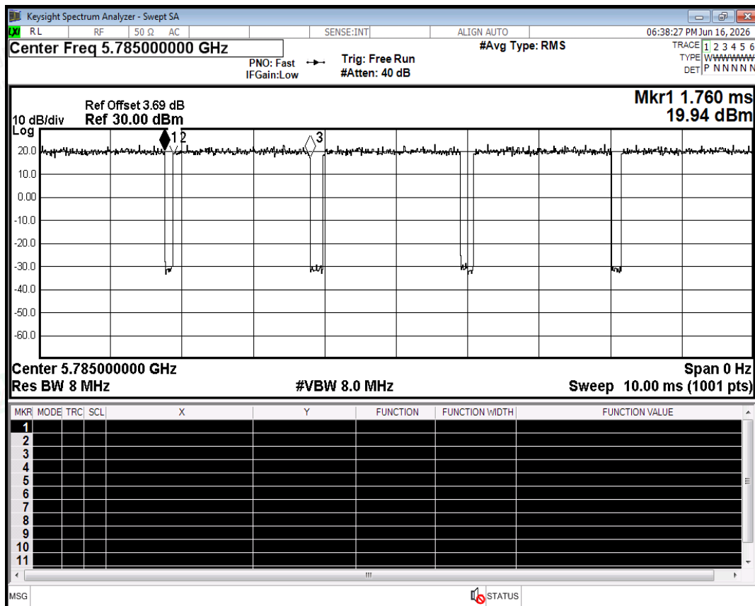
Duty Cycle NVNT n20 5785MHz Ant0
