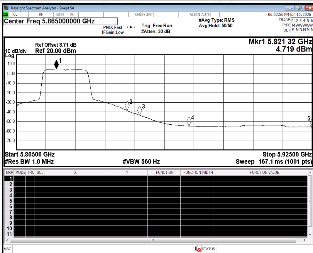
Restrict Band NVNT ac20 5825MHz Ant1 Average
