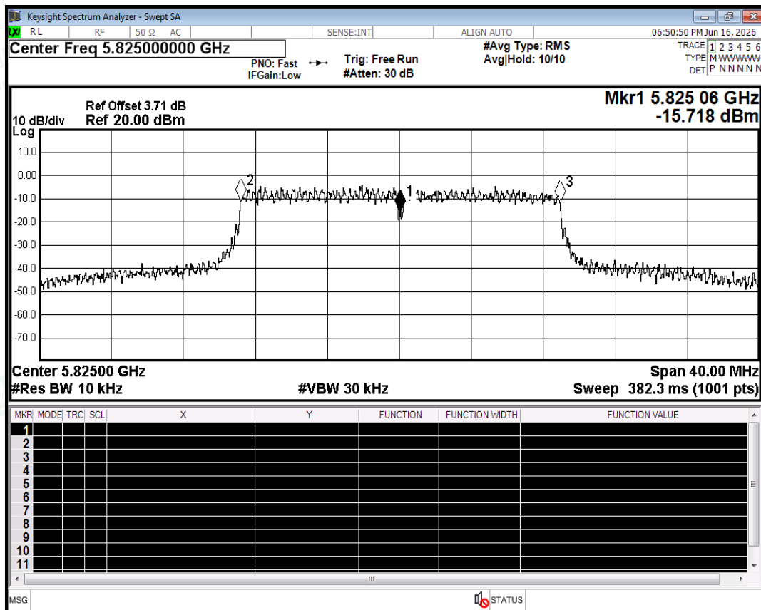
Freq. Stability NVNT ac20 5825MHz Ant0
