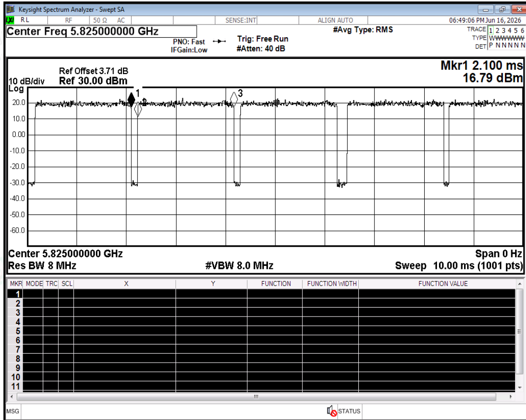
Duty Cycle NVNT ac20 5825MHz Ant0
