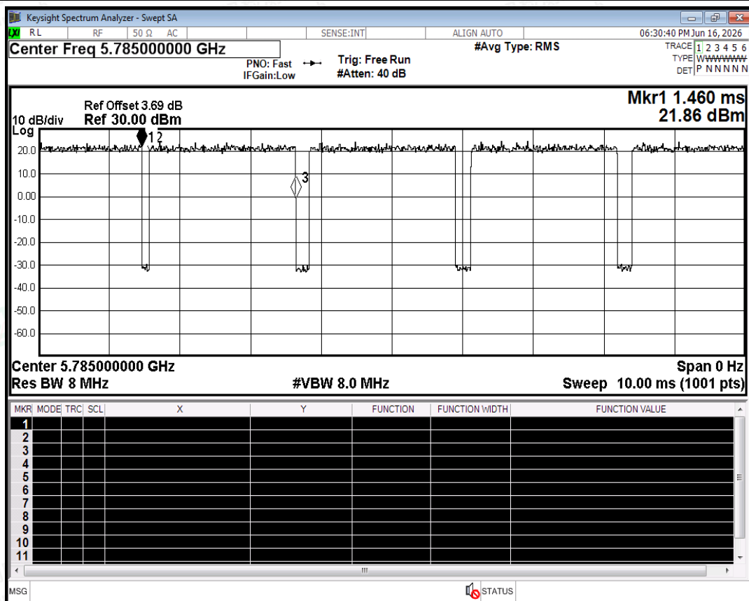
Duty Cycle NVNT a 5785MHz Ant0
