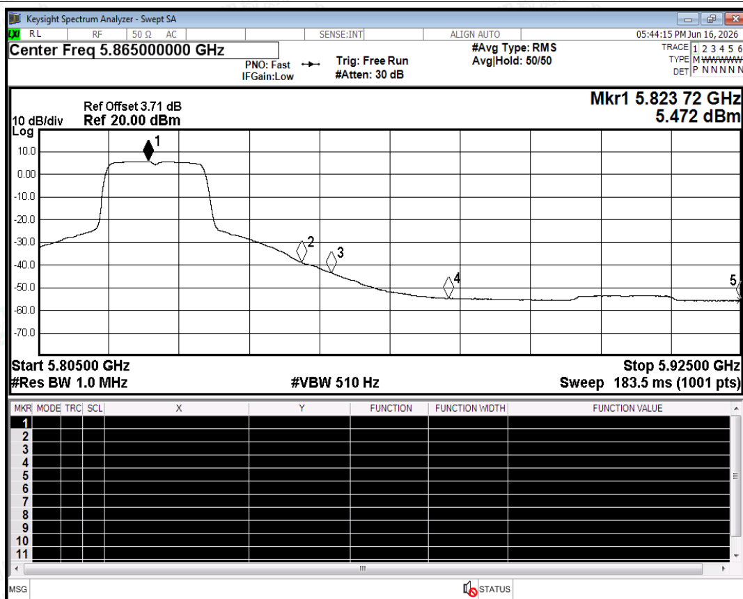
Restrict Band NVNT a 5825MHz Ant1 Average
