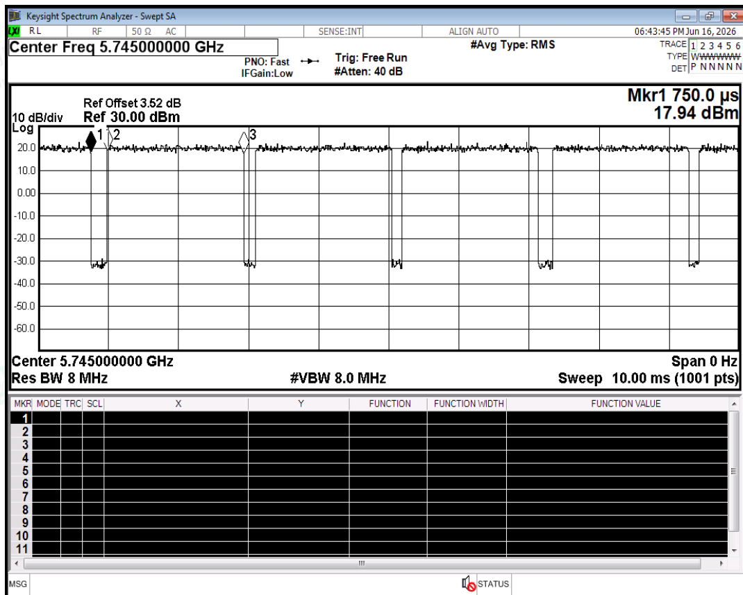
Duty Cycle NVNT ac20 5745MHz Ant0
