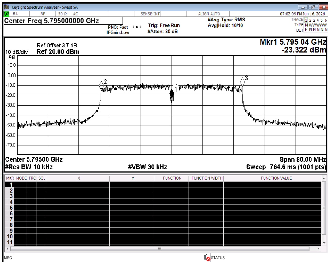
Freq. Stability NVNT ac40 5795MHz Ant0
