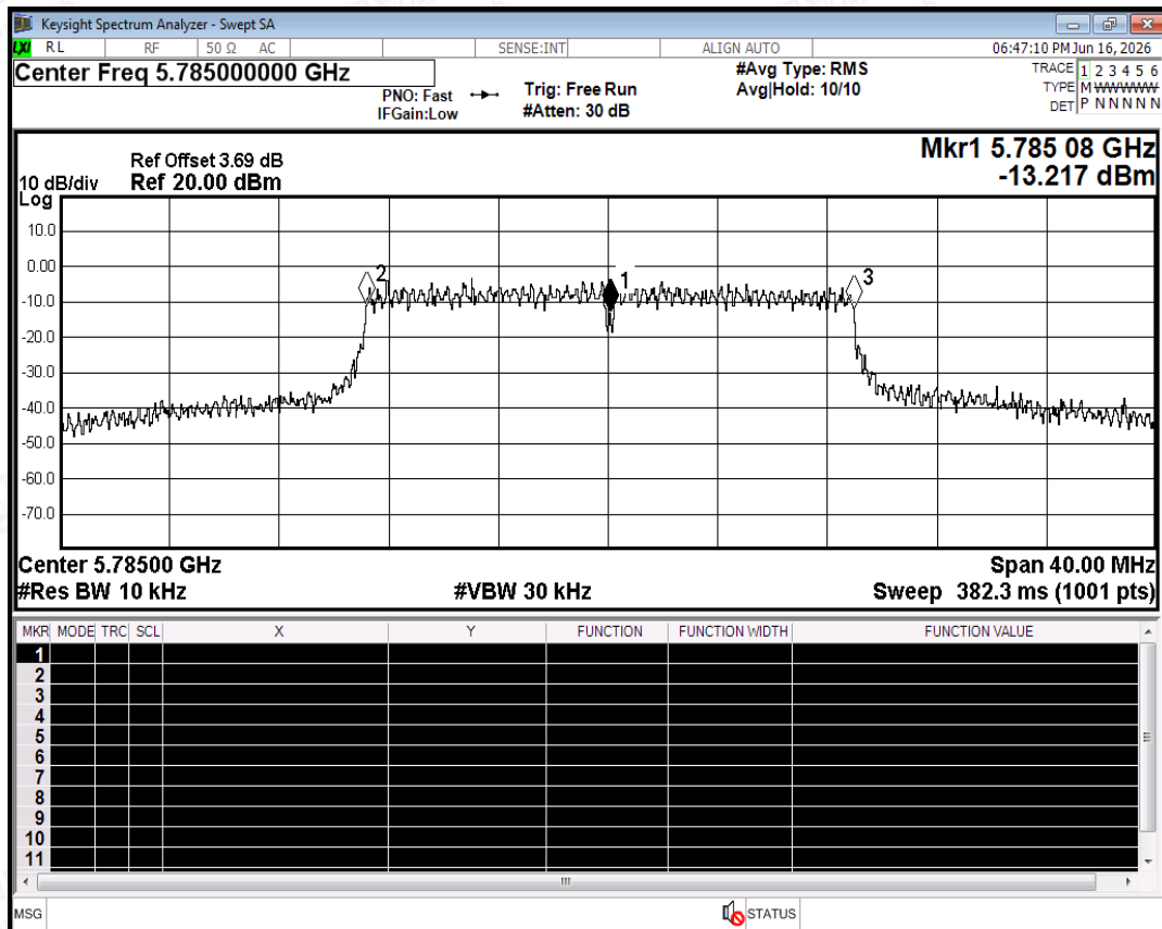
Freq. Stability NVNT ac20 5785MHz Ant0
