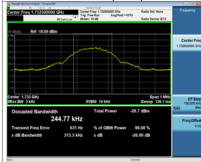
AWS-1 band Uplink Input
