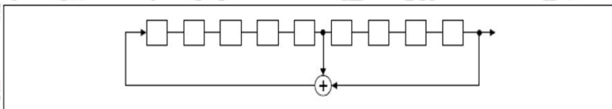
Linear Feedback Shift Register for Generation of the PRBS sequence
