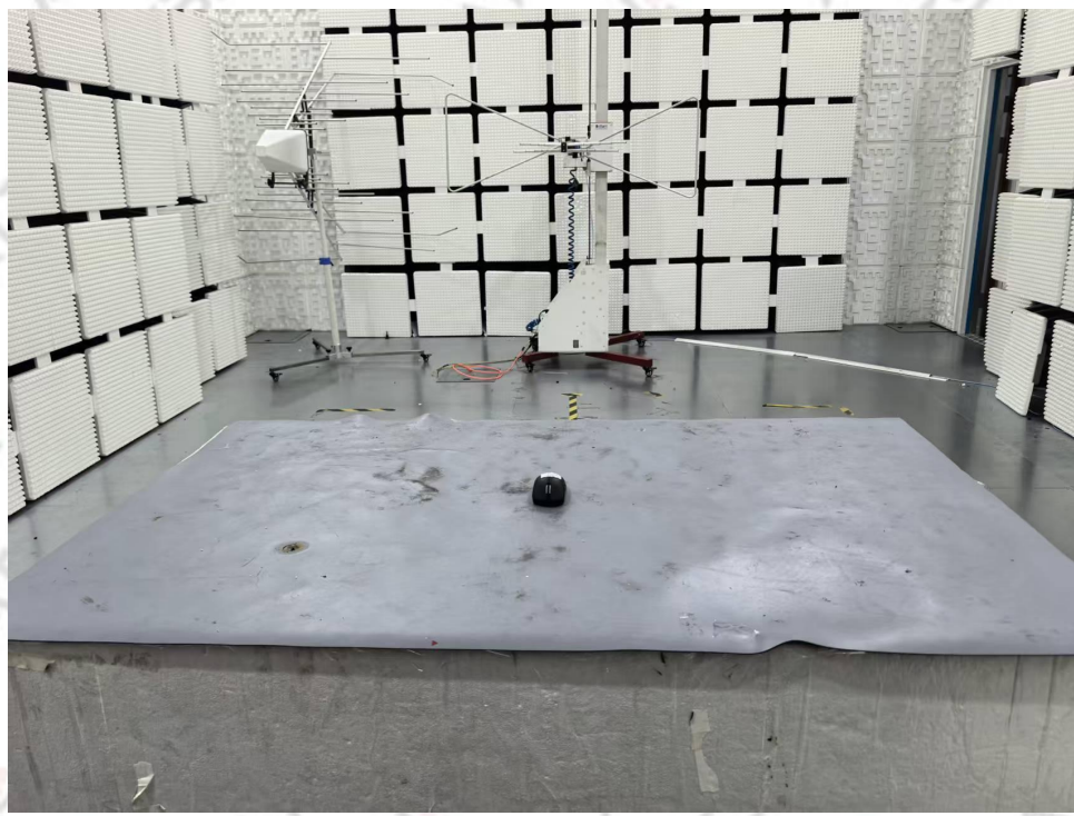
Below 1GHz
