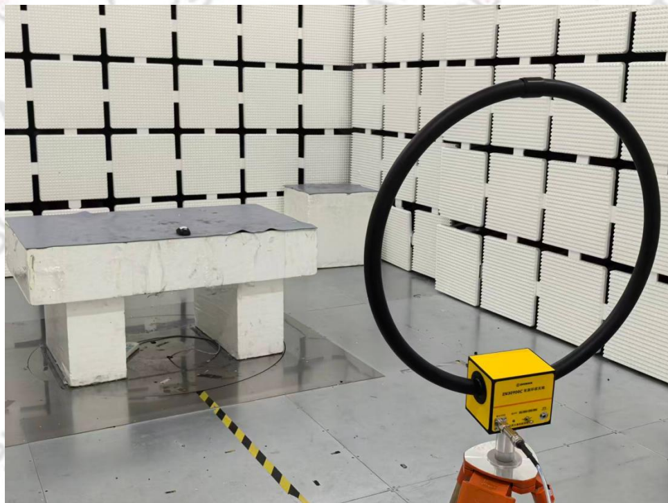
Below 1GHz
