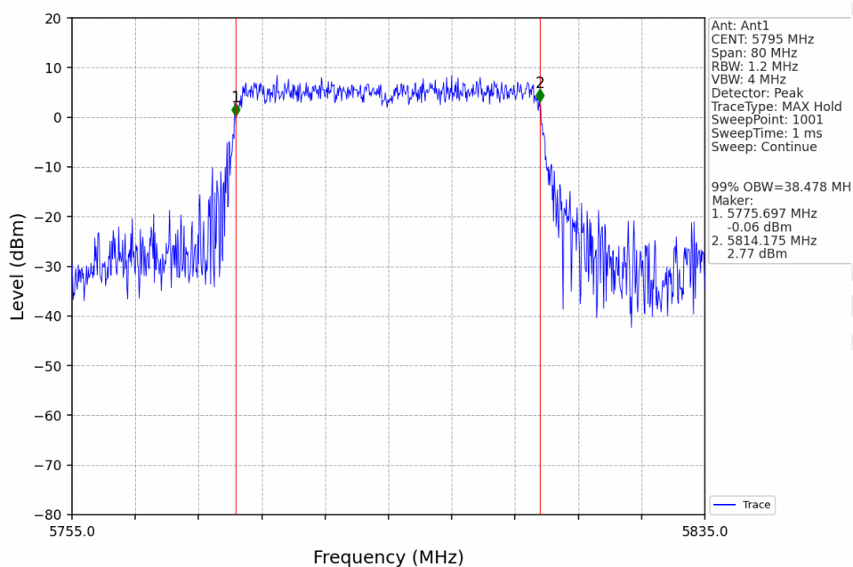
802.11ax(HEW40) HCH 5795MHz FU / Ant1 NTNV
