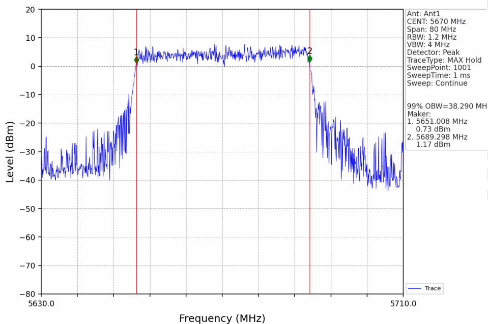
802.11ax(HEW40) HCH 5670MHz FU / Ant1 NTN
