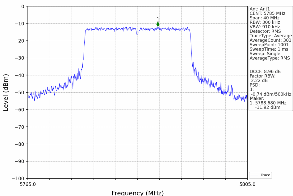
802.11ax(HEW20) MCH 5785MHz FU / Ant1 NTV
