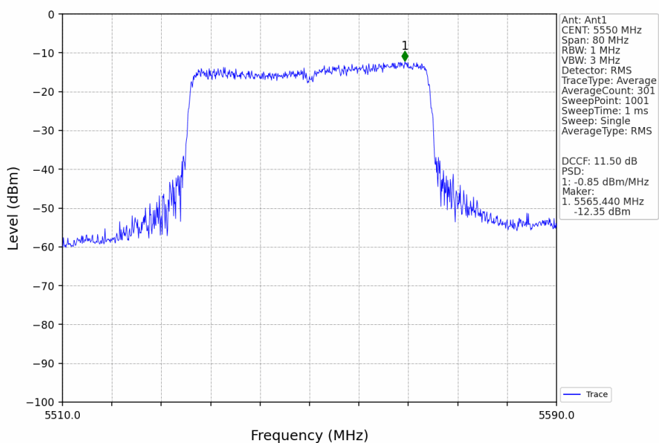
802.11ax(HEW40) MCH 5550MHz FU / Ant1 NTV
