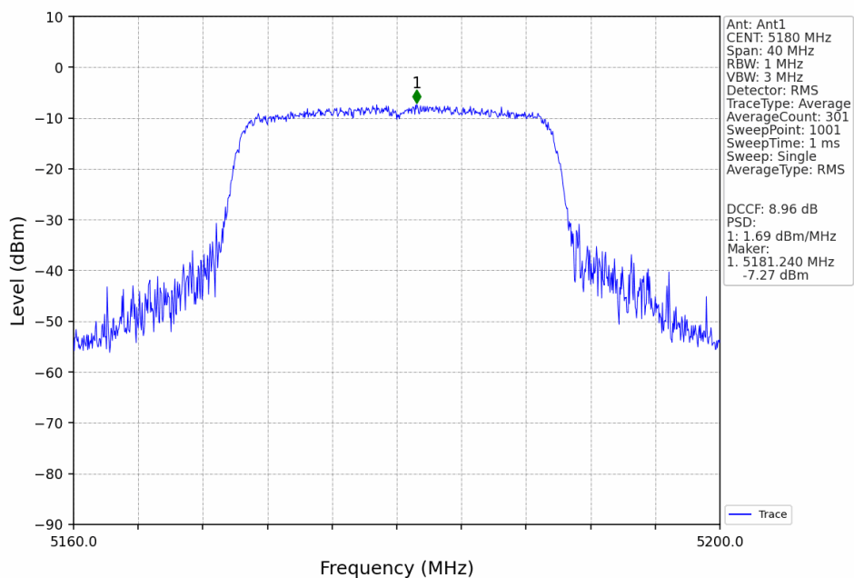
802.11ax(HEW20) LCH 5180MHz FU / Ant1 NTN
