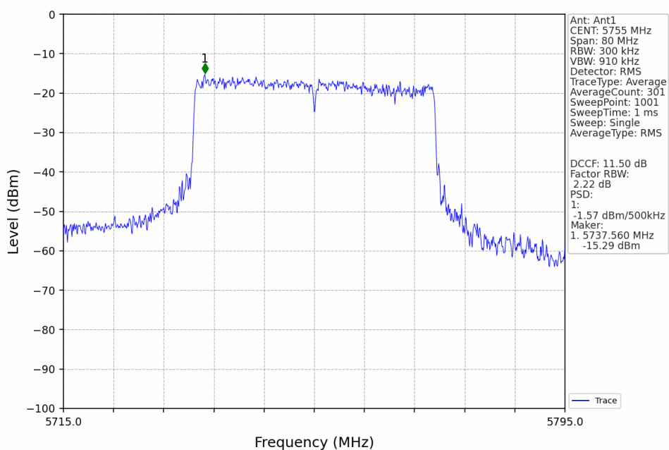
802.11ax(HEW40) LCH 5755MHz FU / Ant1 NTV
