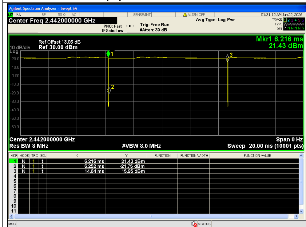
Duty Cycle NVNT b 2442MHz Ant1
