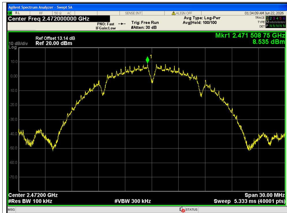
Tx. Spurious NVNT b 2472MHz Ant1 Ref
