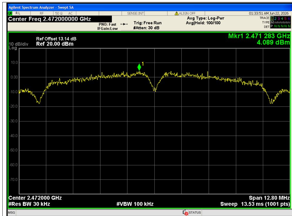
PSD NVNT b 2472MHz Ant1
