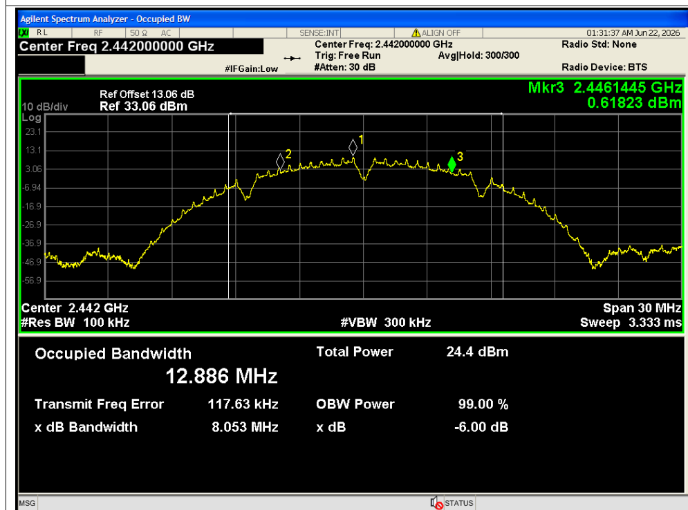
-6dB Bandwidth NVNT b 2442MHz Ant1
