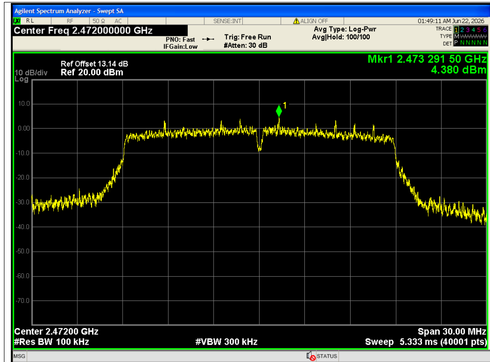
Tx. Spurious NVNT n20 2472MHz Ant1 Ref
