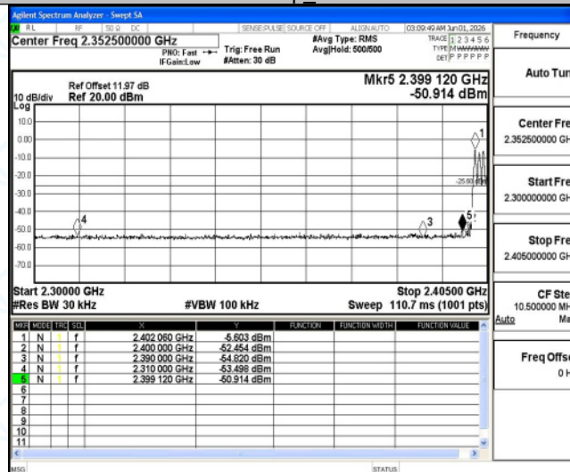
DH5-Ant1-Hop_2402-PASS
