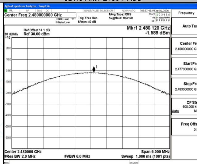
3DH5-Ant1-2480-PASS
