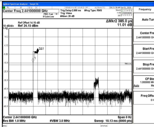
2DH3-Ant1-Hop-PASS
