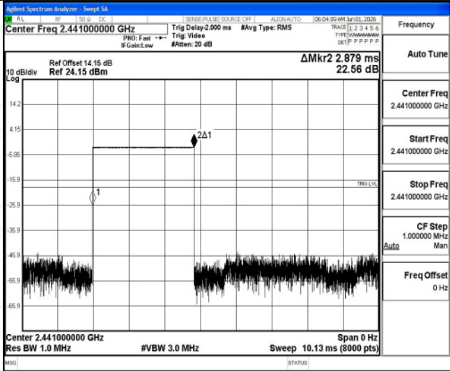
DH5-Ant1-Hop-PASS
