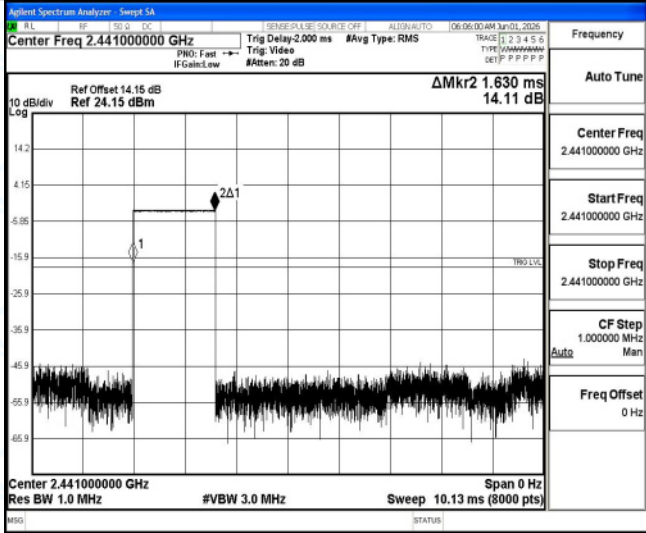
DH3-Ant1-Hop-PASS
