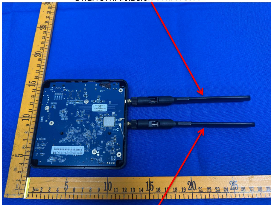
2.4GWIFI/5.2G/5.8GWIFI-ANT2
