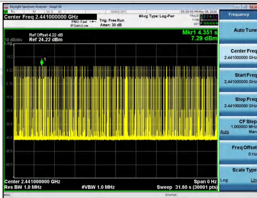
Dwell_Time_(Hopping)_NVNT_ANT1_3-DH1_2441_00_One_Burst_Time
