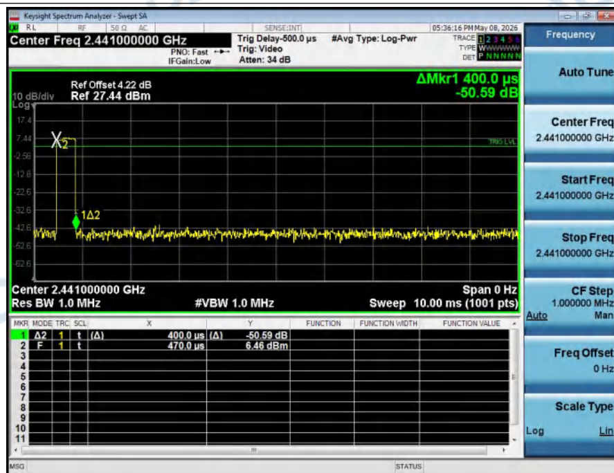
Dwell_Time_(Hopping)_NVNT_ANT1_3-DH1_2441_00_Accumulated
