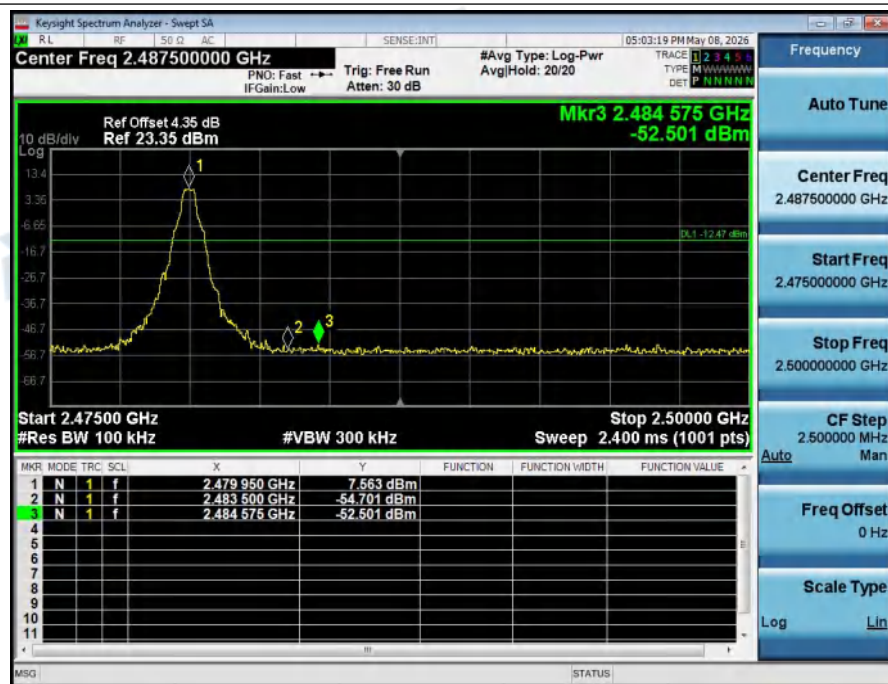
1_Reference_Level_Hopping_NVNT_ANT1_2-DH5_Hopping
