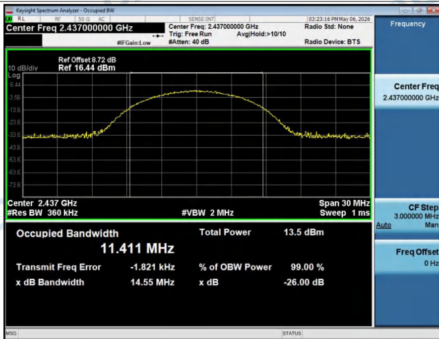
99%_Occupied_Bandwidth_NVNT_ANT2_802_11b_2437
