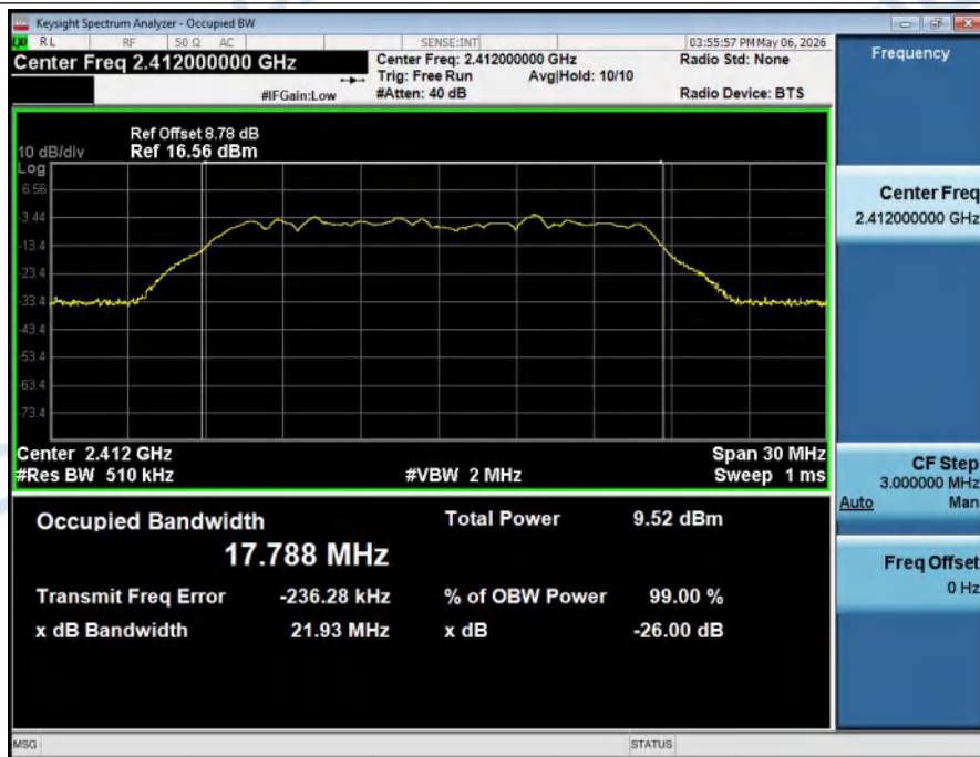
99%_Occupied_Bandwidth_NVNT_ANT2_802_11n(HT20)_2412
