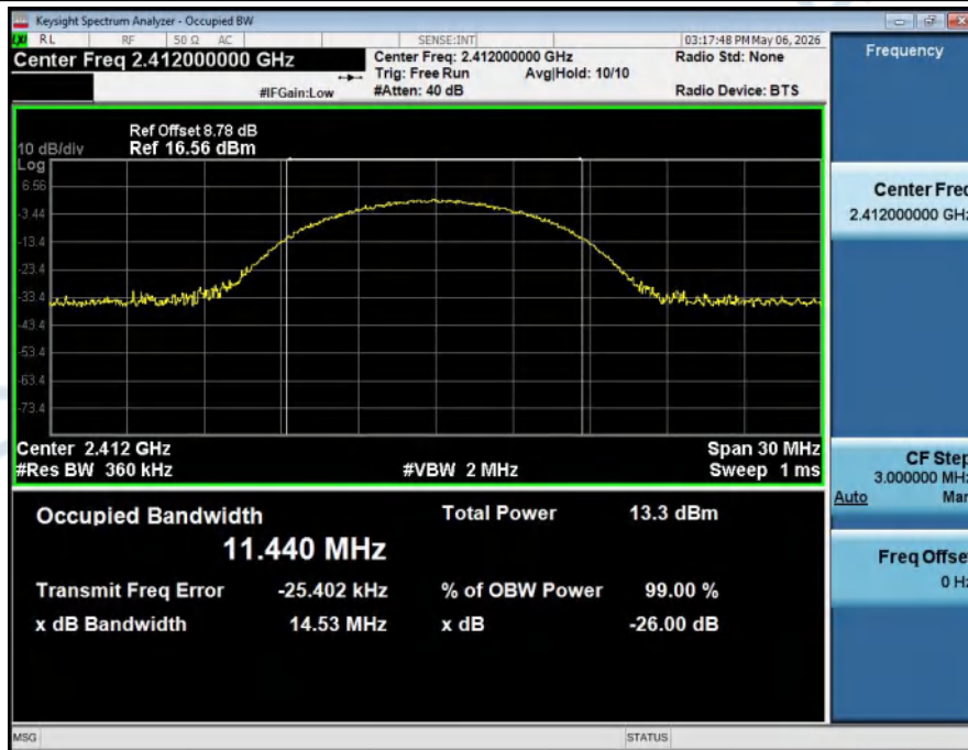
99%_Occupied_Bandwidth_NVNT_ANT2_802_11b_2412
