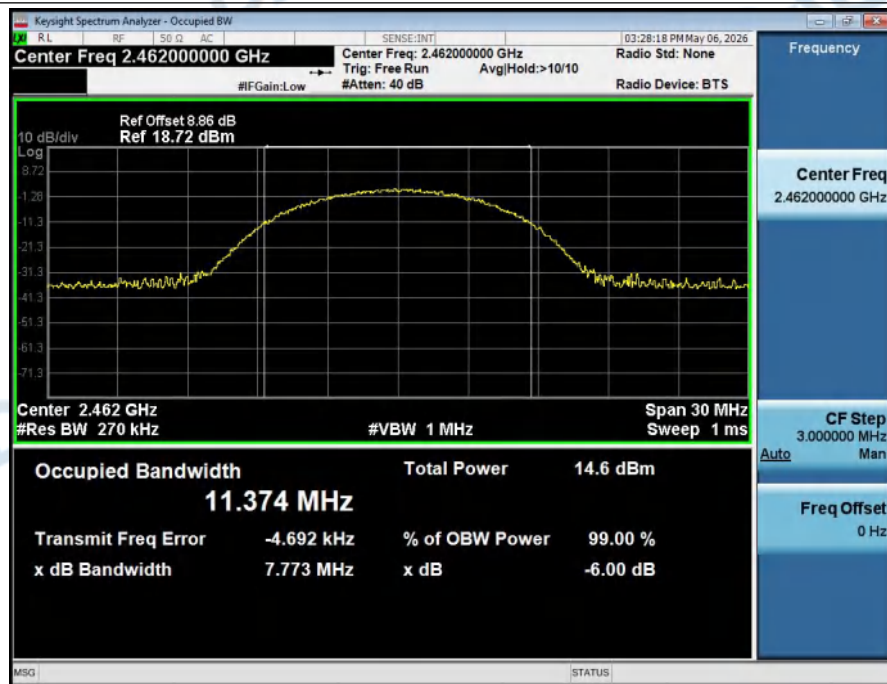
-6dB_Bandwidth_NVNT_ANT2_802_11b_2462
