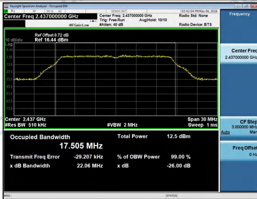
99%_Occupied_Bandwidth_NVNT_ANT2_802_11g_2437
