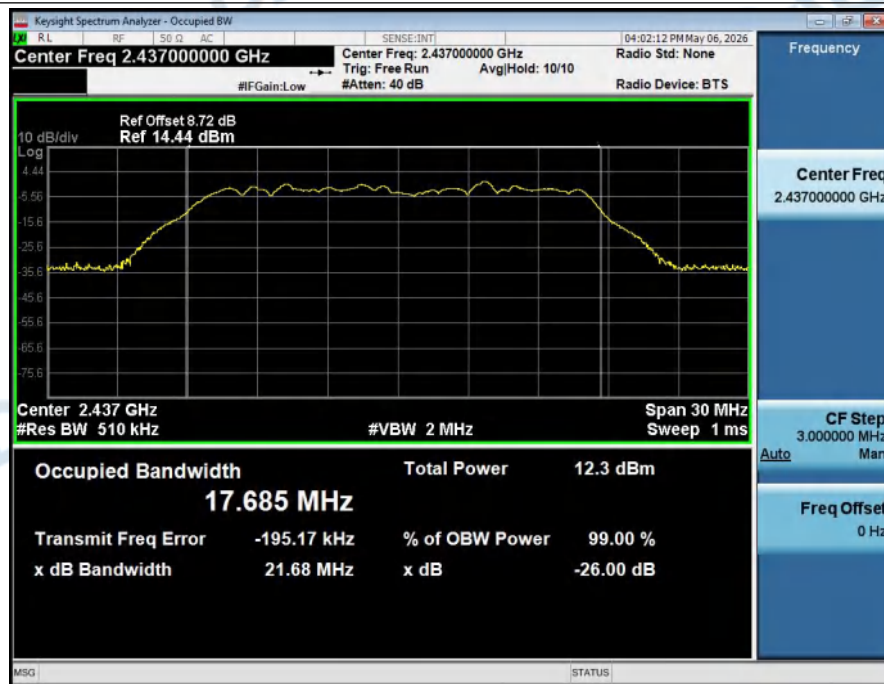
99%_Occupied_Bandwidth_NVNT_ANT2_802_11n(HT20)_2437
