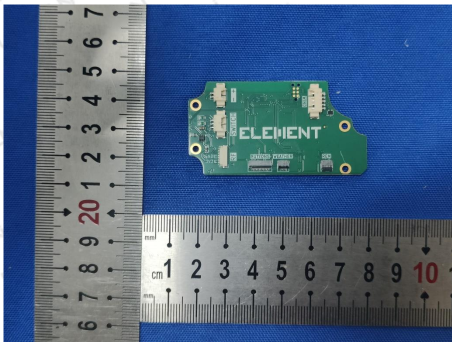
Multilayer Chip Antenna
