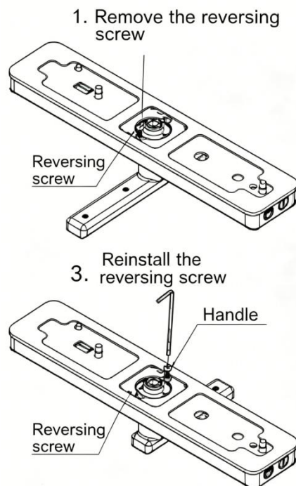
Handle Reversal Diagram
