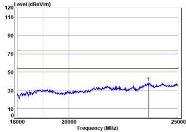
BLE_1M_TX_CH_00_Horizontal-Peak
