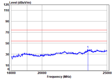
BLE_1M_TX_CH_00_Vertical-Peak
