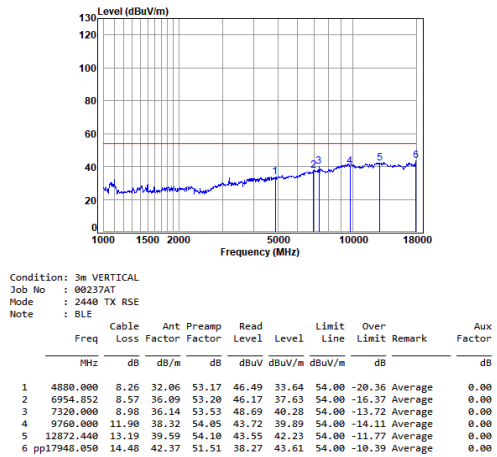
BLE_1M_TX_CH_19_Vertical-Avg
