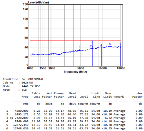
BLE_1M_TX_CH_19_Horizontal-Avg
