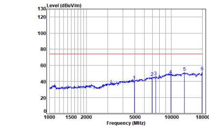
BLE_1M_TX_CH_39_Vertical-Peak
