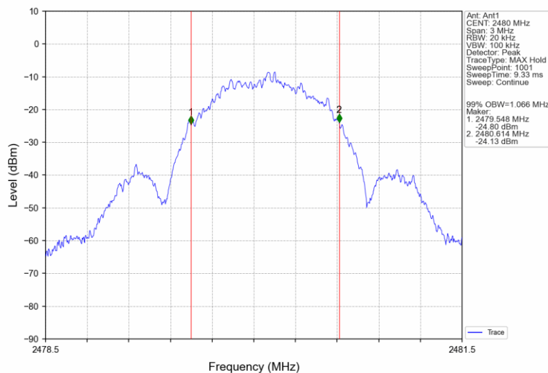
1M_HCH_2480MHz_Ant1_NTNV
