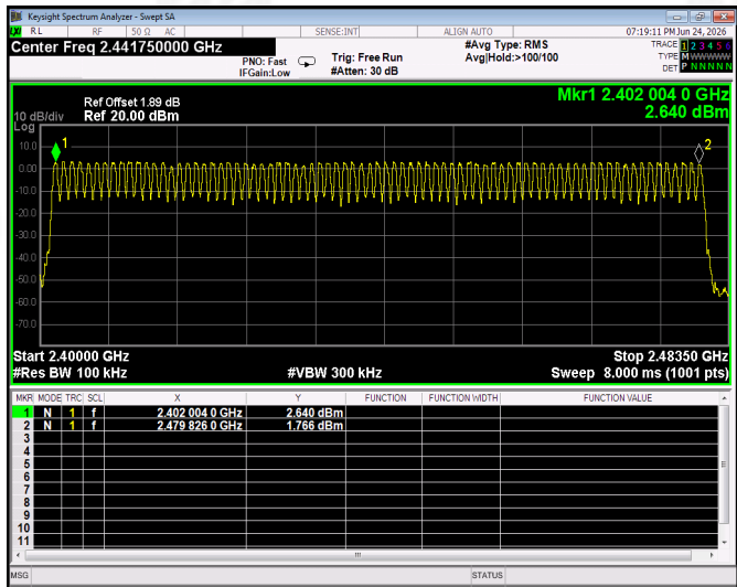
π/4-DQPSK - 2-DH1 Test Plots
