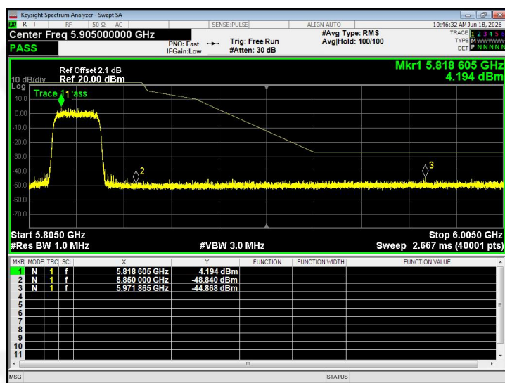
(802.11ax20) Band Edge, Right Side
