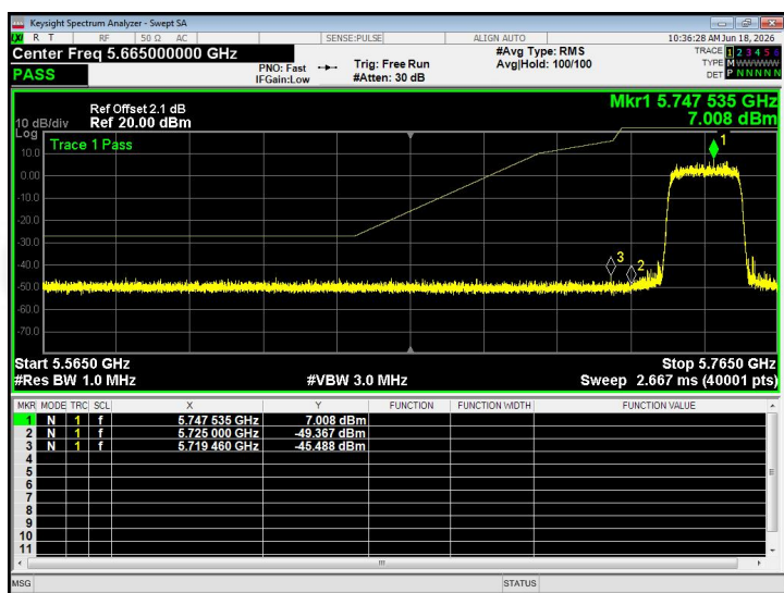
(802.11ax20) Band Edge, Left Side
