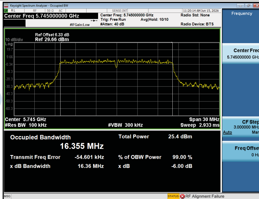
-6dB_Emission_Bandwidth_NVNT_ANT1_802_11a_5745_20M
