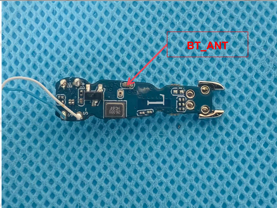
Right ear headphones_BT_Antenna
